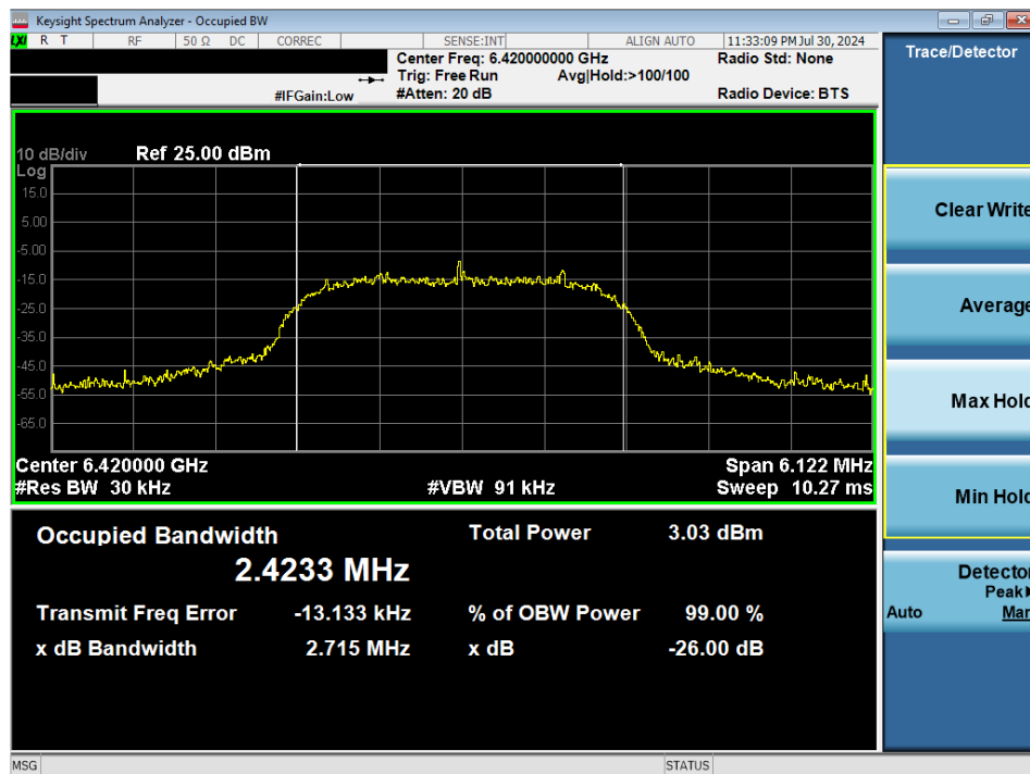
Plot 7-15. 26dB BW & 99% OBW (NB UNII HDRp4 – 6420MHz)
