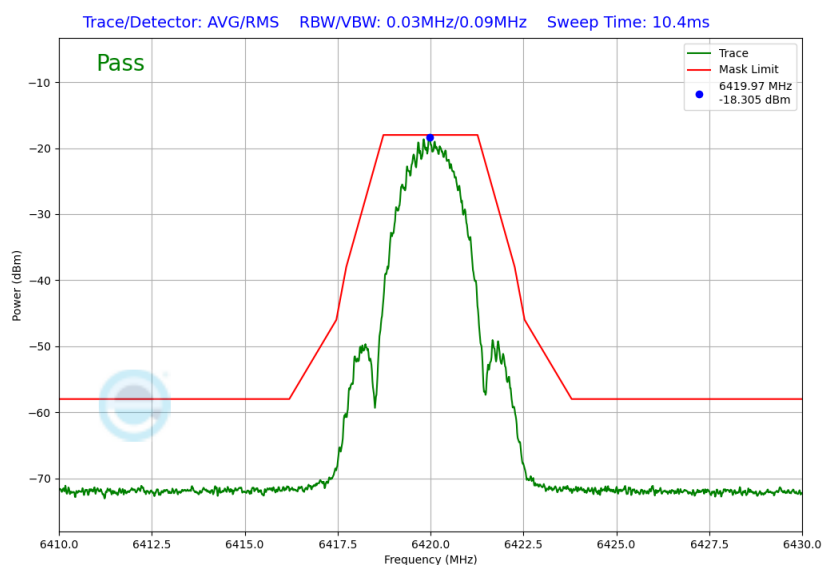
Plot 7-42. VLP In-Band Emission Plot (NB UNII LE, 2Mbps – 6420MHz)
