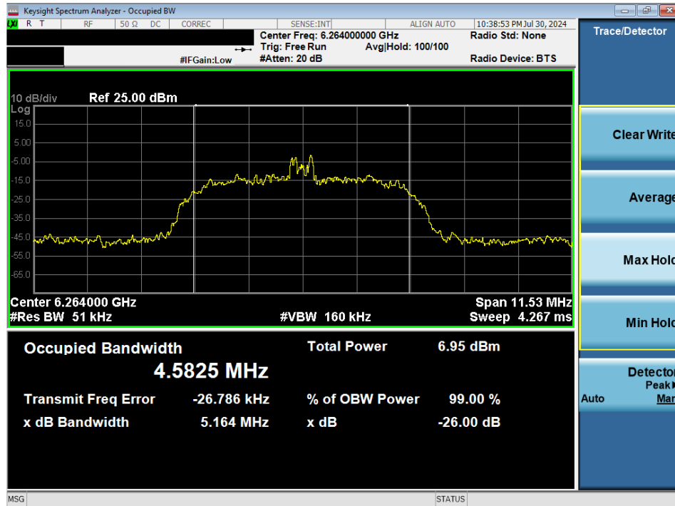
Plot 7-11. 26dB BW & 99% OBW (NB UNII HDR8 – 6264MHz)
