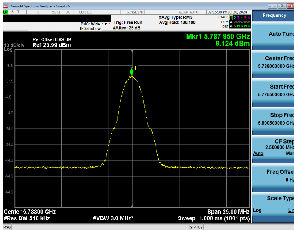
Plot 7-59. PSD (NB UNII LE2M – 5788MHz)
