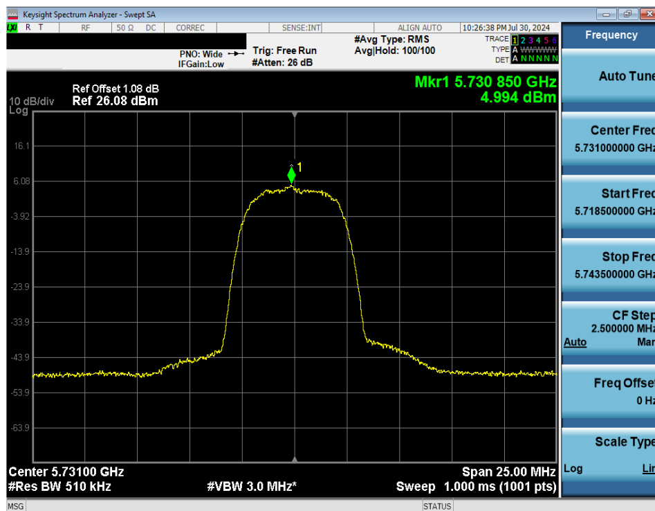
Plot 7-64. PSD (NB UNII HDR8 – 5731MHz)
