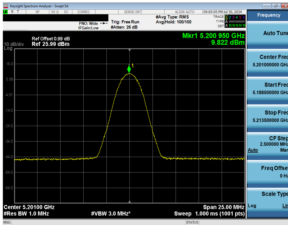
Plot 7-41. FCC PSD (NB UNII LE2M – 5201MHz)
