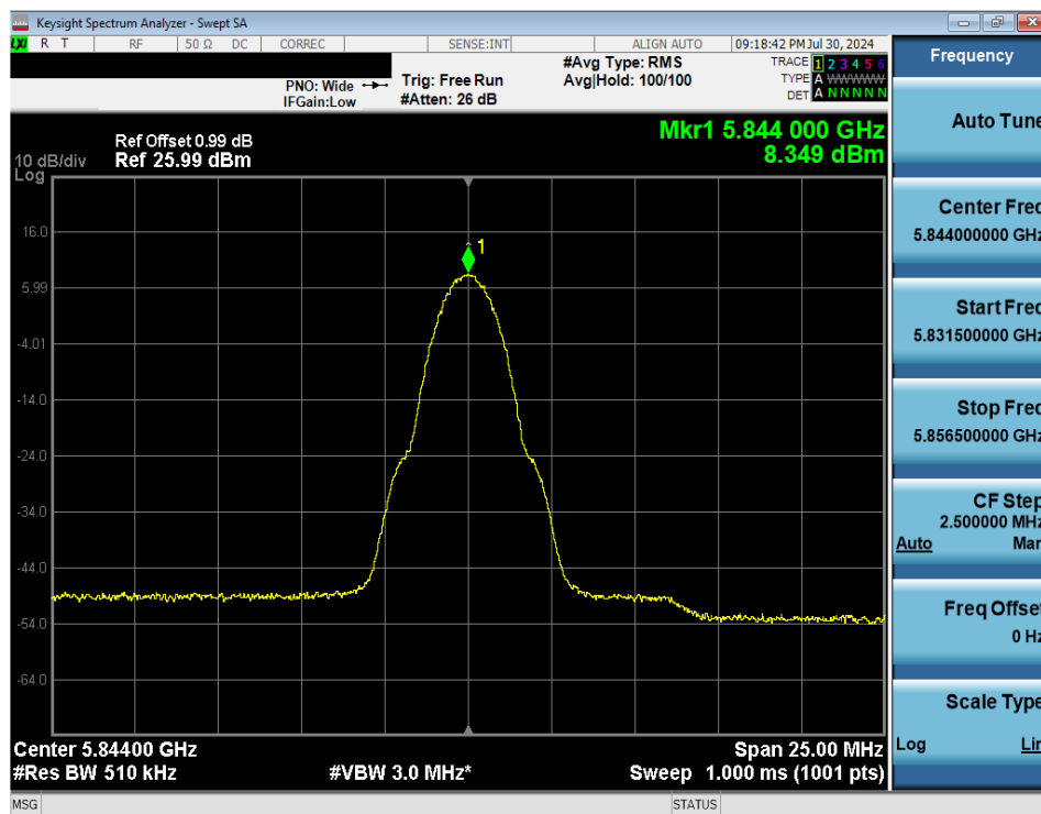
Plot 7-60. PSD (NB UNII LE2M – 5844MHz)
