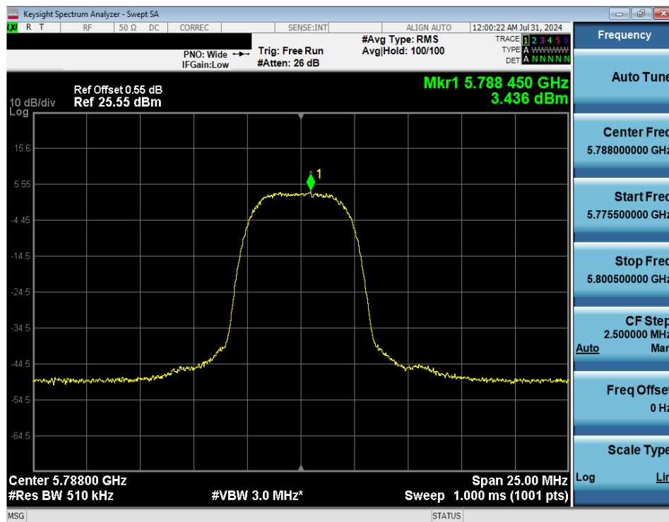
Plot 7-71. PSD (NB UNII HDRp8 – 5788MHz)
