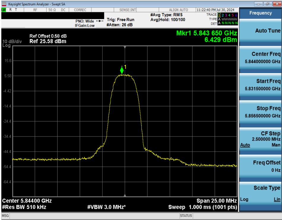
Plot 7-69. PSD (NB UNII HDRp4 – 5844MHz)
