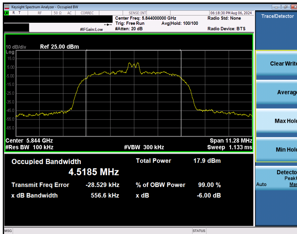
Plot 7-30. 6dB BW & 99% OBW (NB UNII HDR8 – 5844MHz)
