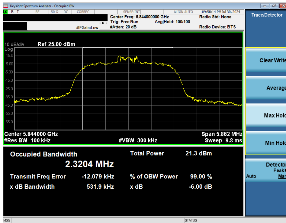
Plot 7-27. 6dB BW & 99% OBW (NB UNII HDR4 – 5844MHz)
