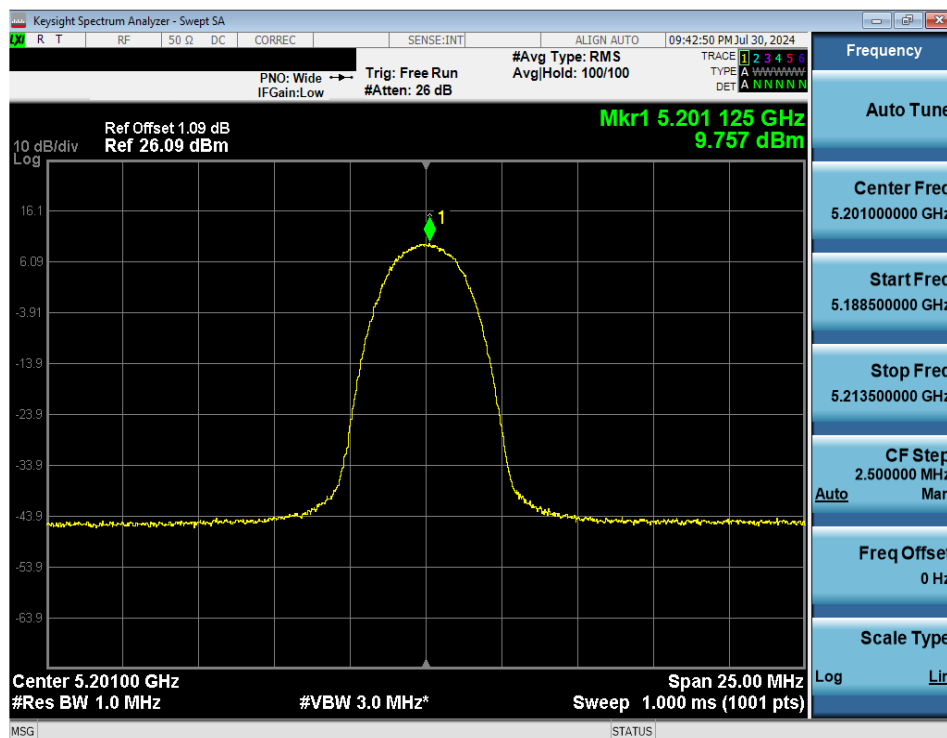
Plot 7-44. FCC PSD (NB UNII HDR4 – 5201MHz)
