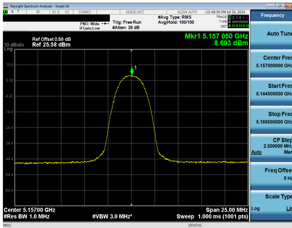
7-49. FCC PSD (NB UNII HDRp4 – 5157MHz)
