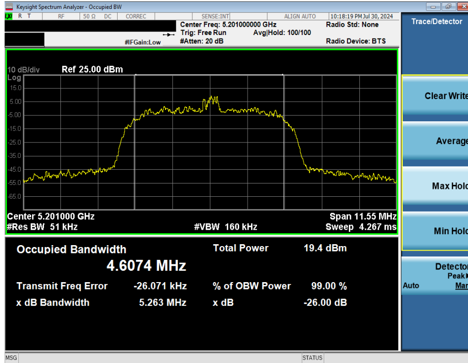
Plot 7-11. 26dB BW & 99% OBW (NB UNII HDR8 – 5201MHz)
