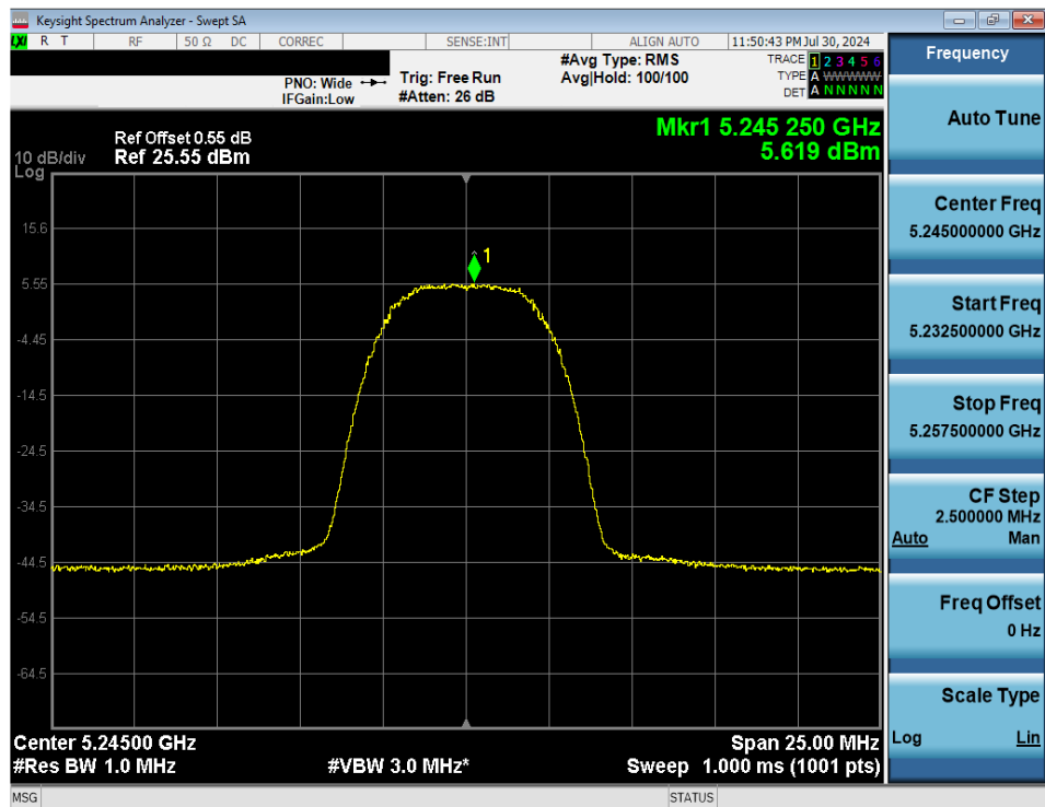
Plot 7-54. FCC PSD (NB UNII HDRp8 – 5245MHz)
