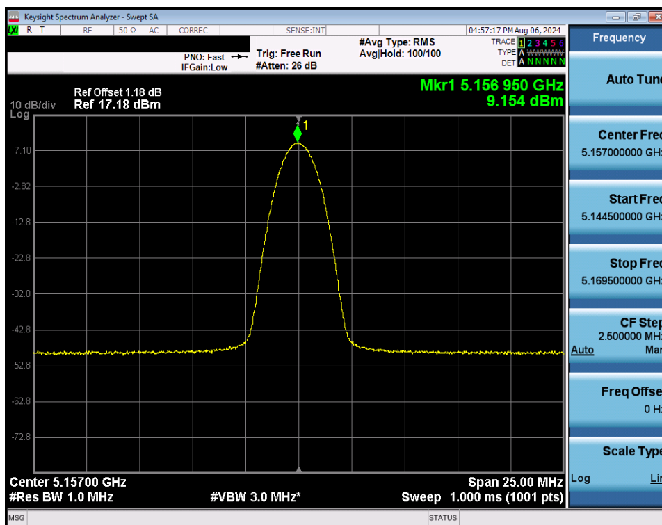
Plot 7-37. FCC PSD (NB UNII BDR – 5157MHz)
