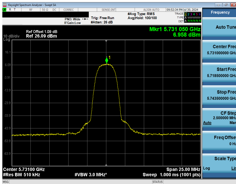
Plot 7-61. PSD (NB UNII HDR4 – 5731MHz)
