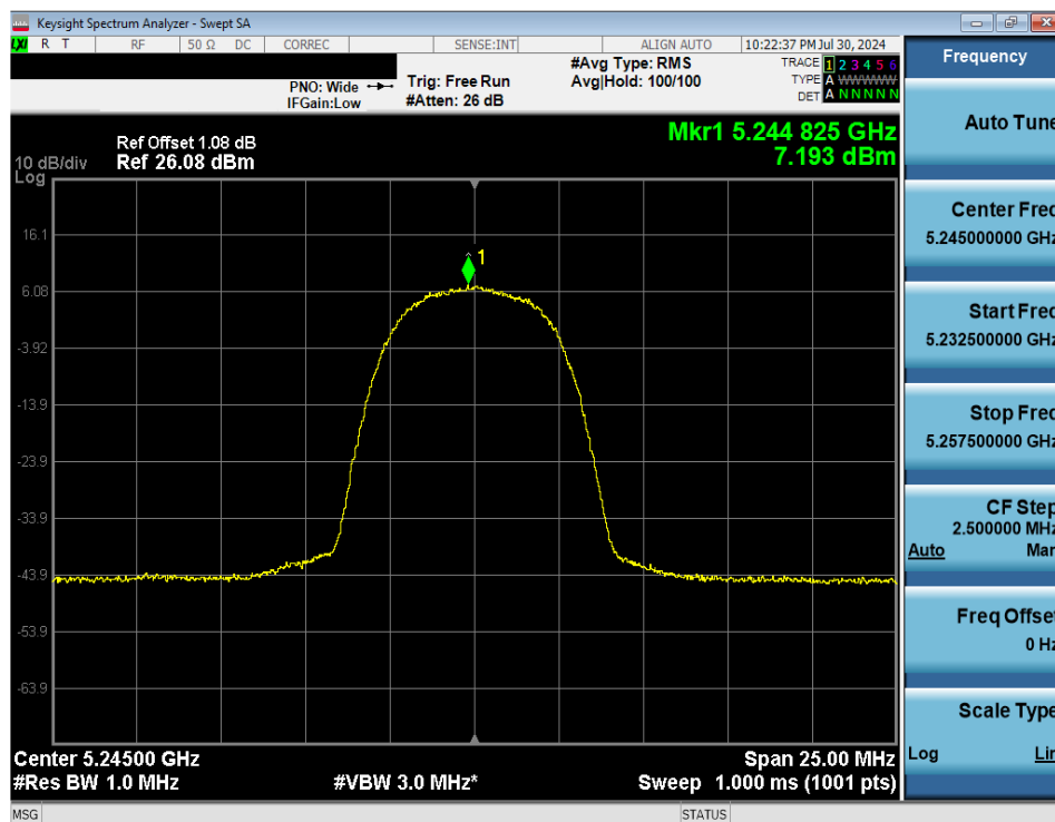
Plot 7-48. FCC PSD (NB UNII HDR8 – 5245MHz)
