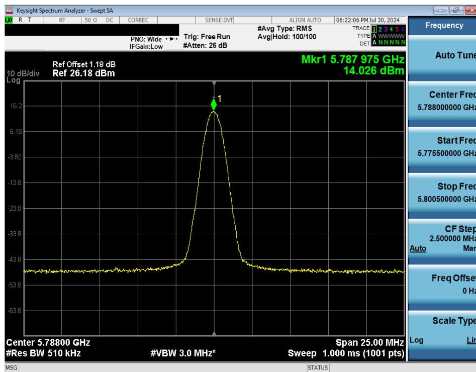
Plot 7-56. PSD (NB UNII BDR – 5788MHz)
