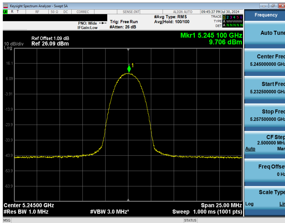
Plot 7-45. FCC PSD (NB UNII HDR4 – 5245MHz)
