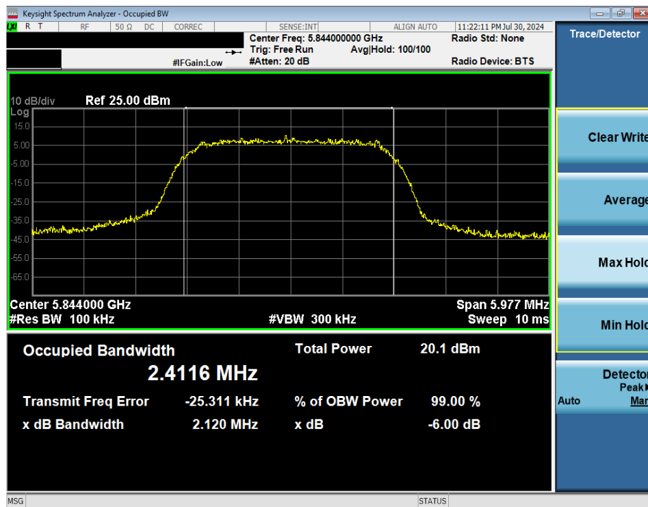
Plot 7-33. 6dB BW & 99% OBW (NB UNII HDRp4 – 5844MHz)
