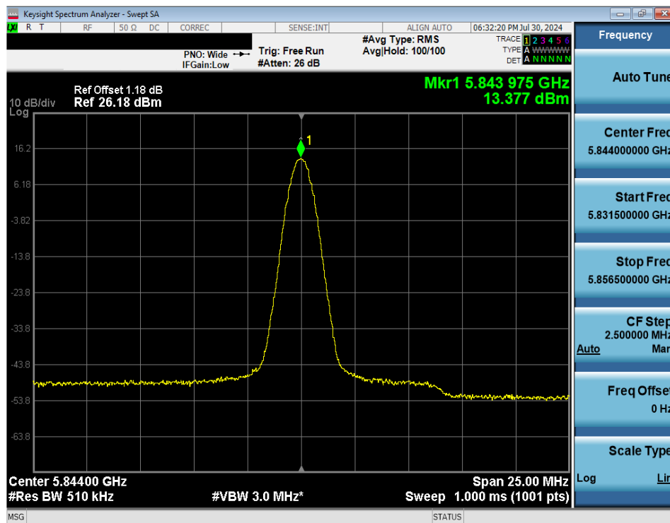
Plot 7-57. PSD (NB UNII BDR – 5844MHz)
