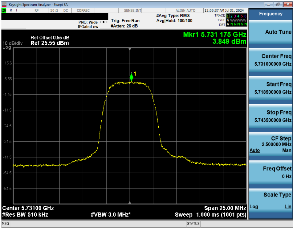
Plot 7-70. PSD (NB UNII HDRp8 – 5731MHz)
