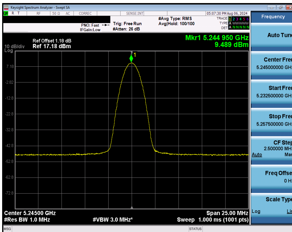
Plot 7-39. FCC PSD (NB UNII BDR – 5245MHz)
