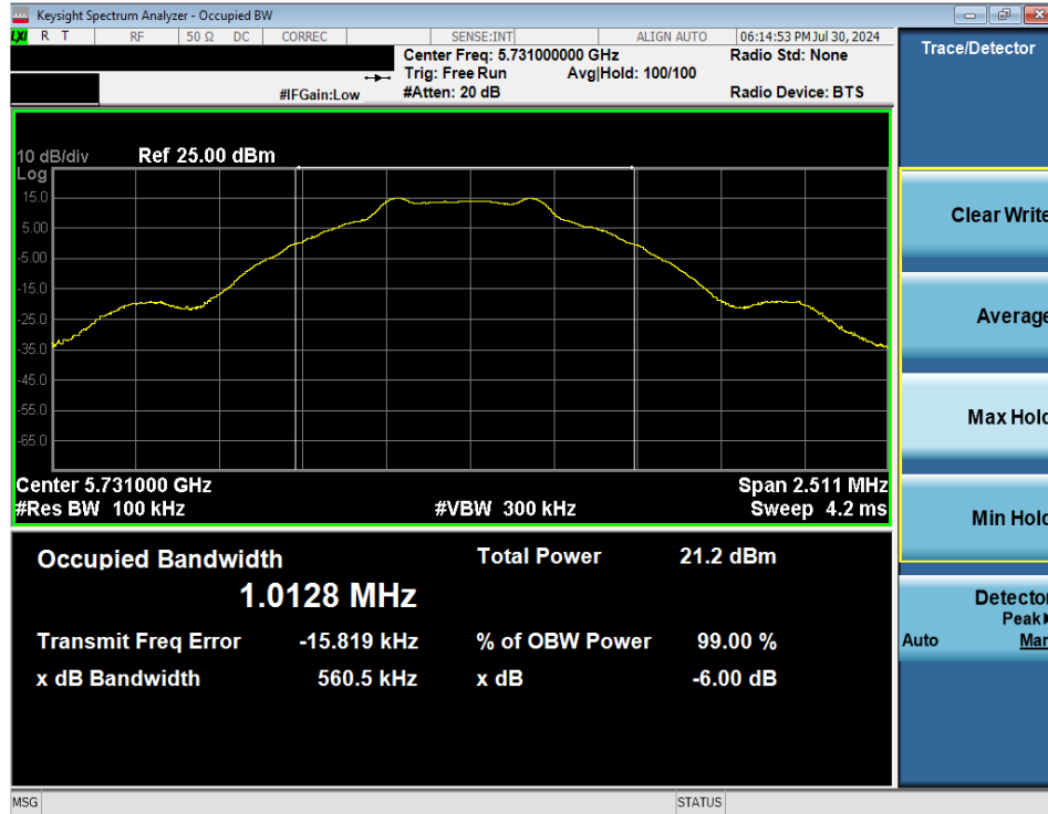
Plot 7-19. 6dB BW & 99% OBW (NB UNII BDR – 5731MHz)
