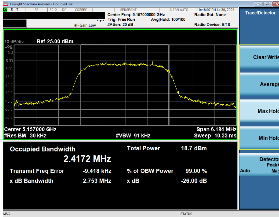
Plot 7-13. 26dB BW & 99% OBW (NB UNII HDRp4 – 5157MHz)
