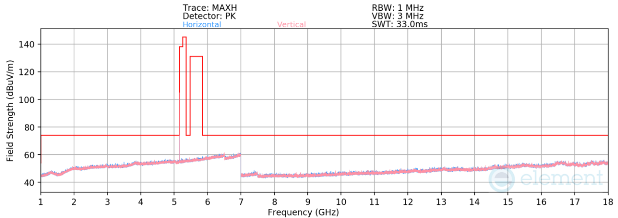
Plot 7-73. Radiated Spurious Emissions 1-18GHz (NB UNII BDR – 5157MHz)
