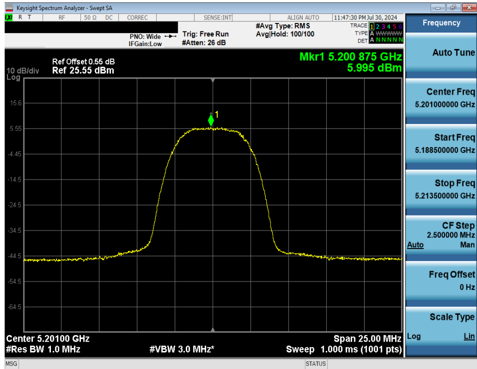
Plot 7-53. FCC PSD (NB UNII HDRp8 – 5201MHz)
