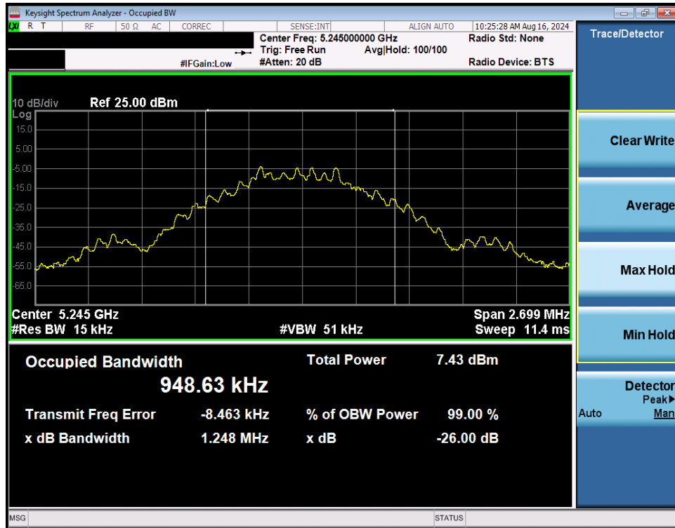
Plot 7-3. 26dB BW & 99% OBW (NB UNII BDR – 5245MHz)
