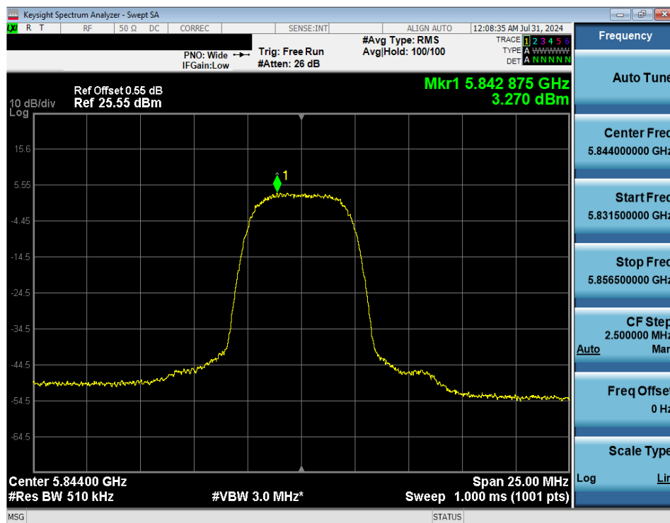
Plot 7-72. PSD (NB UNII HDRp8 – 5844MHz)
