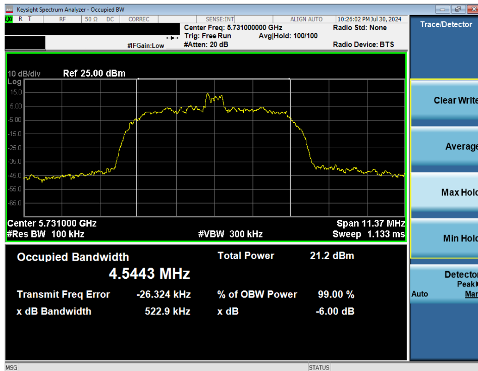
Plot 7-28. 6dB BW & 99% OBW (NB UNII HDR8 – 5731MHz)
