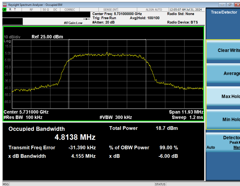
Plot 7-34. 6dB BW & 99% OBW (NB UNII HDRp8 – 5731MHz)
