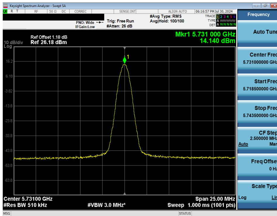
Plot 7-55. PSD (NB UNII BDR – 5731MHz)
