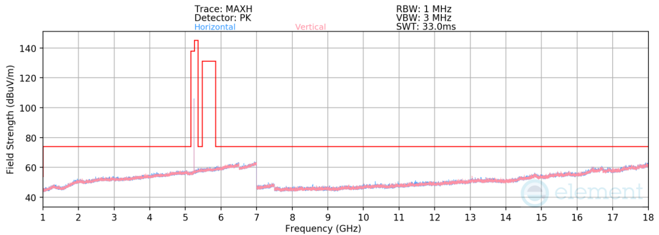
Plot 7-84. Radiated Spurious Emissions 1-18GHz (NB UNII HDR4 – 5245MHz)
