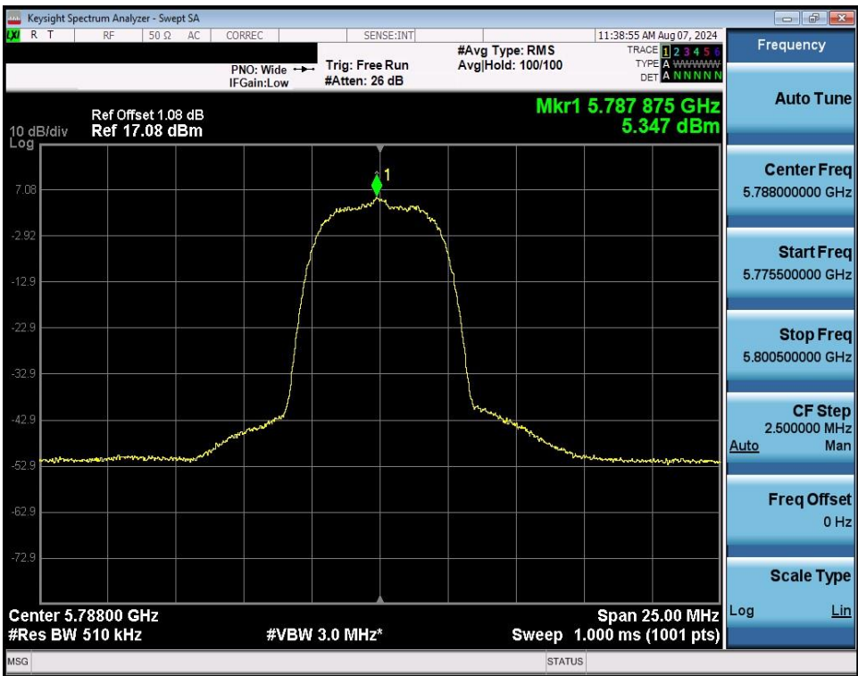
Plot 7-65. PSD (NB UNII HDR8 – 5788MHz)
