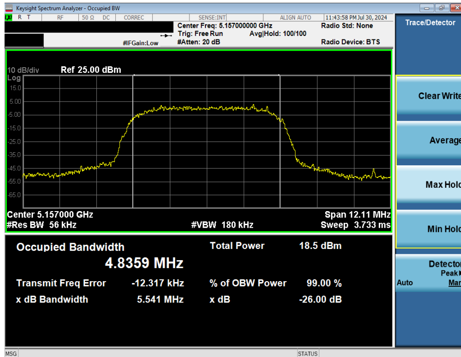
Plot 7-16. 26dB BW & 99% OBW (NB UNII HDRp8 – 5157MHz)
