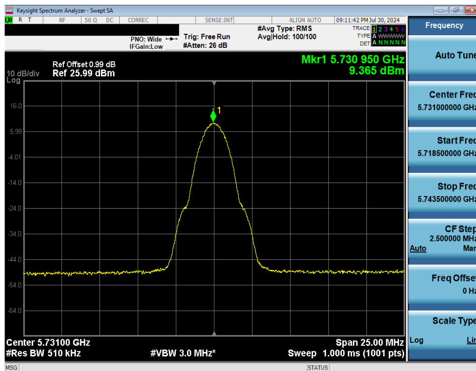
Plot 7-58. PSD (NB UNII LE2M – 5731MHz)
