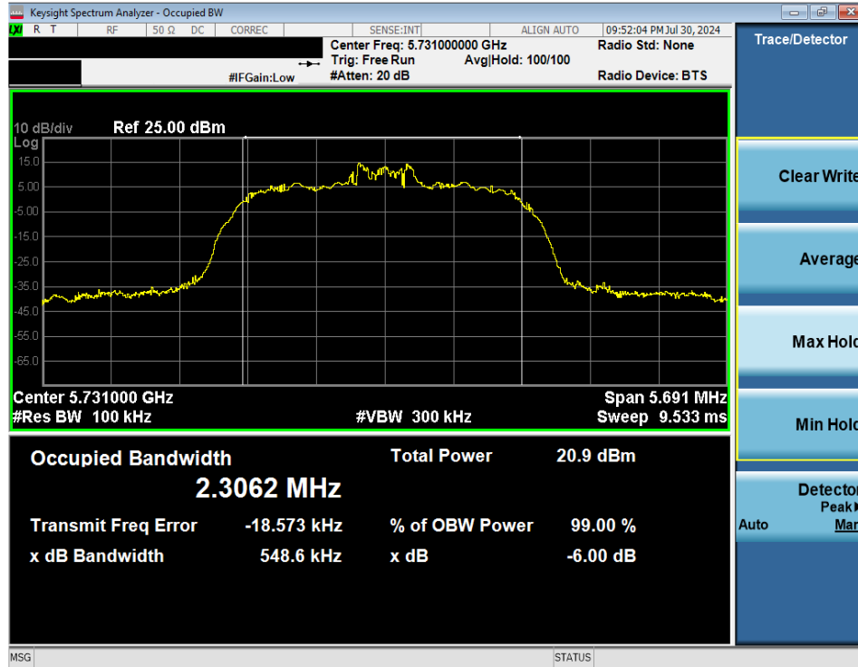
Plot 7-25. 6dB BW & 99% OBW (NB UNII HDR4 – 5731MHz)
