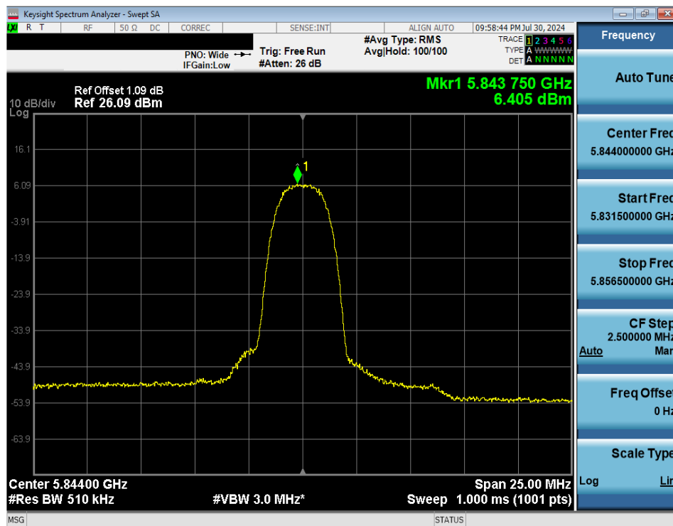
Plot 7-63. PSD (NB UNII HDR4 – 5844MHz)
