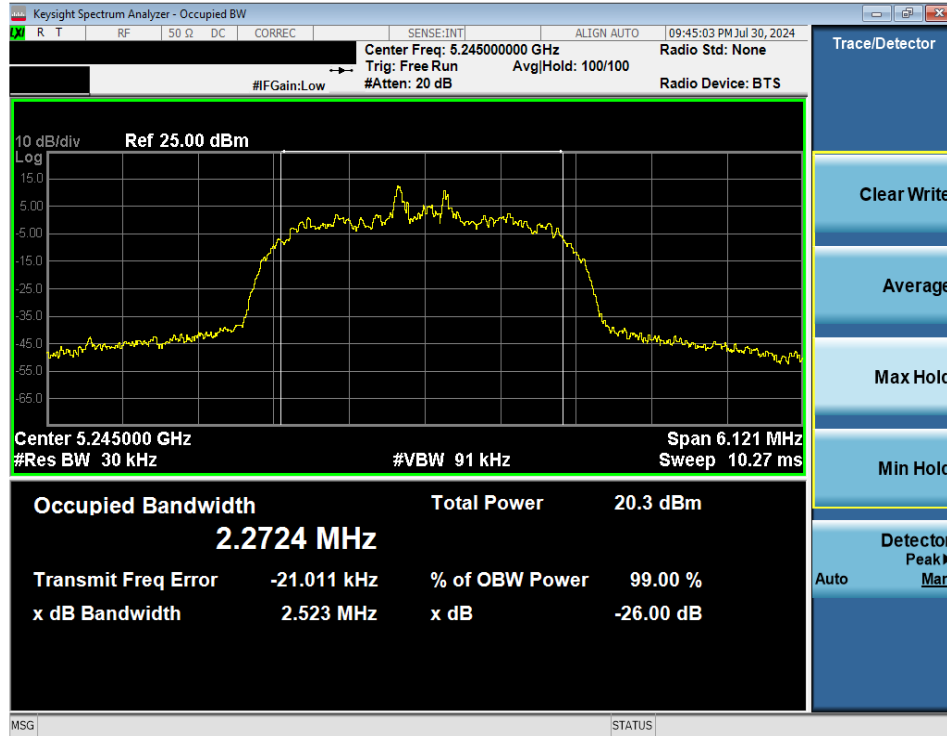
Plot 7-9. 26dB BW & 99% OBW (NB UNII HDR4 – 5245MHz)
