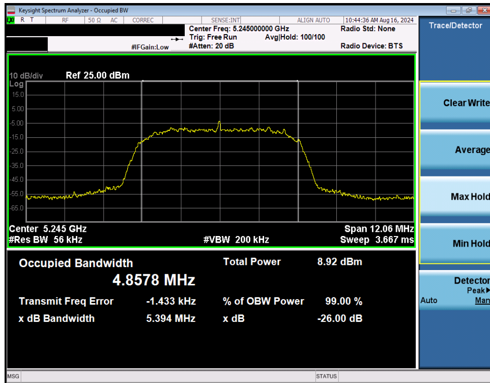
Plot 7-18. 26dB BW & 99% OBW (NB UNII HDRp8 – 5245MHz)
