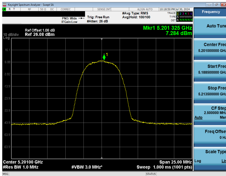
Plot 7-47. FCC PSD (NB UNII HDR8 – 5201MHz)
