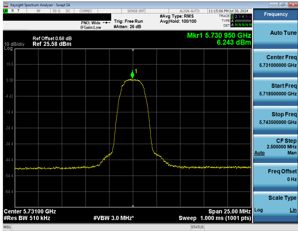
Plot 7-67. PSD (NB UNII HDRp4 – 5731MHz)
