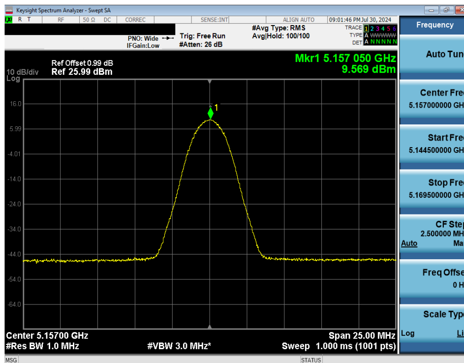
7-40. FCC PSD (NB UNII LE2M – 5157MHz)
