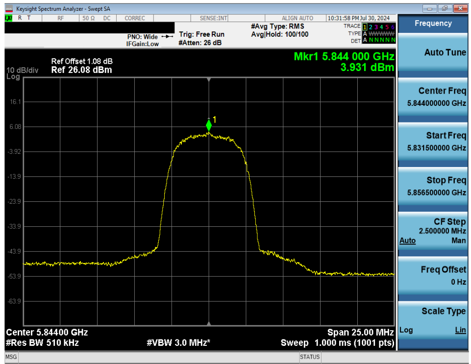
Plot 7-66. PSD (NB UNII HDR8 – 5844MHz)
