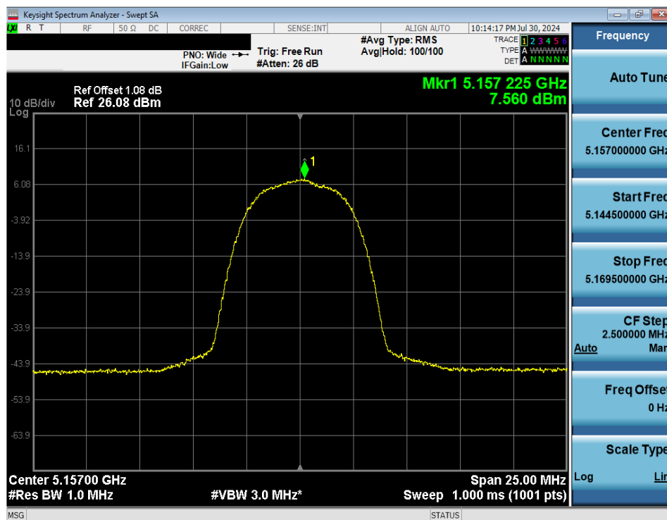
7-46. FCC PSD (NB UNII HDR8 – 5157MHz)
