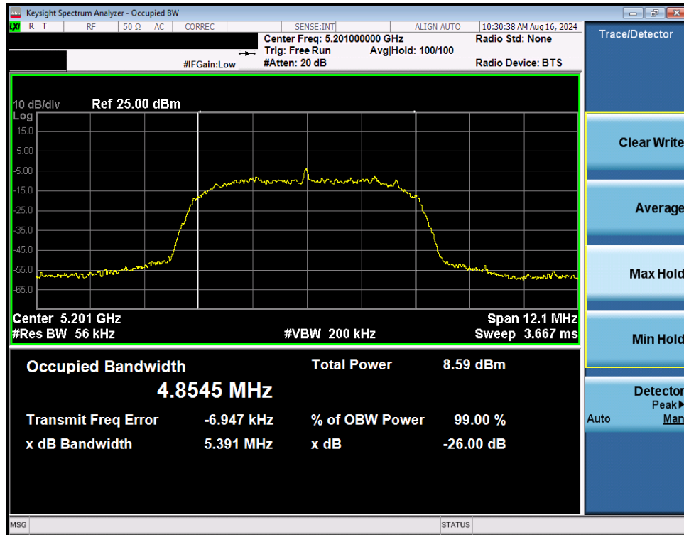
Plot 7-17. 26dB BW & 99% OBW (NB UNII HDRp8 – 5201MHz)
