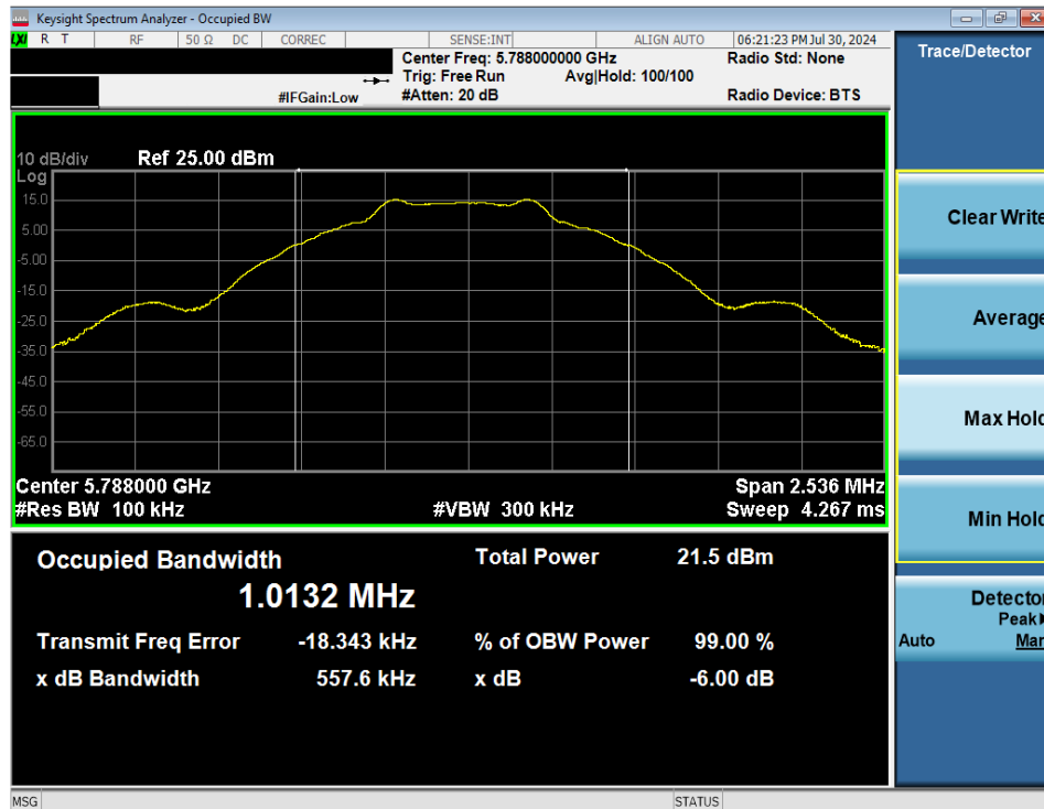
Plot 7-20. 6dB BW & 99% OBW (NB UNII BDR – 5788MHz)
