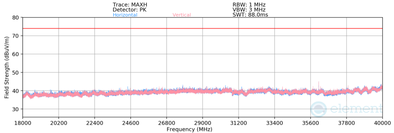
Plot 7-74. Radiated Spurious Emissions 18-40GHz (NB UNII BDR – 5157MHz)
