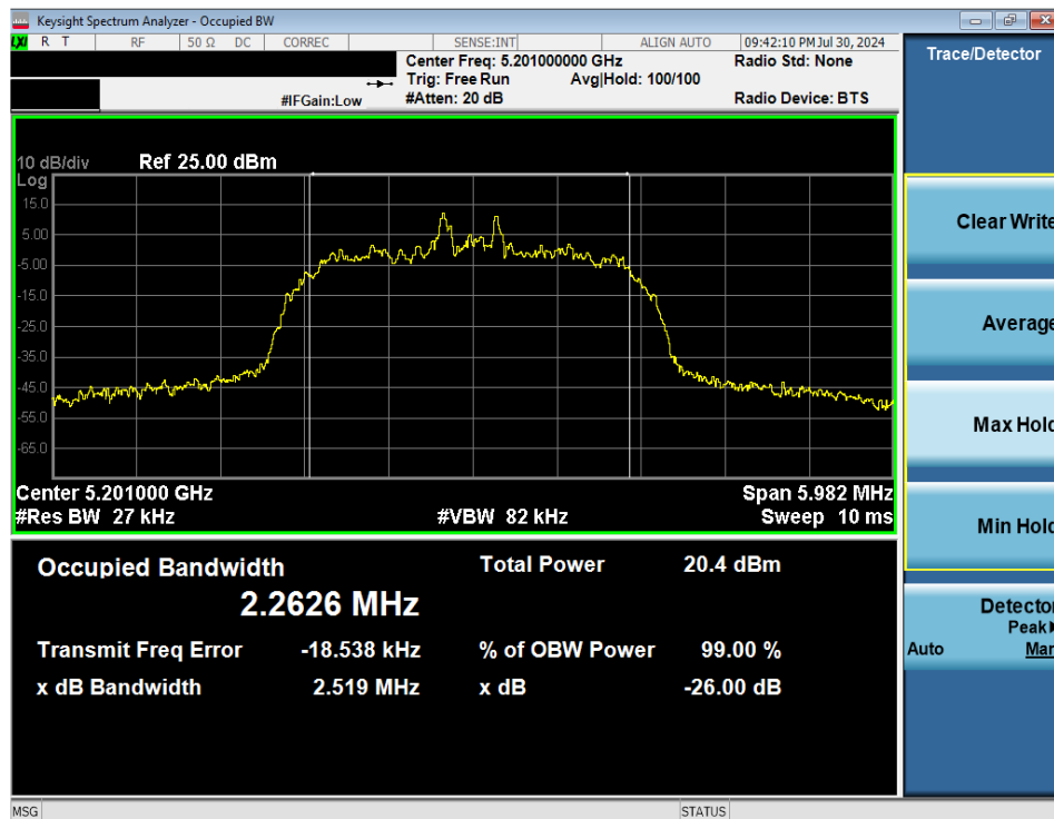
Plot 7-8. 26dB BW & 99% OBW (NB UNII HDR4 – 5201MHz)
