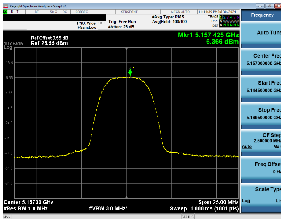
7-52. FCC PSD (NB UNII HDRp8 – 5157MHz)
