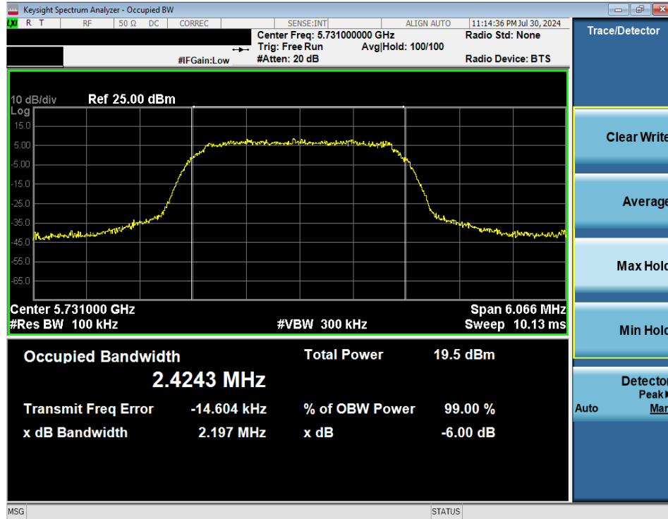
Plot 7-31. 6dB BW & 99% OBW (NB UNII HDRp4 – 5731MHz)
