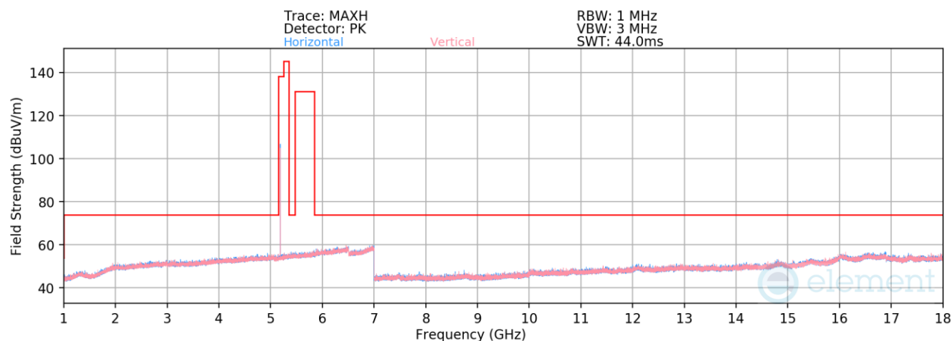
Plot 7-80. Radiated Spurious Emissions 1-18GHz (NB UNII LE2M – 5245MHz)
