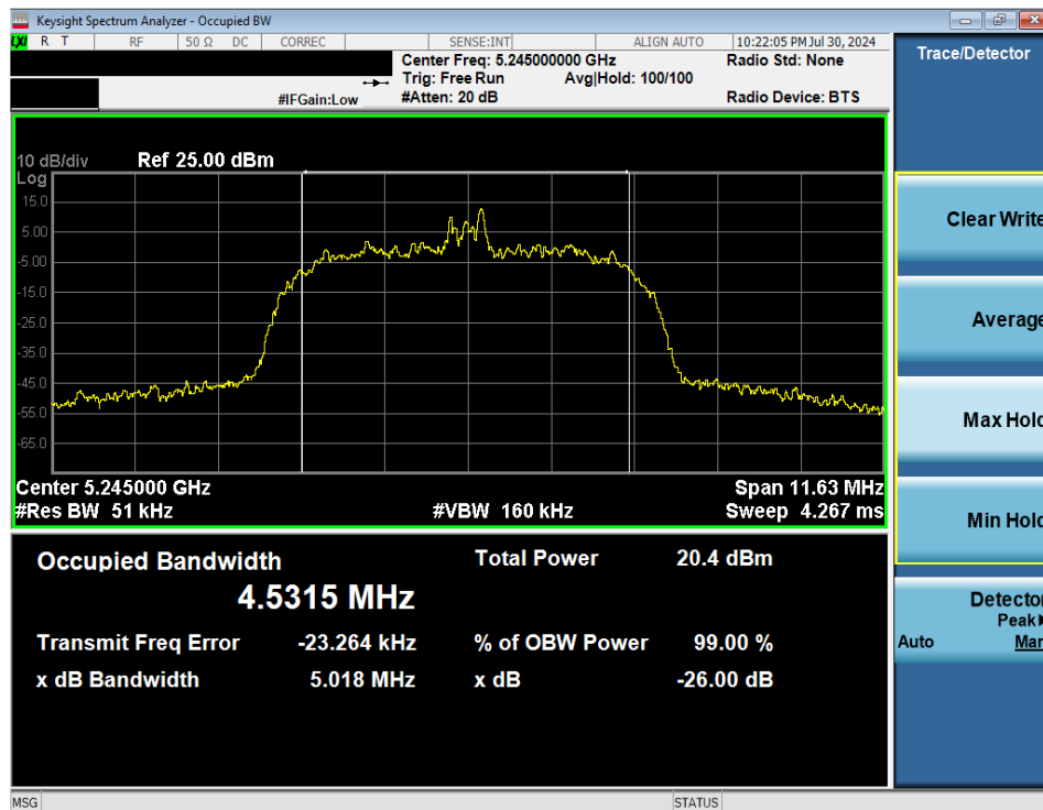
Plot 7-12. 26dB BW & 99% OBW (NB UNII HDR8 – 5245MHz)
