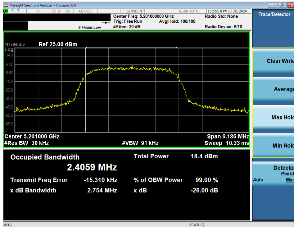
Plot 7-14. 26dB BW & 99% OBW (NB UNII HDRp4 – 5201MHz)
