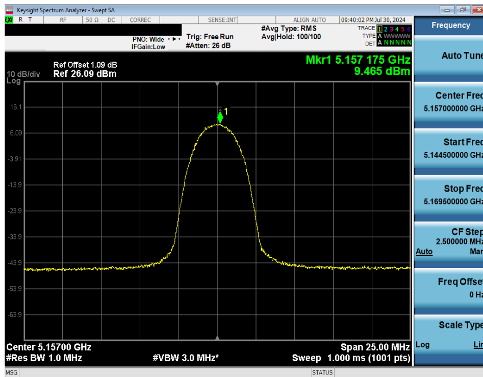
7-43. FCC PSD (NB UNII HDR4 – 5157MHz)
