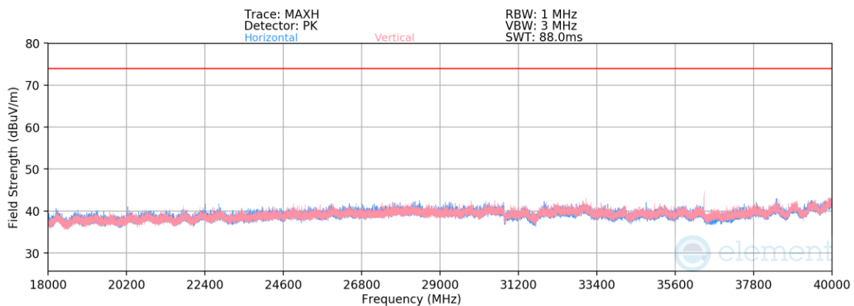
Plot 7-83. Radiated Spurious Emissions 18-40GHz (NB UNII HDR4 – 5201MHz)
