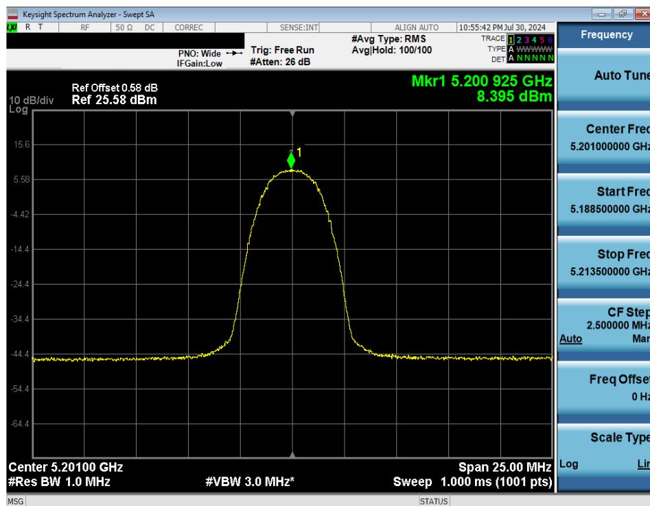
Plot 7-50. FCC PSD (NB UNII HDRp4 – 5201MHz)
