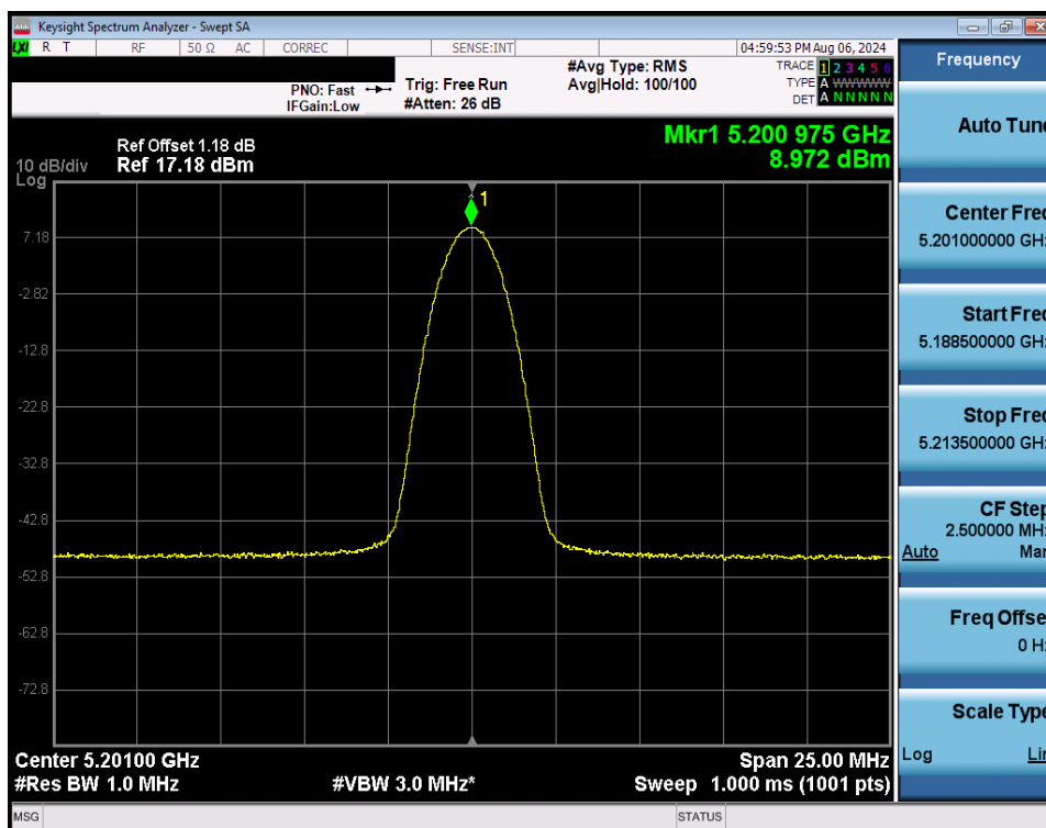
Plot 7-38. FCC PSD (NB UNII BDR – 5201MHz)
