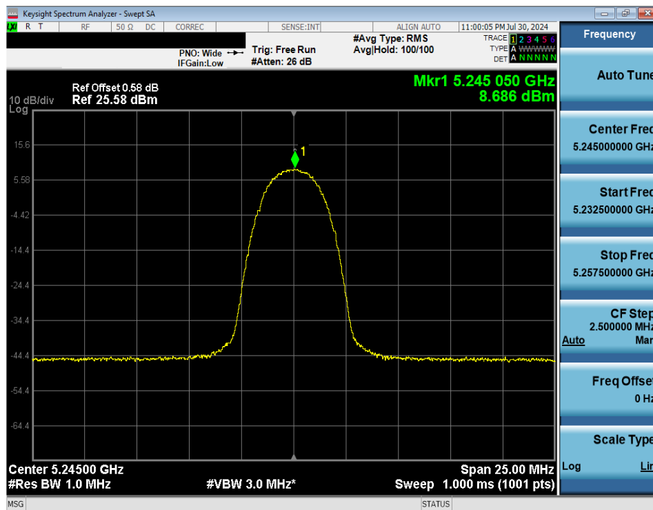
Plot 7-51. FCC PSD (NB UNII HDRp4 – 5245MHz)
