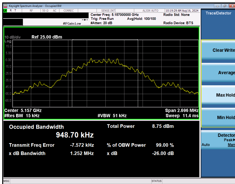
Plot 7-1. 26dB BW & 99% OBW (NB UNII BDR – 5157MHz)
