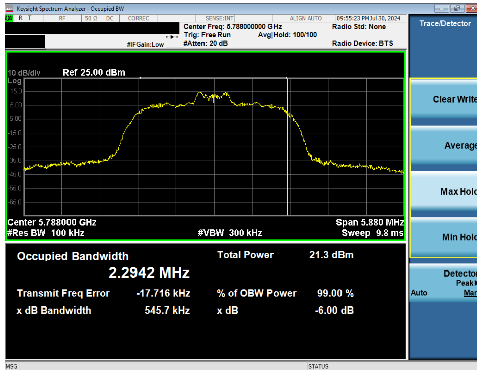
Plot 7-26. 6dB BW & 99% OBW (NB UNII HDR4 – 5788MHz)
