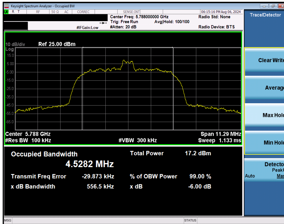
Plot 7-29. 6dB BW & 99% OBW (NB UNII HDR8 – 5788MHz)
