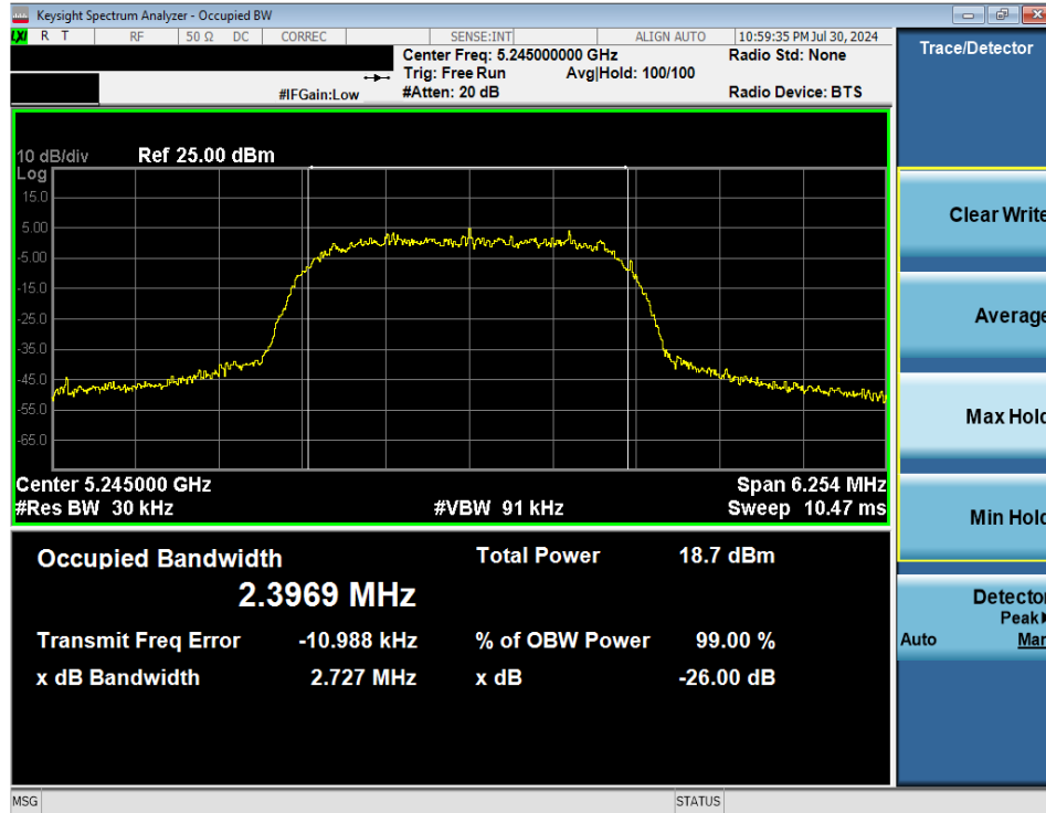
Plot 7-15. 26dB BW & 99% OBW (NB UNII HDRp4 – 5245MHz)
