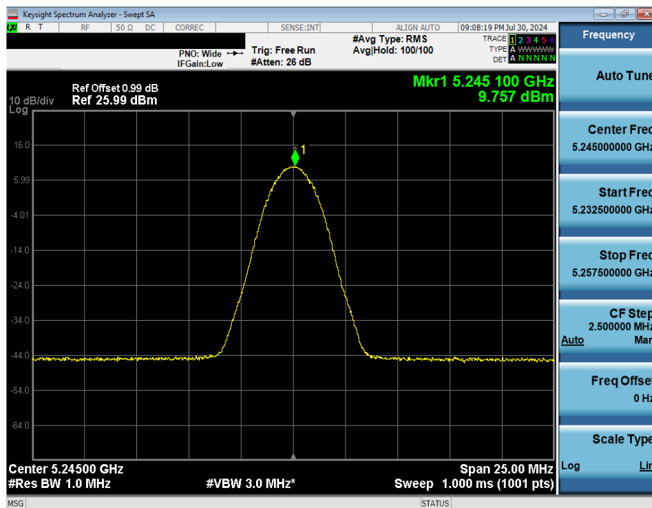
Plot 7-42. FCC PSD (NB UNII LE2M – 5245MHz)
