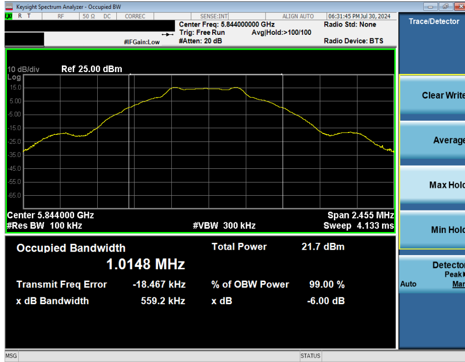
Plot 7-21. 6dB BW & 99% OBW (NB UNII BDR – 5844MHz)
