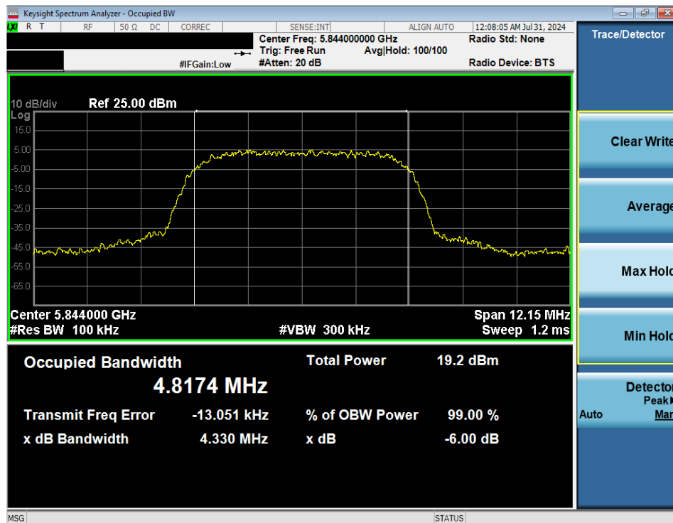
Plot 7-36. 6dB BW & 99% OBW (NB UNII HDRp8 – 5844MHz)
