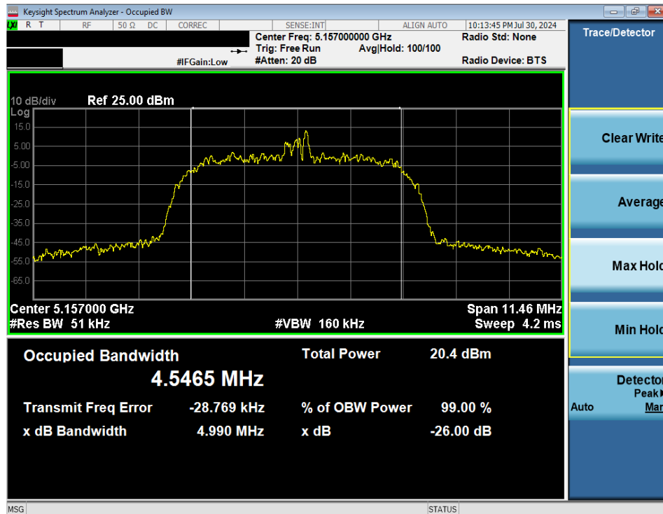
Plot 7-10. 26dB BW & 99% OBW (NB UNII HDR8 – 5157MHz)
