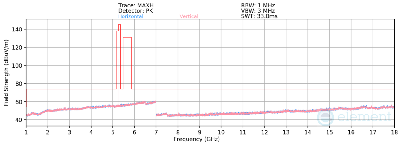
Plot 7-76. Radiated Spurious Emissions 1-18GHz (NB UNII BDR – 5245MHz)
