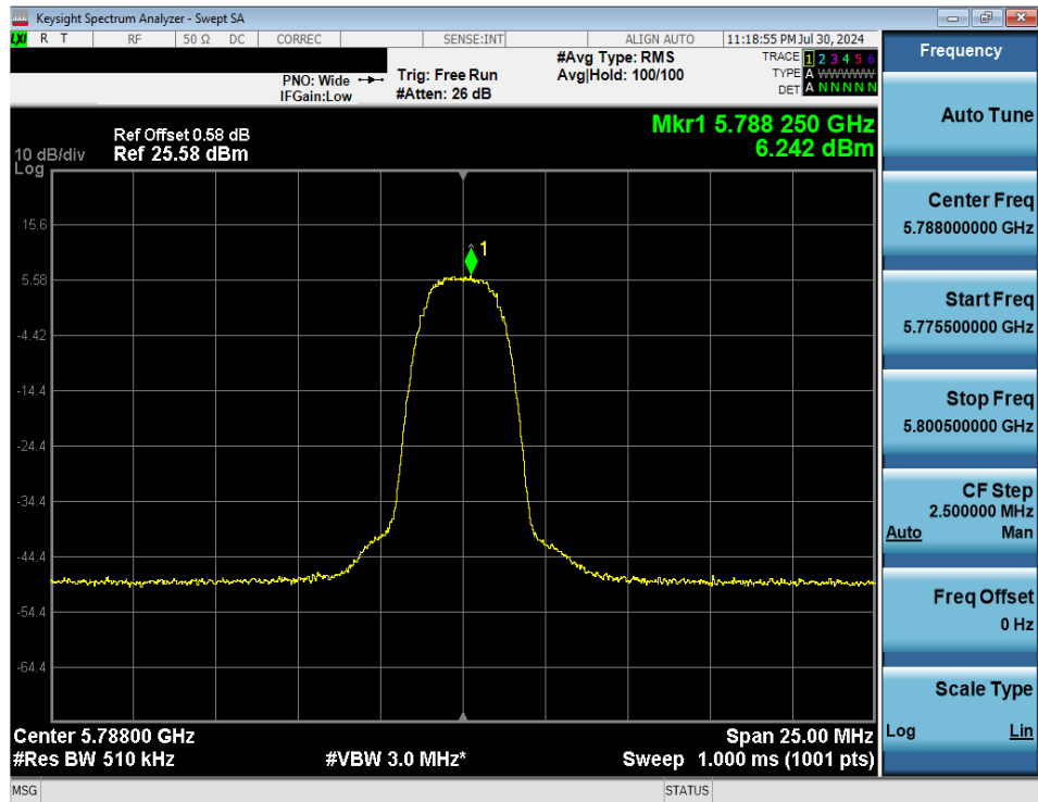
Plot 7-68. PSD (NB UNII HDRp4 – 5788MHz)
