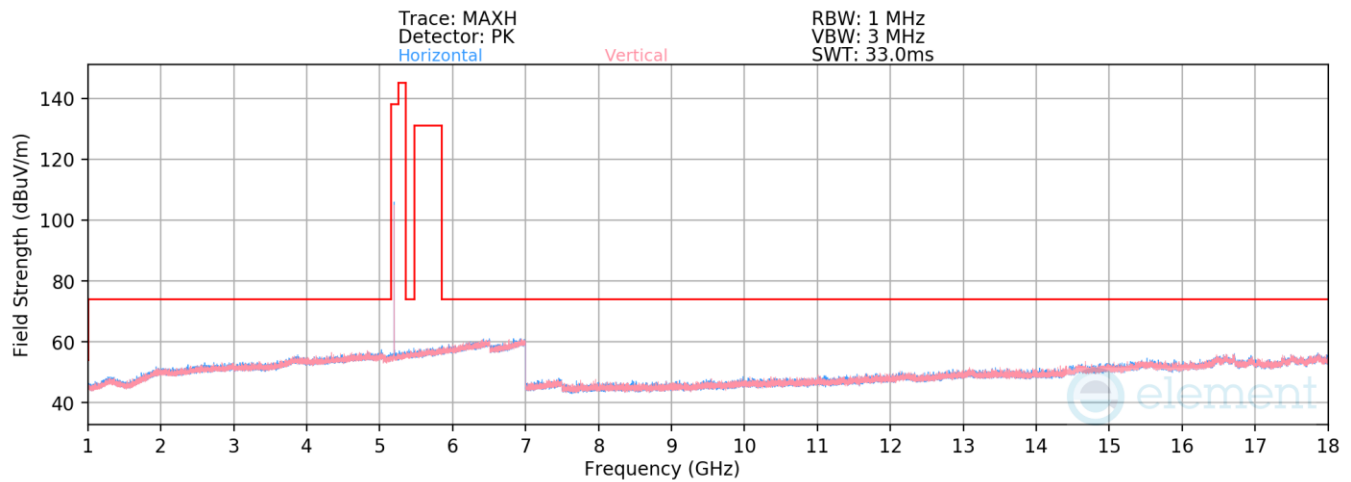
Plot 7-75. Radiated Spurious Emissions 1-18GHz (NB UNII BDR – 5201MHz)
