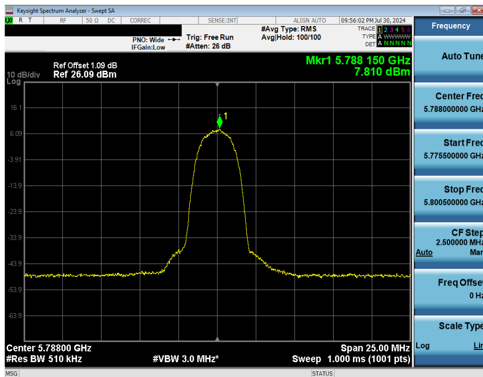
Plot 7-62. PSD (NB UNII HDR4 – 5788MHz)
