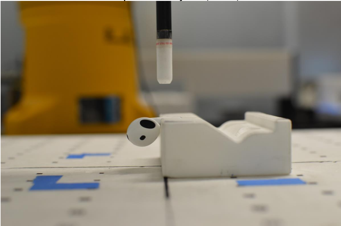
SAR Test Setup Photo 9: Body-Worn, Button, 9.34 mm
