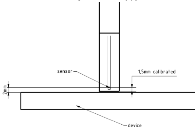
Figure F-2 EUMmWVx Probe
