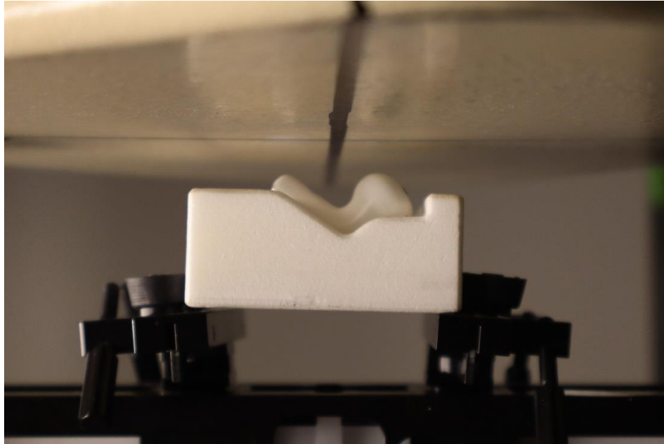
SAR Test Setup Photo 1: Head, Front, 5 mm
