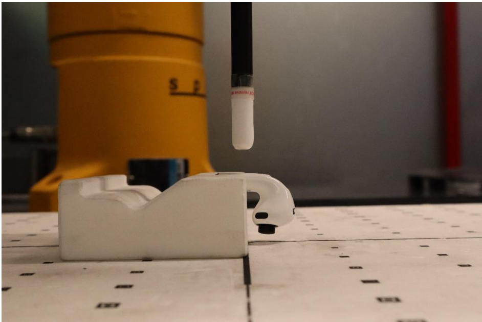
mmWave Test Setup Photo 6: Body-Worn, Back, 9.82 mm
