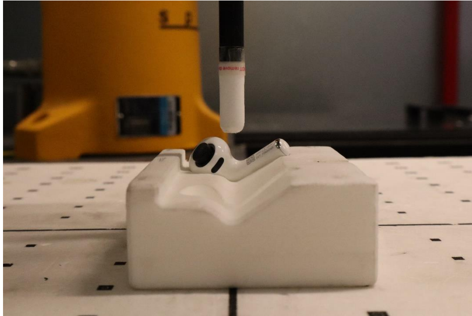
mmWave Test Setup Photo 4: Head, Front, 2 mm
