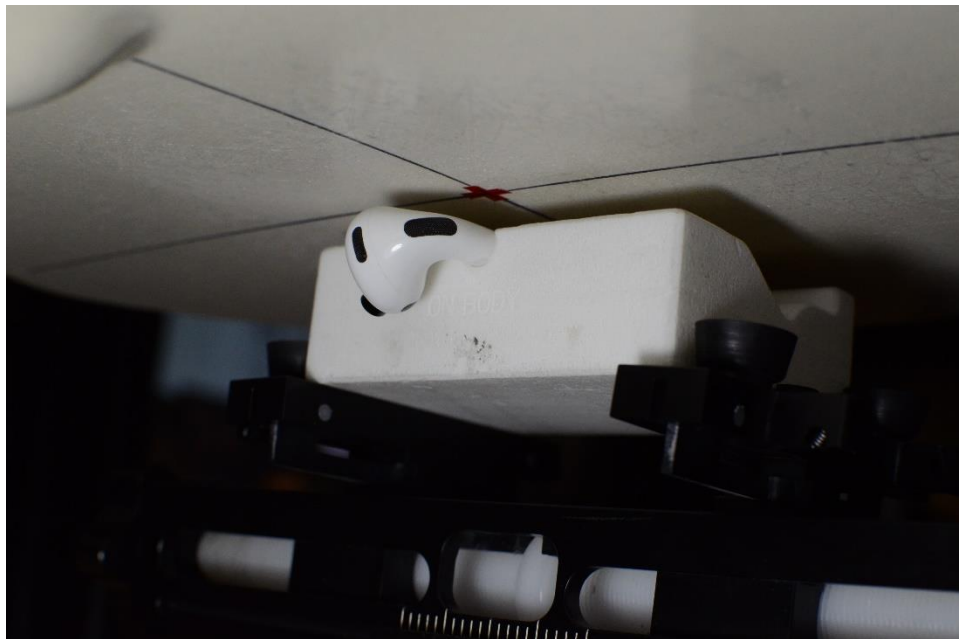
SAR Test Setup Photo 4: Body-Worn, Left, 5 mm
