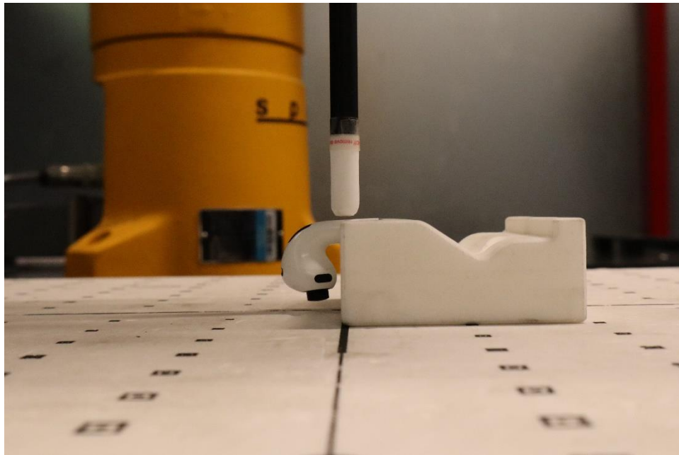
mmWave Test Setup Photo 6: Body-Worn, Back, 2 mm
