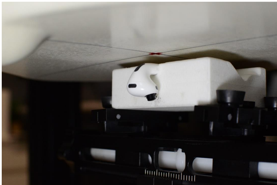
SAR Test Setup Photo 2: Body-Worn, Back Side, 5 mm
