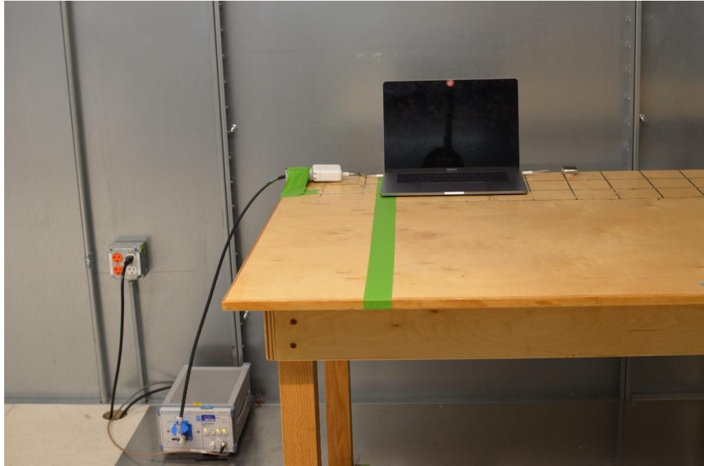
Figure 3: AC Line Conducted Emissions (Front View)
