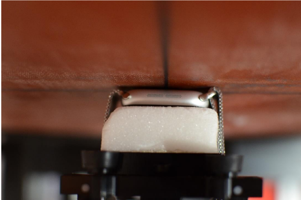
NFC Test Setup Photo 9 – Aluminum with Metal Loop Wristband, Extremity, Back Side at 0 mm
