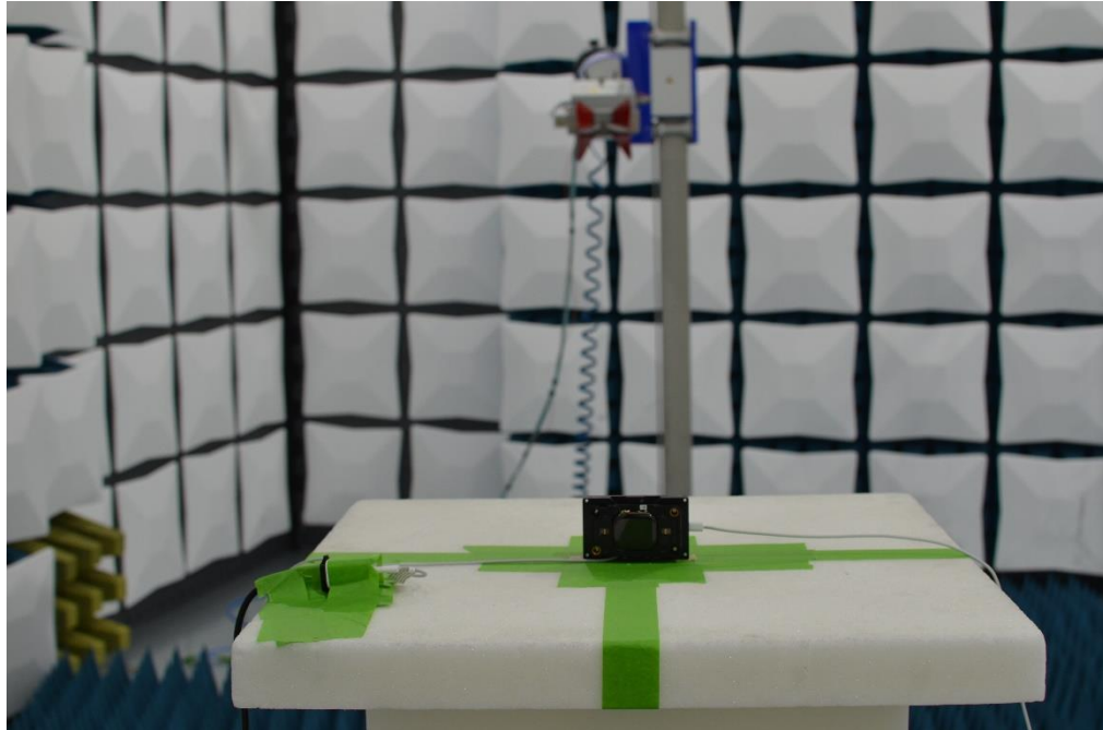
Figure 11: 1-18GHz Test Setup (Rear View)
