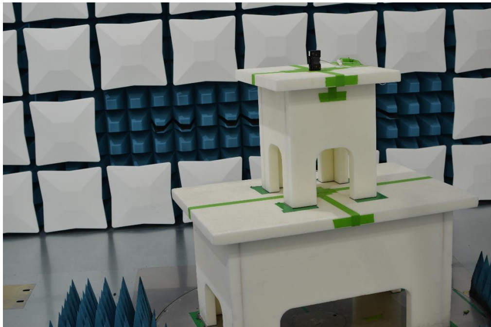
Figure 12: 1-18GHz Test Setup (Front View)
