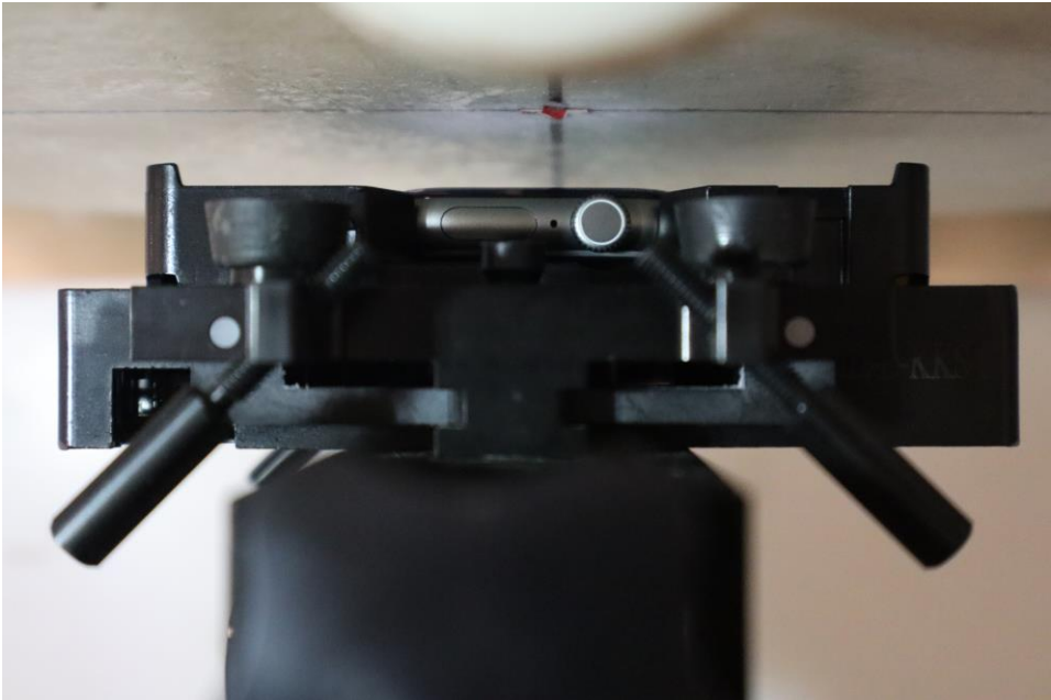
Test Setup Photo 6 – Radiated Test Setup for Head (Front Side) at 10.0 mm
