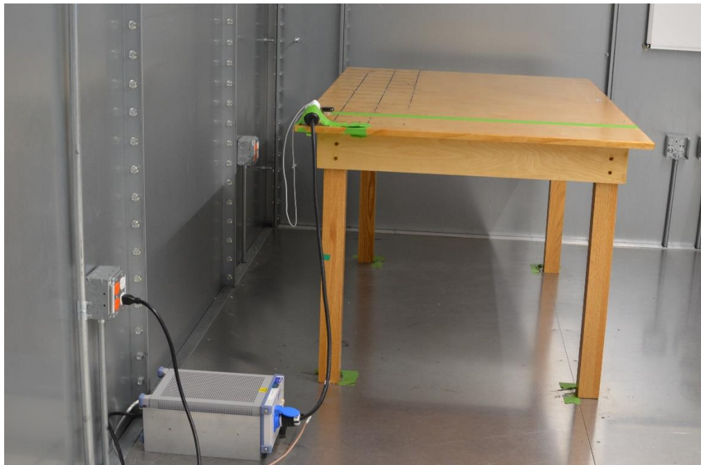
Figure 2: AC Line Conducted Emissions (Side View)
