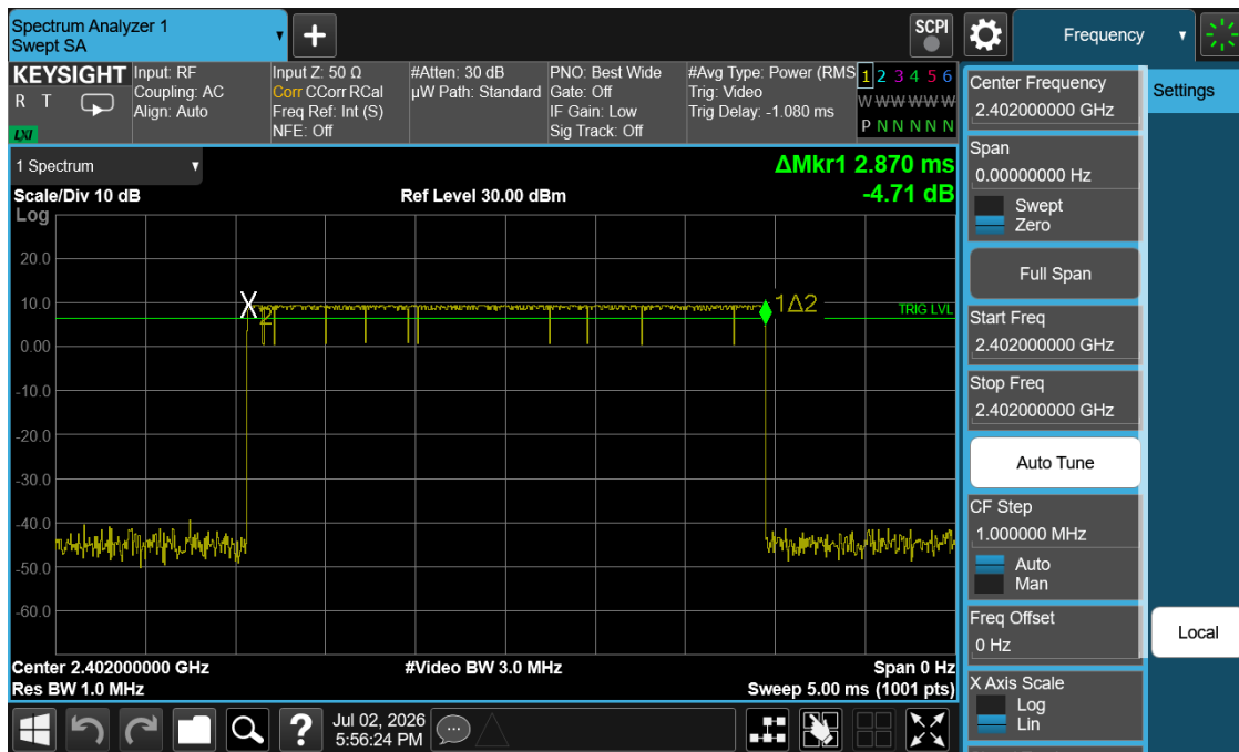
Plot 7-13. Time of Occupancy Plot (Bluetooth, GFSK)
