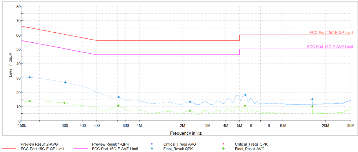
Plot 7-31. AC Line-Conducted Test Plot (L1, GFSK – Ch.78, with AC/DC Adapter)
