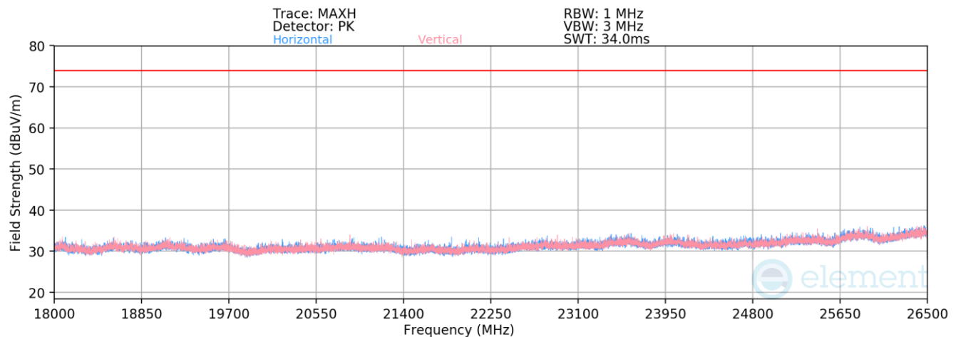
Plot 7-25. Radiated Spurious Emissions above 18GHz (BT GFSK – Ch. 78)
