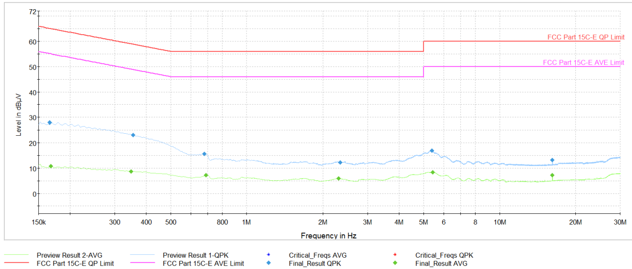
Plot 7-32. AC Line-Conducted Test Plot (N, GFSK – Ch.78, with AC/DC Adapter)
