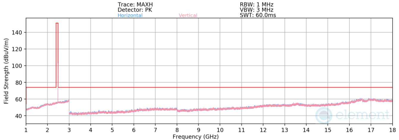
Plot 7-24. Radiated Spurious Emissions above 1GHz (BT GFSK – Ch. 78)
