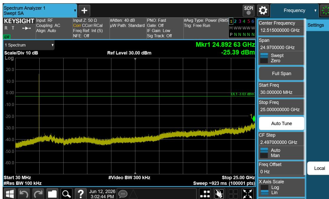
Plot 7-21. Conducted Spurious Plot (Bluetooth, GFSK – Ch. 78)
