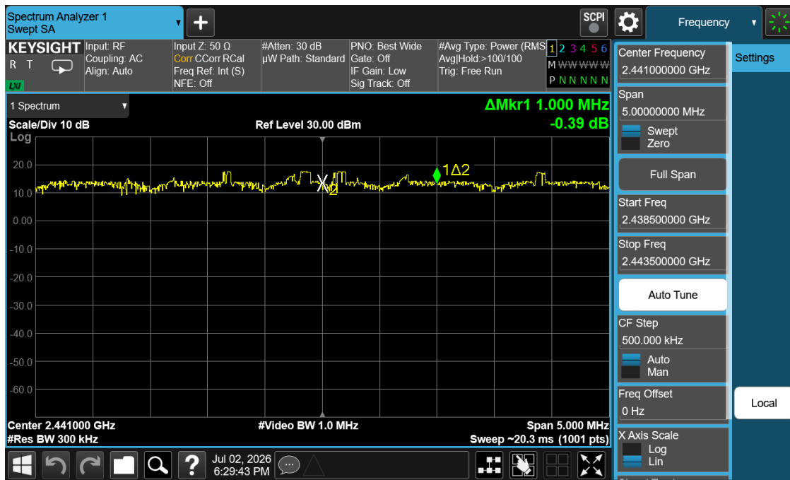
Plot 7-12. Channel Spacing Plot (Bluetooth, 8DPSK)
