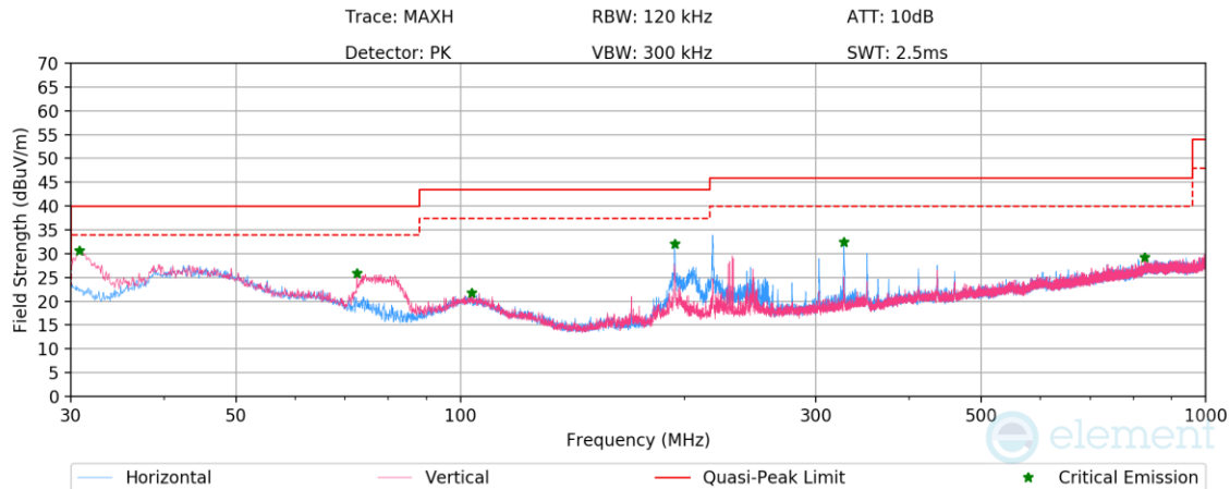
Plot 7-30. Radiated Spurious Emissions Below 1GHz (GFSK – Ch.78, with AC/DC Adapter)
