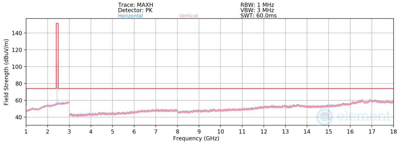
Plot 7-23. Radiated Spurious Emissions above 1GHz (BT GFSK – Ch. 39)
