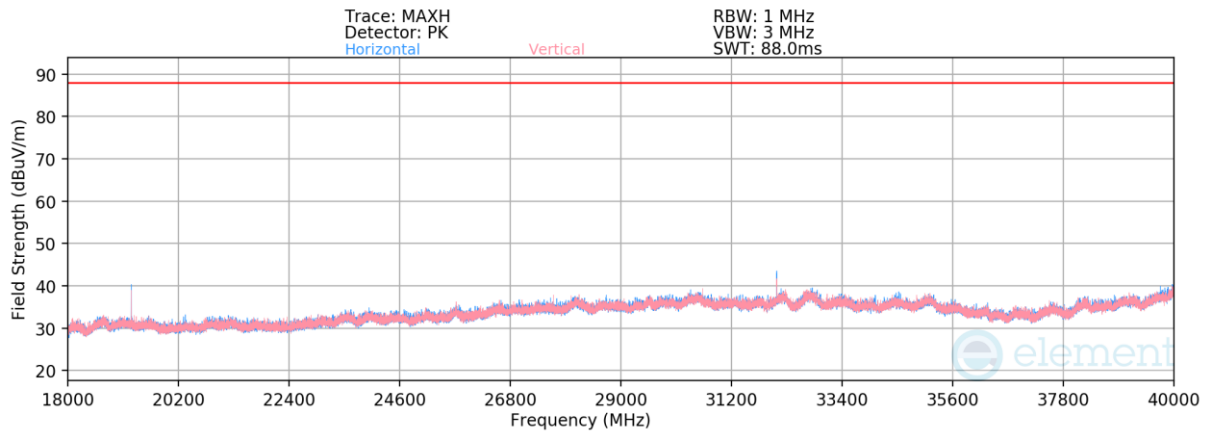
Plot 7-37. Radiated Spurious Emissions Above 18GHz (LE1M – 6420MHz)
