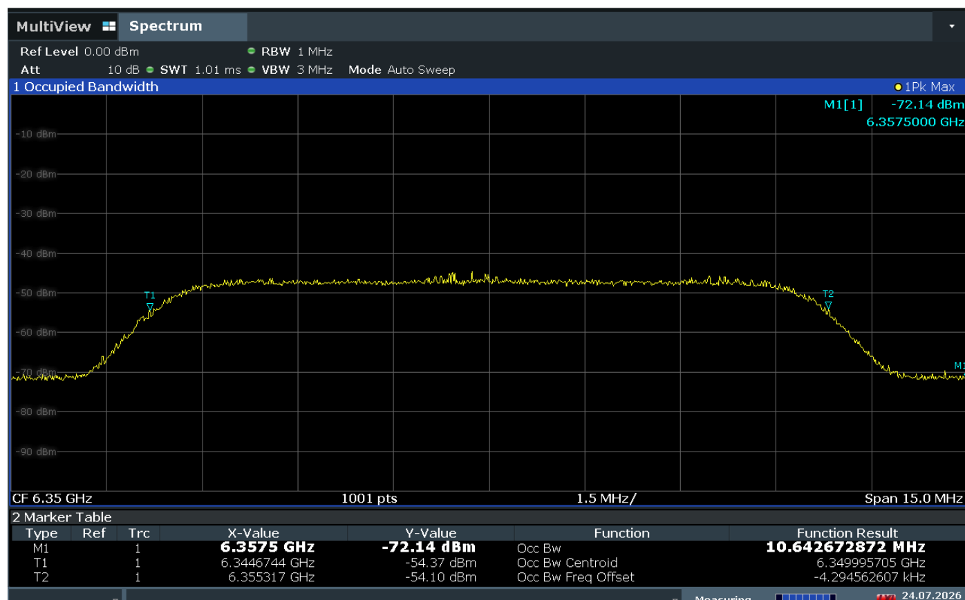
Plot 7-22. AWGN Signal
