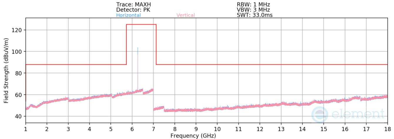
Plot 7-35. Radiated Spurious Emissions 1-18GHz (LE1M – 6264MHz)
