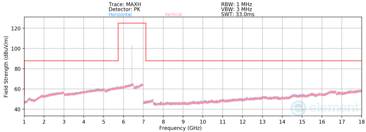
Plot 7-36. Radiated Spurious Emissions 1-18GHz (LE1M – 6420MHz)
