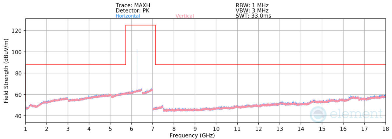
Plot 7-31. Radiated Spurious Emissions 1-18GHz (BDR GFSK – 6264MHz)
