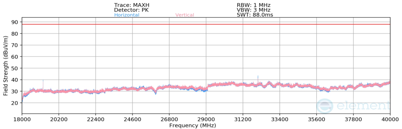
Plot 7-33. Radiated Spurious Emissions Above 18GHz (BDR GFSK – 6420MHz)
