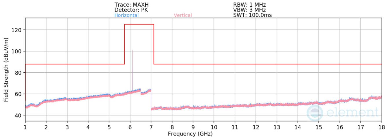
Plot 7-34. Radiated Spurious Emissions 1-18GHz (LE1M – 6108MHz)
