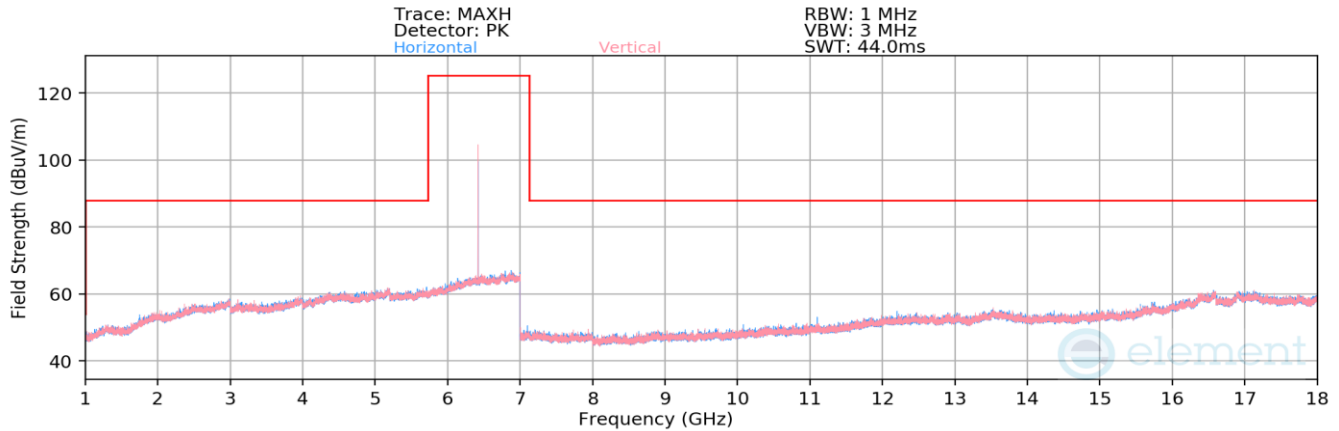
Plot 7-32. Radiated Spurious Emissions 1-18GHz (BDR GFSK – 6420MHz)
