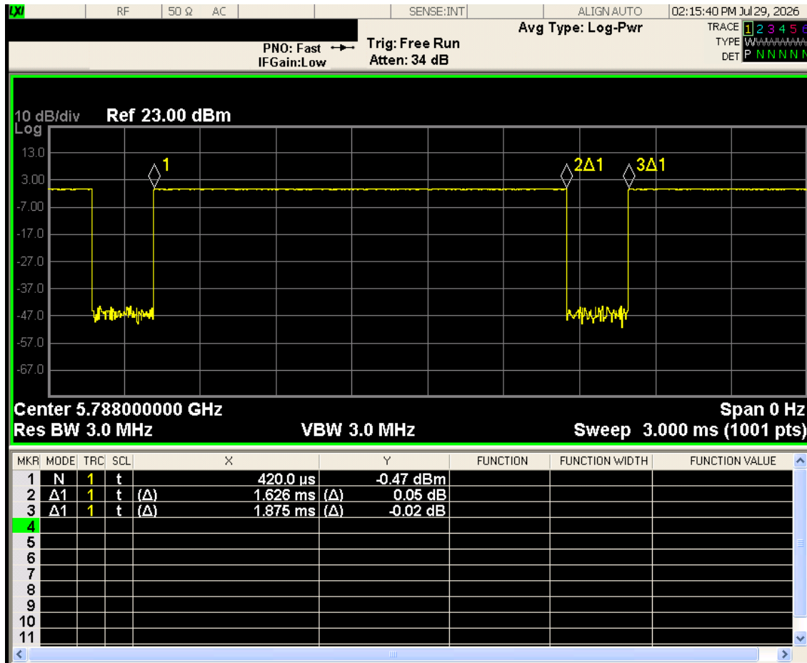
Figure 7-3 NB UNII-3 Transmission Plot
