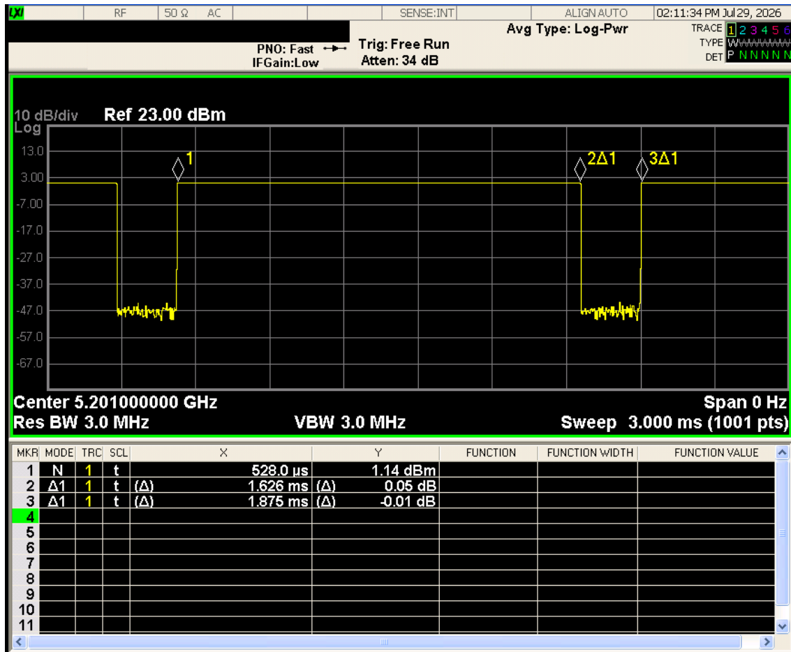
Figure 7-2 NB UNII-1 Transmission Plot
