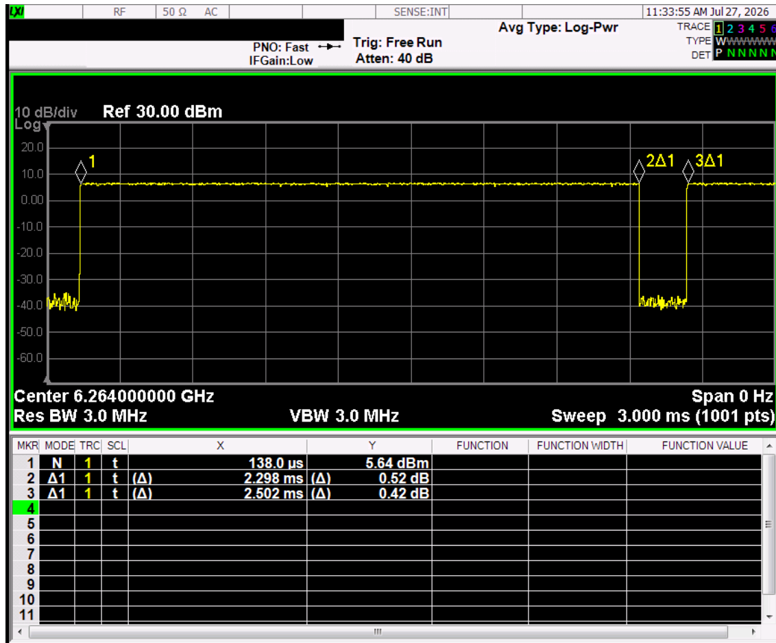
Figure 7-4 NB UNII-5 Transmission Plot
