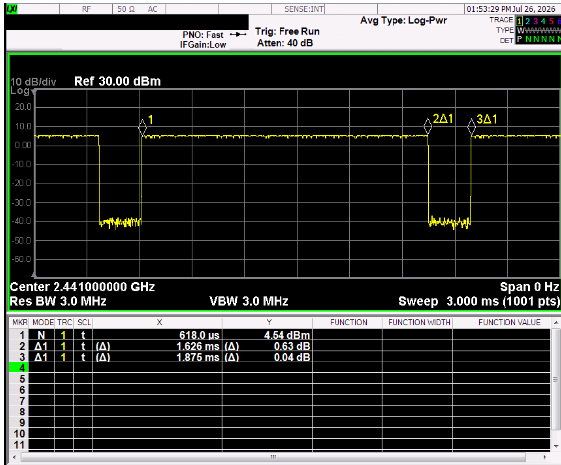
Figure 7-1 2.4 GHz Bluetooth Transmission Plot
