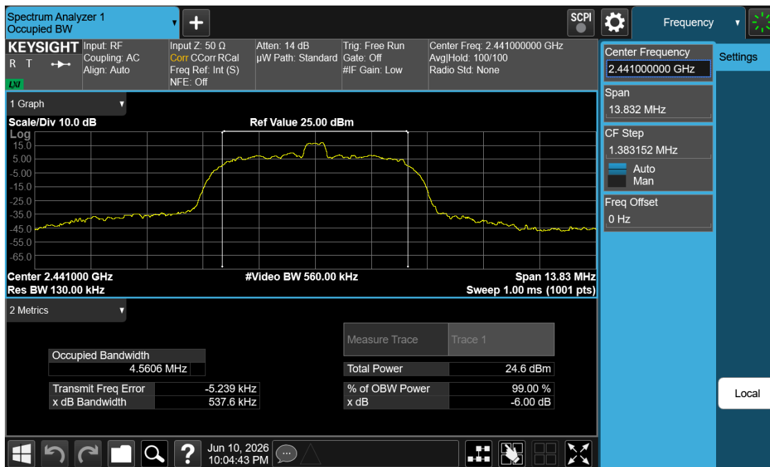
Plot 7-5. 99% OBW Plot (Bluetooth (HDR8), 8Mbps – Ch. 38)
