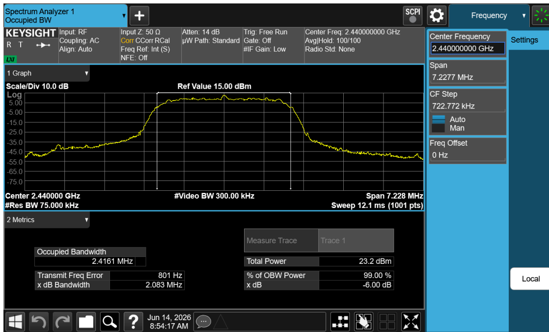
Plot 7-8. 99% OBW Plot (Bluetooth (HDRp4), 4Mbps – Ch. 38)
