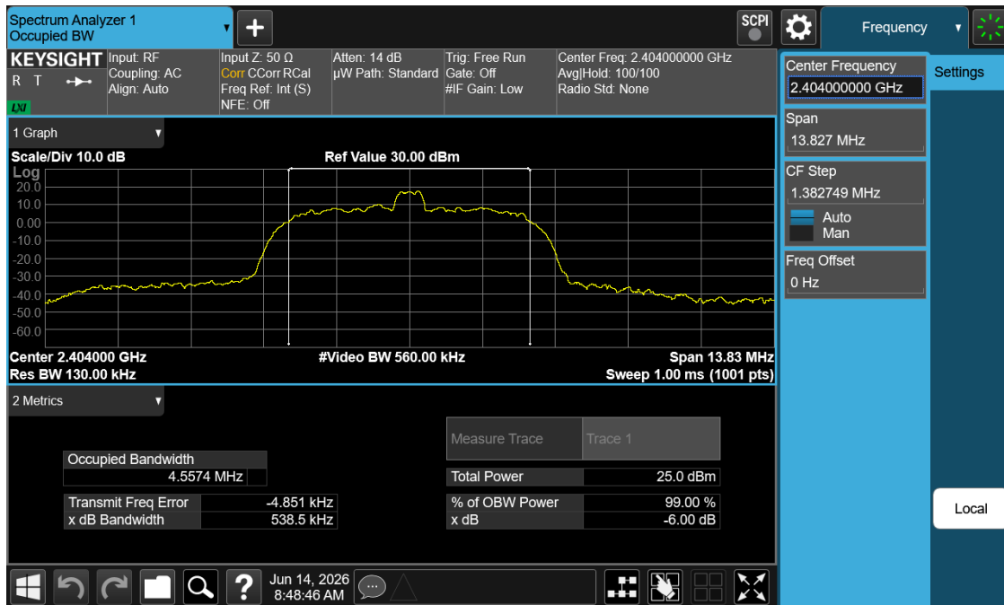
Plot 7-4. 99% OBW Plot (Bluetooth (HDR8), 8Mbps – Ch. 1)
