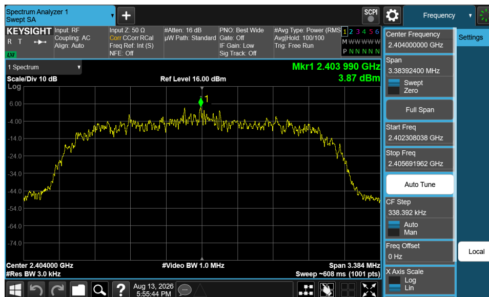
Plot 7-25. Power Spectral Density Plot (Bluetooth (HDR4), 4Mbps, – Ch. 1)
