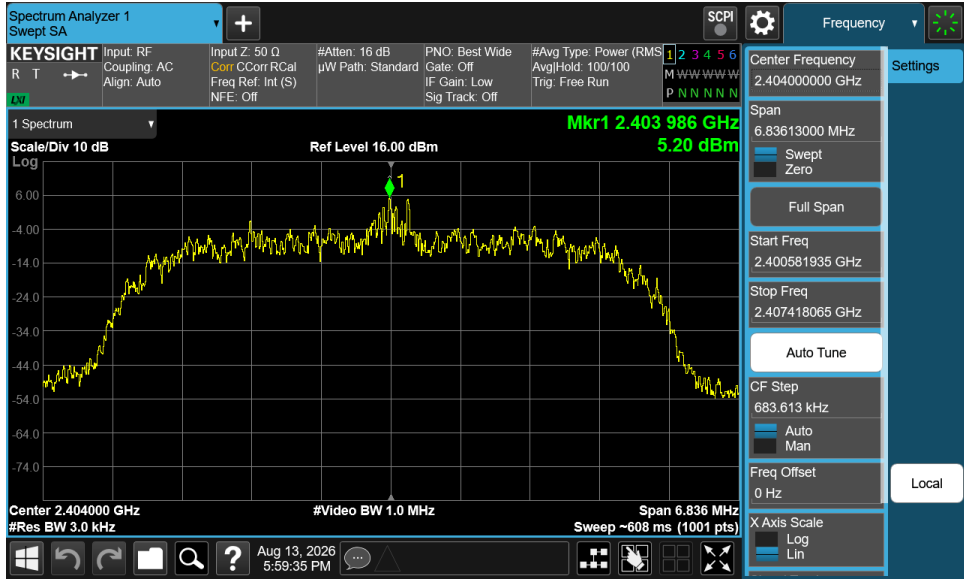
Plot 7-28. Power Spectral Density Plot (Bluetooth (HDR8), 8Mbps, – Ch. 1)
