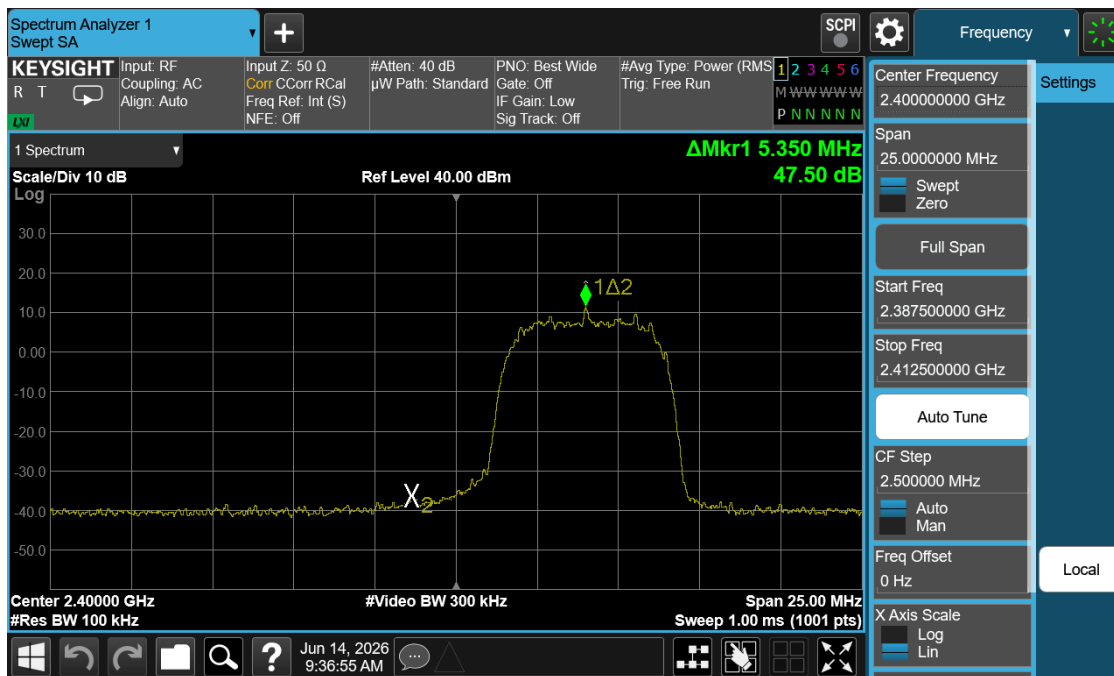
Plot 7-43. Band Edge Plot (Bluetooth (HDRp8) – Ch. 1)
