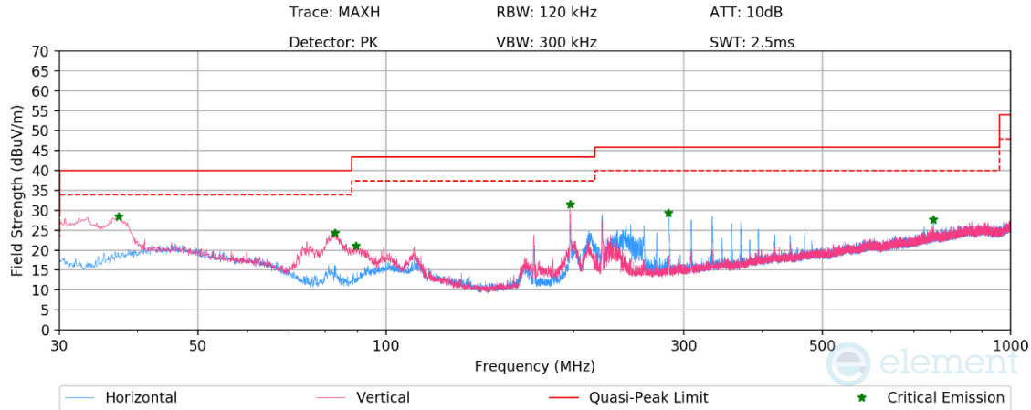
Plot 7-67. Radiated Spurious Emissions Below 1GHz (HDR4 – Ch.73 with AC/DC Adapter)
