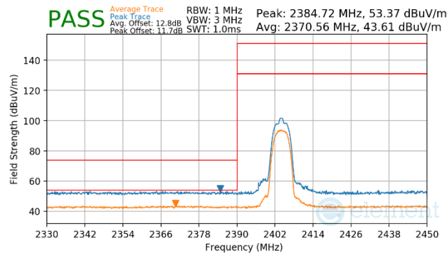
Plot 7-60. Radiated Restricted Lower Band Edge Measurement
