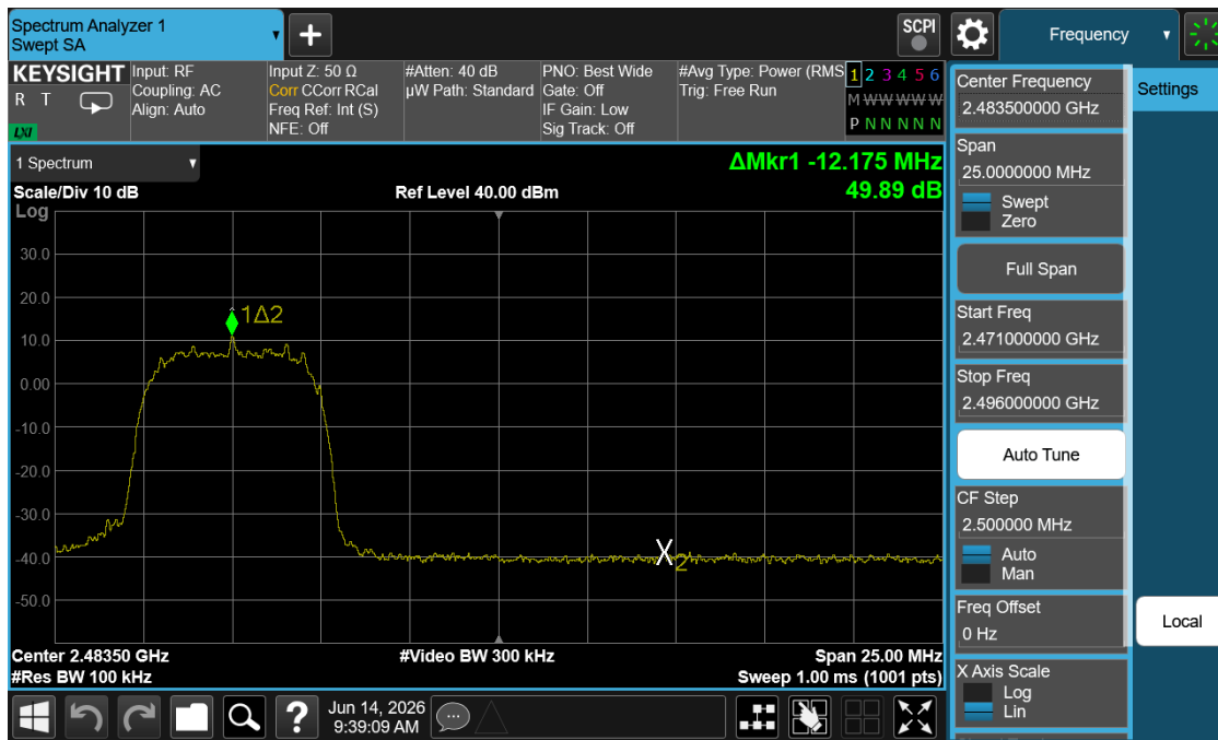
Plot 7-44. Band Edge Plot (Bluetooth (HDRp8) – Ch. 73)
