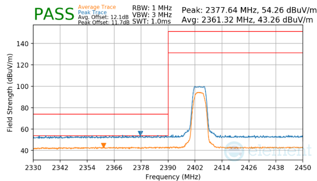
Plot 7-62. Radiated Restricted Lower Band Edge Measurement
