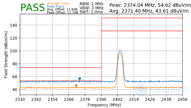
Plot 7-59. Radiated Restricted Lower Band Edge Measurement
