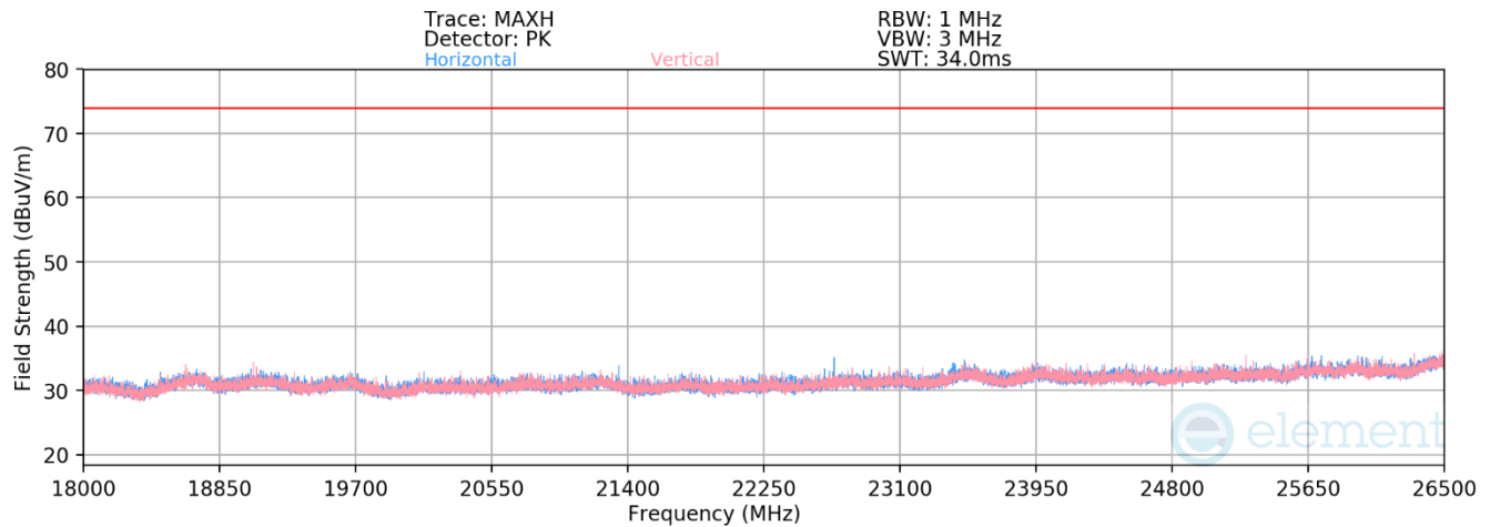
Plot 7-58. Radiated Spurious Emissions above 18GHz (4Mbps, HDRp4 – Ch. 1)
