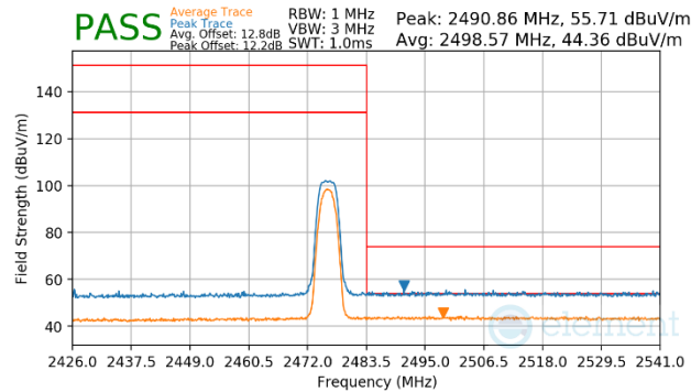
Plot 7-65. Radiated Restricted Upper Band Edge Measurement
