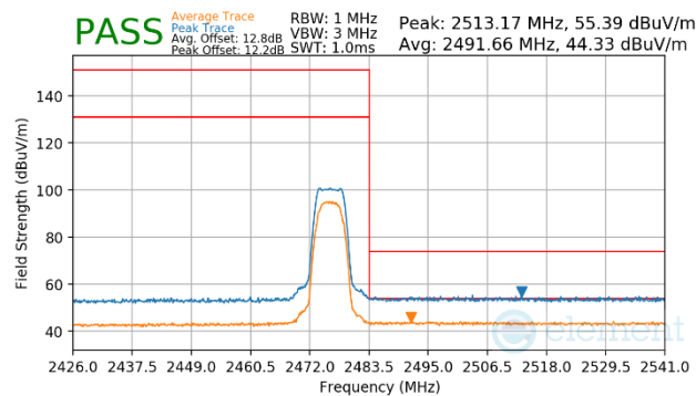
Plot 7-66. Radiated Restricted Upper Band Edge Measurement
