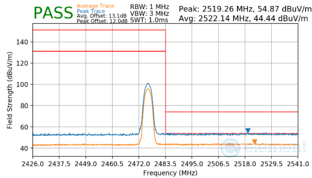
Plot 7-63. Radiated Restricted Upper Band Edge Measurement
