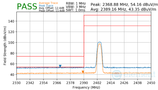
Plot 7-61. Radiated Restricted Lower Band Edge Measurement
