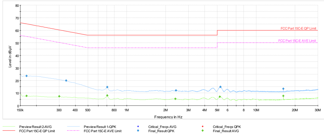
Plot 7-69. AC Line Conducted Plot with Bluetooth HDR (N, HDR4 - Ch.73 with AC/DC Adapter)
