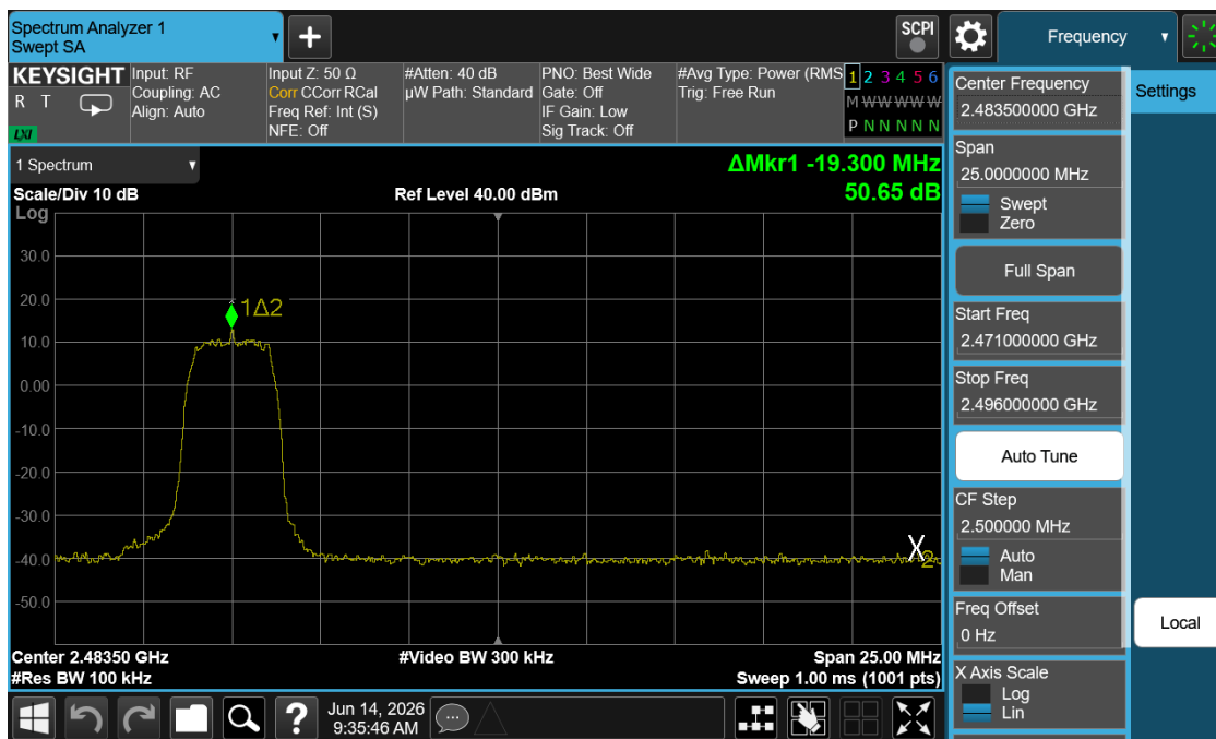
Plot 7-42. Band Edge Plot (Bluetooth (HDRp4) – Ch. 73)
