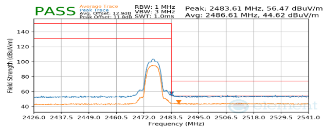
Plot 7-64. Radiated Restricted Upper Band Edge Measurement
