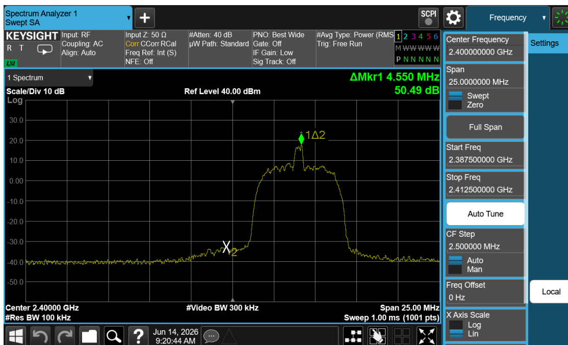
Plot 7-39. Band Edge Plot (Bluetooth (HDR8) – Ch. 1)
