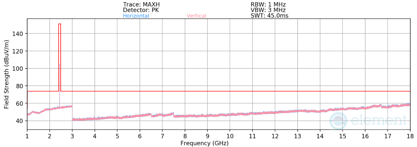
Plot 7-52. Radiated Spurious Emissions 1-18GHz (4Mbps, HDR4 – Ch. 38)
