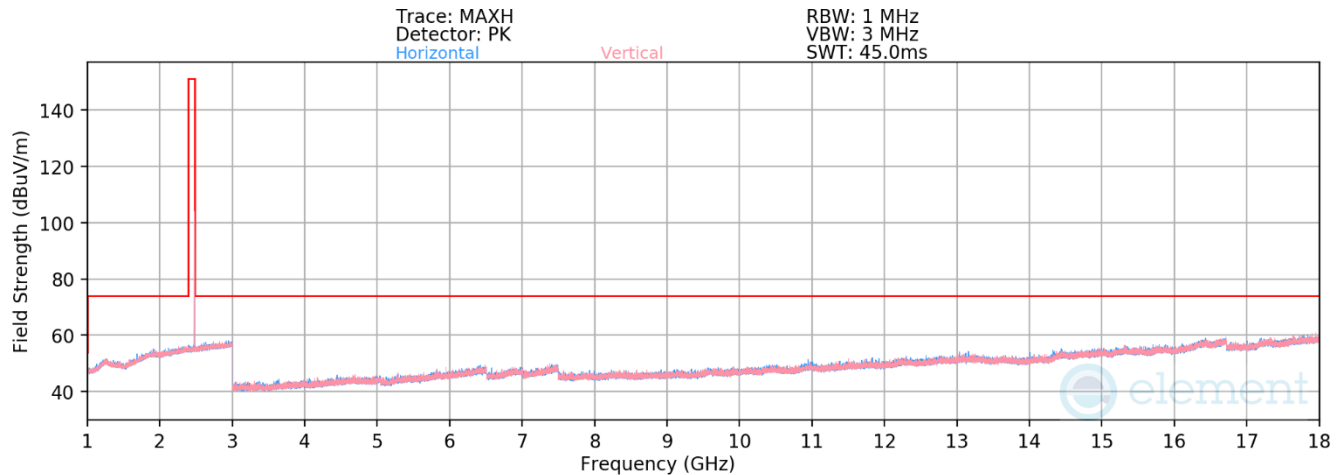
Plot 7-53. Radiated Spurious Emissions 1-18GHz (4Mbps, HDR4 – Ch. 73)
