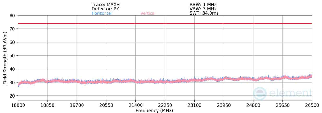
Plot 7-54. Radiated Spurious Emissions above 18GHz (4Mbps, HDR4 – Ch. 73)
