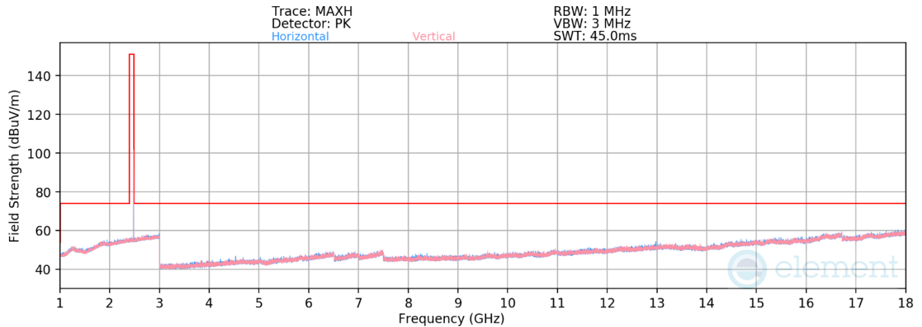
Plot 7-57. Radiated Spurious Emissions 1-18GHz (4Mbps, HDRp4 – Ch. 73)
