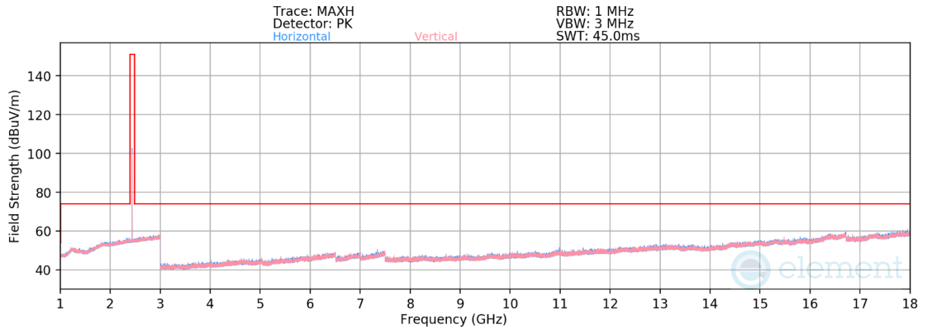
Plot 7-56. Radiated Spurious Emissions 1-18GHz (4Mbps, HDRp4 – Ch. 38)
