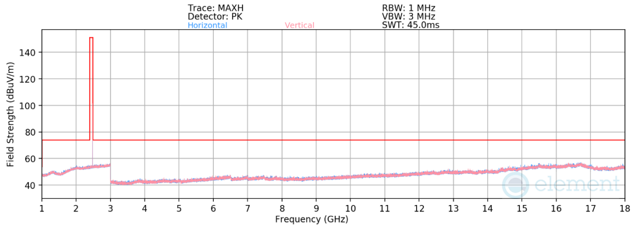
Plot 7-29. Radiated Spurious Emissions 1-18GHz (1 Mbps – Ch. 39)
