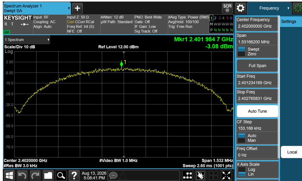
Plot 7-13. Power Spectral Density Plot (Bluetooth (LE), 1 Mbps – Ch. 37)
