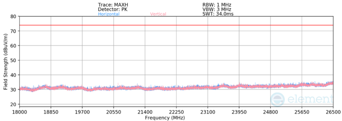
Plot 7-28. Radiated Spurious Emissions Above 18GHz (1 Mbps – Ch. 17)
