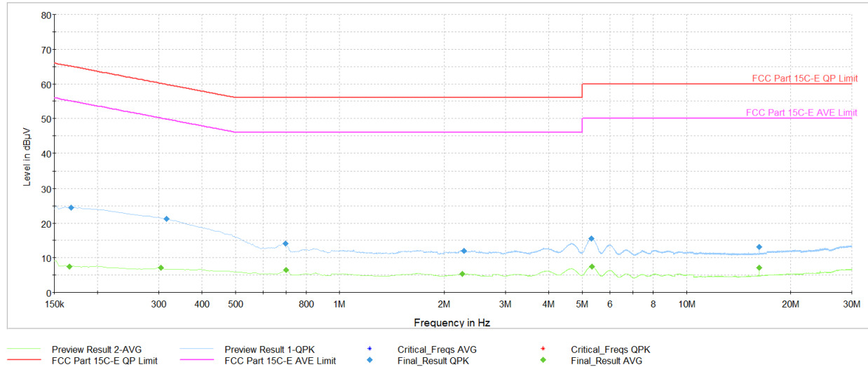
Plot 7-36. AC Line Conducted Plot with Bluetooth LE (N, 1 Mbps – Ch.17, with AC/DC Adapter)
