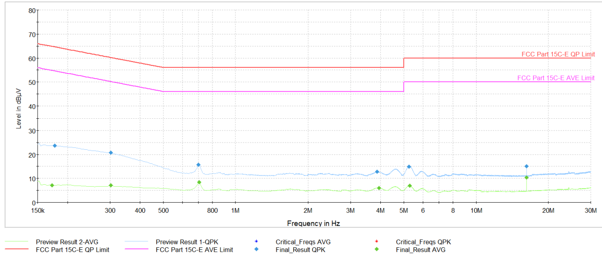
Plot 7-35. AC Line Conducted Plot with Bluetooth LE (L1, 1 Mbps – Ch.17 with AC/DC Adapter)
