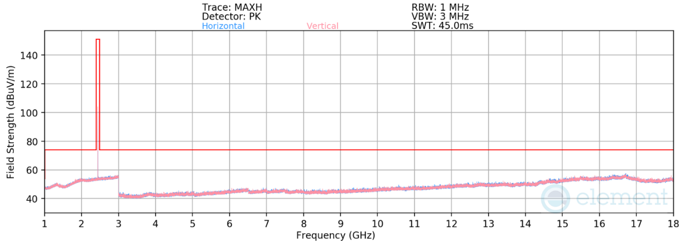
Plot 7-27. Radiated Spurious Emissions 1-18GHz (1 Mbps – Ch. 17)
