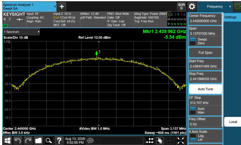
Plot 7-17. Power Spectral Density Plot (Bluetooth (LE), 2 Mbps– Ch. 17)
