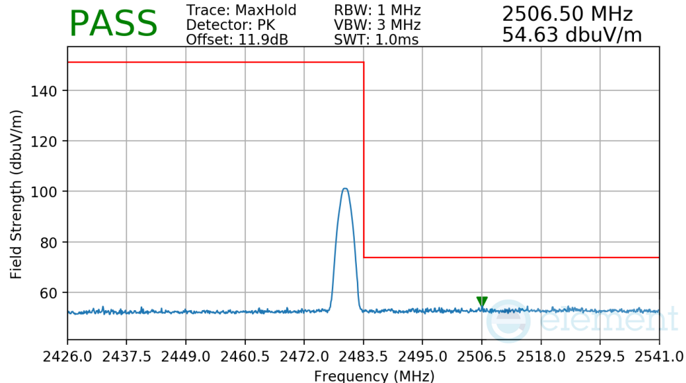
Plot 7-29. Radiated Restricted Upper Band Edge Measurement
