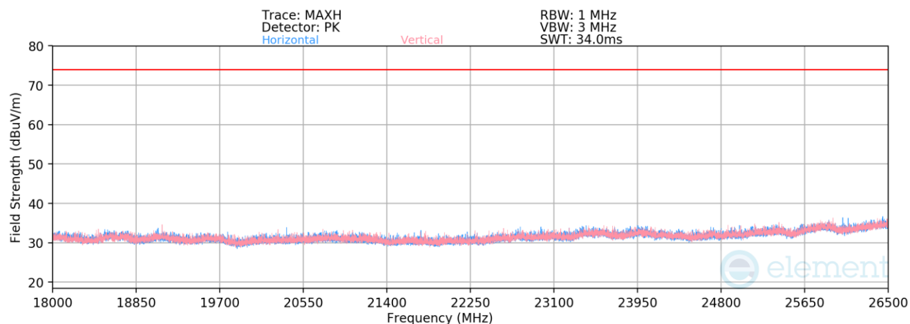
Plot 7-24. Radiated Spurious Emissions above 18GHz (BT GFSK – Ch. 39)
