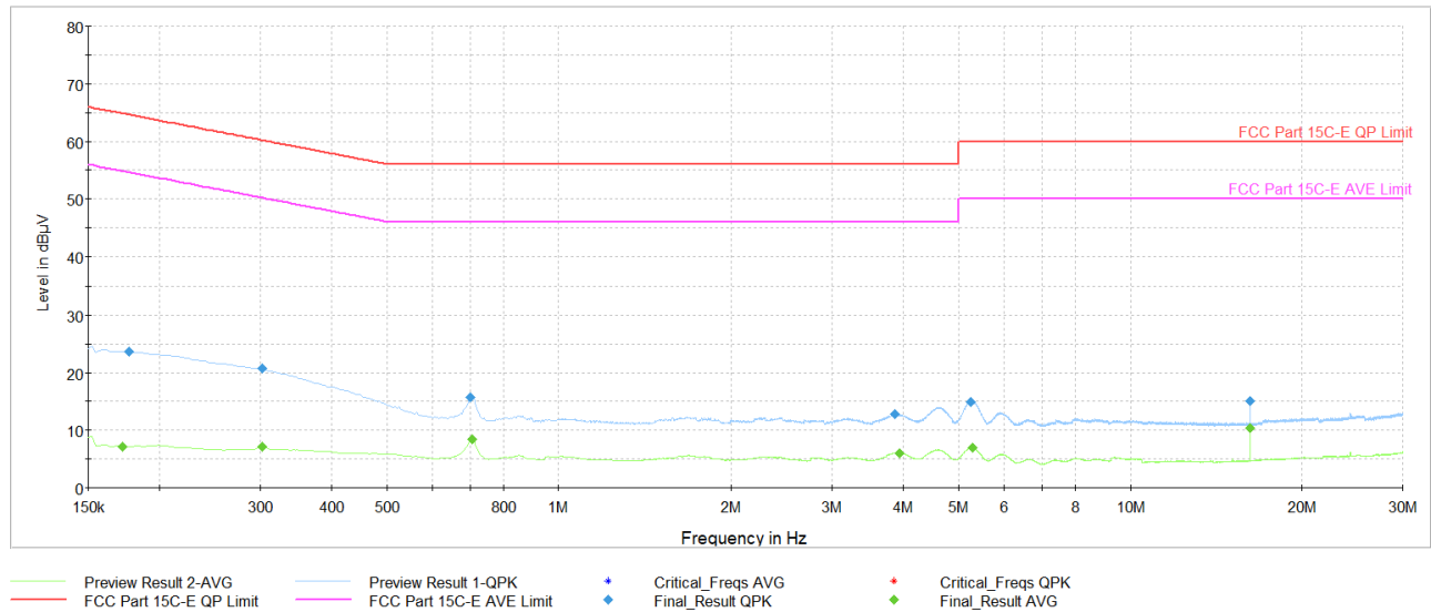
Plot 7-31. AC Line-Conducted Test Plot (L1, GFSK – Ch.39, with AC/DC Adapter)
