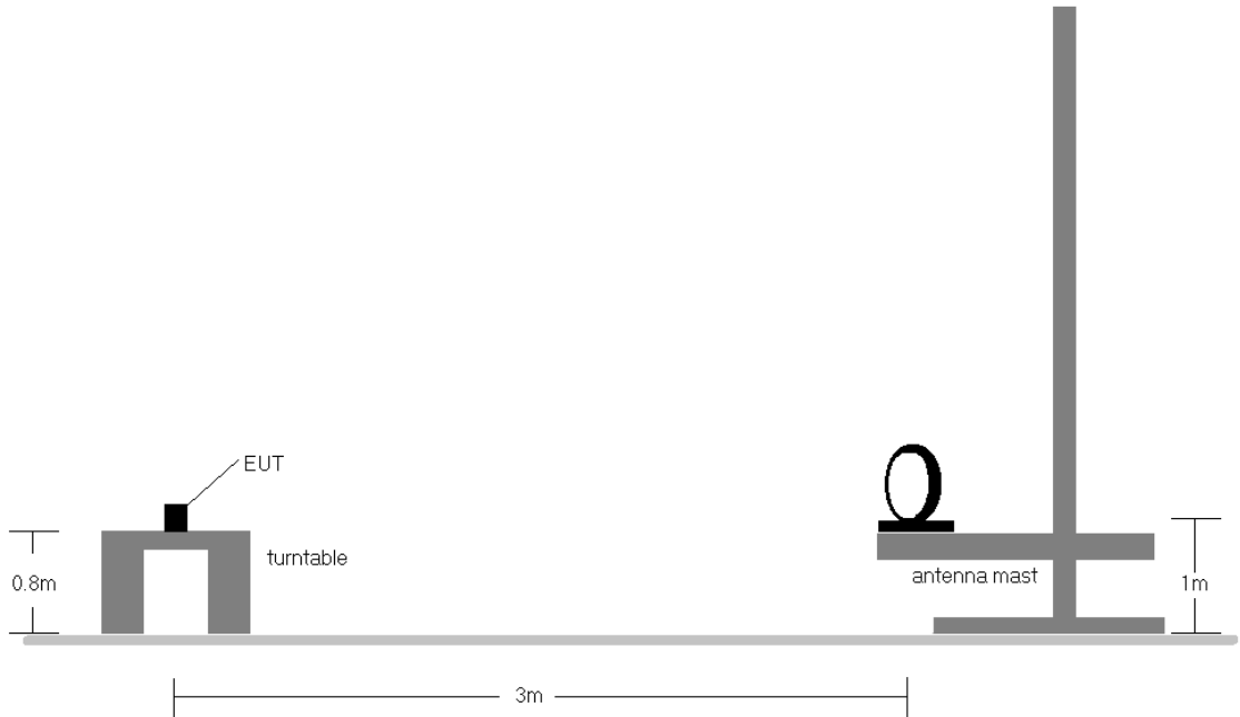
Figure 7-9. Radiated Test Setup < 30MHz
