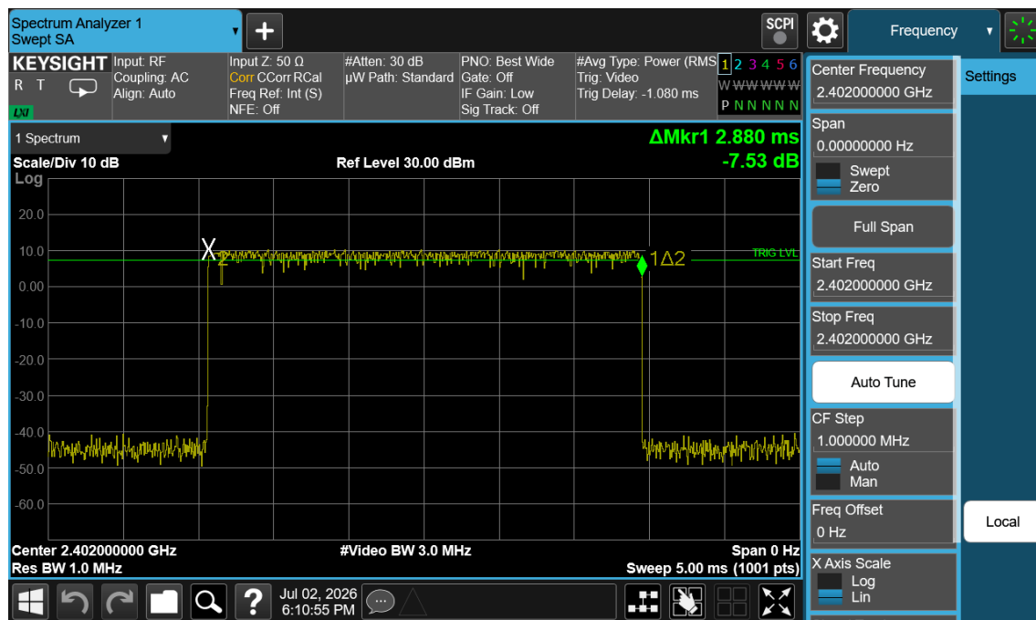
Plot 7-14. Time of Occupancy Plot (Bluetooth, 8DPSK)
