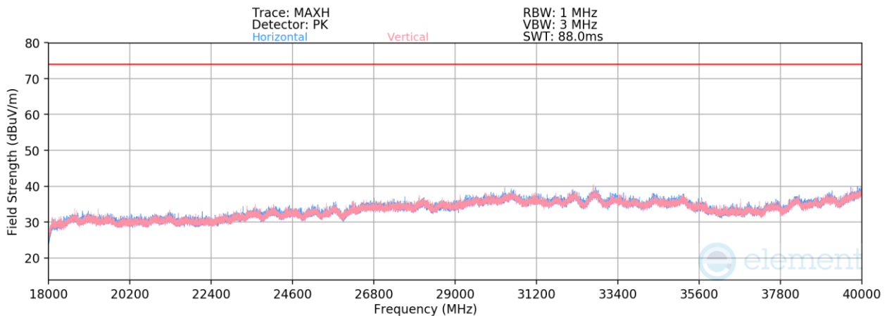
Plot 7-45. Radiated Spurious Emissions Above 18GHz (NB UNII HDR4 – 5157MHz)
