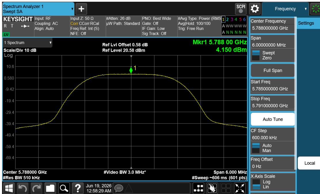
Plot 7-34. PSD (NB UNII HDRp4 – 5788MHz)
