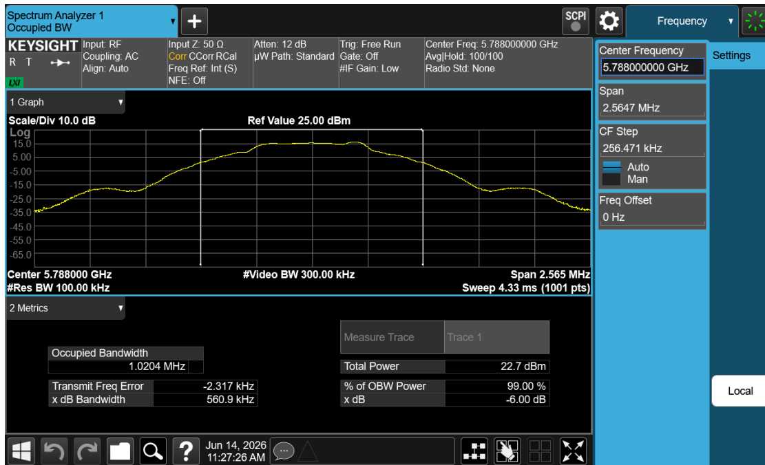
Plot 7-15. 6dB BW (NB UNII BDR – 5788MHz)
