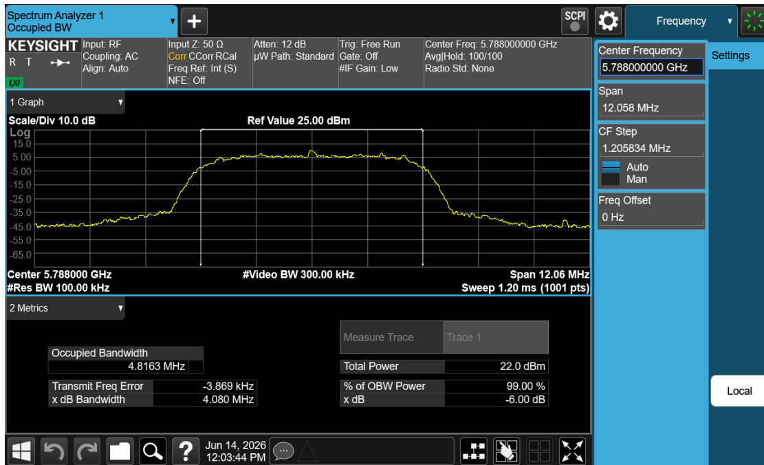
Plot 7-21. 6dB BW (NB UNII HDRp8 – 5788MHz)
