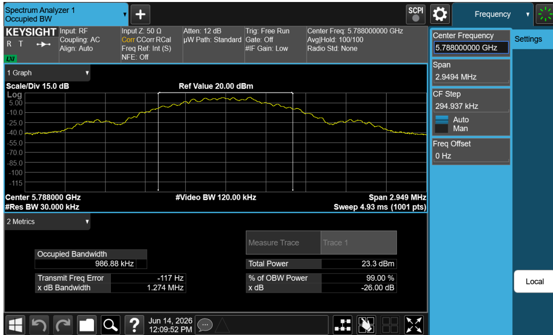
Plot 7-8. 99% OBW (NB UNII BDR – 5788MHz)
