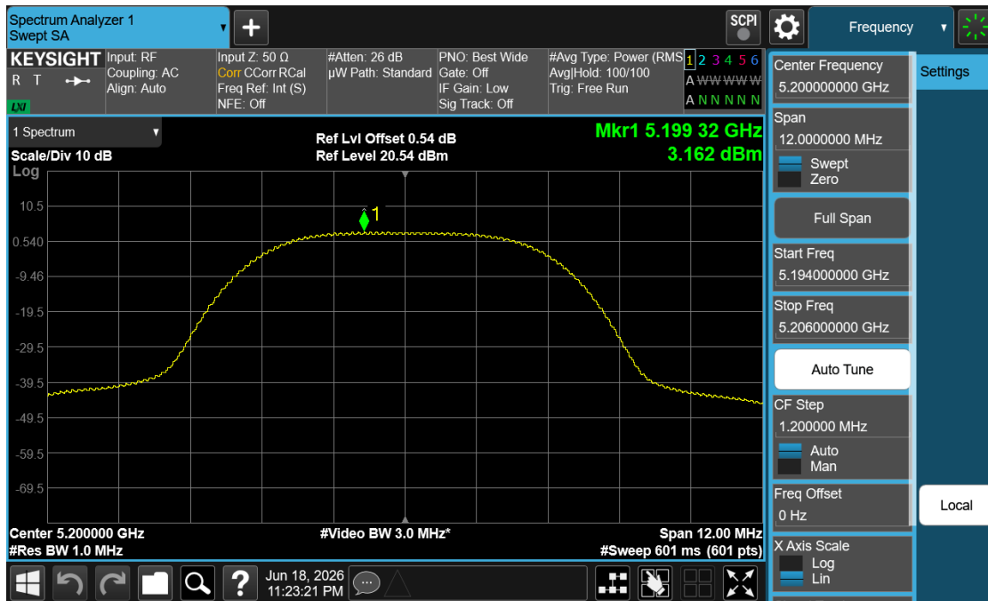
Plot 7-28. PSD (NB UNII HDRp8 – 5200MHz)
