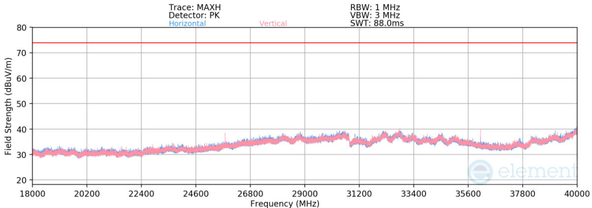
Plot 7-37. Radiated Spurious Emissions Above 18GHz (NB UNII BDR – 5157MHz)
