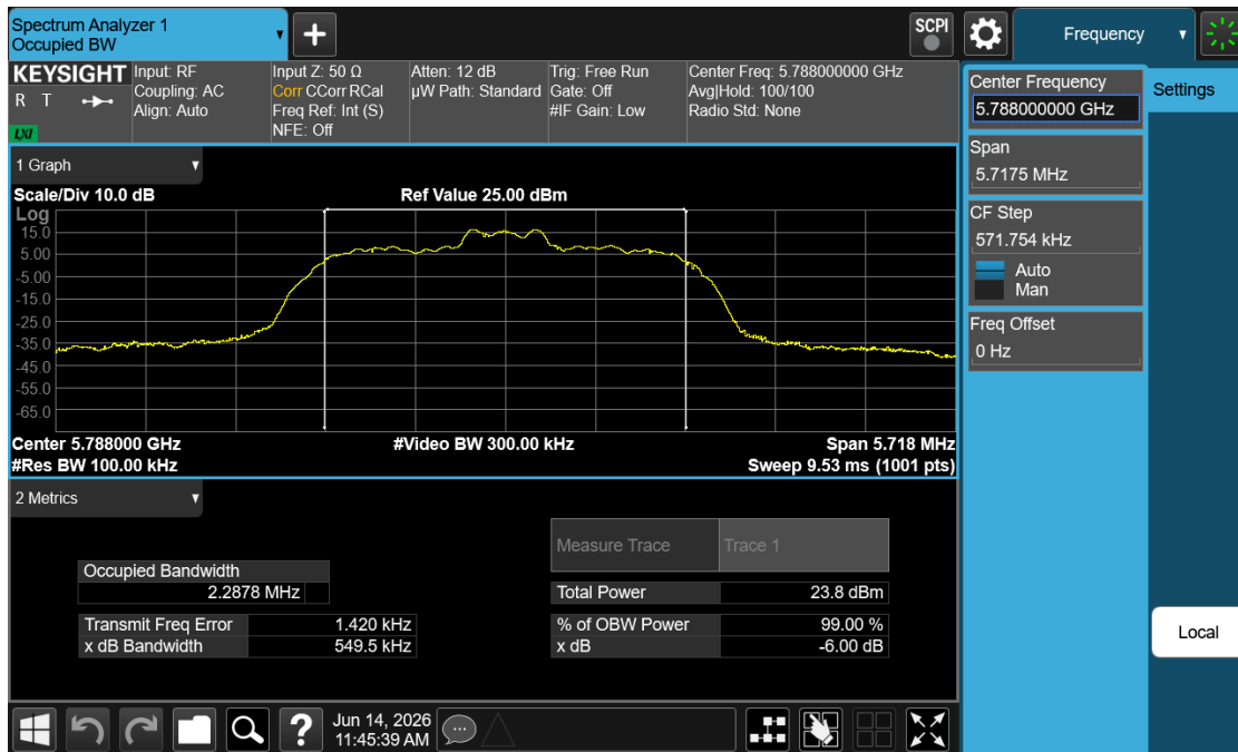
Plot 7-18. 6dB BW (NB UNII HDR4 – 5788MHz)
