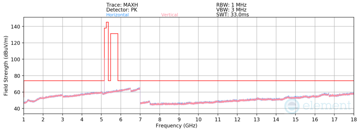
Plot 7-44. Radiated Spurious Emissions 1-18GHz (NB UNII HDR4 – 5157MHz)
