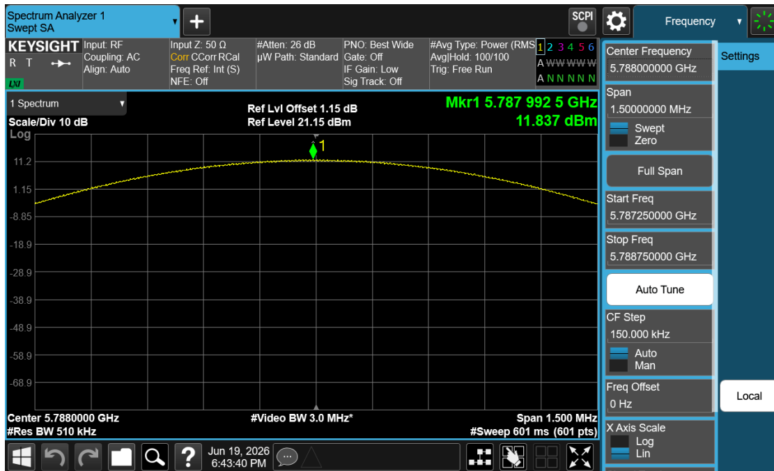
Plot 7-29. PSD (NB UNII BDR – 5788MHz)
