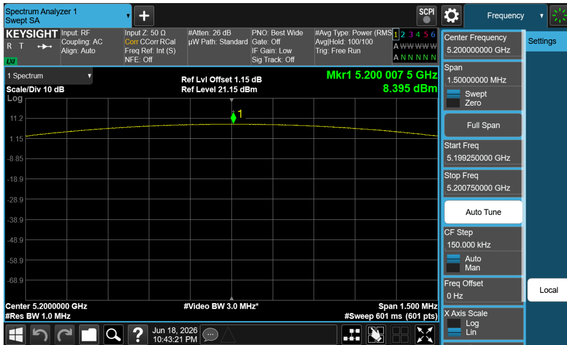
Plot 7-22. PSD (NB UNII BDR – 5200MHz)
