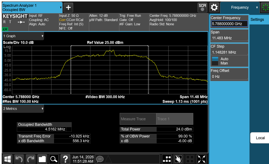
Plot 7-19. 6dB BW (NB UNII HDR8 – 5788MHz)
