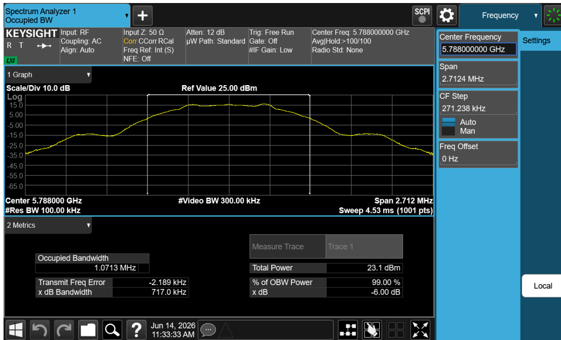
Plot 7-16. 6dB BW (NB UNII LE1M – 5788MHz)
