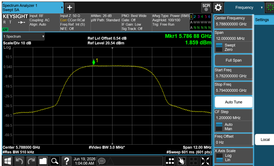
Plot 7-35. PSD (NB UNII HDRp8 – 5788MHz)
