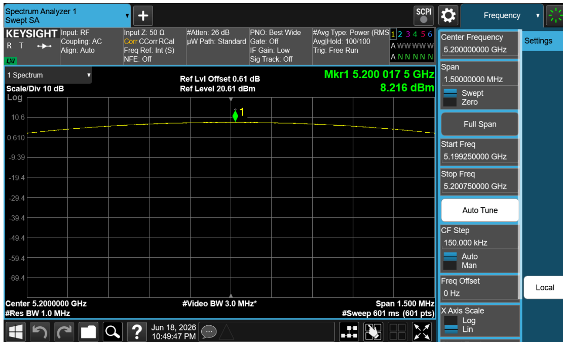
Plot 7-23. PSD (NB UNII LE1M – 5200MHz)
