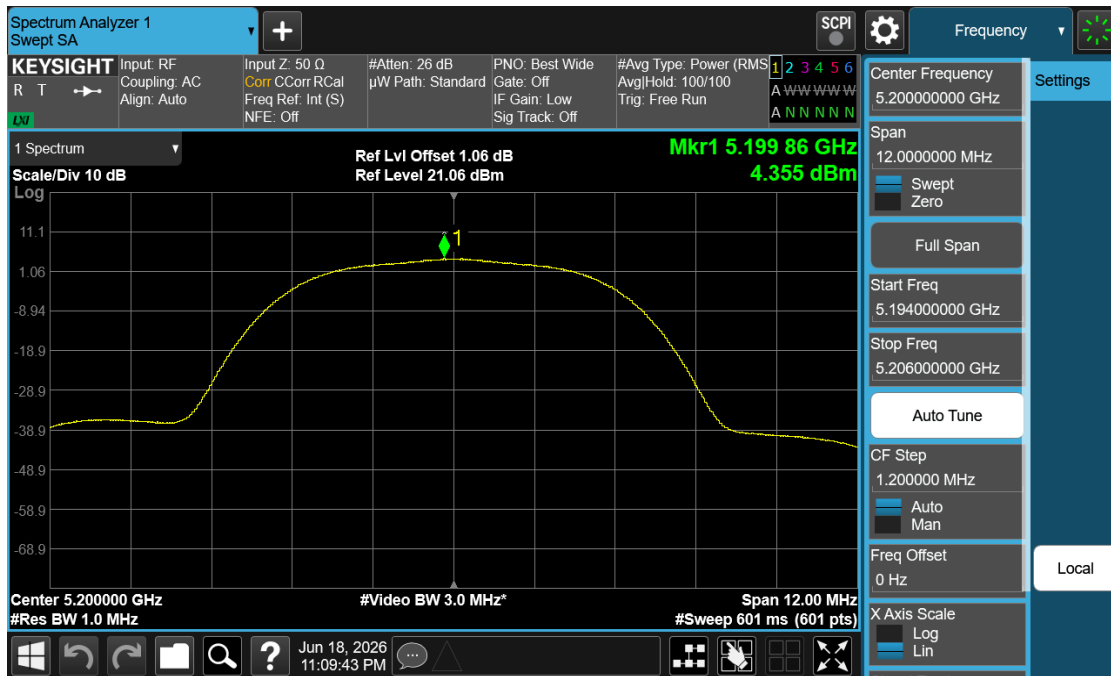
Plot 7-26. PSD (NB UNII HDR8 – 5200MHz)
