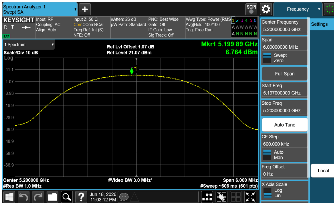
Plot 7-25. PSD (NB UNII HDR4 – 5200MHz)
