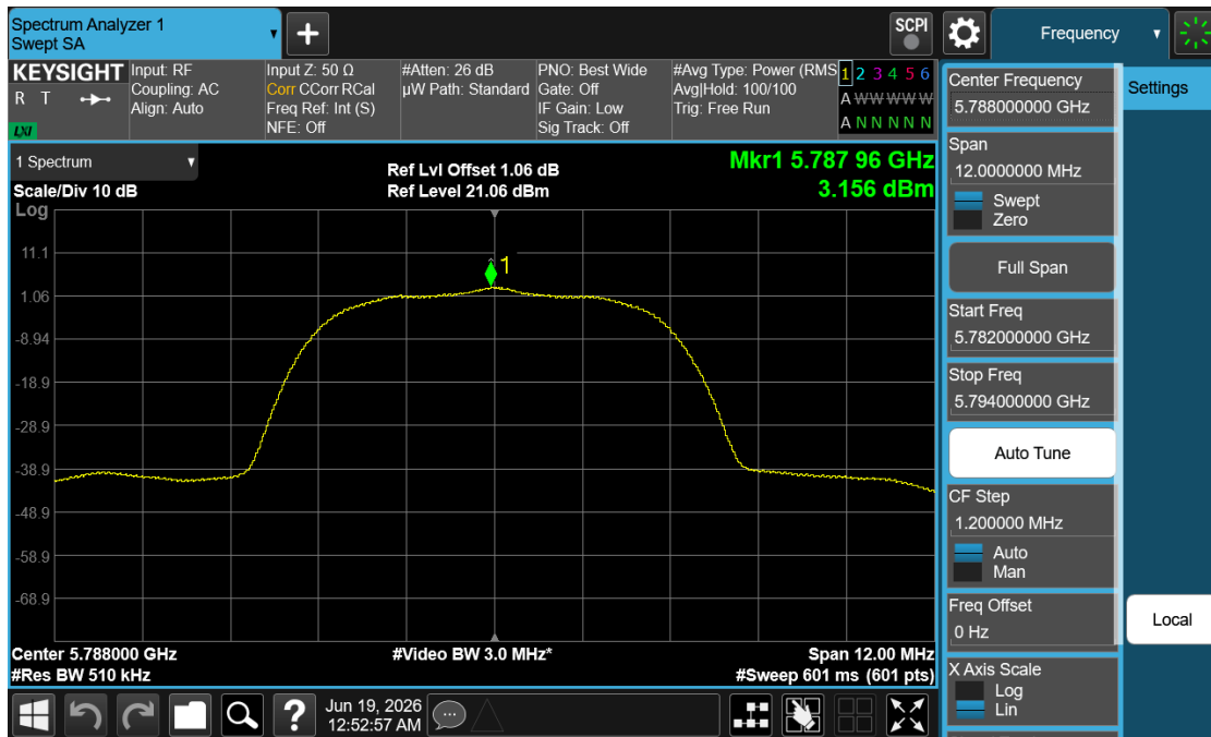
Plot 7-33. PSD (NB UNII HDR8 – 5788MHz)
