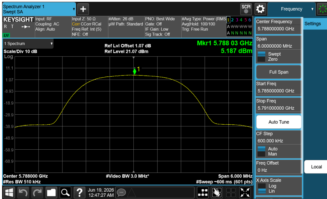
Plot 7-32. PSD (NB UNII HDR4 – 5788MHz)
