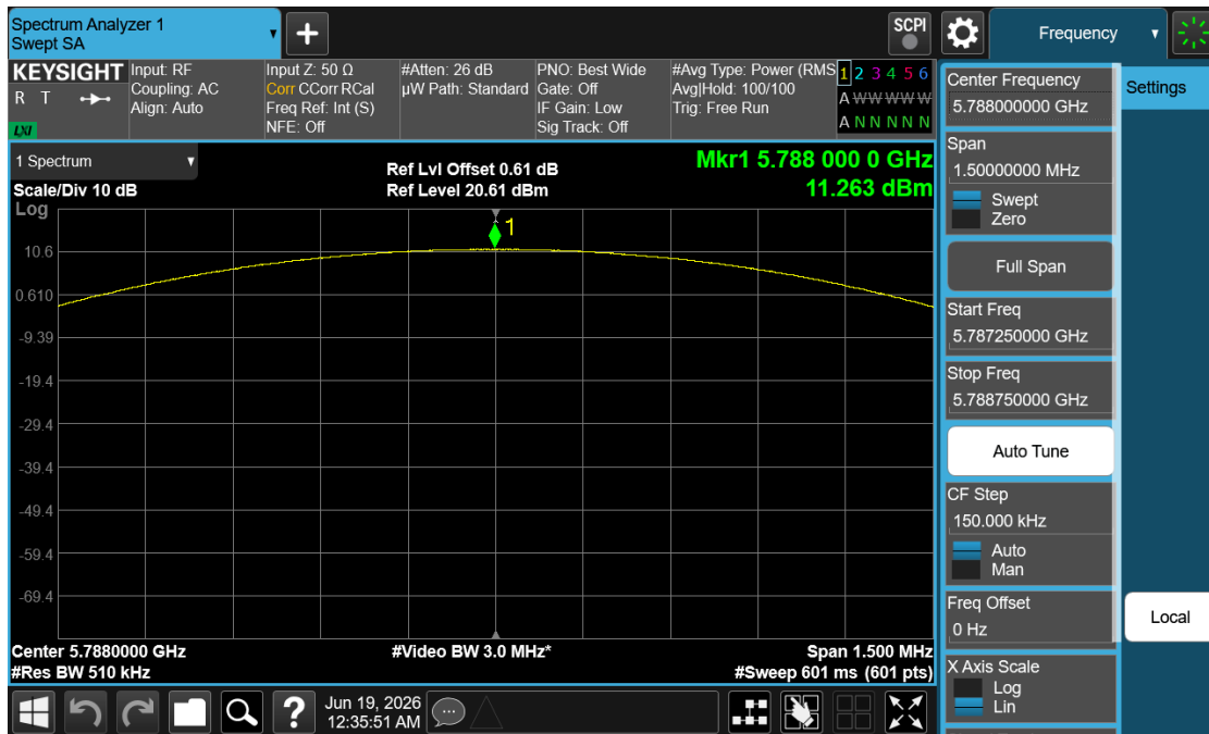
Plot 7-30. PSD (NB UNII LE1M – 5788MHz)
