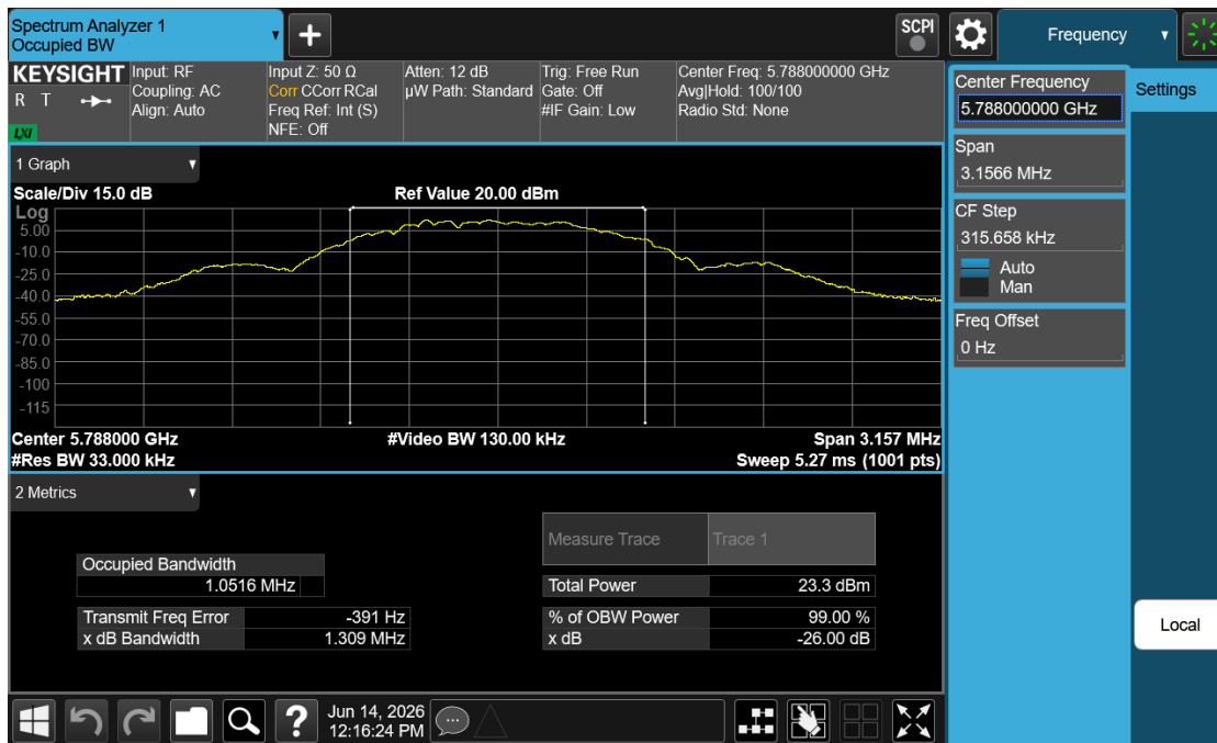
Plot 7-9. 99% OBW (NB UNII LE1M – 5788MHz)
