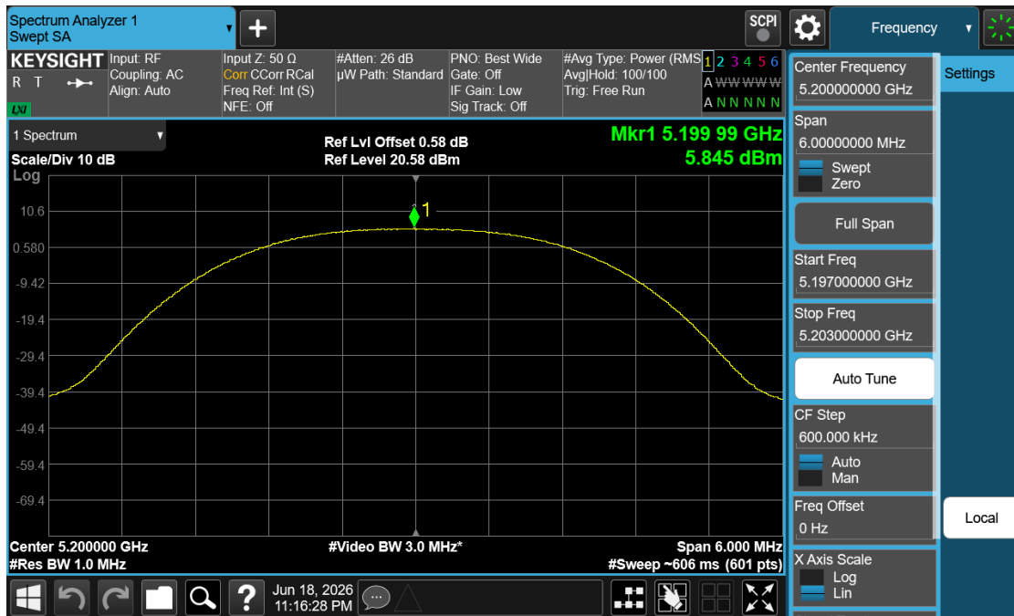
Plot 7-27. PSD (NB UNII HDRp4 – 5200MHz)
