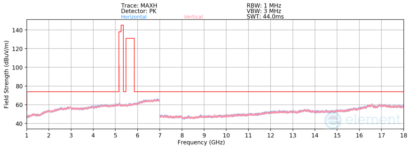
Plot 7-38. Radiated Spurious Emissions 1-18GHz (NB UNII BDR – 5200MHz)
