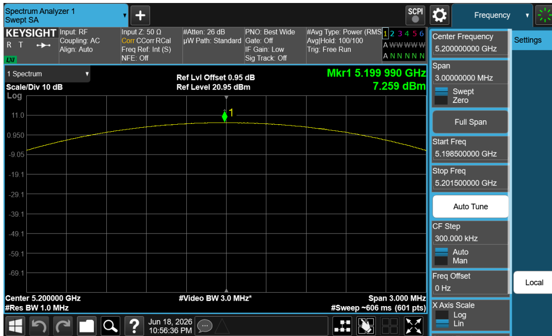
Plot 7-24. PSD (NB UNII LE2M – 5200MHz)
