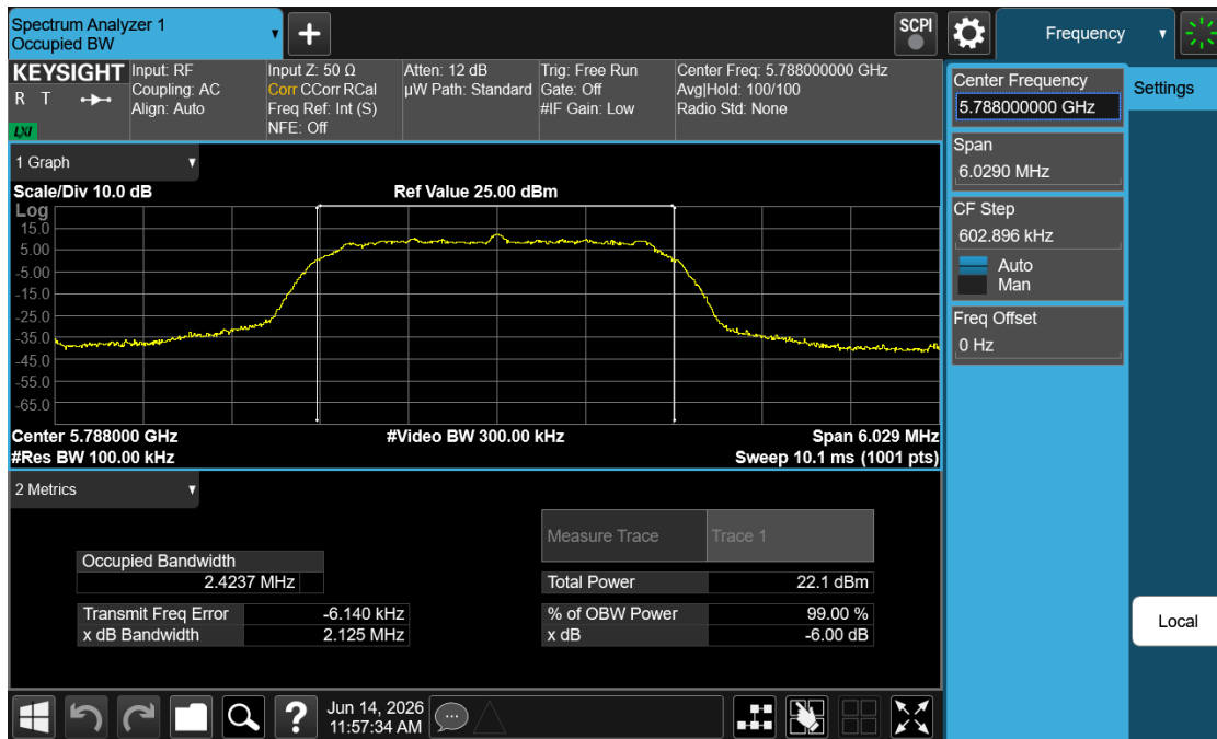
Plot 7-20. 6dB BW (NB UNII HDRp4 – 5788MHz)
