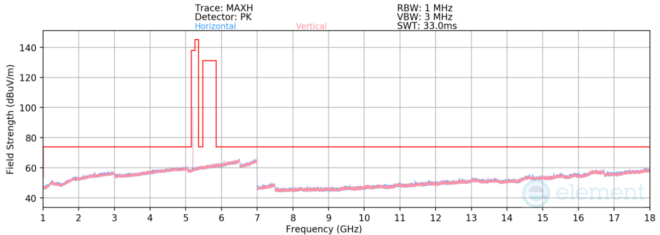
Plot 7-46. Radiated Spurious Emissions 1-18GHz (NB UNII HDR4 – 5200MHz)
