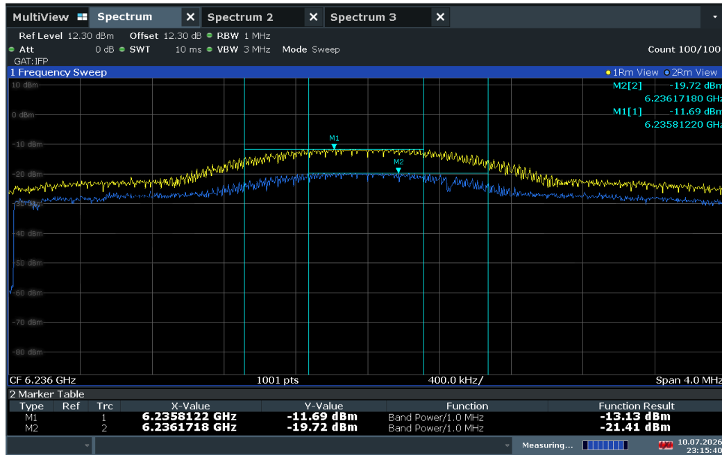
Plot 7-28. Power Density Plot – 6236MHz
