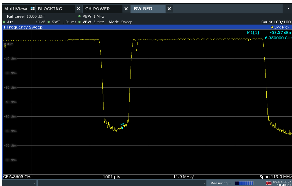
Plot 7-26. After AWGN Signal Injected
