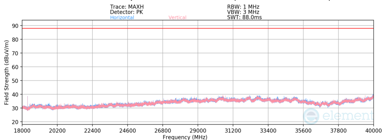
Plot 7-35. Radiated Spurious Emissions Above 18GHz (NB UNII LE1M – 6108MHz)
