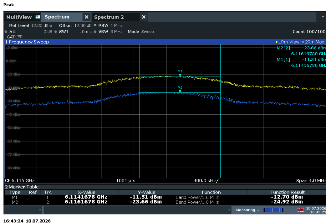
Plot 7-27. Power Density Plot 6115MHz
