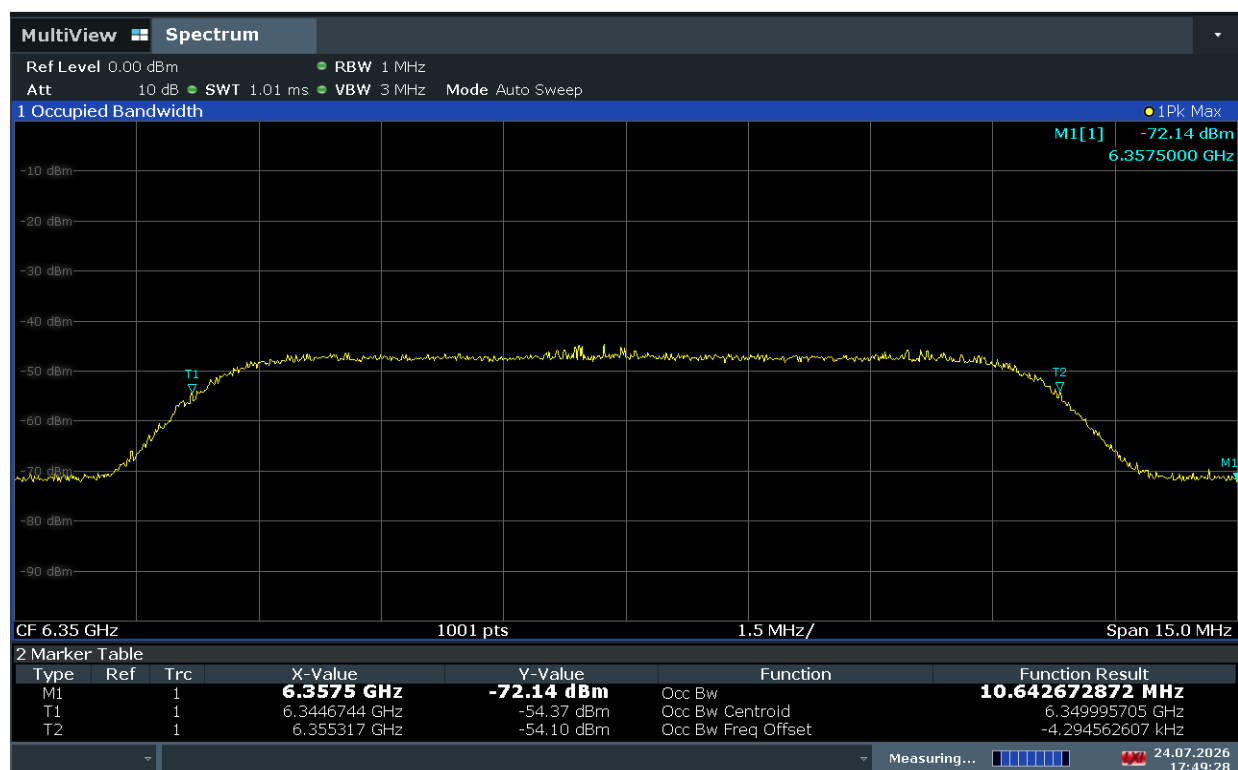
Plot 7-22. AWGN Signal
