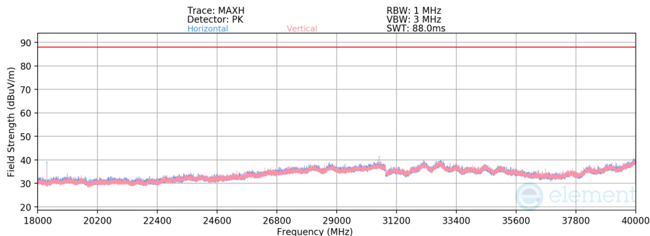
Plot 7-31. Radiated Spurious Emissions Above 18GHz (NB UNII BDR – 6108MHz)
