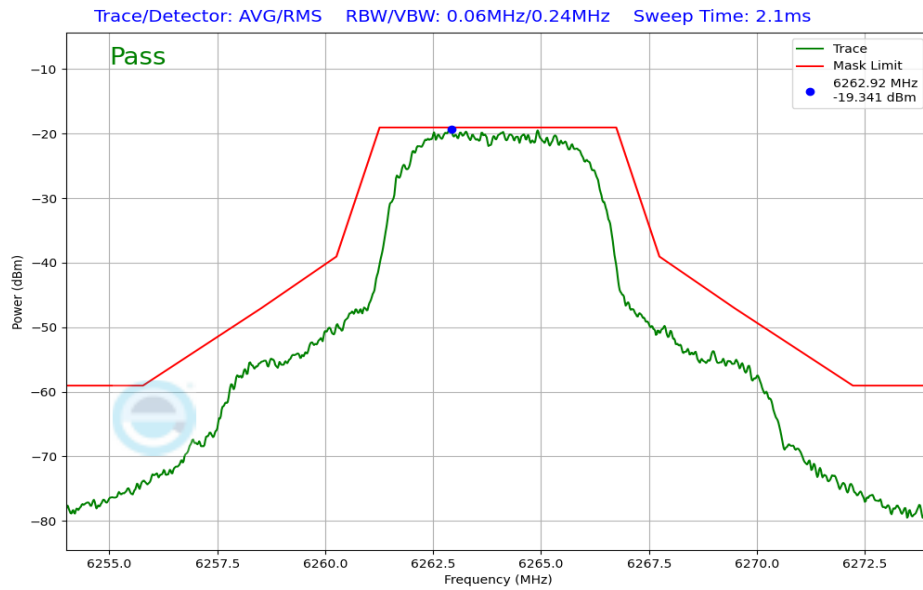
Plot 7-21. In-Band Emission (NB UNII HDRp8 – 6264MHz)
