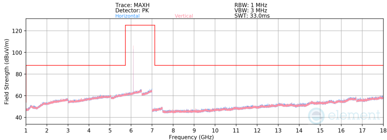
Plot 7-30. Radiated Spurious Emissions 1-18GHz (NB UNII BDR – 6108MHz)
