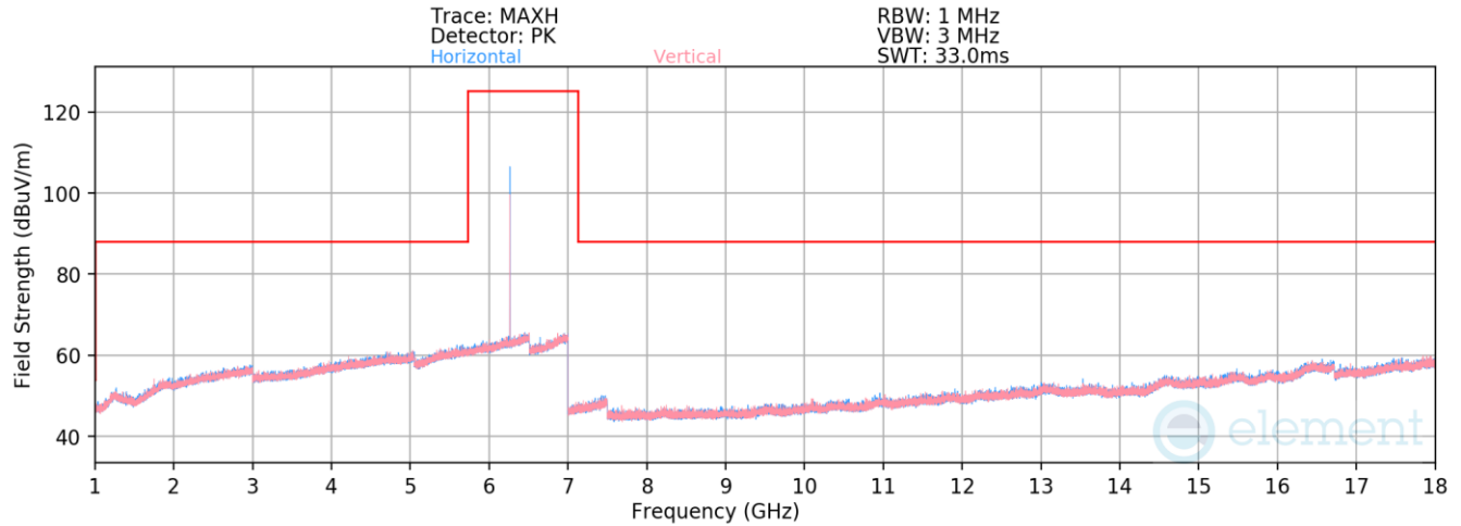
Plot 7-36. Radiated Spurious Emissions 1-18GHz (NB UNII LE1M – 6264MHz)
