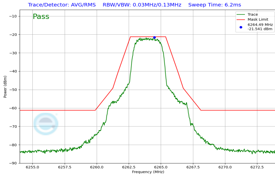
Plot 7-20. In-Band Emission (NB UNII HDRp4 – 6264MHz)
