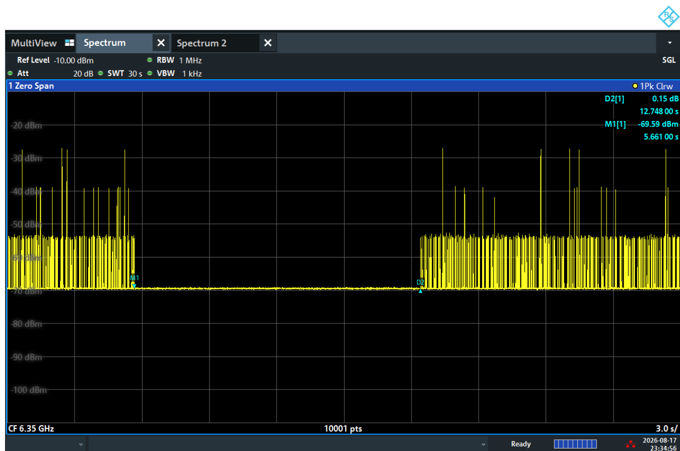
Plot 7-24. Contention Based Protocol Timing Plot
