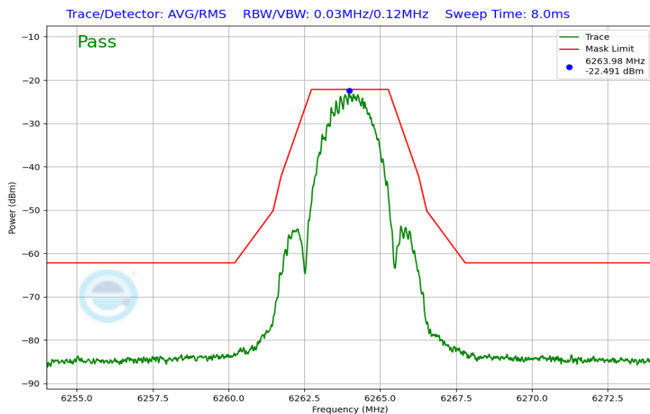
Plot 7-17. In-Band Emission (NB UNII LE2M – 6264MHz)
