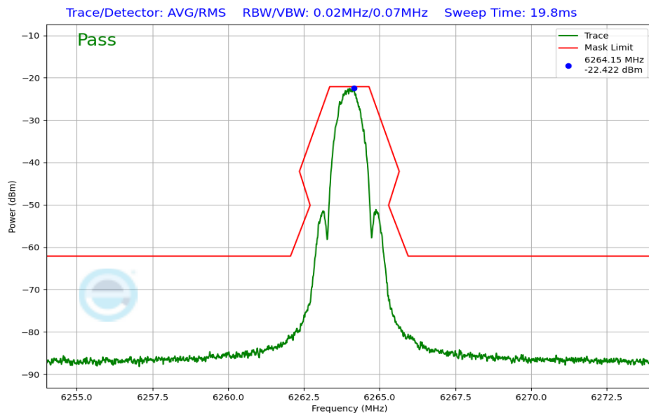
Plot 7-16. In-Band Emission (NB UNII LE1M – 6264MHz)
