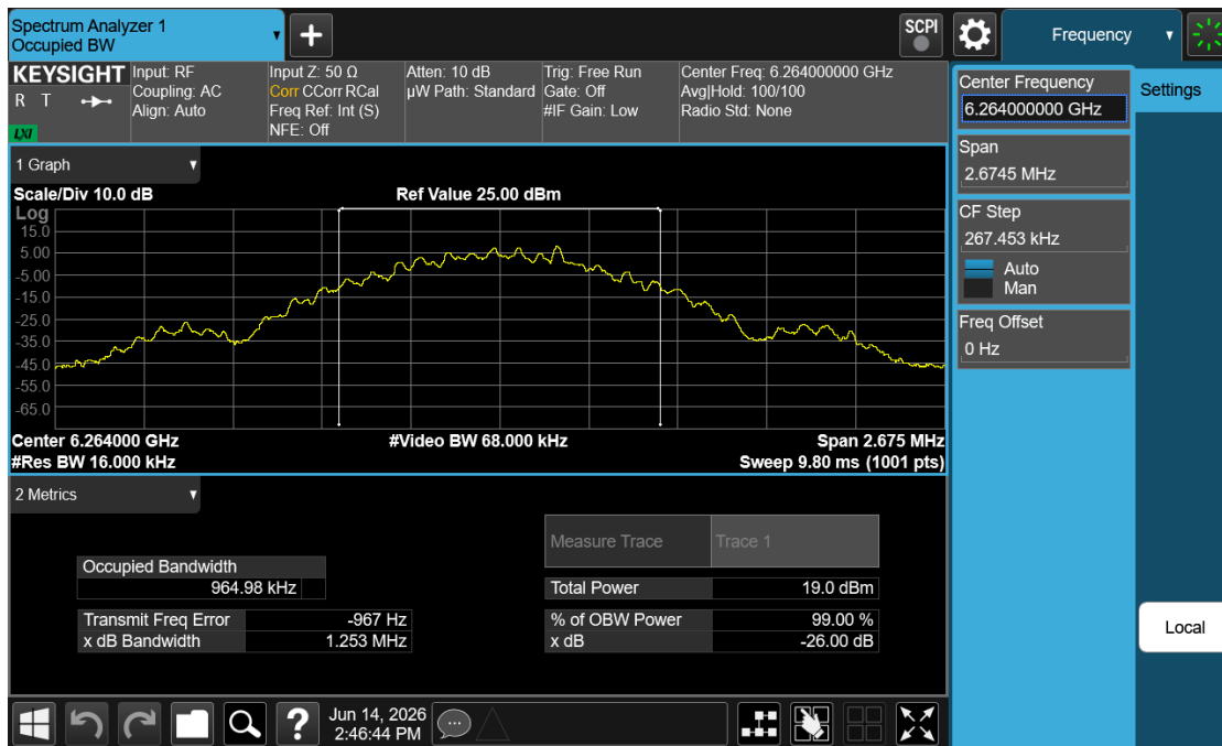
Plot 7-1. 26dB BW & 99% OBW (NB UNII BDR – 6264MHz)
