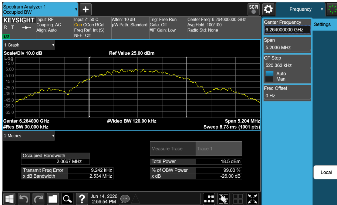
Plot 7-3. 26dB BW & 99% OBW (NB UNII LE2M – 6264MHz)
