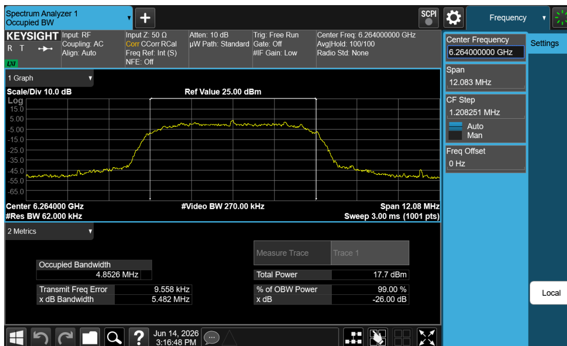
Plot 7-7. 26dB BW & 99% OBW (NB UNII HDRp8 – 6264MHz)
