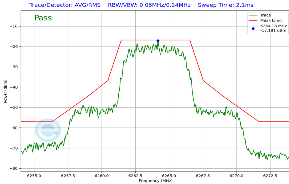
Plot 7-19. In-Band Emission (NB UNII HDR8 – 6264MHz)
