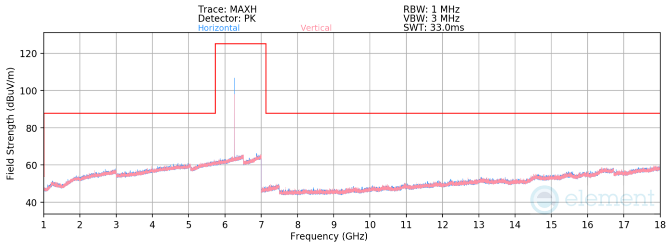
Plot 7-32. Radiated Spurious Emissions 1-18GHz (NB UNII BDR – 6264MHz)
