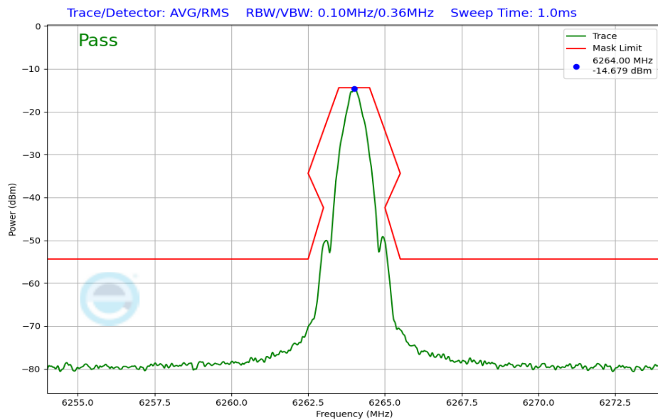
Plot 7-15. In-Band Emission (NB UNII BDR – 6264MHz)
