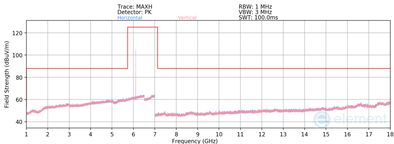
Plot 7-34. Radiated Spurious Emissions 1-18GHz (NB UNII LE1M – 6108MHz)
