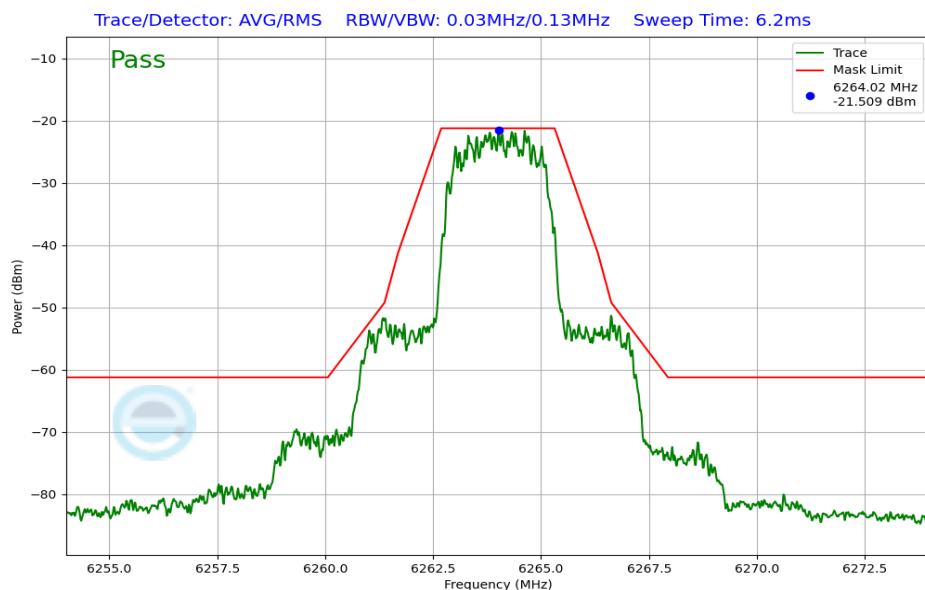
Plot 7-18. In-Band Emission (NB UNII HDR4 – 6264MHz)
