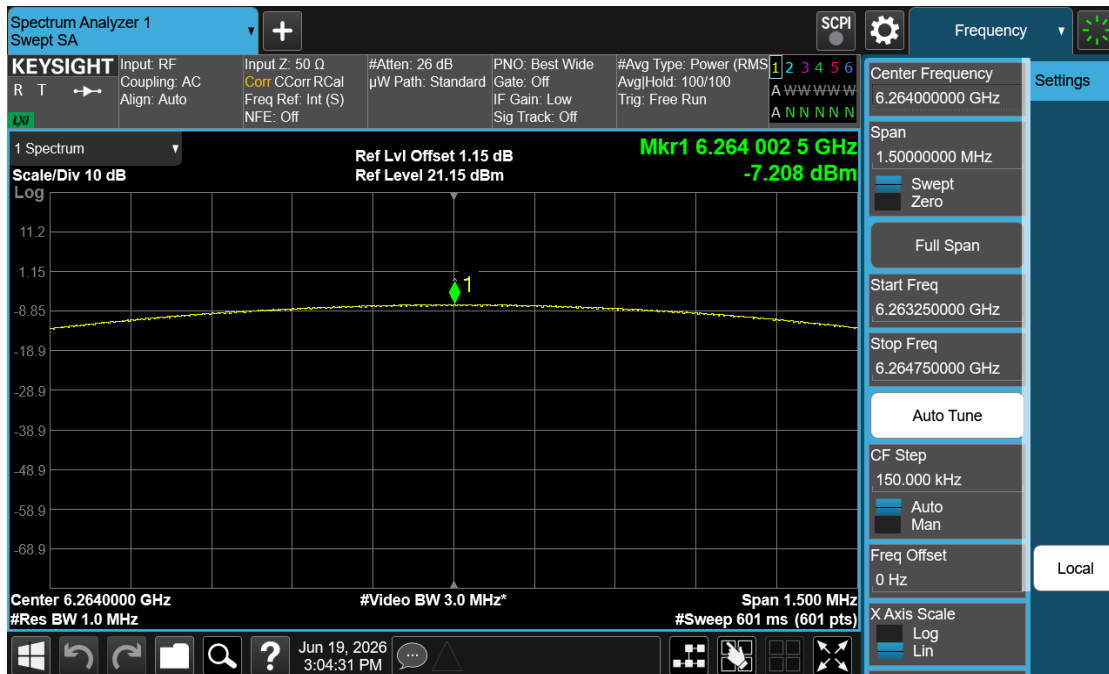
Plot 7-8. PSD (NB UNII BDR – 6264MHz)
