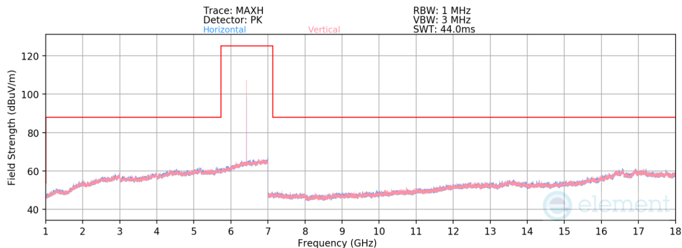
Plot 7-33. Radiated Spurious Emissions 1-18GHz (NB UNII BDR – 6420MHz)
