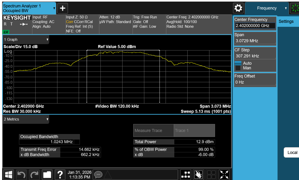
Plot 7-1. 99% BW Plot (Bluetooth (LE), 1Mbps – Ch. 0)
