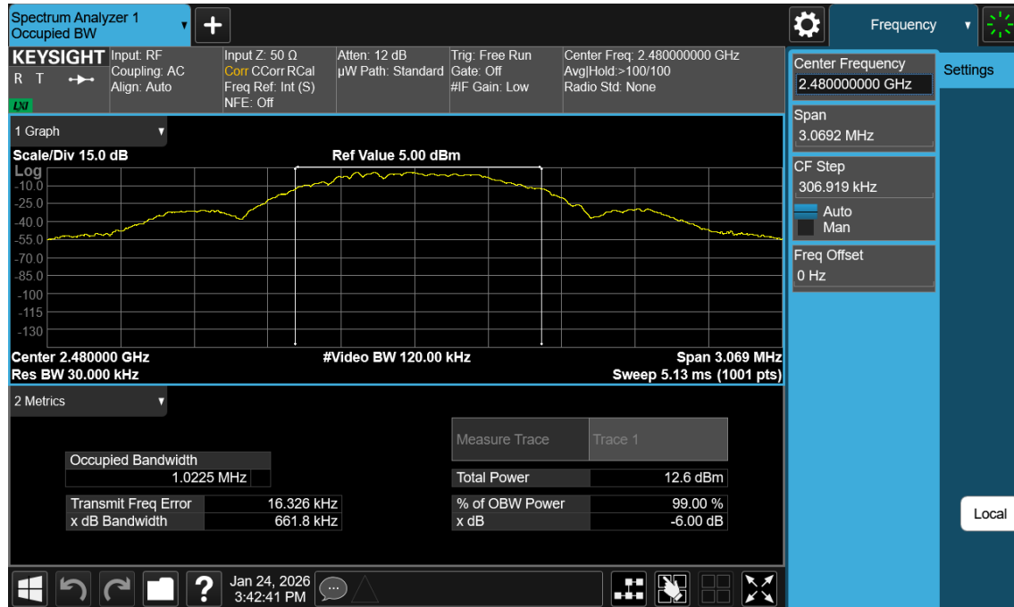
Plot 7-3. 99% BW Plot (Bluetooth (LE), 1Mbps – Ch. 39)
