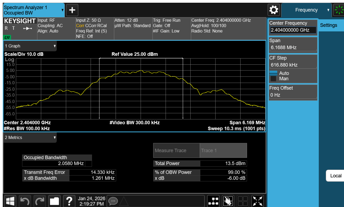
Plot 7-10. 6dB BW Plot (Bluetooth (LE), 2Mbps – Ch. 1)
