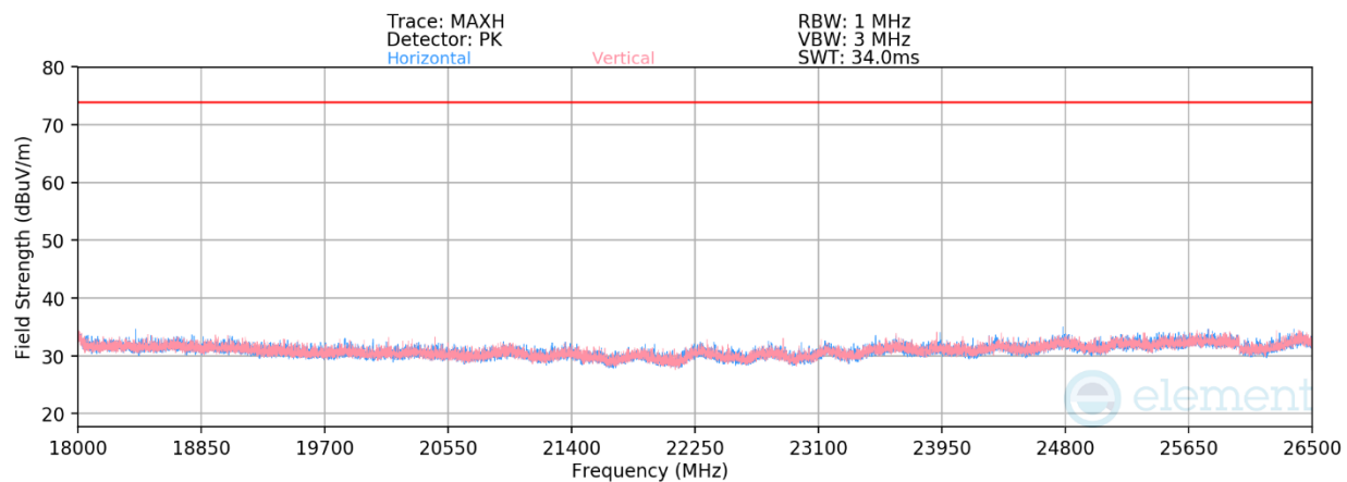
Plot 7-32. Radiated Spurious Emissions Above 18GHz (1Mbps – Ch. 39)
