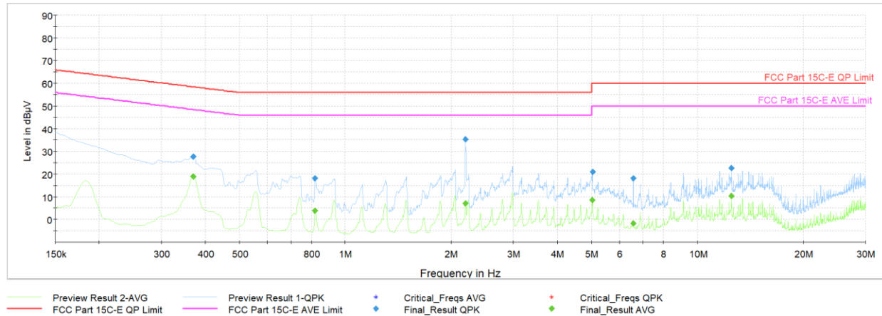
Plot 7-38. AC Line Conducted Plot with Bluetooth LE (L1, 1Mbps – Ch.39 with AC/DC Adaptor)
