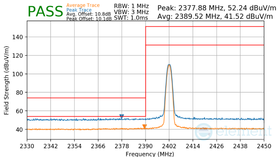
Plot 7-33. Radiated Restricted Lower Band Edge Measurement (Average & Peak)
