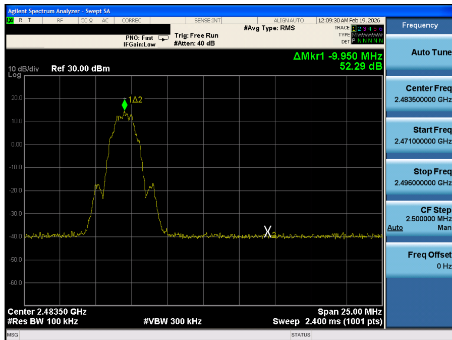
Plot 7-22. Band Edge Plot (Bluetooth (LE), 2Mbps – Ch. 38)
