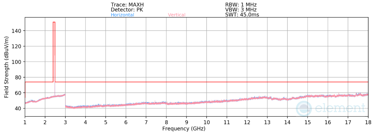
Plot 7-31. Radiated Spurious Emissions 1-18GHz (1Mbps – Ch. 39)
