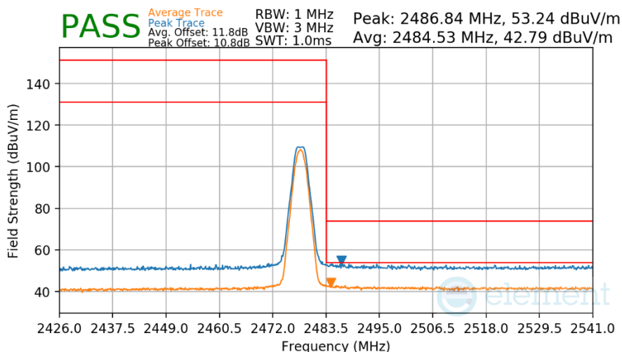
Plot 7-36. Radiated Restricted Upper Band Edge Measurement (Average & Peak)
