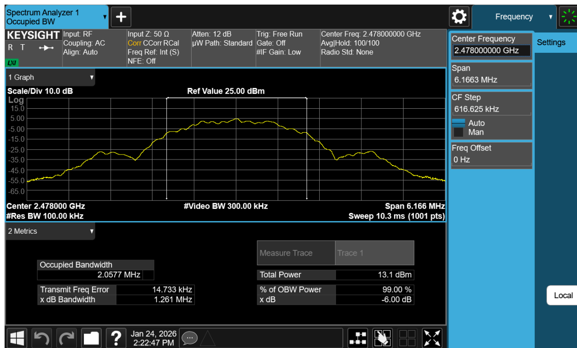
Plot 7-12. 6dB BW Plot (Bluetooth (LE), 2Mbps – Ch. 38)
