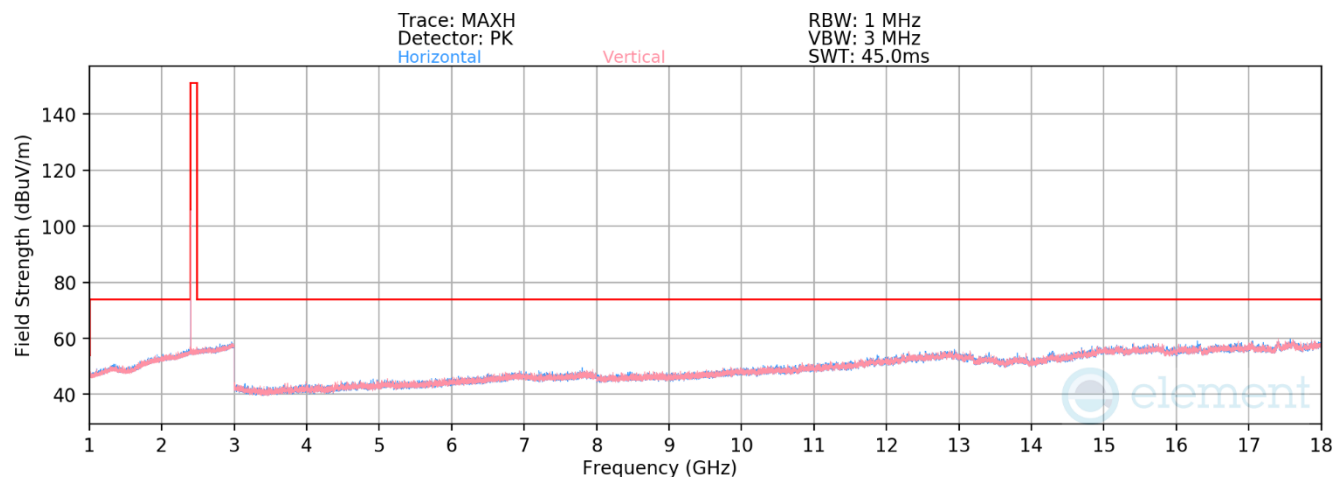
Plot 7-29. Radiated Spurious Emissions 1-18GHz (1Mbps – Ch. 0)
