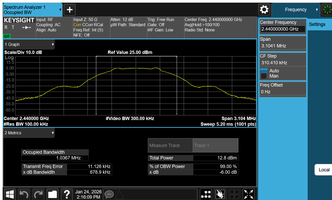
Plot 7-8. 6dB BW Plot (Bluetooth (LE), 1Mbps – Ch. 19)
