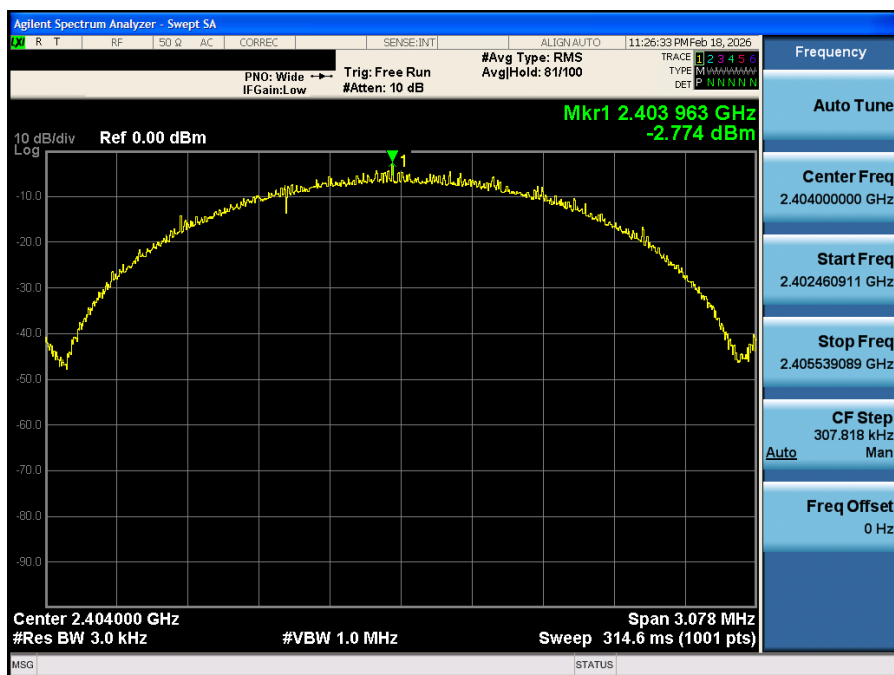
Plot 7-16. Power Spectral Density Plot (Bluetooth (LE), 2Mbps – Ch. 1)
