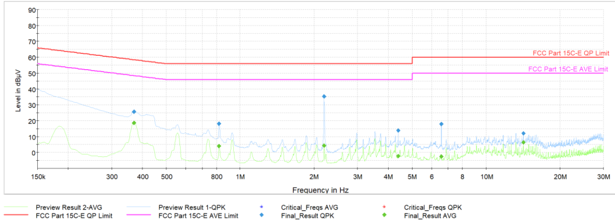
Plot 7-39. AC Line Conducted Plot with Bluetooth LE (N, 1Mbps – Ch.39, with Laptop)
