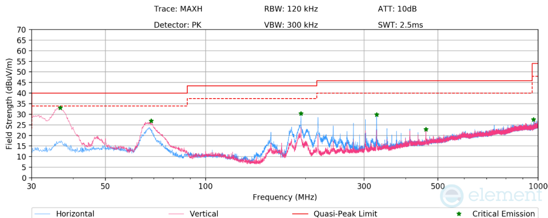
Plot 7-37. Radiated Spurious Emissions Below 1GHz (1Mbps – Ch.39, Pol. H & V, with AC/DC Adaptor)
