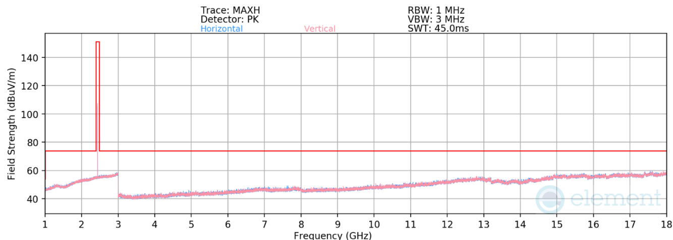
Plot 7-30. Radiated Spurious Emissions 1-18GHz (1Mbps – Ch. 19)
