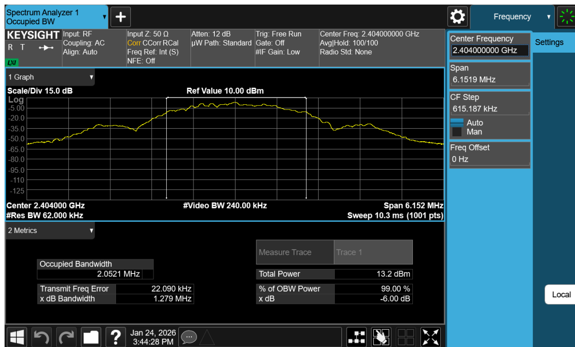
Plot 7-4. 99% BW Plot (Bluetooth (LE), 2Mbps – Ch. 1)
