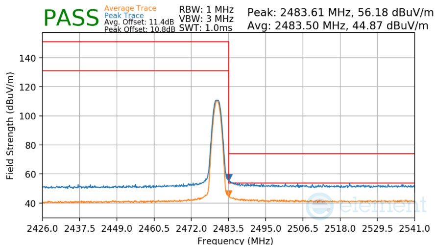
Plot 7-34. Radiated Restricted Upper Band Edge Measurement (Average & Peak)
