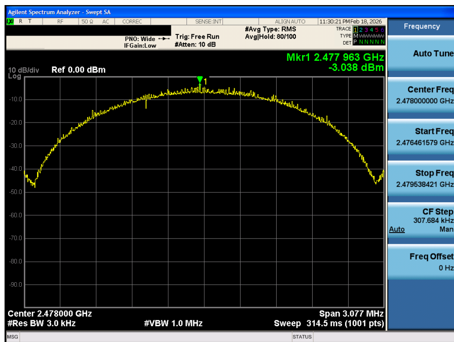
Plot 7-18. Power Spectral Density Plot (Bluetooth (LE), 2Mbps – Ch. 38)
