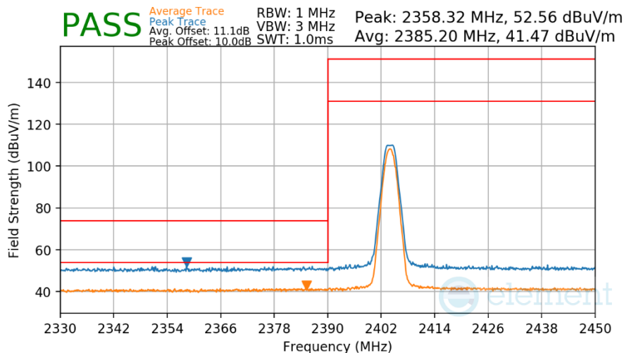
Plot 7-35. Radiated Restricted Lower Band Edge Measurement (Average & Peak)
