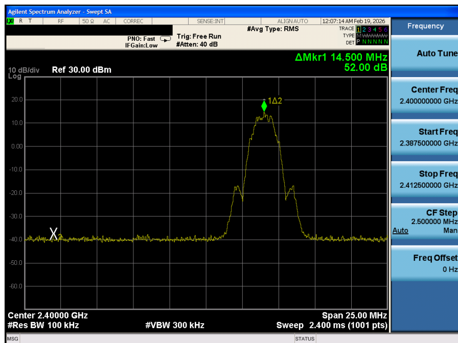
Plot 7-21. Band Edge Plot (Bluetooth (LE), 2Mbps – Ch. 1)
