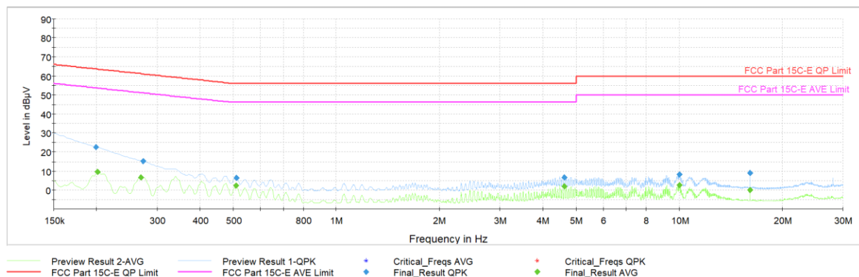
Plot 7-38. AC Line-Conducted Test Plot (L1, GFSK – Ch.78, with AC/DC Adapter)
