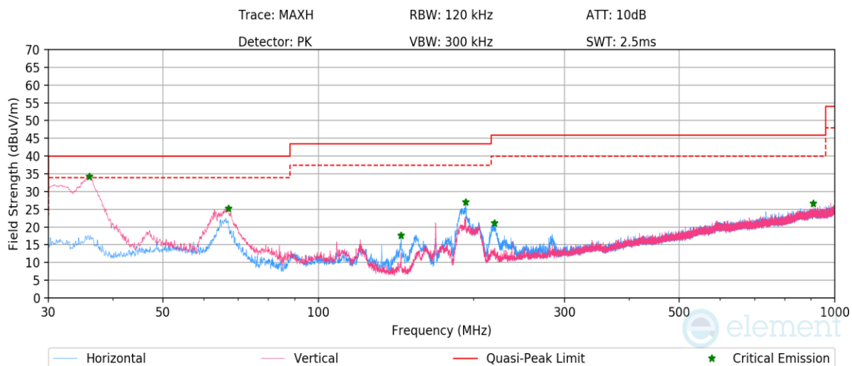
Plot 7-37. Radiated Spurious Emissions Below 1GHz (GFSK – Ch.78, with AC/DC Adapter)
