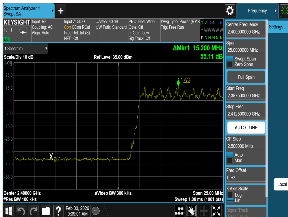
Plot 7-13. Band Edge Plot (Bluetooth with Hopping Enabled, 8DPSK – Ch.0)
