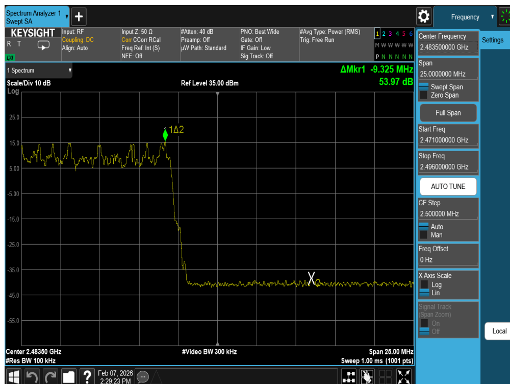
Plot 7-14. Band Edge Plot (Bluetooth with Hopping Enabled, 8DPSK – Ch.78)
