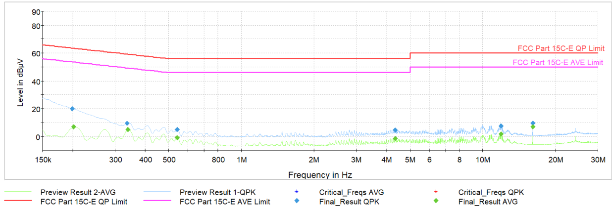
Plot 7-39. AC Line-Conducted Test Plot (N, GFSK – Ch.78, with AC/DC Adapter)
