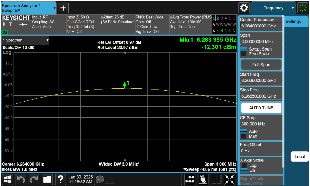
Plot 7-10. PSD (NB UNII LE2M – 6264MHz)
