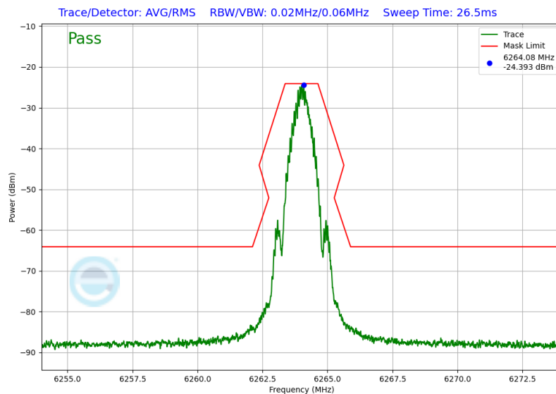
Plot 7-15. In-Band Emission (NB UNII BDR – 6264MHz)
