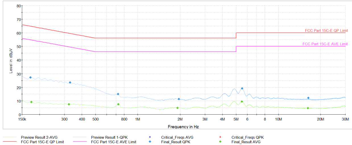
Plot 7-55. AC Line Conducted Plot (NB UNII LE1M – 6420MHz) (L1) with AC/DC adaptor
