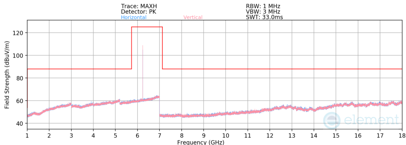
Plot 7-30. Radiated Spurious Emissions 1-18GHz (BDR - 6264MHz)
