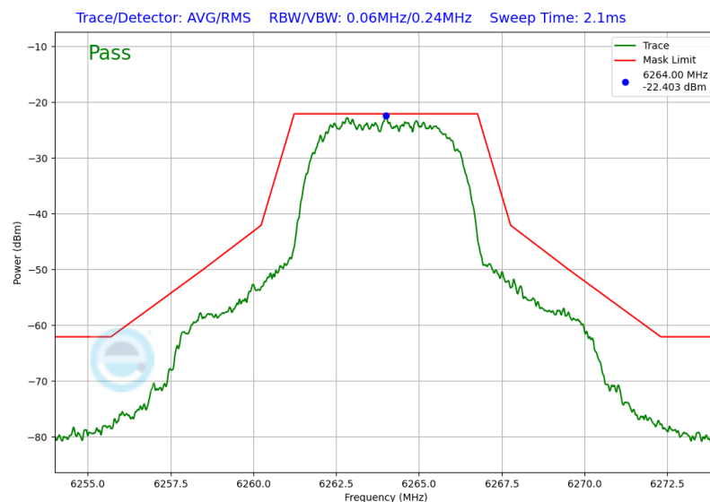
Plot 7-21. In-Band Emission (NB UNII HDRp8 – 6264MHz)
