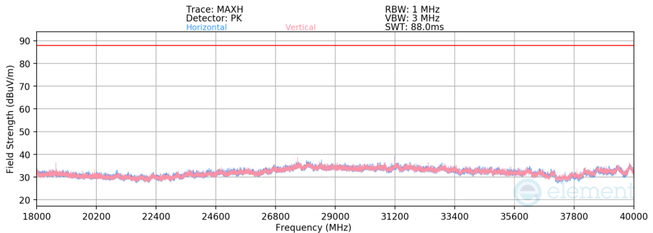
Plot 7-39. Radiated Spurious Emissions Above 18GHz (LE1M – 6264MHz)
