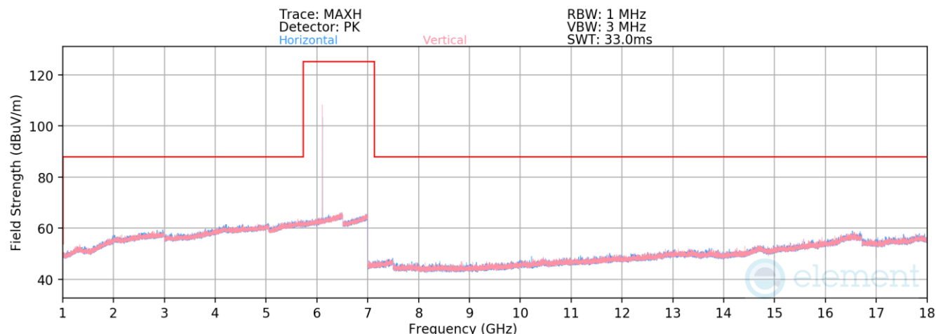
Plot 7-37. Radiated Spurious Emissions 1-18GHz (LE1M – 6108MHz)
