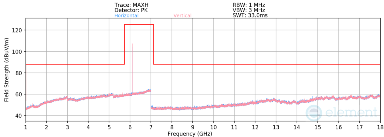
Plot 7-29. Radiated Spurious Emissions 1-18GHz (BDR – 6108MHz)
