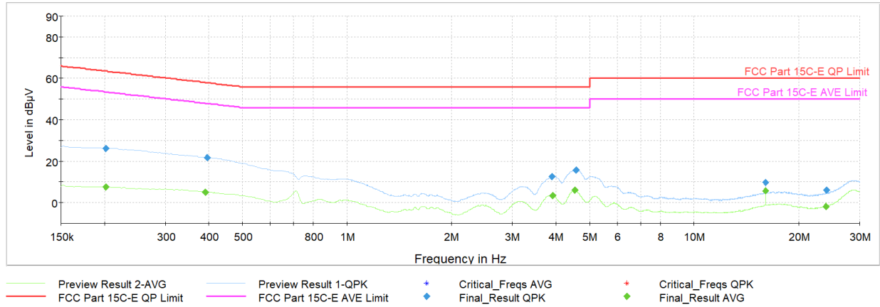
Plot 7-52. AC Line Conducted Plot (NB UNII BDR – 6420MHz) (N) with AC/DC adaptor
