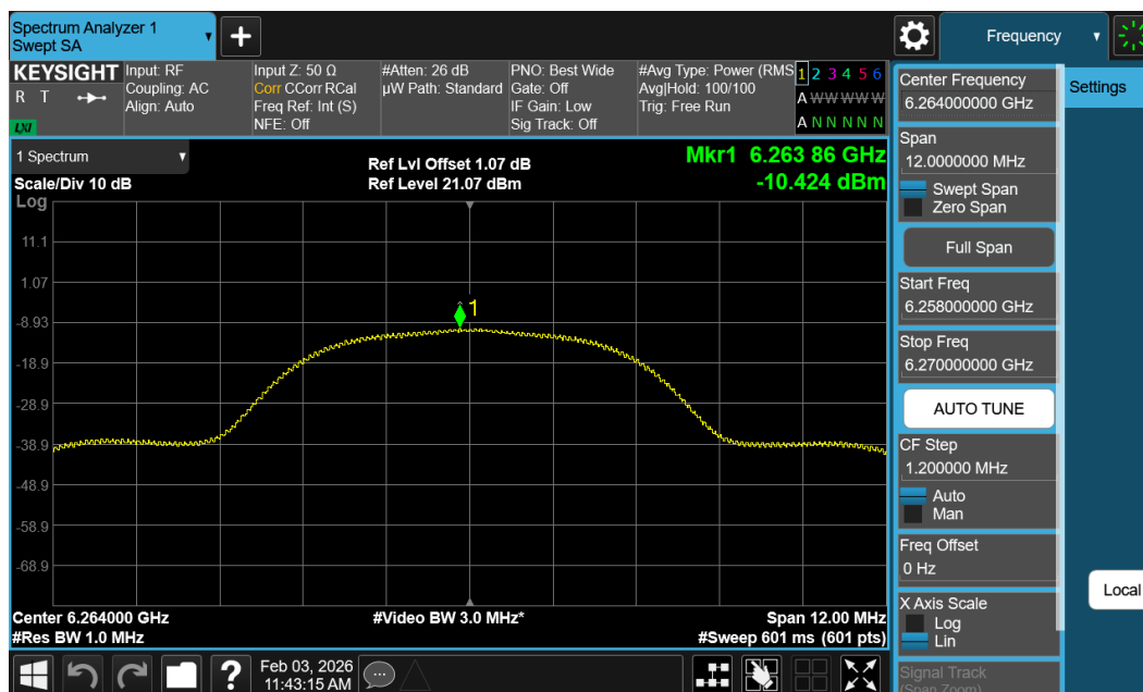
Plot 7-12. PSD (NB UNII HDR8 – 6264MHz)
