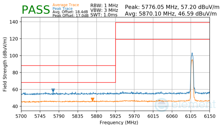
Plot 7-45 Radiated Lower Band Edge Measurement
