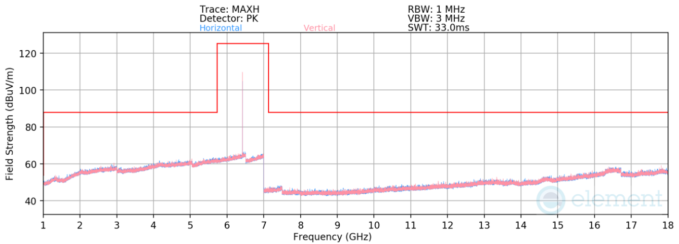
Plot 7-40. Radiated Spurious Emissions 1-18GHz (LE1M – 6420MHz)
