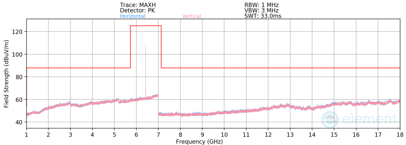
Plot 7-31. Radiated Spurious Emissions 1-18GHz (BDR – 6420MHz)
