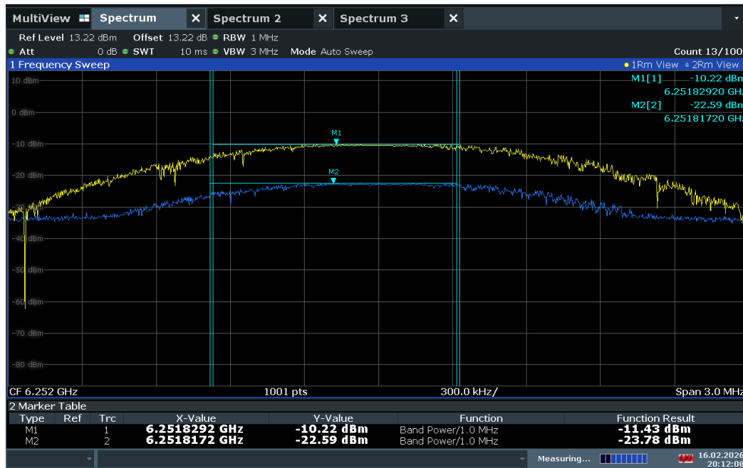
Plot 7-27. Power Density Plot – 6252MHz
