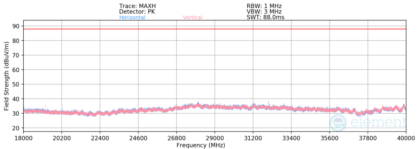
Plot 7-36. Radiated Spurious Emissions Above 18GHz (HDR4 – 6420MHz)
