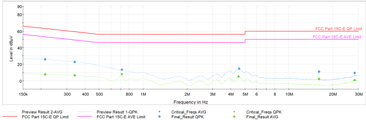
Plot 7-51. AC Line Conducted Plot (NB UNII BDR – 6420MHz) (L1) with AC/DC adaptor
