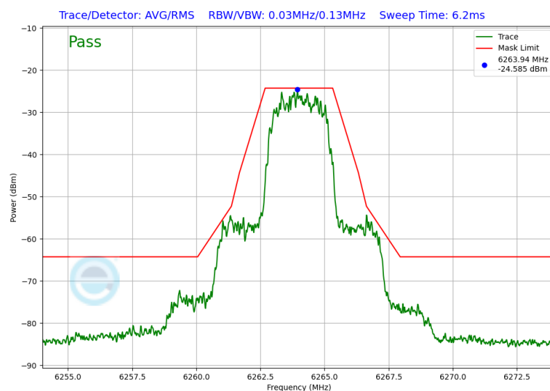
Plot 7-18. In-Band Emission (NB UNII HDR4 – 6264MHz)
