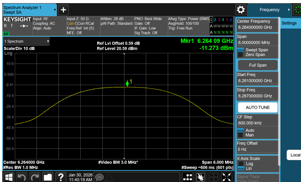
Plot 7-13. PSD (NB UNII HDRp4 – 6264MHz)
