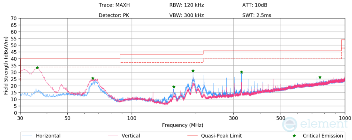
Plot 7-48. Radiated Spurious Emissions Below 1GHz (NB UNII BDR – 6420MHz), with AC/DC adaptor
