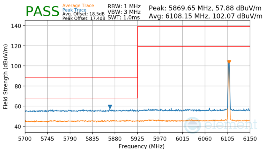
Plot 7-42 Radiated Lower Band Edge Measurement
