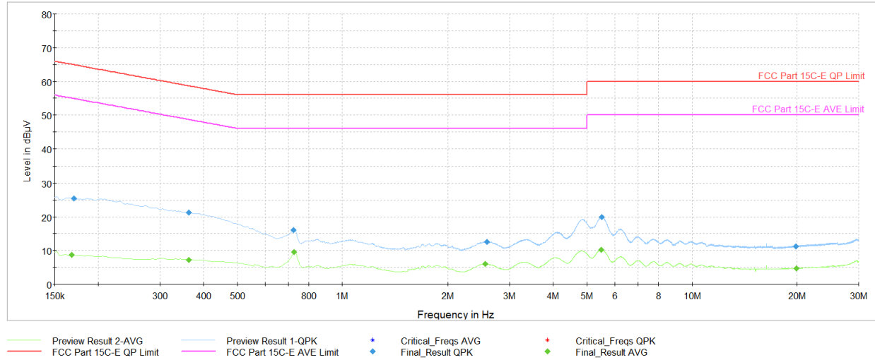
Plot 7-54. AC Line Conducted Plot (NB UNII HDR4 – 6264MHz) (N) with AC/DC adaptor
