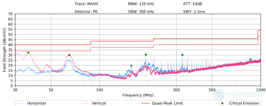
Plot 7-49. Radiated Spurious Emissions Below 1GHz (NB UNII HDR4 – 6420MHz), with AC/DC adaptor
