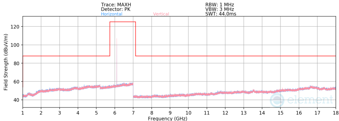
Plot 7-33. Radiated Spurious Emissions 1-18GHz (HDR4 – 6108MHz)
