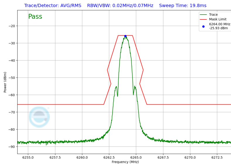
Plot 7-16. In-Band Emission (NB UNII LE1M – 6264MHz)
