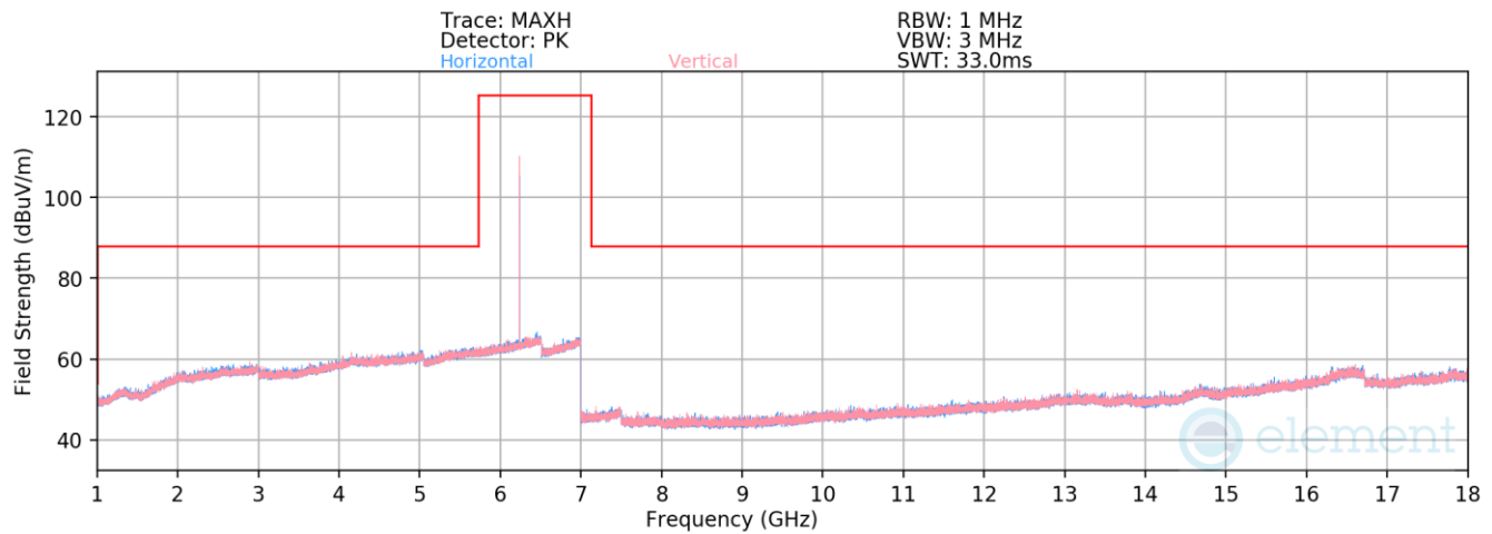
Plot 7-38. Radiated Spurious Emissions 1-18GHz (LE1M – 6264MHz)
