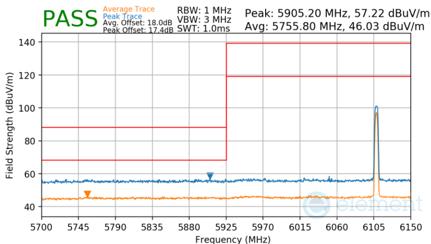
Plot 7-46 Radiated Lower Band Edge Measurement
