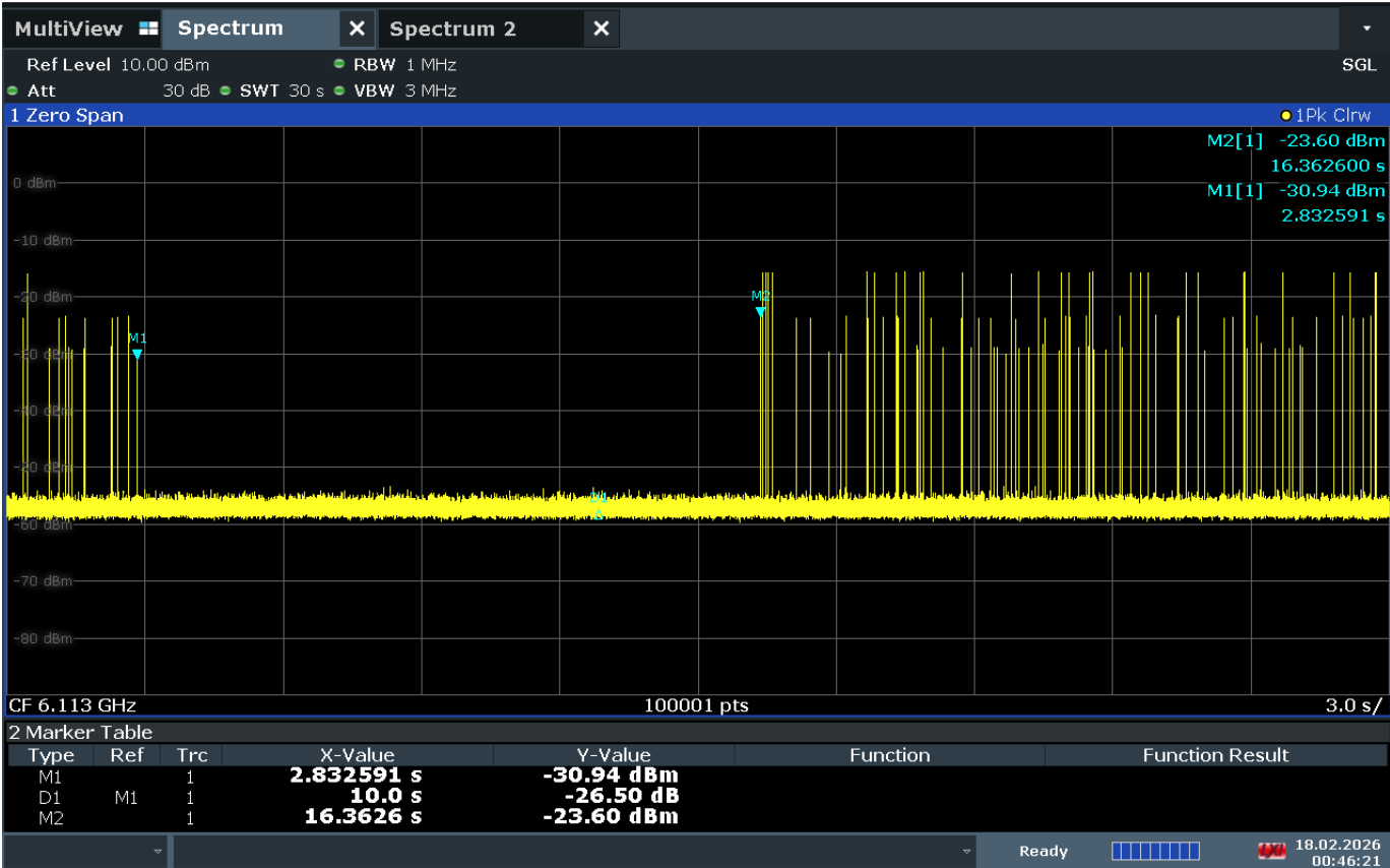
Plot 7-23. Contention Based Protocol Timing Plot
