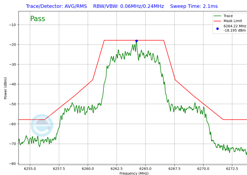
Plot 7-19. In-Band Emission (NB UNII HDR8 – 6264MHz)
