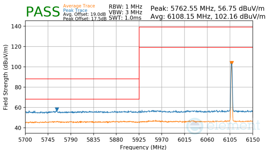
Plot 7-41 Radiated Lower Band Edge Measurement
