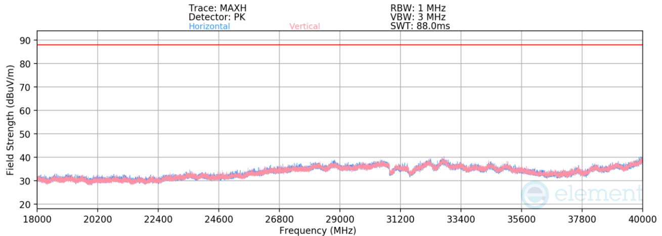
Plot 7-32. Radiated Spurious Emissions Above 18GHz (BDR – 6420MHz)
