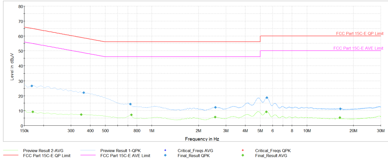
Plot 7-53. AC Line Conducted Plot (NB UNII HDR4 – 6264MHz) (L1) with AC/DC adaptor
