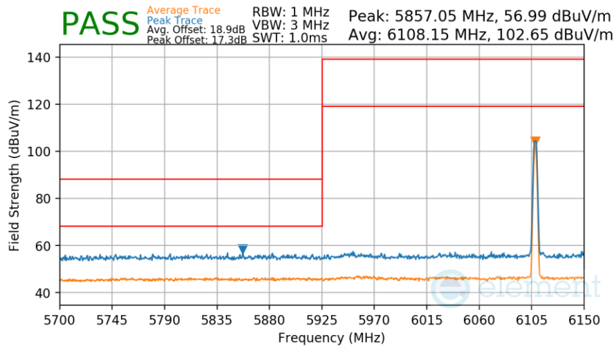
Plot 7-43 Radiated Lower Band Edge Measurement
