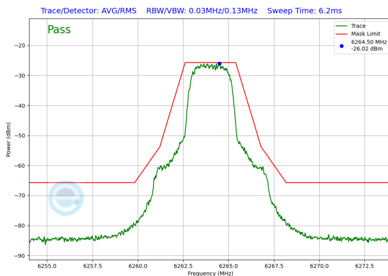
Plot 7-20. In-Band Emission (NB UNII HDRp4 – 6264MHz)
