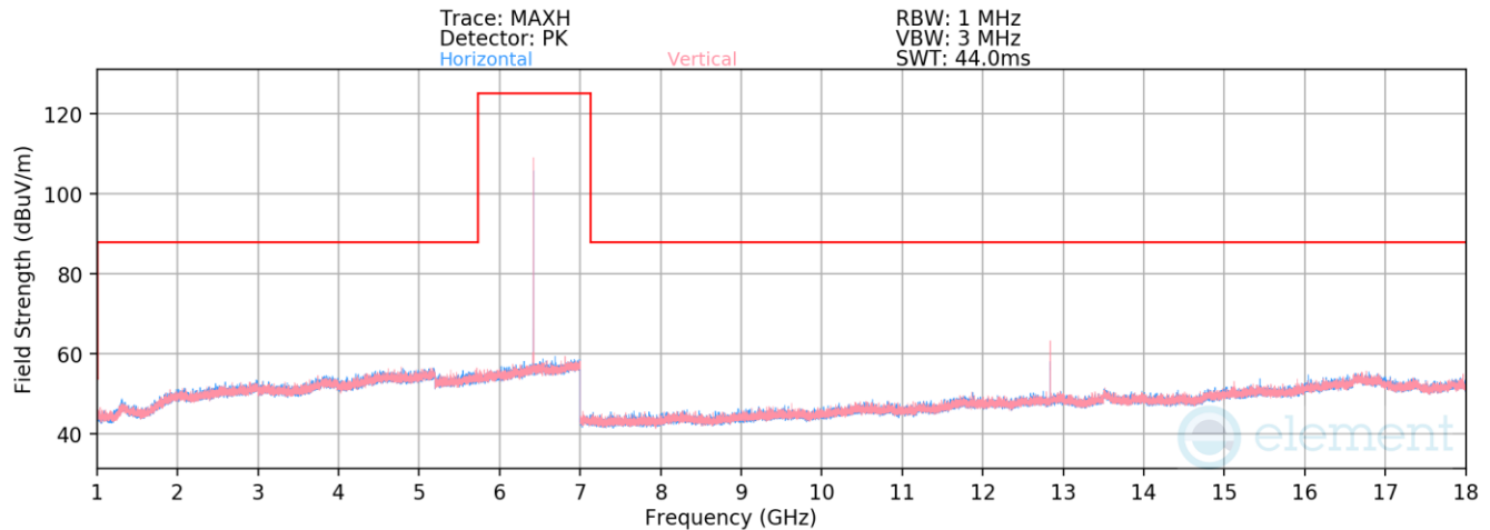
Plot 7-35. Radiated Spurious Emissions 1-18GHz (HDR4 – 6420MHz)
