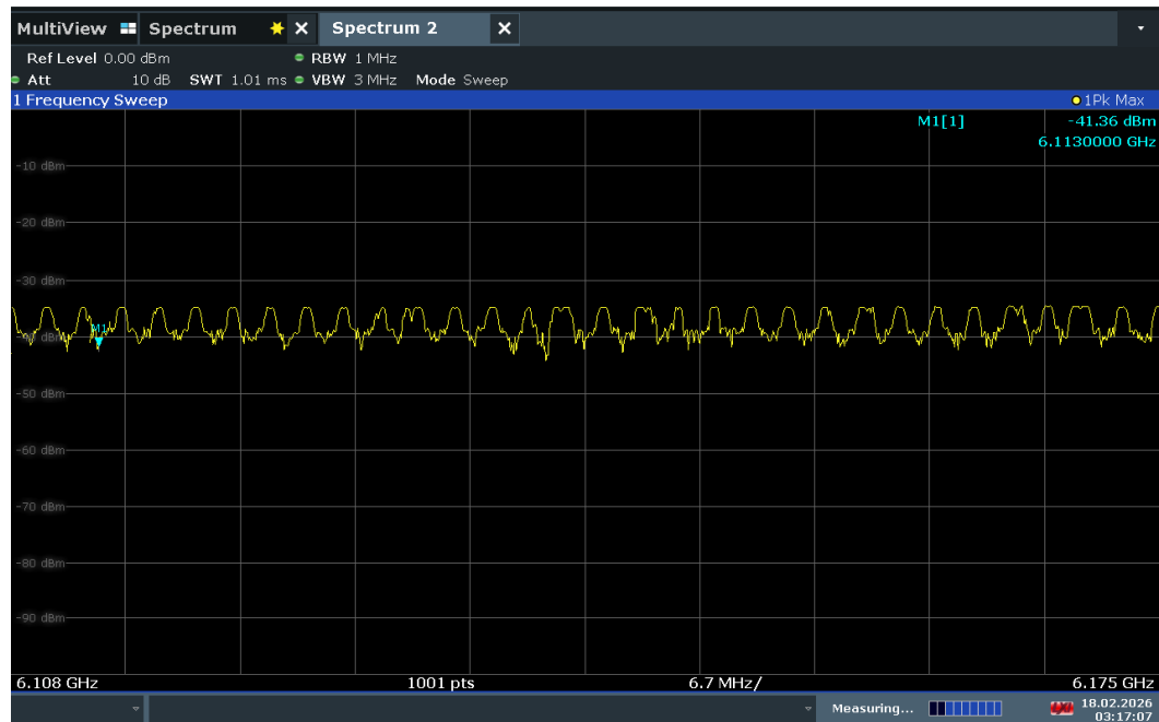
Plot 7-24. Before AWGN Signal Injected
