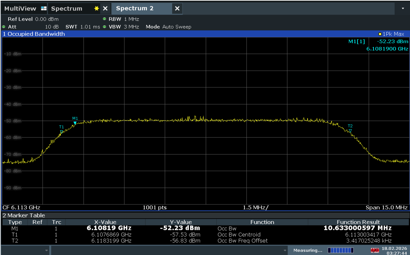
Plot 7-22. AWGN Signal
