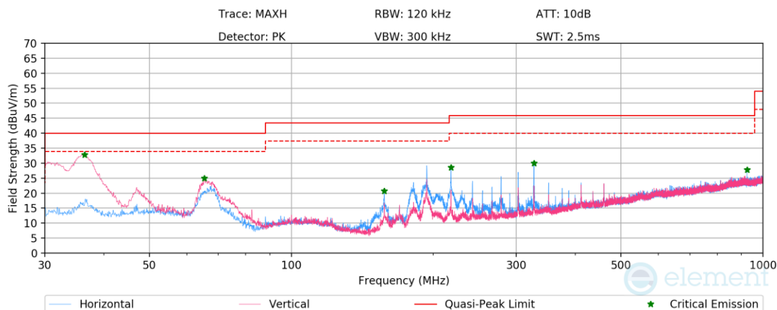
Plot 7-50. Radiated Spurious Emissions Below 1GHz (NB UNII LE1M – 6264MHz), with AC/DC adaptor
