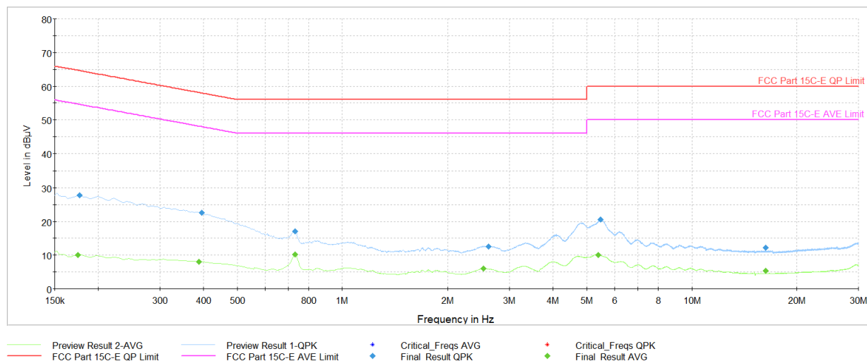
Plot 7-56. AC Line Conducted Plot (NB UNII LE1M – 6420MHz) (N) with AC/DC adaptor
