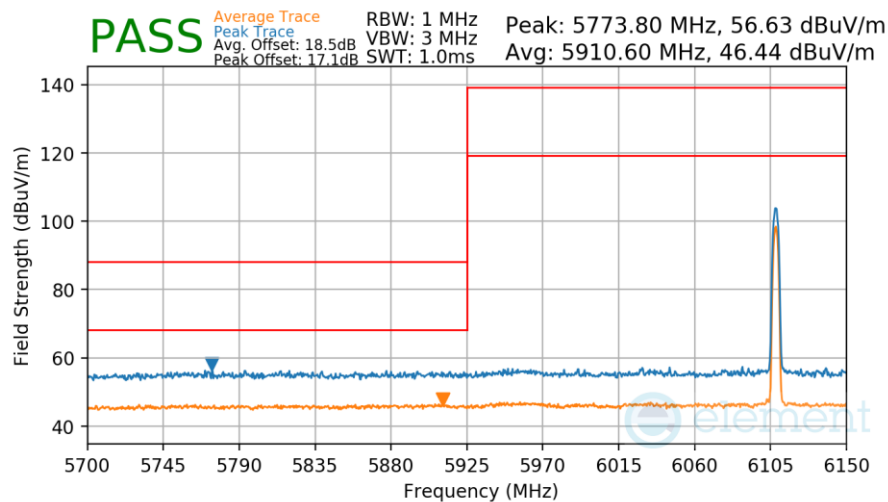
Plot 7-44 Radiated Lower Band Edge Measurement
