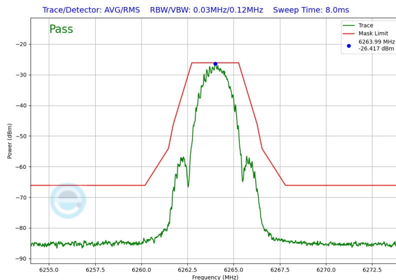
Plot 7-17. In-Band Emission (NB UNII LE2M – 6264MHz)
