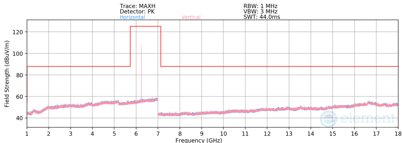
Plot 7-34. Radiated Spurious Emissions 1-18GHz (HDR4 – 6264MHz)
