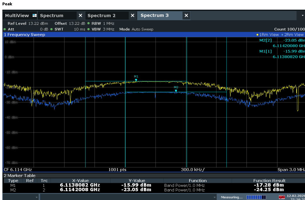
Plot 7-26. Power Density Plot 6114MHz
