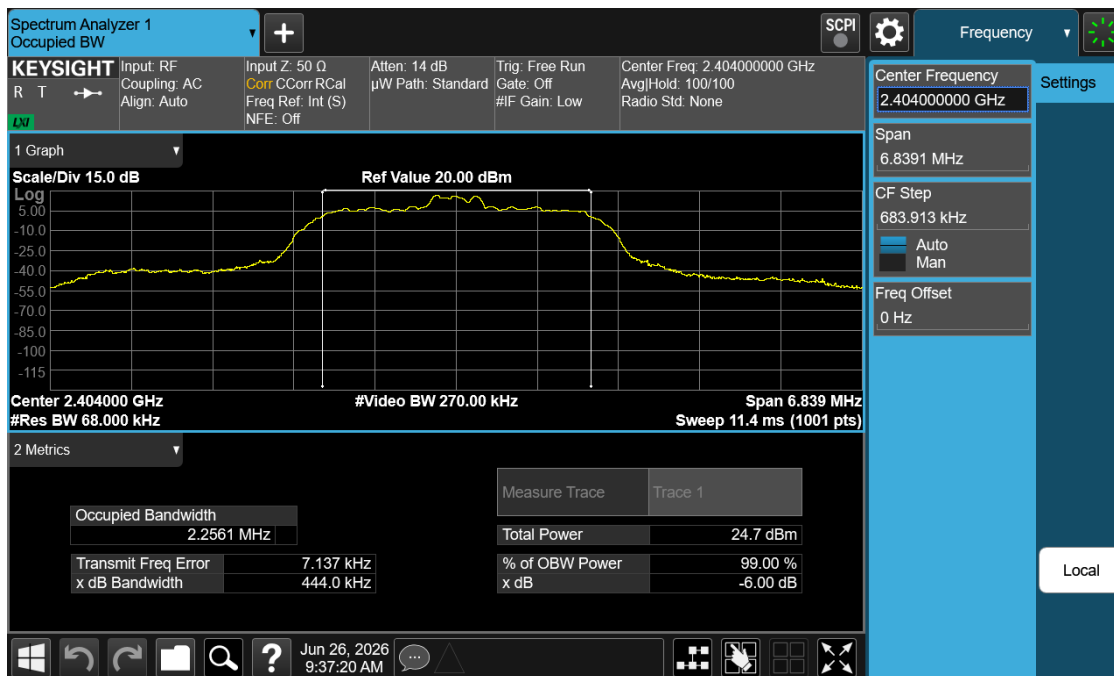
Plot 7-1. 99% OBW Plot (Bluetooth (HDR4), 4Mbps – Ch. 1)
