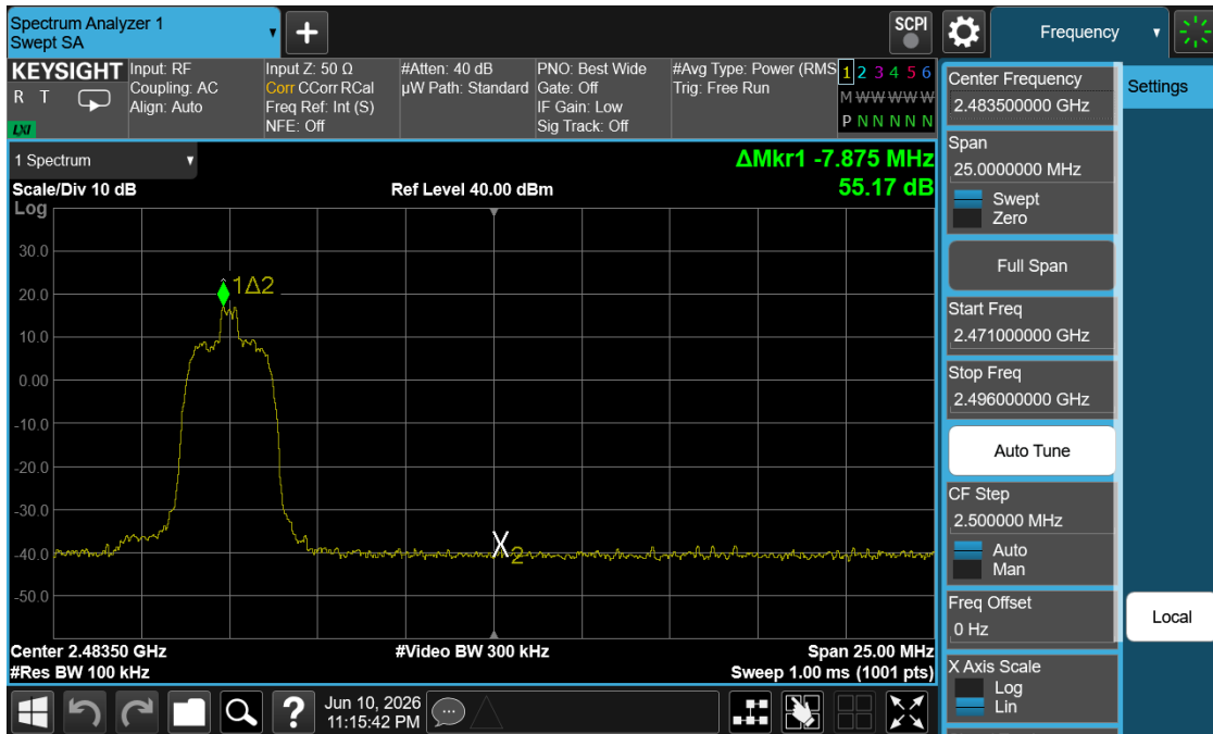
Plot 7-38. Band Edge Plot (Bluetooth (HDR4) – Ch. 73)
