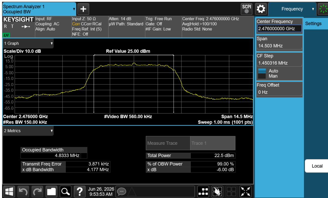
Plot 7-12. 99% OBW Plot (Bluetooth (HDRp8), 8Mbps, – Ch. 73)
