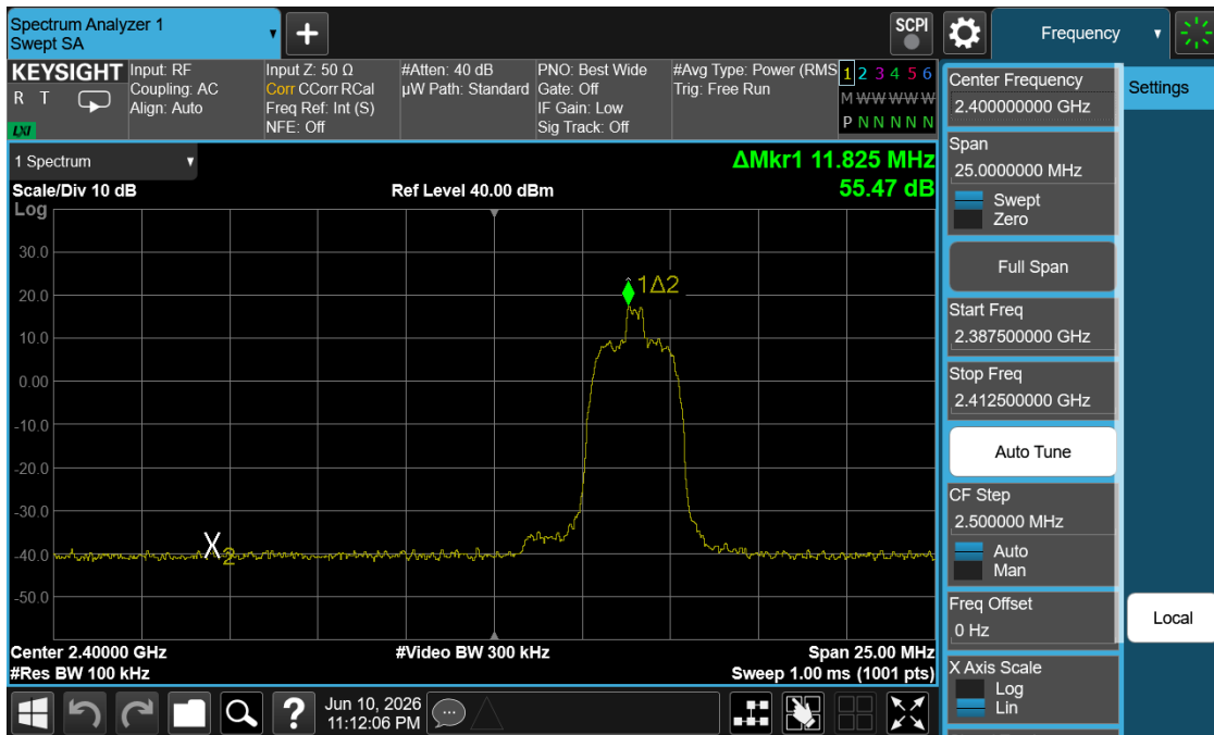
Plot 7-37. Band Edge Plot (Bluetooth (HDR4) – Ch. 1)
