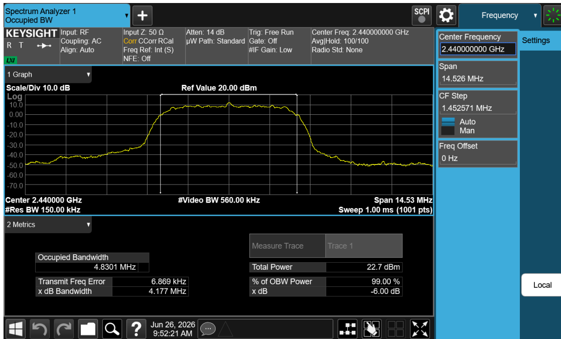
Plot 7-11. 99% OBW Plot (Bluetooth (HDRp8), 8Mbps, – Ch. 38)
