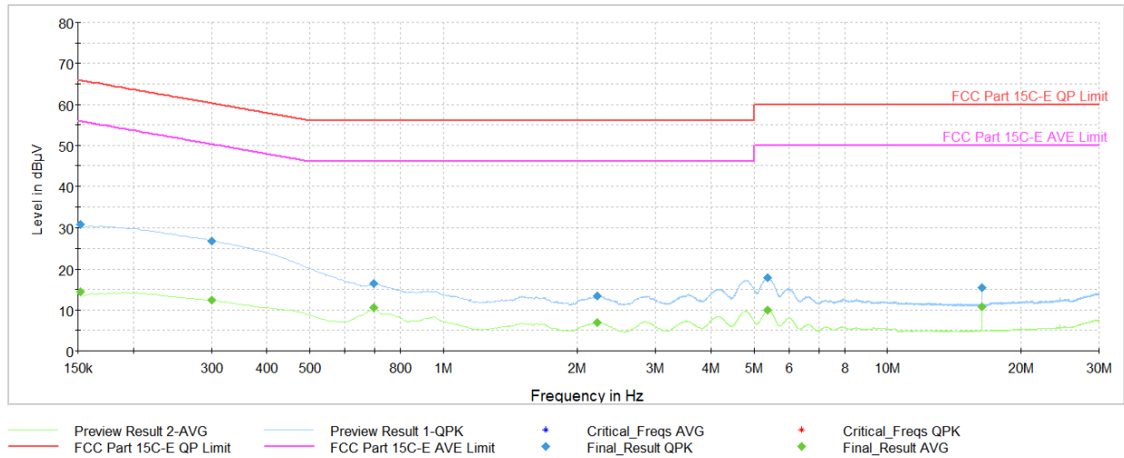
Plot 7-35. AC Line Conducted Plot with Bluetooth LE (L1, 1Mbps – Ch.17 with AC/DC Adapter)
