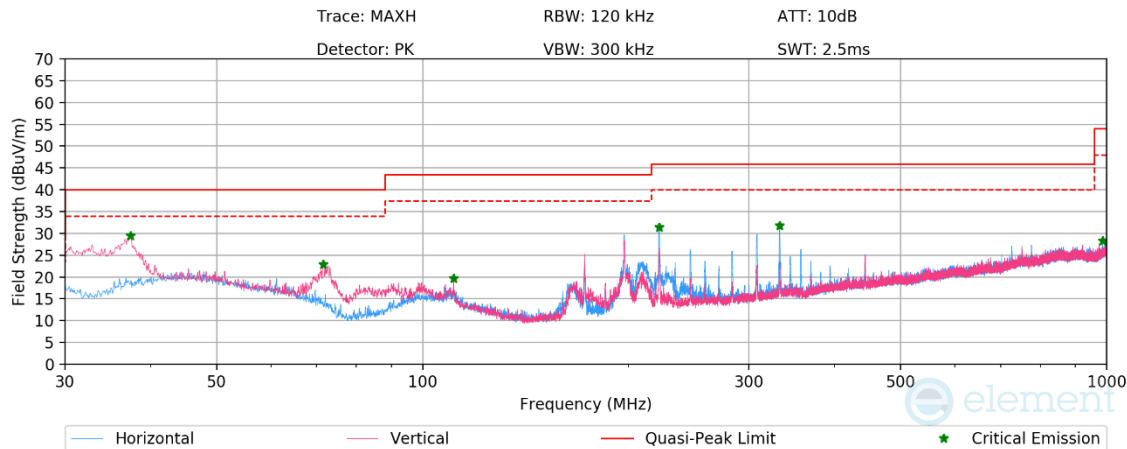
Plot 7-34. Radiated Spurious Emissions Below 1GHz (1Mbps – Ch.17, Pol. H & V, with AC/DC Adapter)
