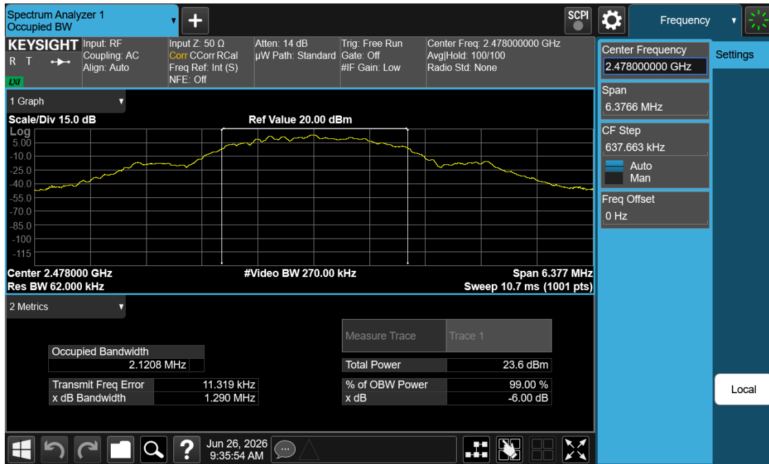
Plot 7-6. 99% OBW Plot (Bluetooth (LE), 2Mbps– Ch. 36)
