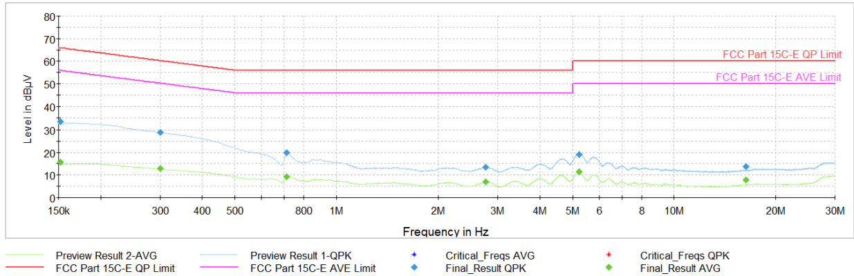
Plot 7-36. AC Line Conducted Plot with Bluetooth LE (N, 1Mbps – Ch.17, with AC/DC Adapter)
