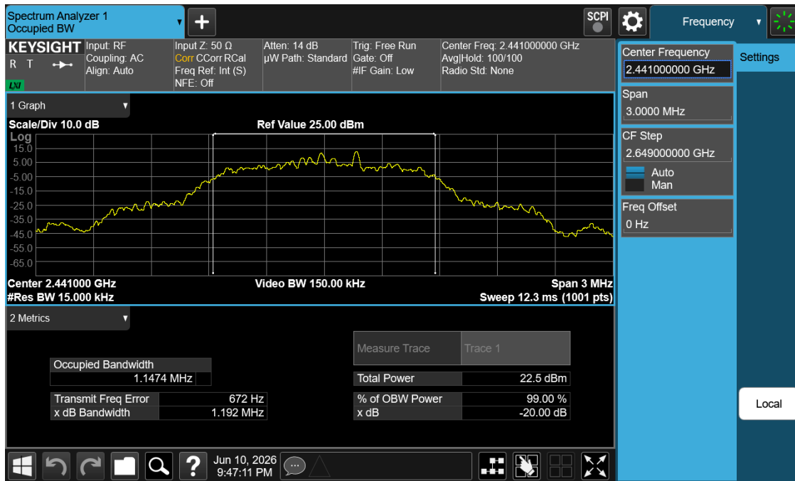
Plot 7-2. 20dB BW and 99% OBW Plot (Bluetooth, 8DPSK, – Ch. 39)
