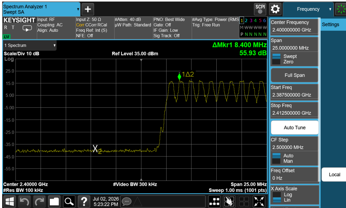
Plot 7-5. Band Edge Plot (Bluetooth with Hopping Enabled, GFSK)
