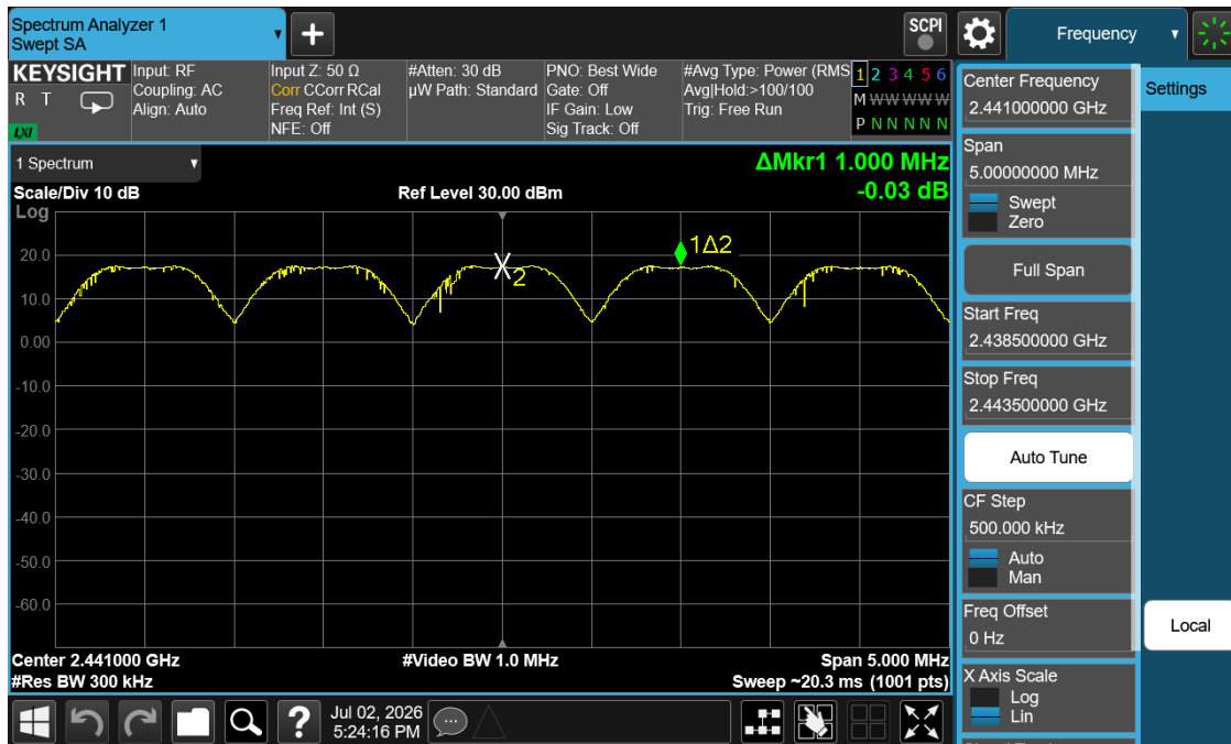
Plot 7-11. Channel Spacing Plot (Bluetooth, GFSK,)
