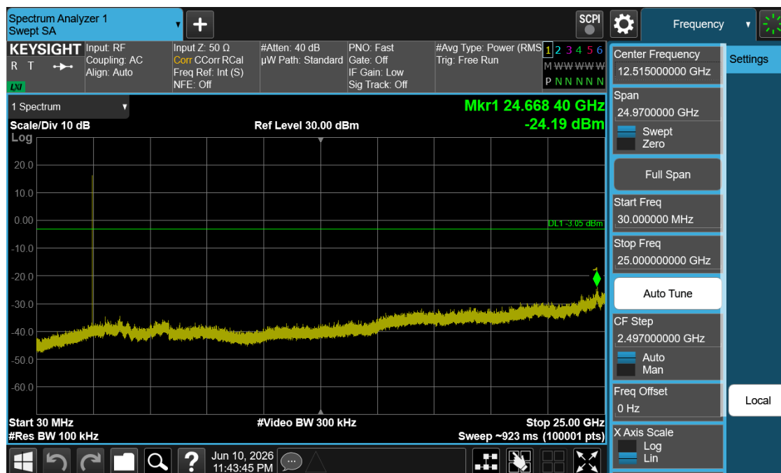
Plot 7-21. Conducted Spurious Plot (Bluetooth, GFSK, – Ch. 78)
