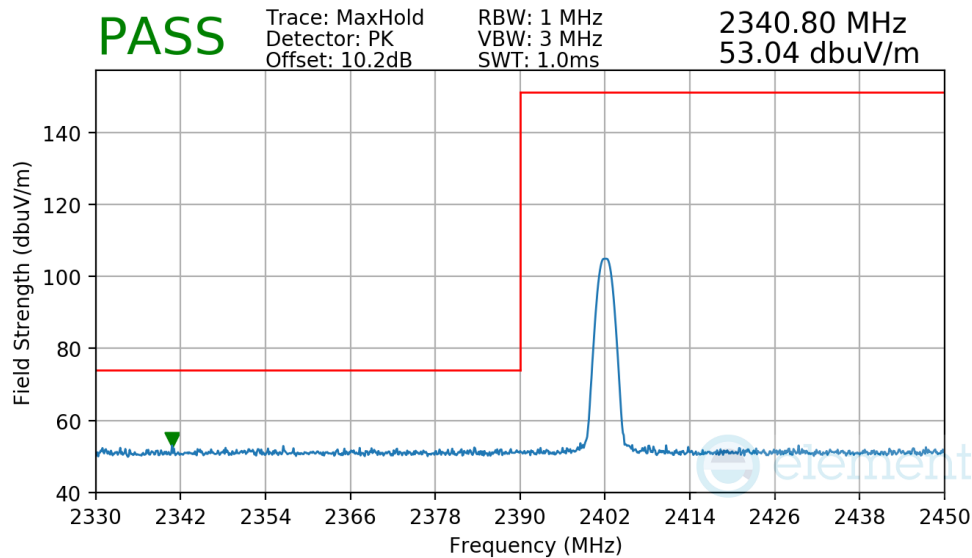
Plot 7-26. Radiated Restricted Lower Band Edge Measurement
