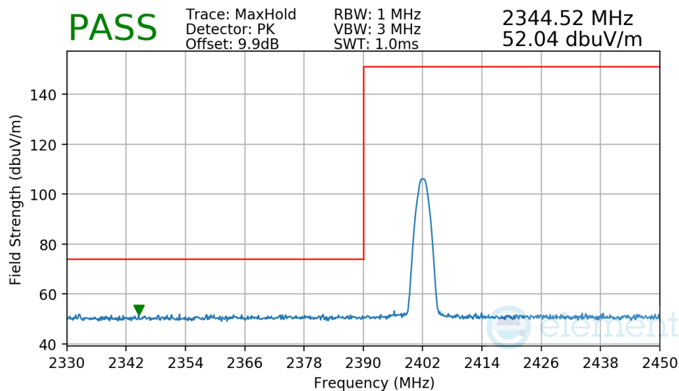
Plot 7-27. Radiated Restricted Lower Band Edge Measurement
