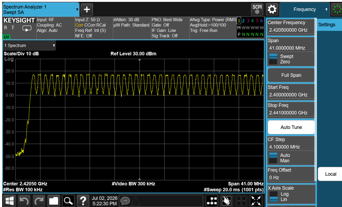
Plot 7-15. Low End Spectrum Channel Hopping Plot (Bluetooth, GFSK,)
