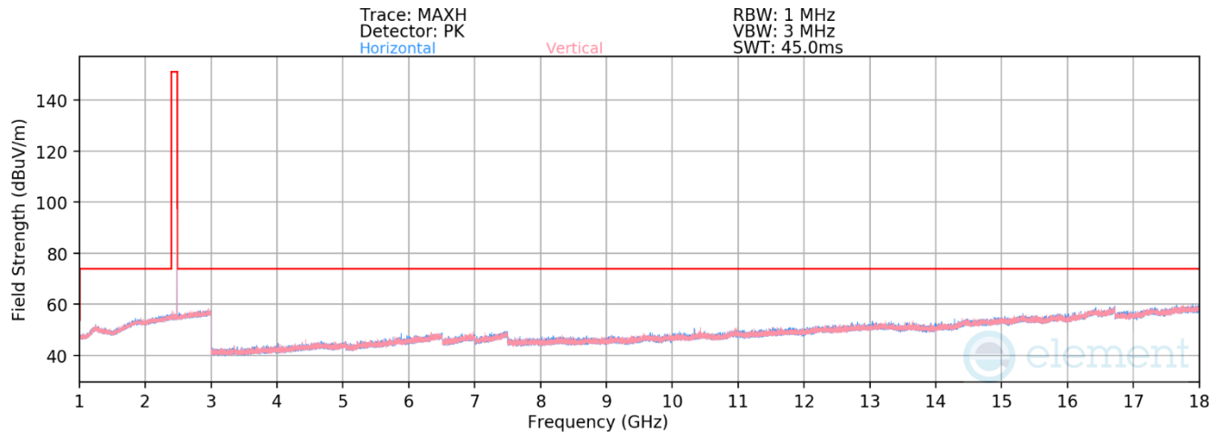
Plot 7-25. Radiated Spurious Emissions above 1GHz (BT GFSK – Ch. 78)
