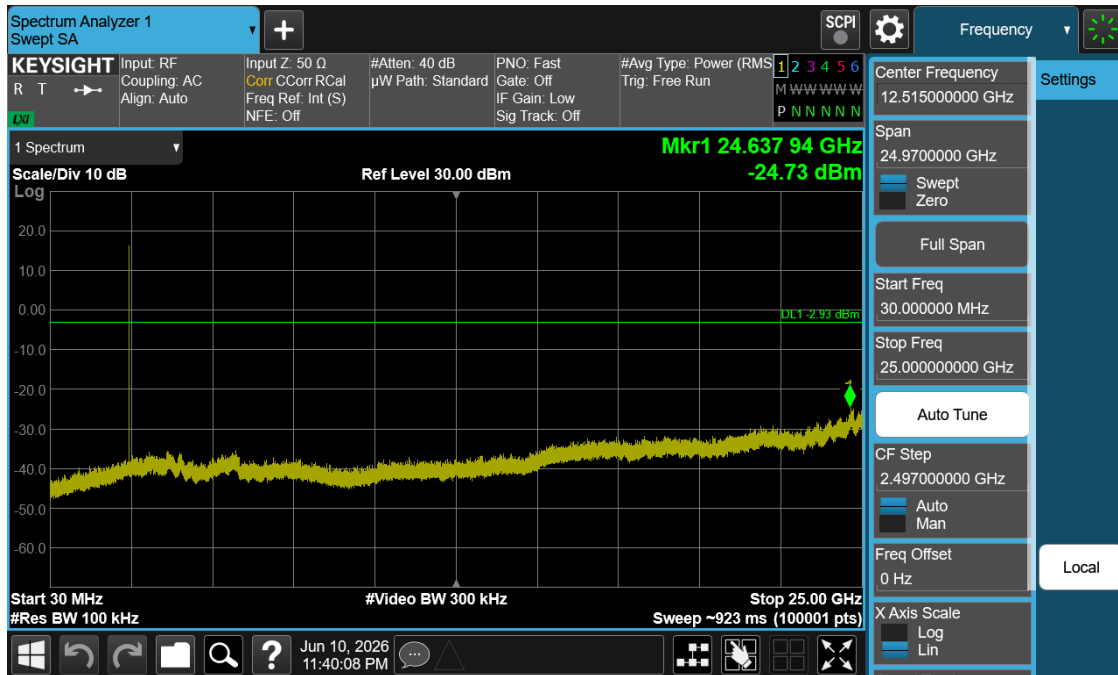
Plot 7-20. Conducted Spurious Plot (Bluetooth, GFSK, – Ch. 39)
