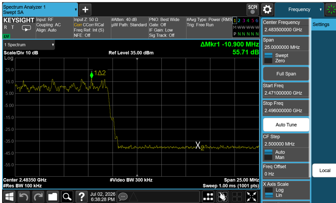
Plot 7-10. Band Edge Plot (Bluetooth with Hopping Enabled, 8DPSK)
