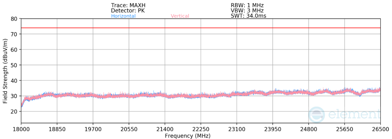
Plot 7-23. Radiated Spurious Emissions above 18GHz (BT GFSK – Ch. 0)
