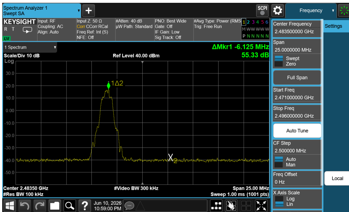
Plot 7-8. Band Edge Plot (Bluetooth with Hopping Disabled, 8DPSK – Ch. 78)
