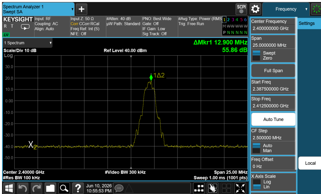
Plot 7-7. Band Edge Plot (Bluetooth with Hopping Disabled, 8DPSK – Ch. 0)
