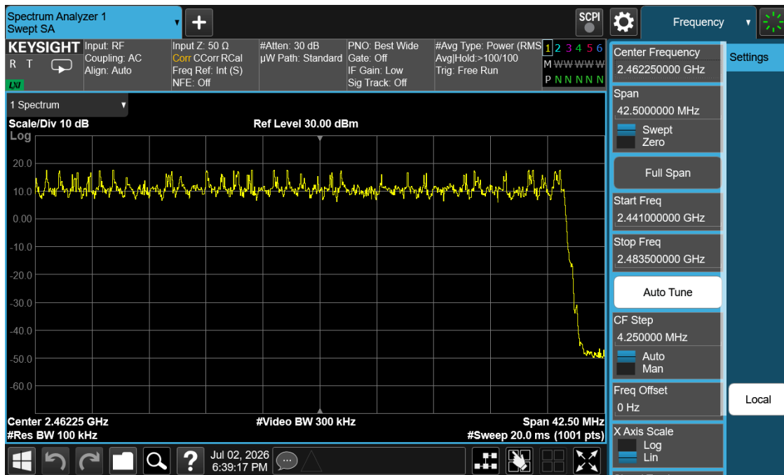
Plot 7-18. High End Spectrum Channel Hopping Plot (Bluetooth, 8DPSK,)
