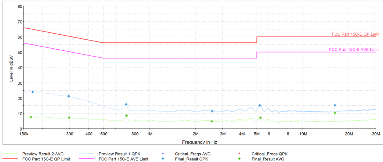
Plot 7-31. AC Line-Conducted Test Plot (L1, GFSK – Ch.0, with AC/DC Adapter)
