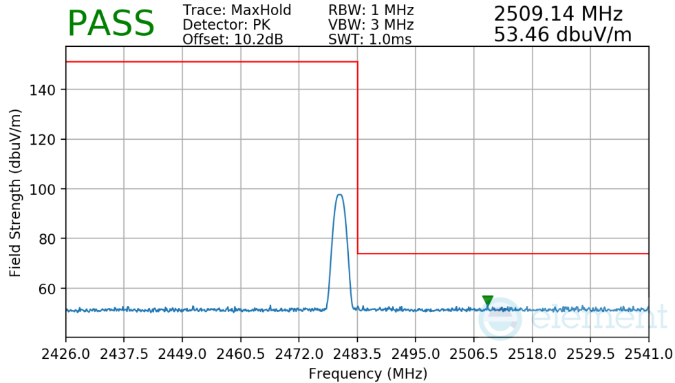
Plot 7-28. Radiated Restricted Upper Band Edge Measurement
