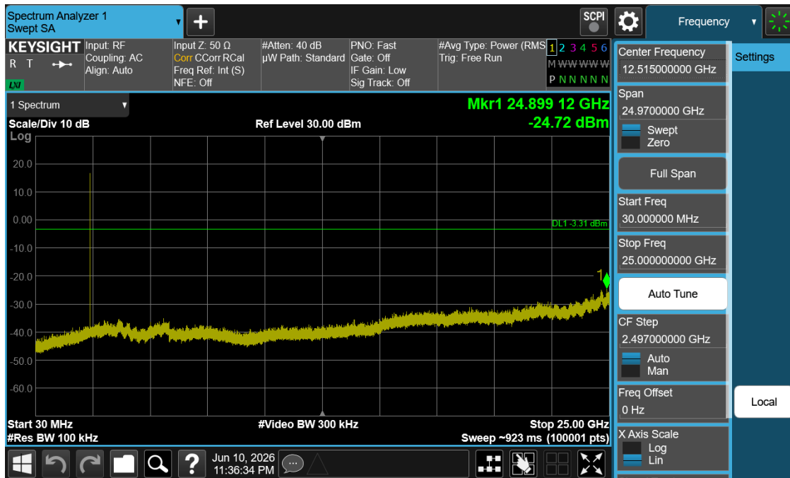
Plot 7-19. Conducted Spurious Plot (Bluetooth, GFSK, – Ch. 0)
