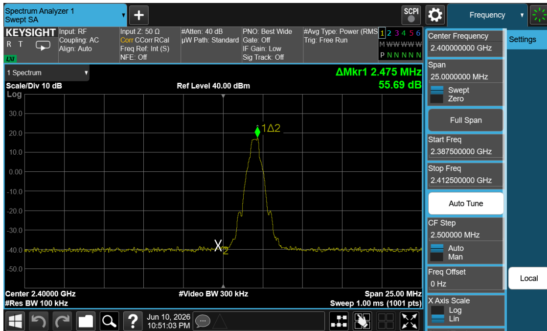
Plot 7-3. Band Edge Plot (Bluetooth with Hopping Disabled, GFSK – Ch. 0)
