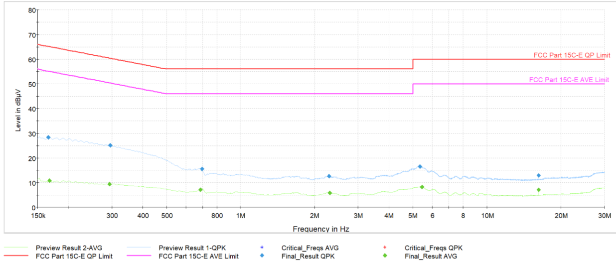
Plot 7-32. AC Line-Conducted Test Plot (N, GFSK – Ch.0, with AC/DC Adapter)
