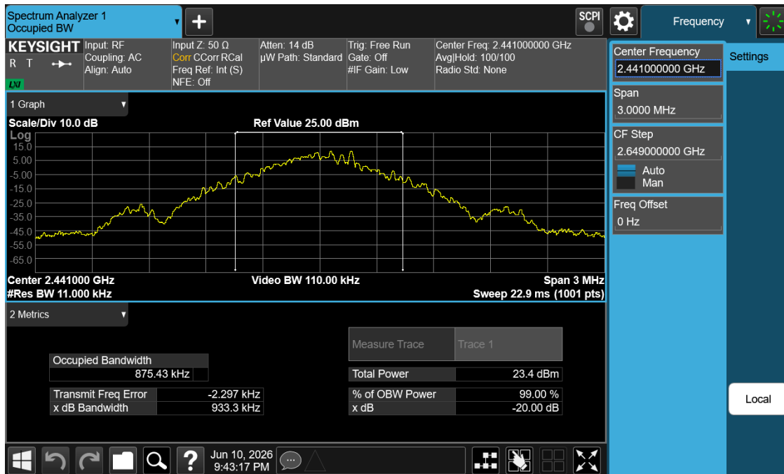
Plot 7-1. 20dB BW and 99% OBW Plot (Bluetooth, GFSK – Ch. 39)
