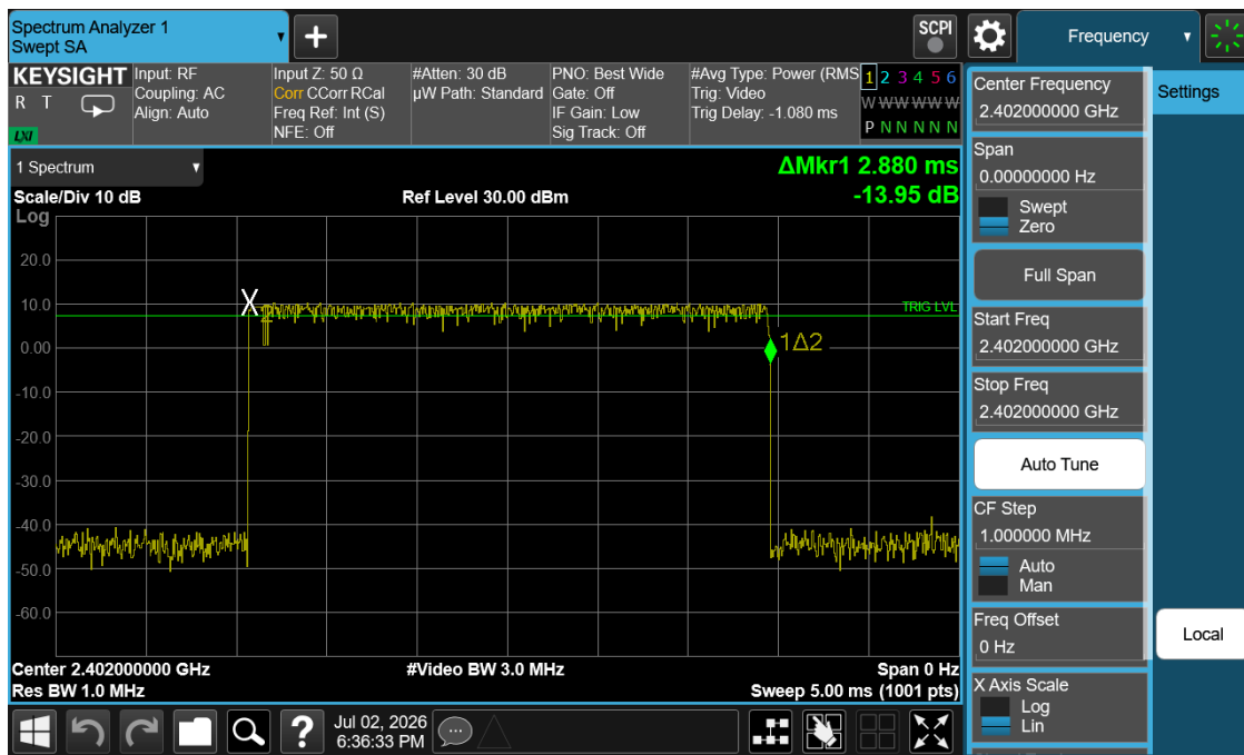
Plot 7-14. Time of Occupancy Plot (Bluetooth, 8DPSK,)
