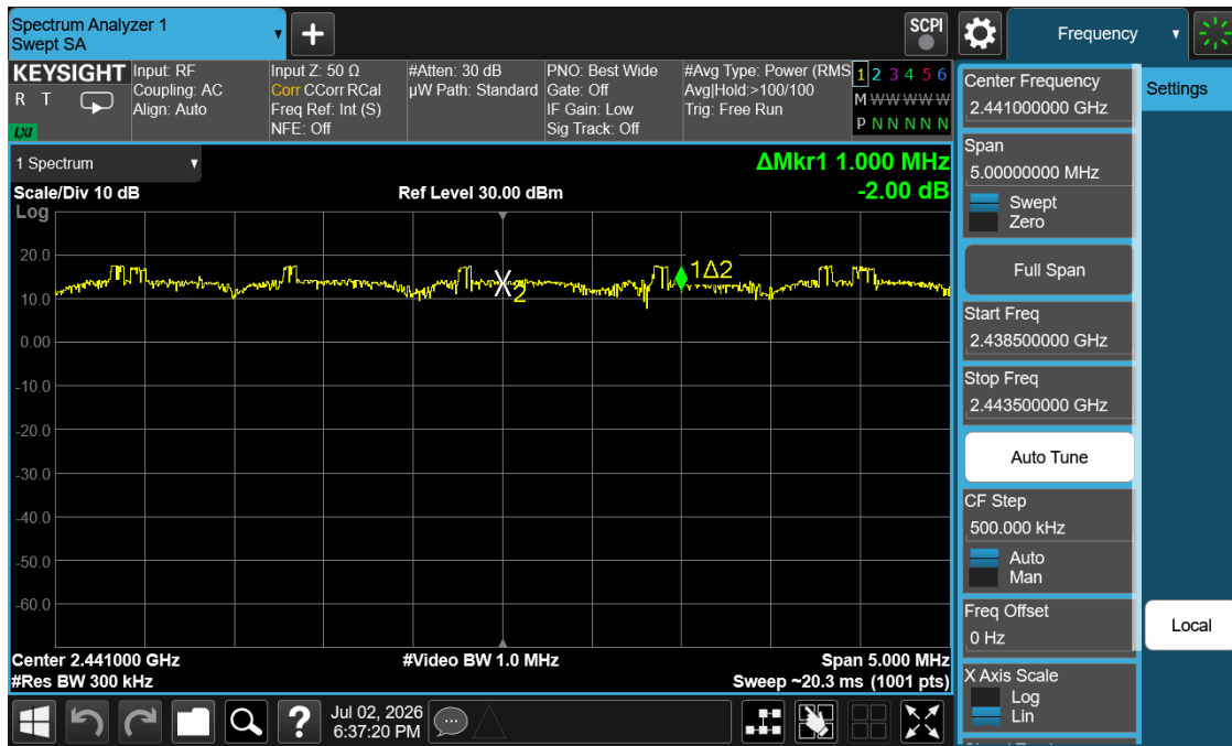
Plot 7-12. Channel Spacing Plot (Bluetooth, 8DPSK,)
