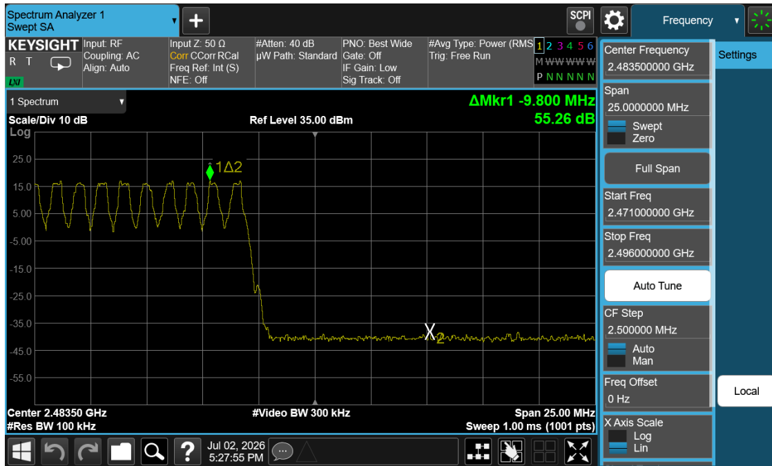
Plot 7-6. Band Edge Plot (Bluetooth with Hopping Enabled, GFSK)
