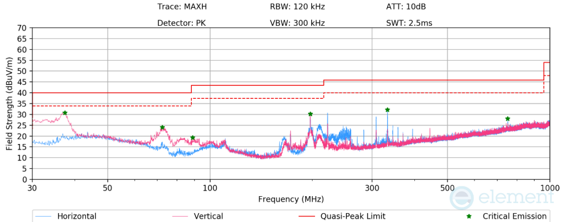
Plot 7-30. Radiated Spurious Emissions Below 1GHz (GFSK – Ch.0, with AC/DC Adapter)
