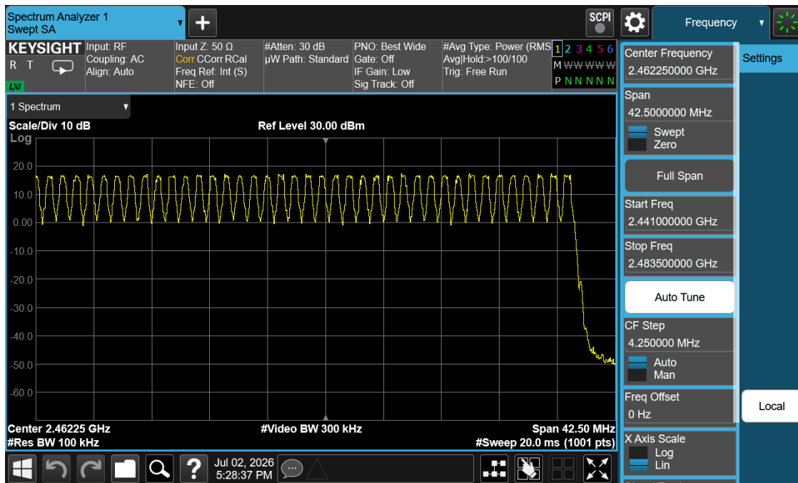
Plot 7-16. High End Spectrum Channel Hopping Plot (Bluetooth, GFSK,)
