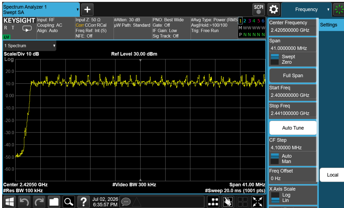
Plot 7-17. Low End Spectrum Channel Hopping Plot (Bluetooth, 8DPSK,)
