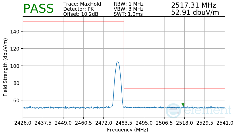
Plot 7-29. Radiated Restricted Upper Band Edge Measurement
