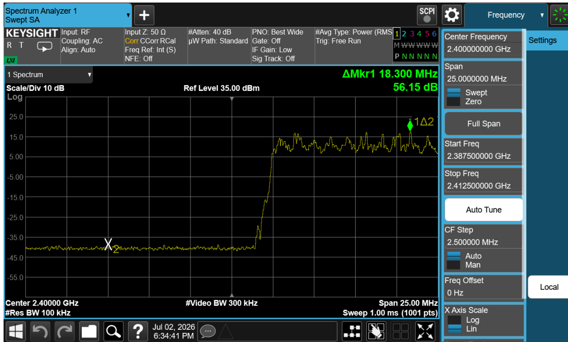
Plot 7-9. Band Edge Plot (Bluetooth with Hopping Enabled, 8DPSK)
