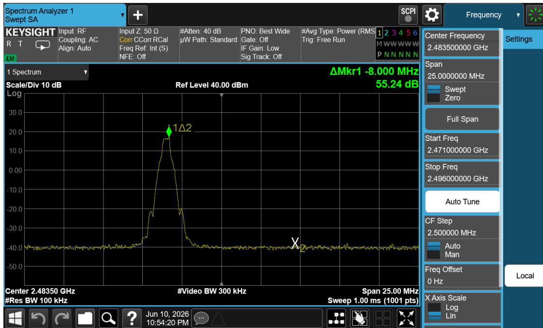
Plot 7-4. Band Edge Plot (Bluetooth with Hopping Disabled, GFSK – Ch. 78)
