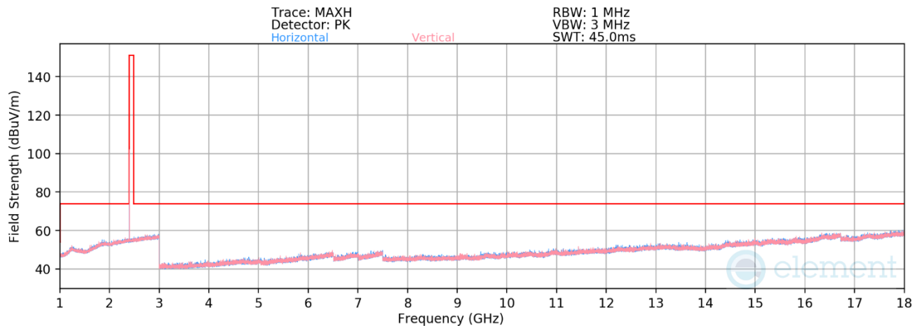
Plot 7-22. Radiated Spurious Emissions above 1GHz (BT GFSK – Ch. 0)
