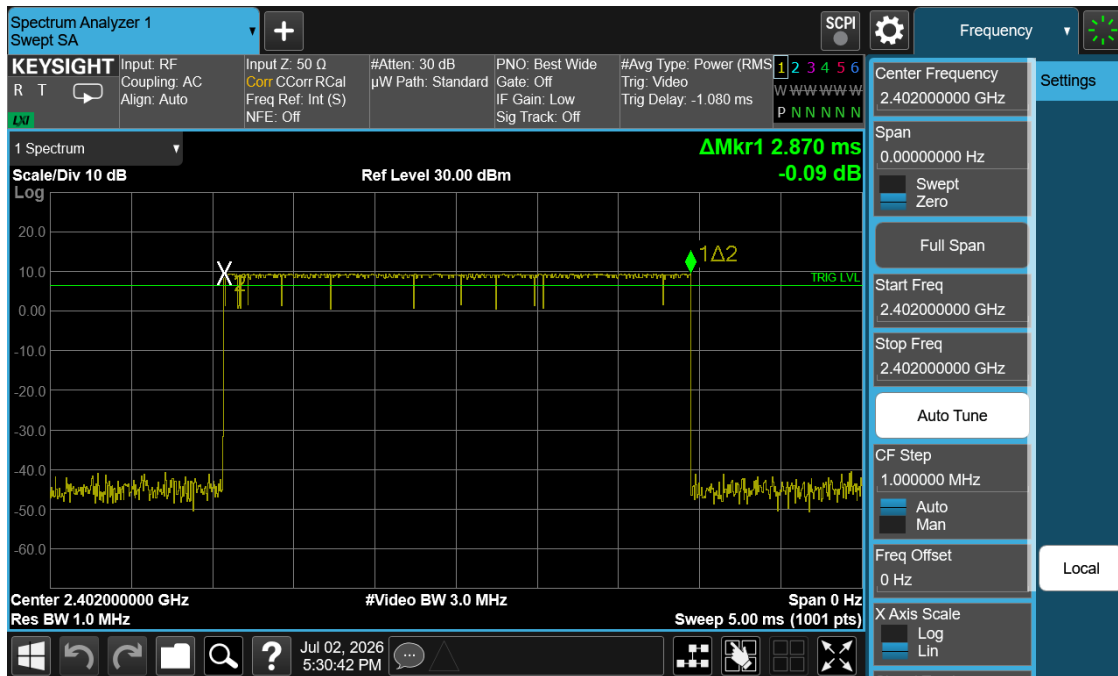
Plot 7-13. Time of Occupancy Plot (Bluetooth, GFSK,)
