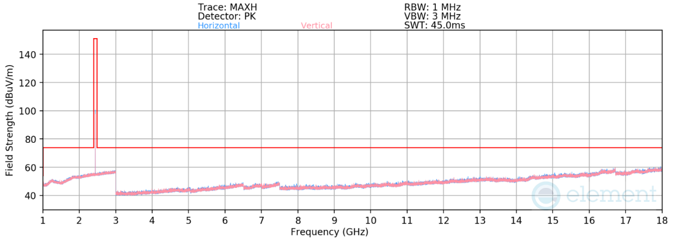
Plot 7-24. Radiated Spurious Emissions above 1GHz (BT GFSK – Ch. 39)
