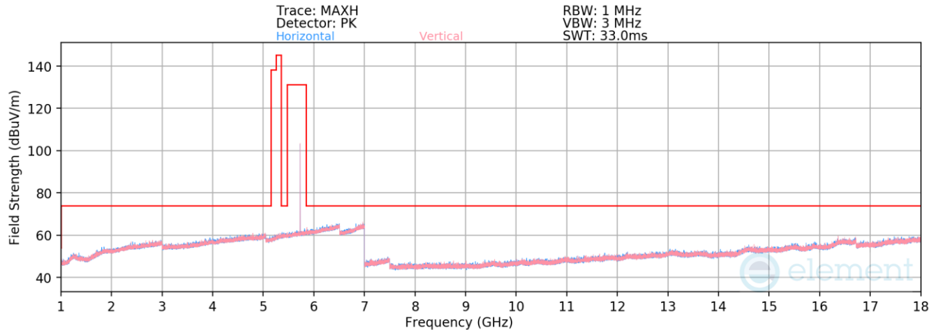
Plot 7-48. Radiated Spurious Emissions 1-18GHz (NB UNII HDR4 – 5731MHz)
