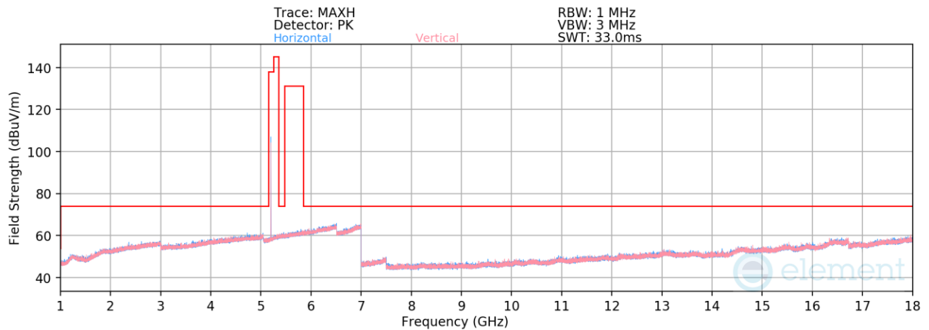
Plot 7-45. Radiated Spurious Emissions 1-18GHz (NB UNII HDR4 – 5200MHz)
