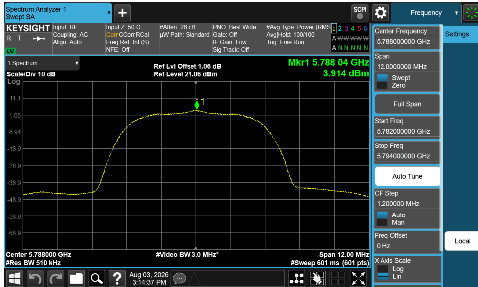
Plot 7-33. PSD (NB UNII HDR8 – 5788MHz)
