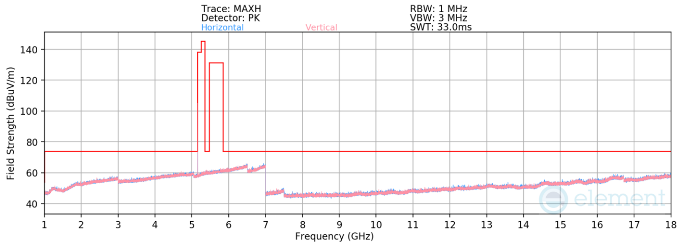
Plot 7-36. Radiated Spurious Emissions 1-18GHz (NB UNII BDR – 5157MHz)
