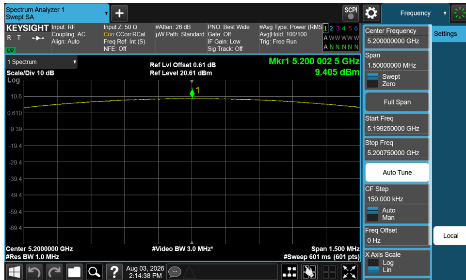
Plot 7-23. PSD (NB UNII LE1M – 5200MHz)
