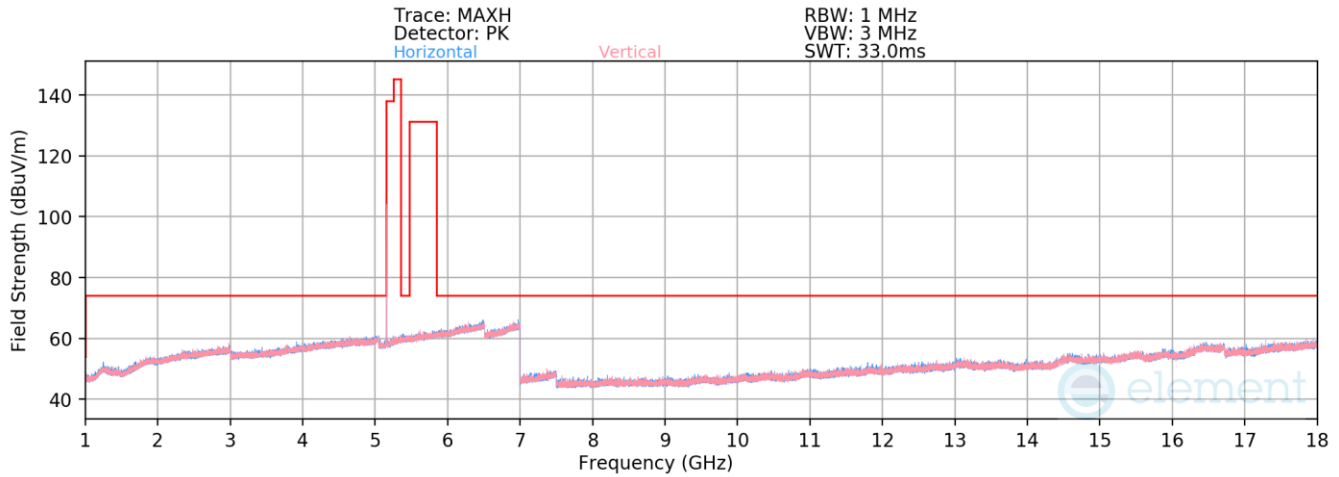
Plot 7-44. Radiated Spurious Emissions 1-18GHz (NB UNII HDR4 – 5157MHz)
