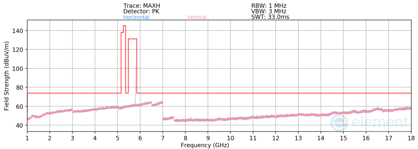
Plot 7-49. Radiated Spurious Emissions 1-18GHz (NB UNII HDR4 – 5788MHz)
