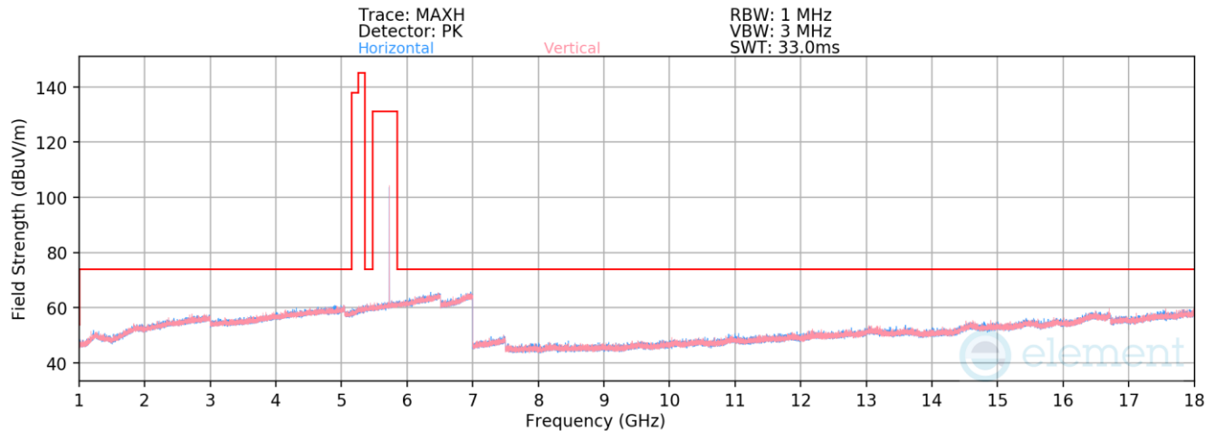
Plot 7-40. Radiated Spurious Emissions 1-18GHz (NB UNII BDR – 5731MHz)
