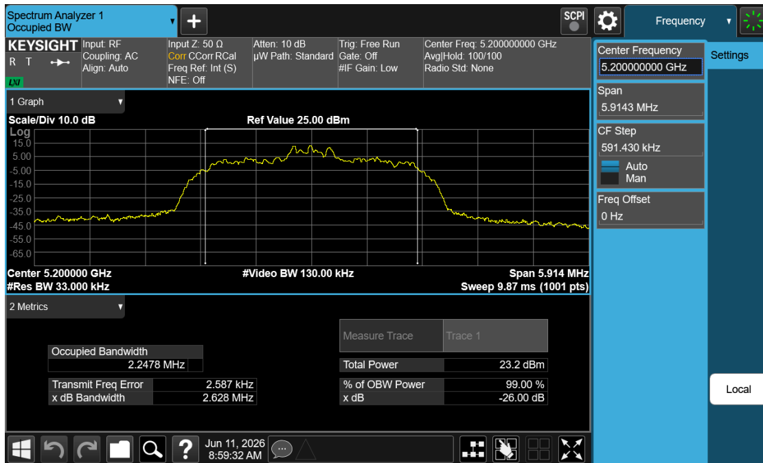
Plot 7-4. 26dB BW & 99% OBW (NB UNII HDR4 – 5200MHz)
