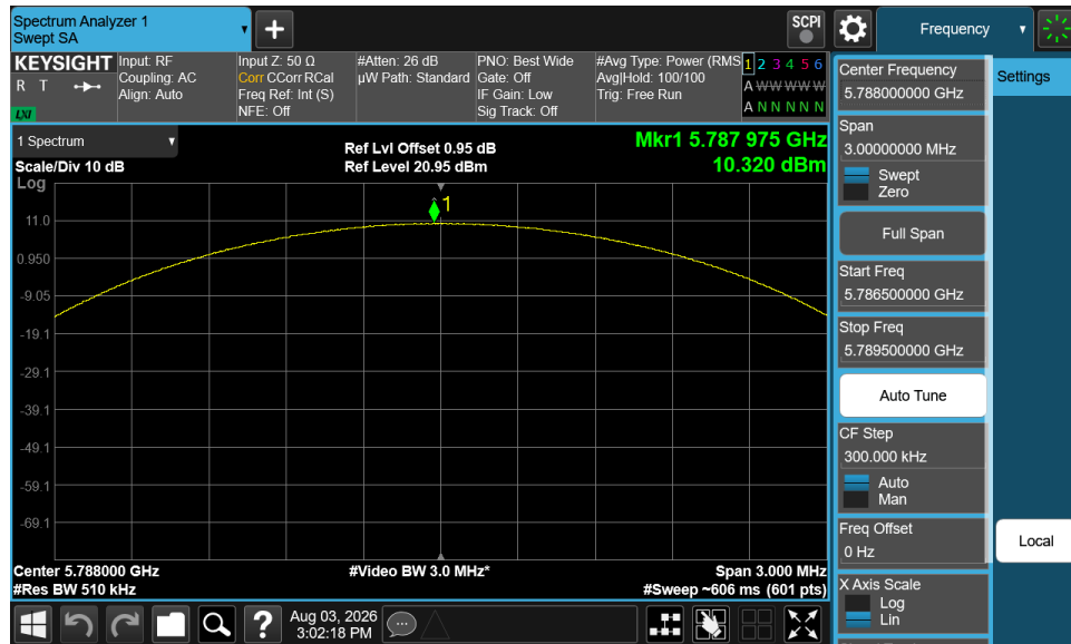
Plot 7-31. PSD (NB UNII LE2M – 5788MHz)
