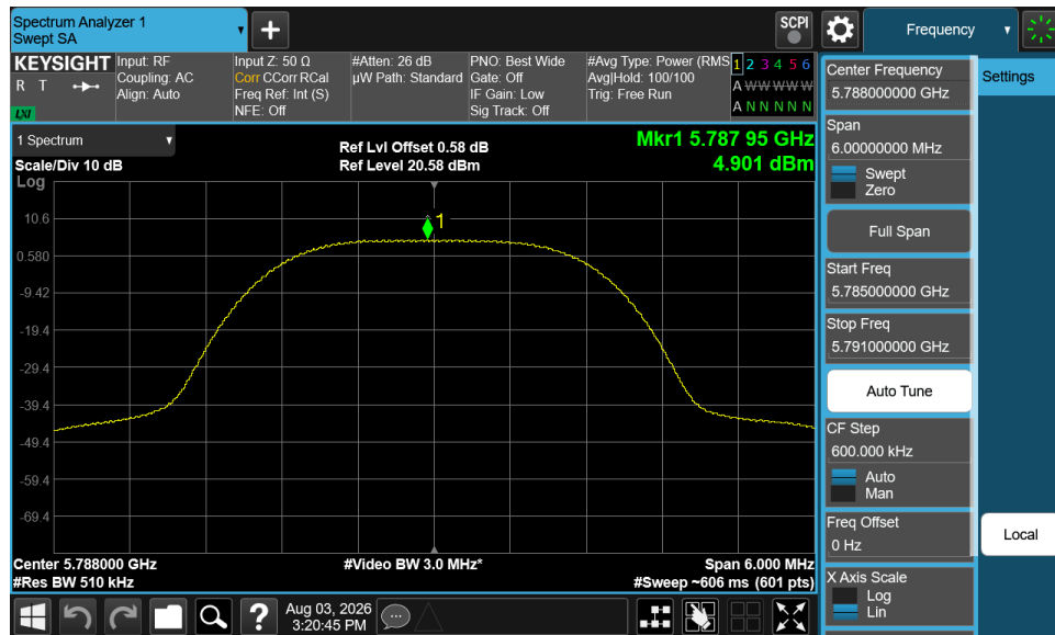
Plot 7-34. PSD (NB UNII HDRp4 – 5788MHz)
