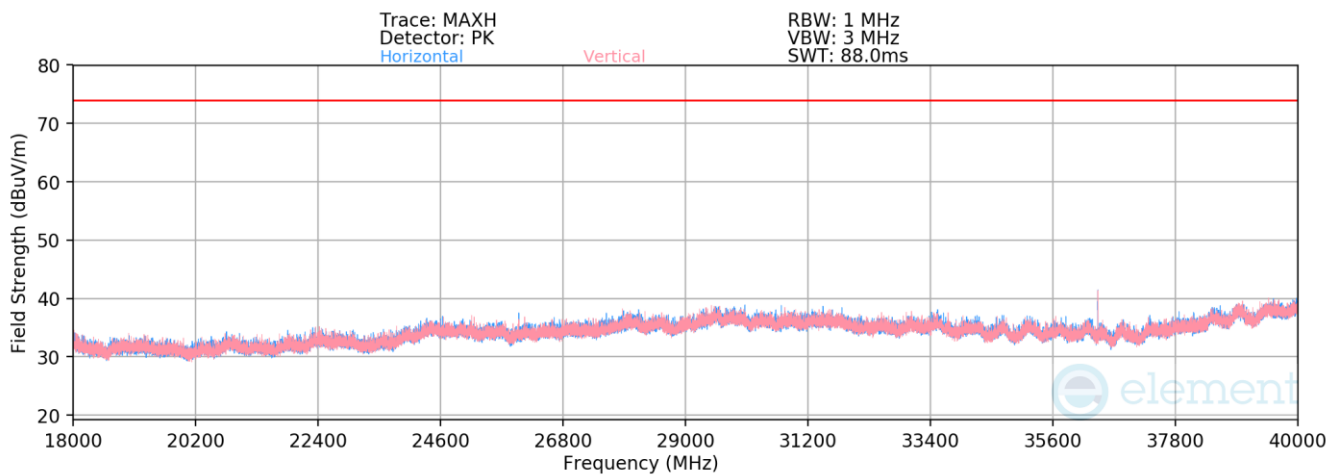
Plot 7-38. Radiated Spurious Emissions Above 18GHz (NB UNII BDR – 5200MHz)
