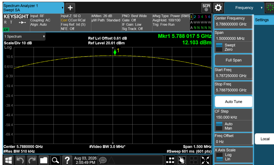
Plot 7-30. PSD (NB UNII LE1M – 5788MHz)
