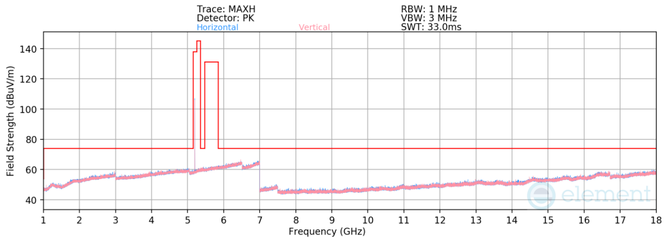
Plot 7-37. Radiated Spurious Emissions 1-18GHz (NB UNII BDR – 5200MHz)
