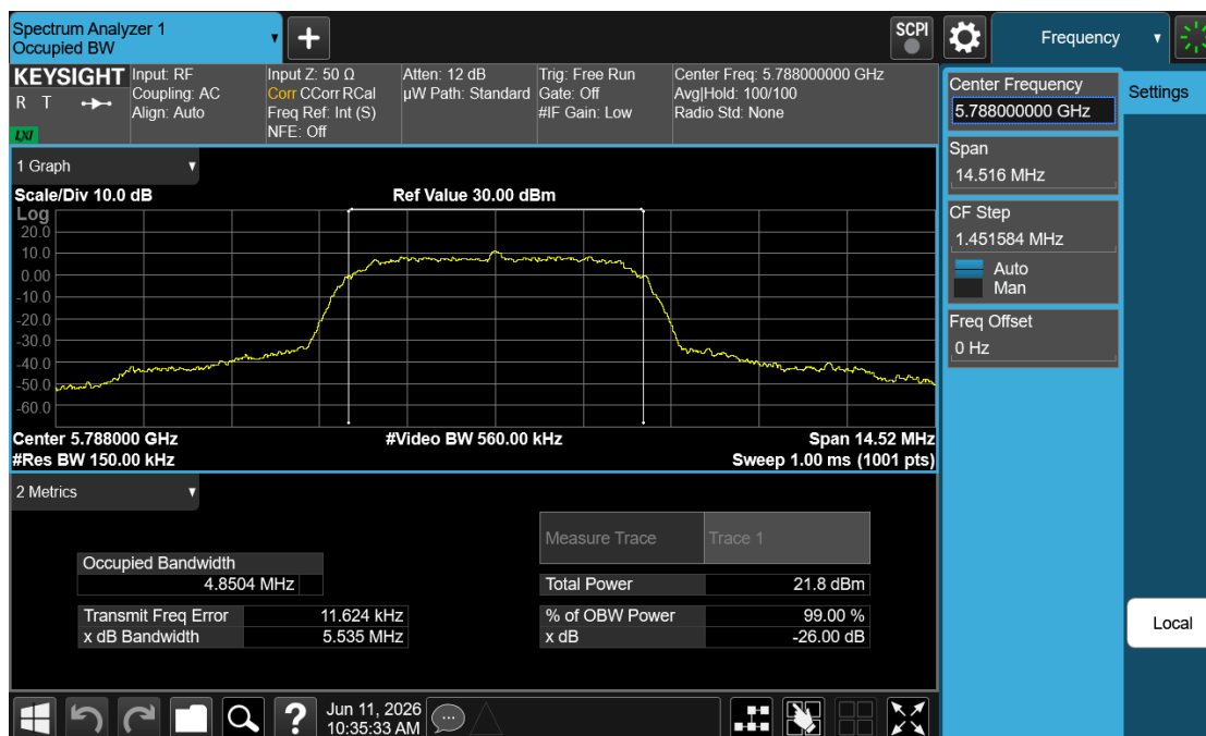
Plot 7-14. 99% OBW (NB UNII HDRp8 – 5788MHz)
