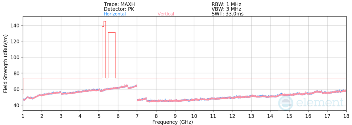
Plot 7-42. Radiated Spurious Emissions 1-18GHz (NB UNII BDR – 5844MHz)
