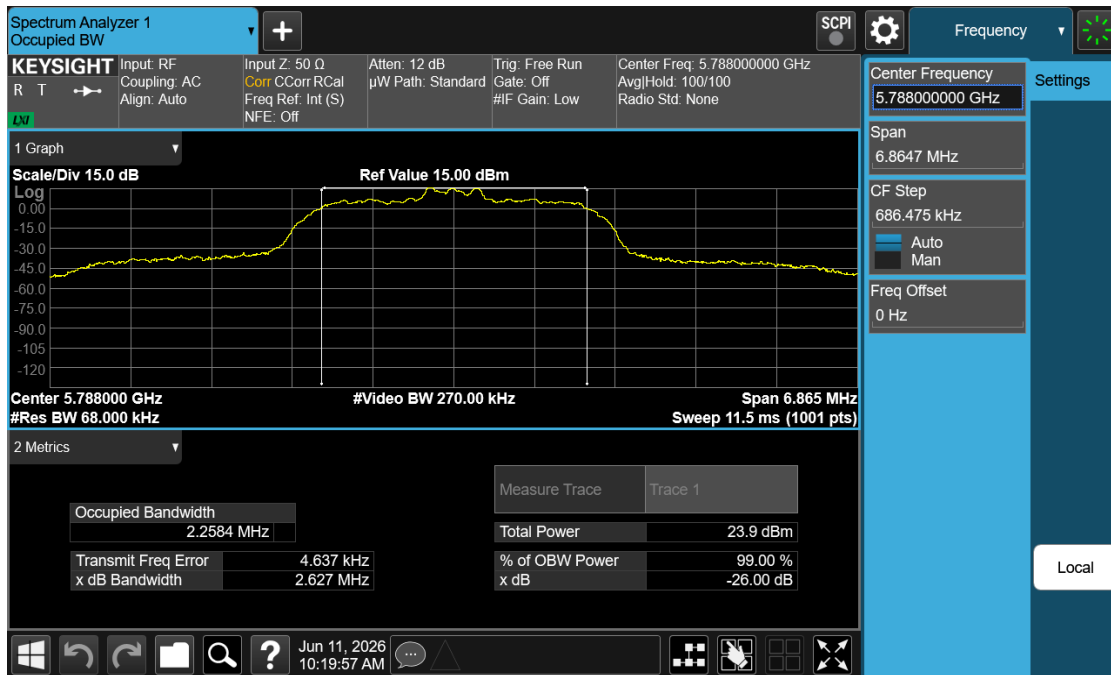
Plot 7-11. 99% OBW (NB UNII HDR4 – 5788MHz)
