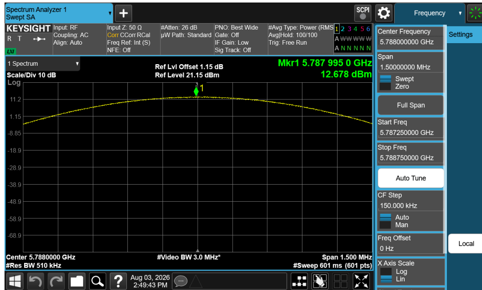
Plot 7-29. PSD (NB UNII BDR – 5788MHz)
