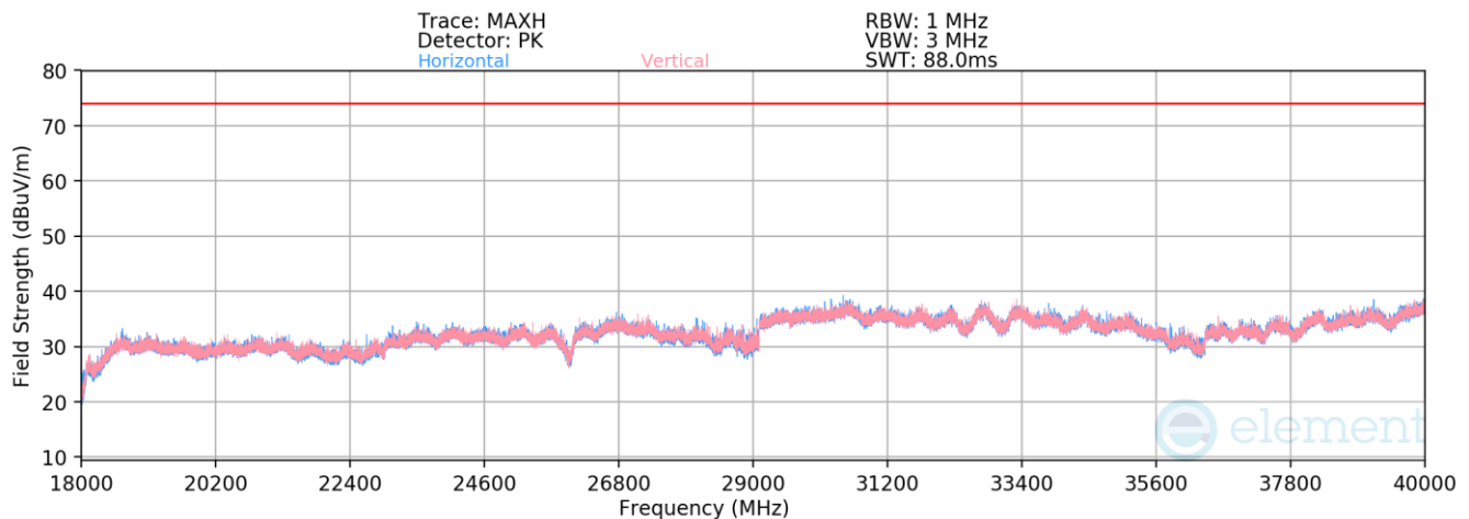
Plot 7-51. Radiated Spurious Emissions Above 18GHz (NB UNII HDR4 – 5844MHz)
