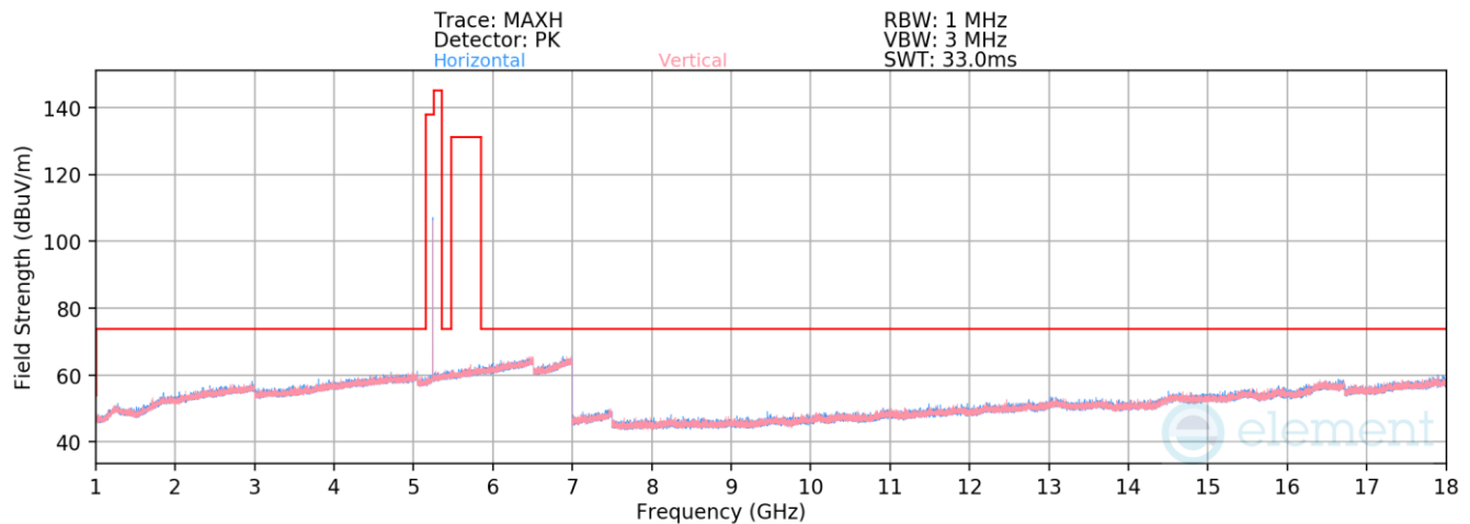
Plot 7-39. Radiated Spurious Emissions 1-18GHz (NB UNII BDR – 5245MHz)
