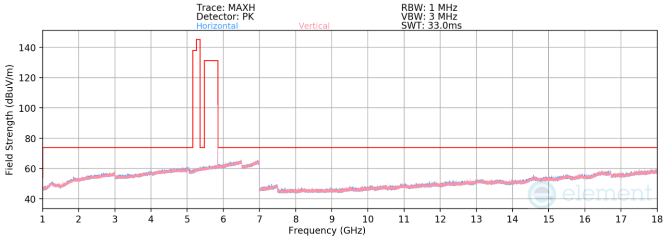
Plot 7-50. Radiated Spurious Emissions 1-18GHz (NB UNII HDR4 – 5844MHz)
