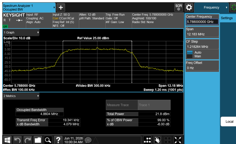
Plot 7-21. 6dB BW & 99% OBW (NB UNII HDRp8 – 5788MHz)
