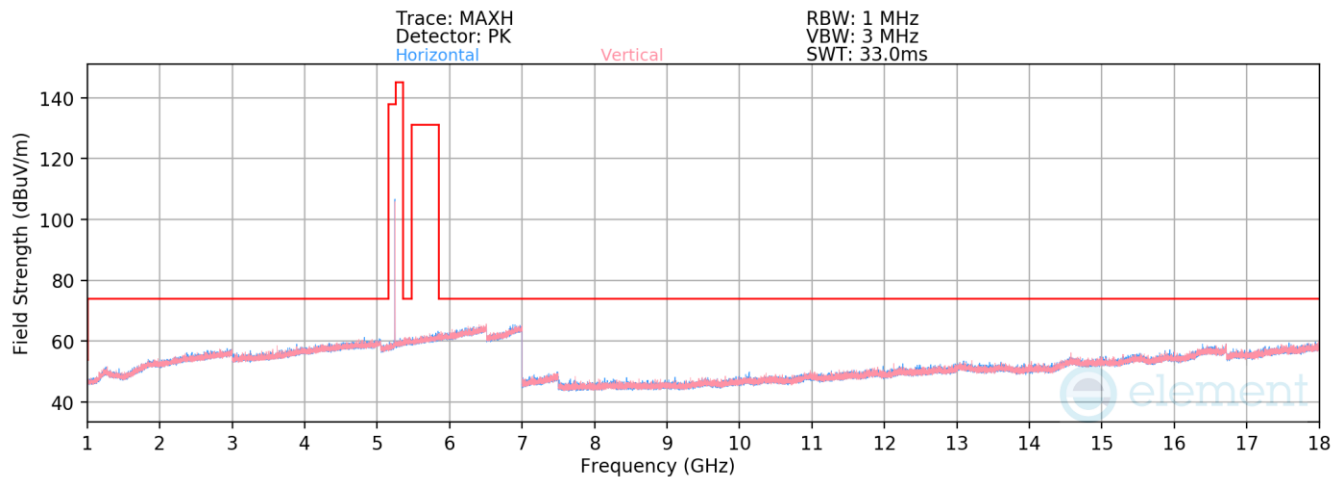
Plot 7-47. Radiated Spurious Emissions 1-18GHz (NB UNII HDR4 – 5245MHz)
