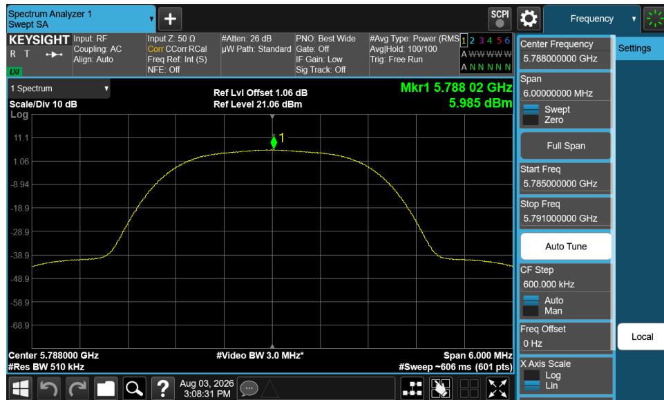
Plot 7-32. PSD (NB UNII HDR4 – 5788MHz)
