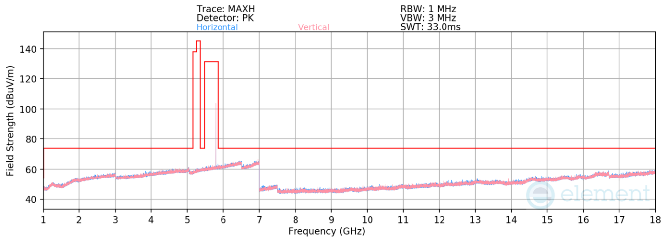
Plot 7-41. Radiated Spurious Emissions 1-18GHz (NB UNII BDR – 5788MHz)
