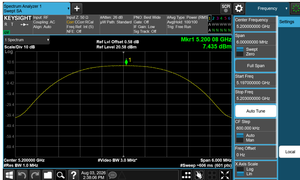
Plot 7-27. PSD (NB UNII HDRp4 – 5200MHz)
