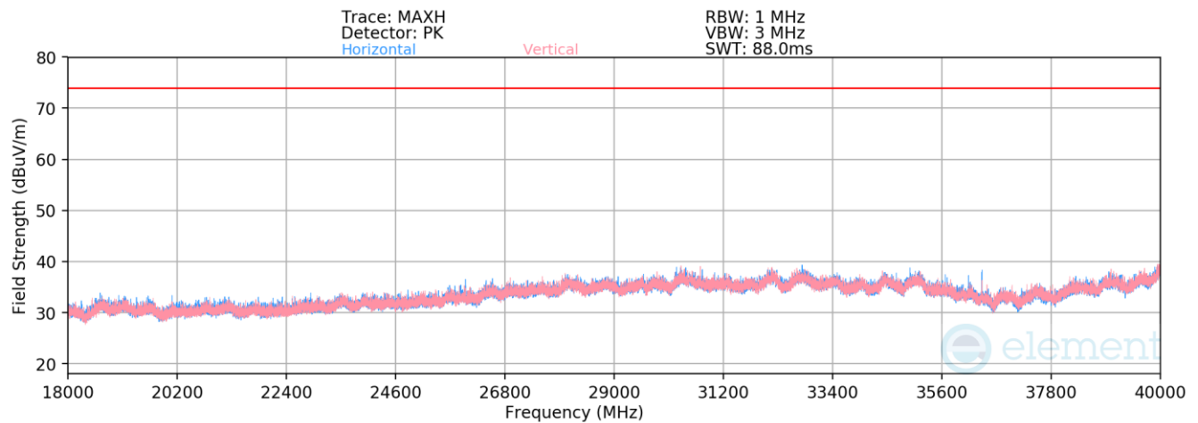
Plot 7-46. Radiated Spurious Emissions Above 18GHz (NB UNII HDR4 – 5200MHz)
