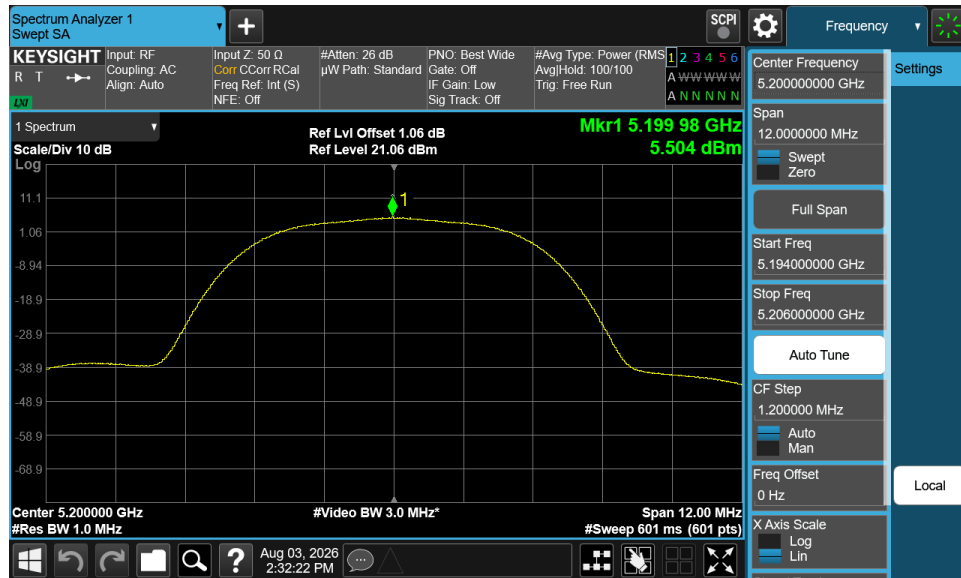
Plot 7-26. PSD (NB UNII HDR8 – 5200MHz)
