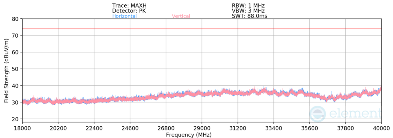
Plot 7-43. Radiated Spurious Emissions Above 18GHz (NB UNII BDR – 5844MHz)
