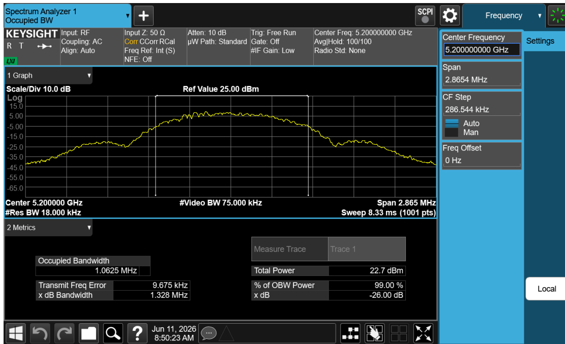
Plot 7-2. 26dB BW & 99% OBW (NB UNII LE1M – 5200MHz)
