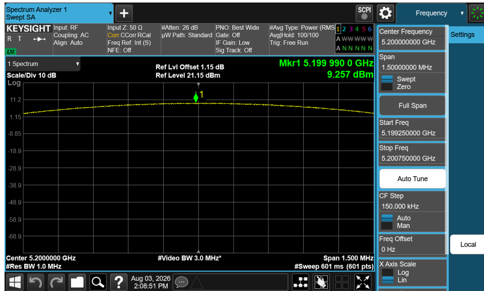
Plot 7-22. PSD (NB UNII BDR – 5200MHz)
