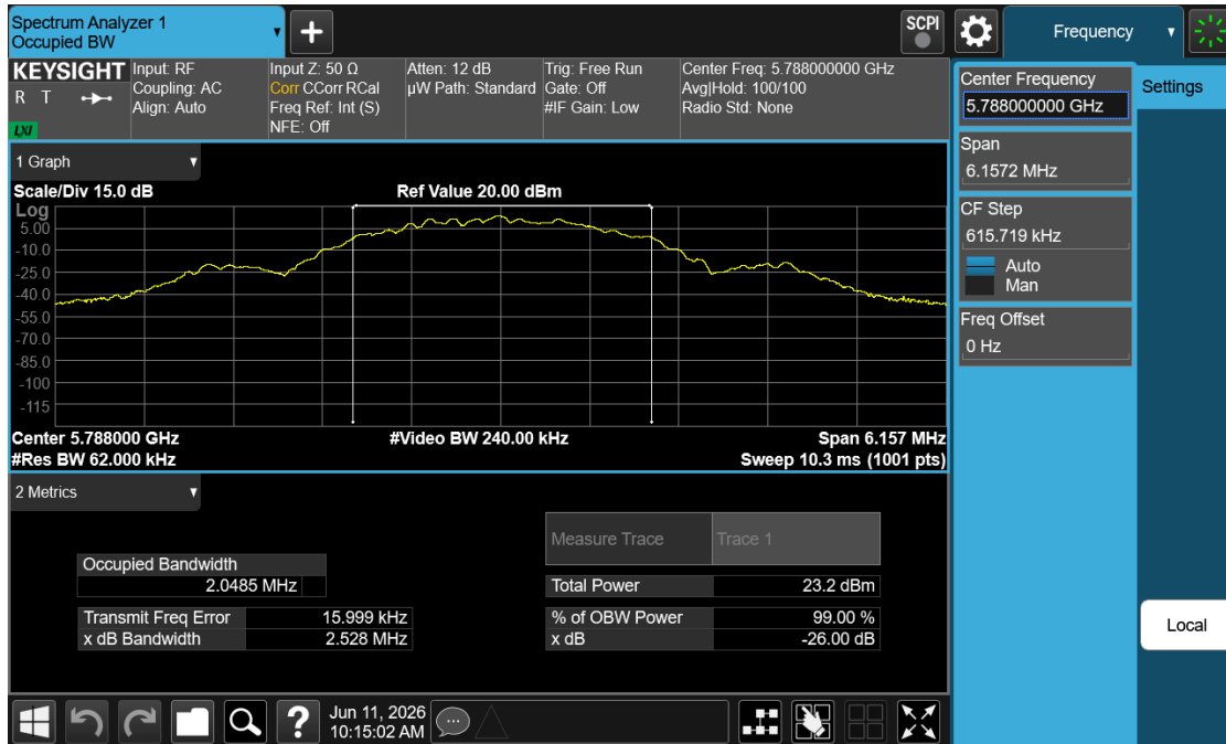
Plot 7-10. 99% OBW (NB UNII LE2M – 5788MHz)
