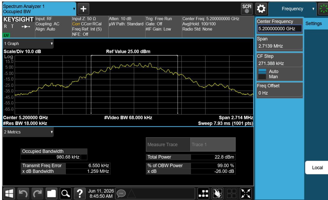
Plot 7-1. 26dB BW & 99% OBW (NB UNII BDR – 5200MHz)
