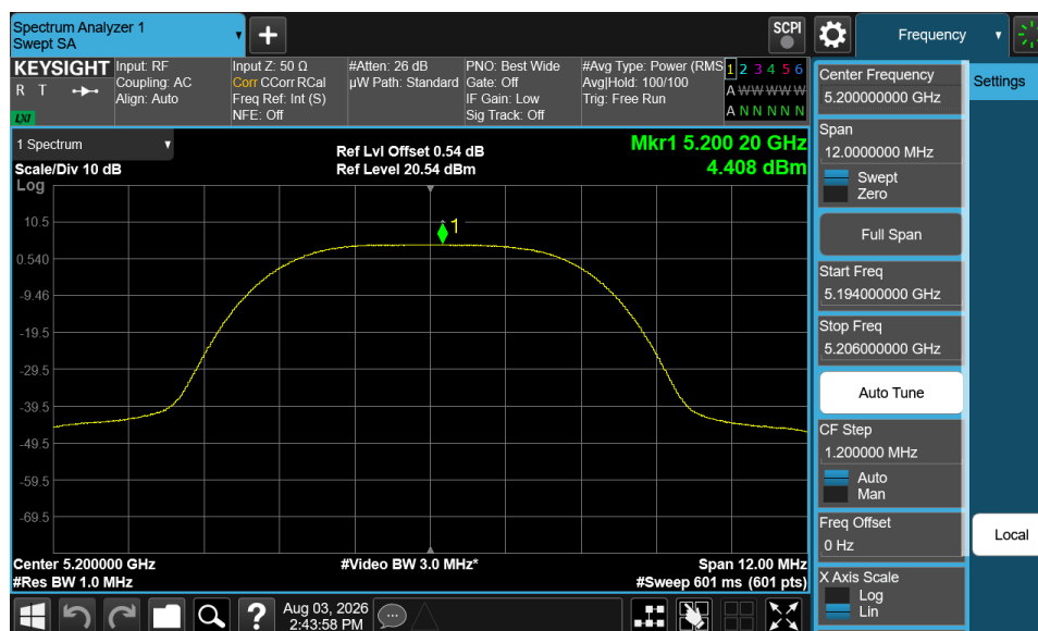
Plot 7-28. PSD (NB UNII HDRp8 - 5200MHz)
