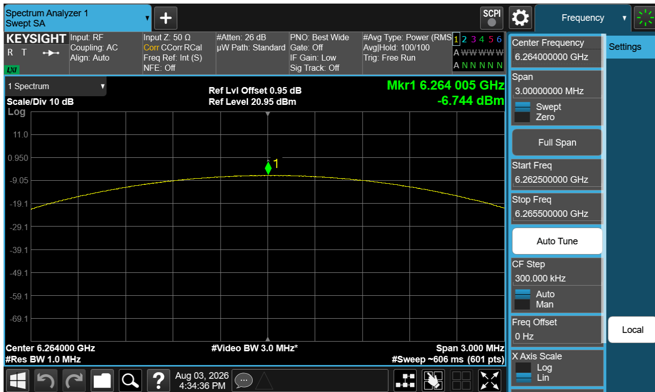
Plot 7-10. PSD (NB UNII LE2M – 6264MHz)
