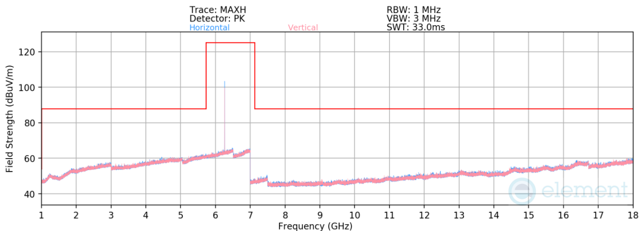
Plot 7-31. Radiated Spurious Emissions 1-18GHz (NB UNII BDR – 6264MHz)
