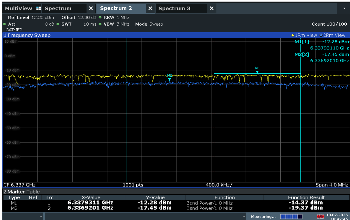
Plot 7-29. Power Density Plot – 6337MHz
