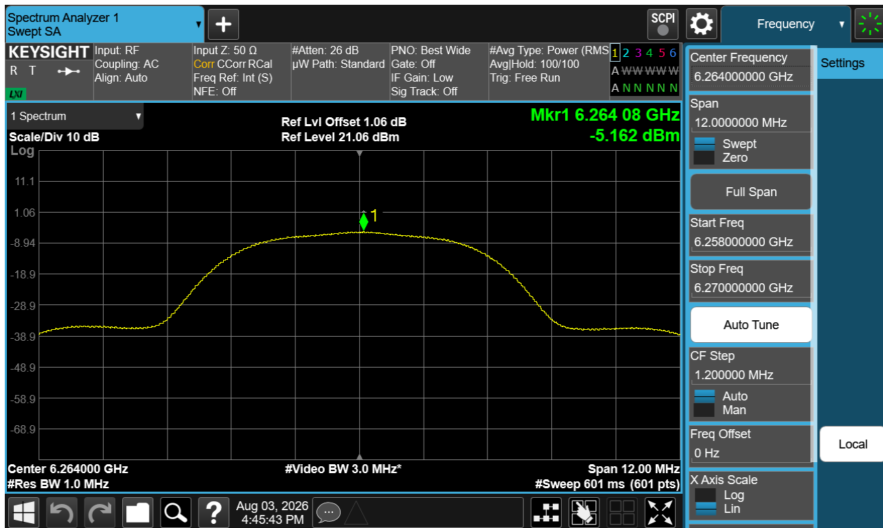
Plot 7-12. PSD (NB UNII HDR8 – 6264MHz)
