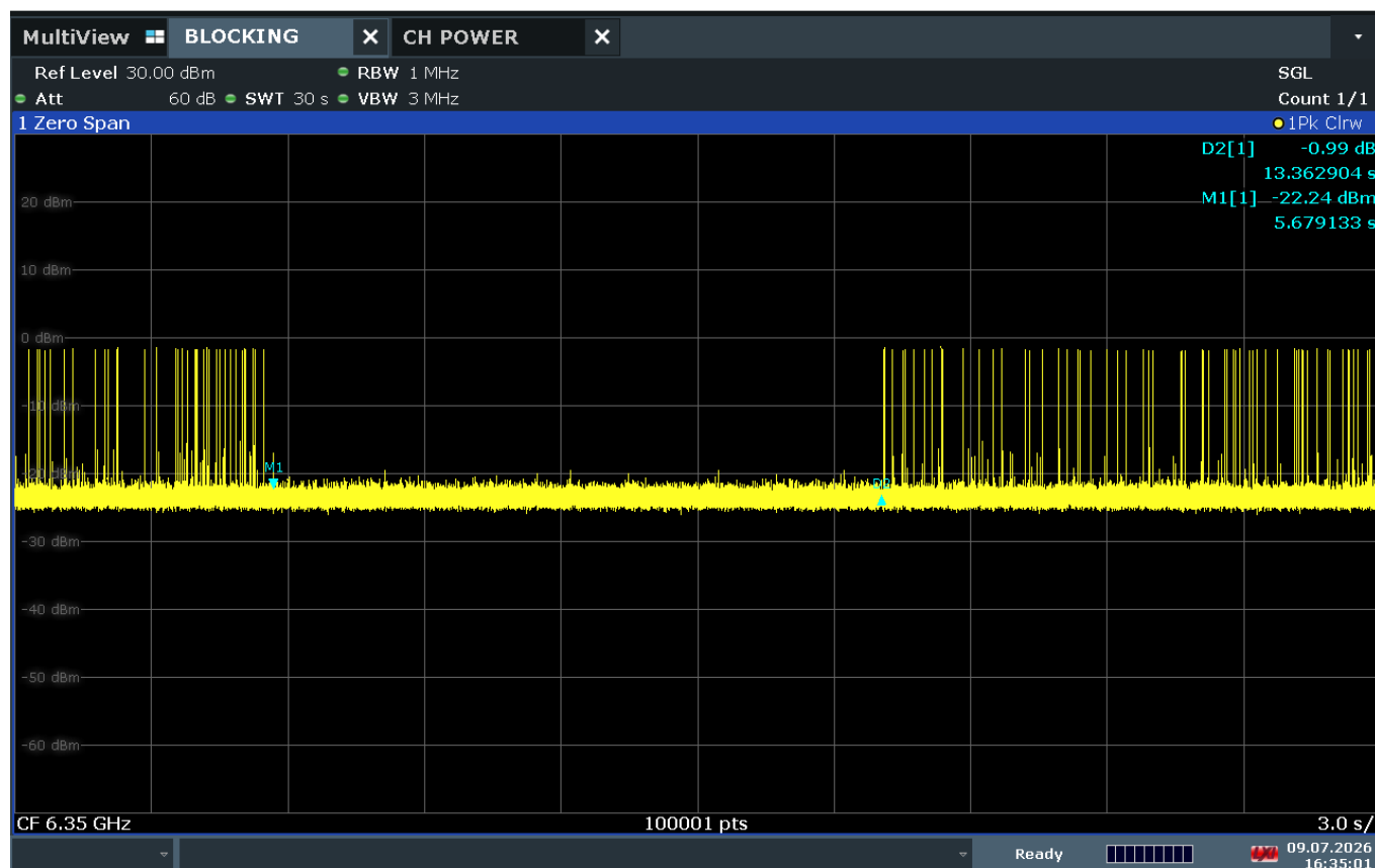
Plot 7-24. Contention Based Protocol Timing Plot
