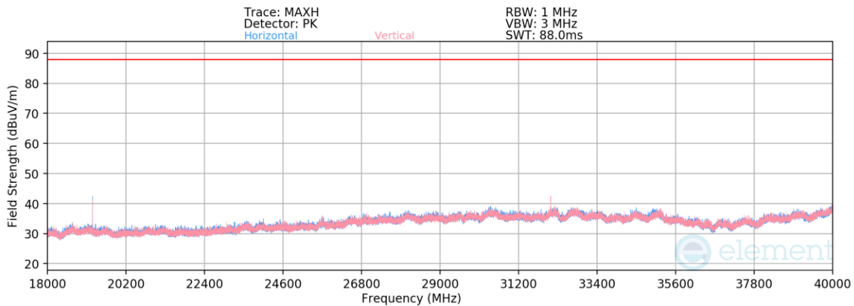
Plot 7-33. Radiated Spurious Emissions Above 18GHz (NB UNII BDR – 6420MHz)
