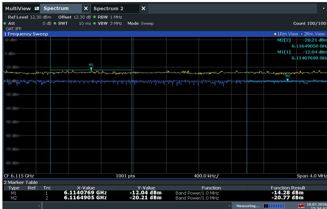
Plot 7-27. Power Density Plot 6115MHz
