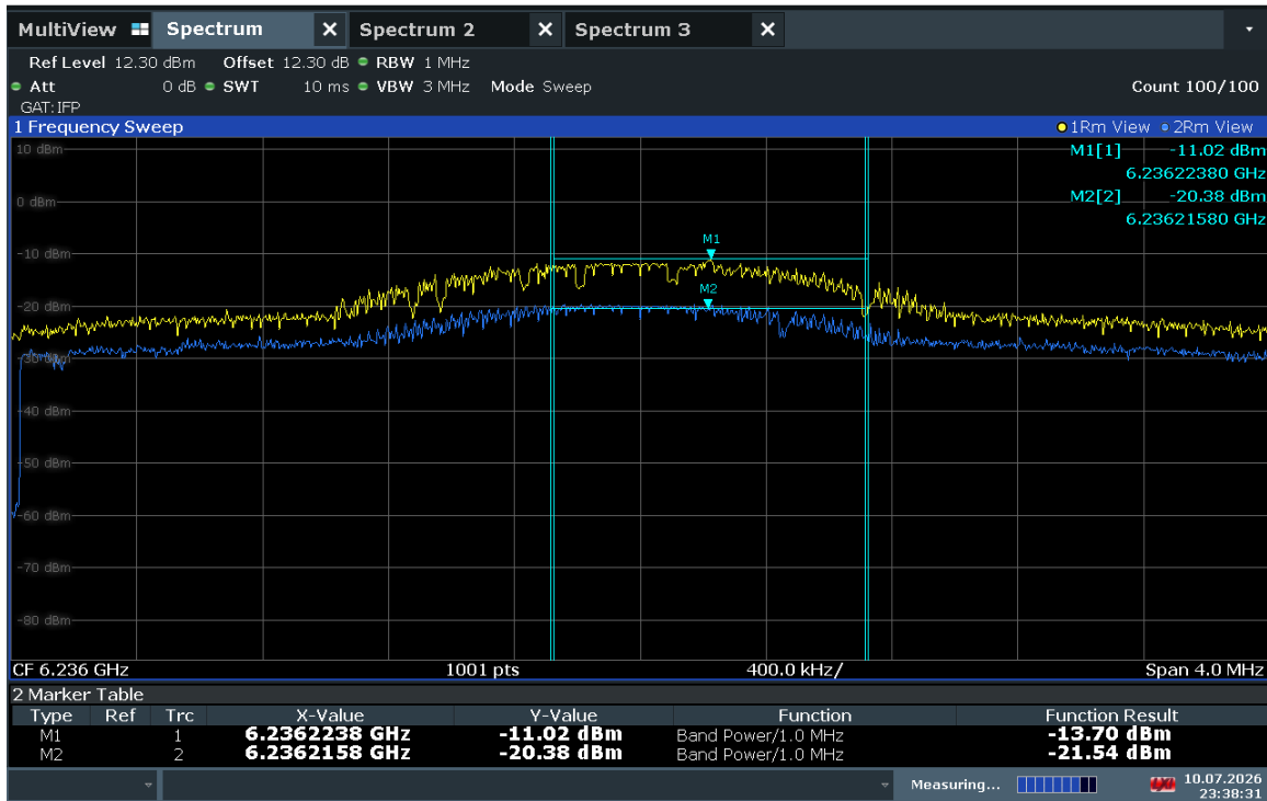
Plot 7-28. Power Density Plot – 6236MHz
