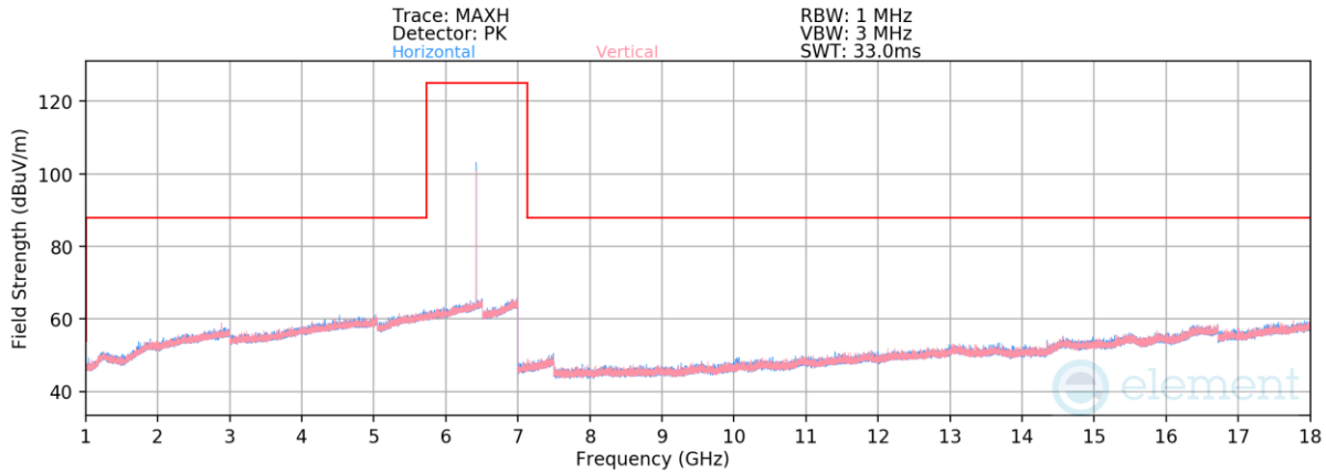
Plot 7-32. Radiated Spurious Emissions 1-18GHz (NB UNII BDR – 6420MHz)
