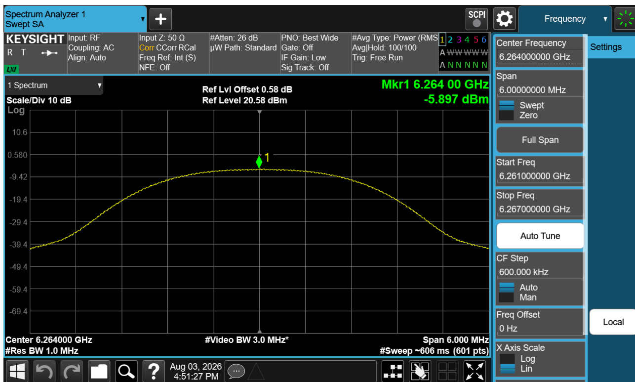
Plot 7-13. PSD (NB UNII HDRp4 – 6264MHz)
