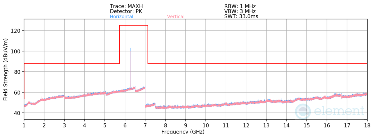
Plot 7-35. Radiated Spurious Emissions 1-18GHz (NB UNII LE1M – 6264MHz)
