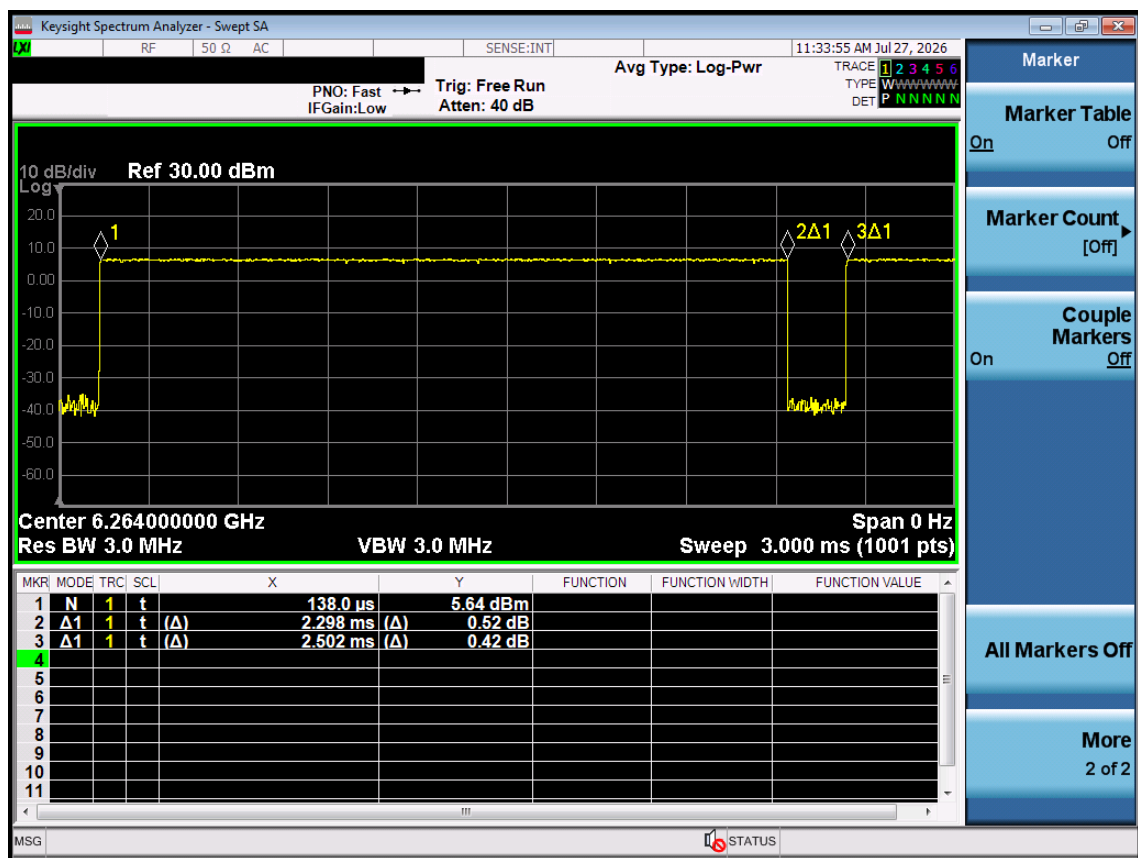
Figure 7-4 NB UNII-5 Transmission Plot
