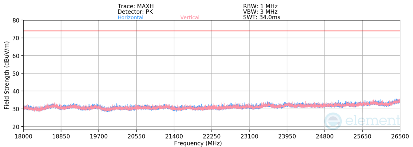
Plot 7-57. Radiated Spurious Emissions above 18GHz (4Mbps, HDRp4 – Ch. 38)
