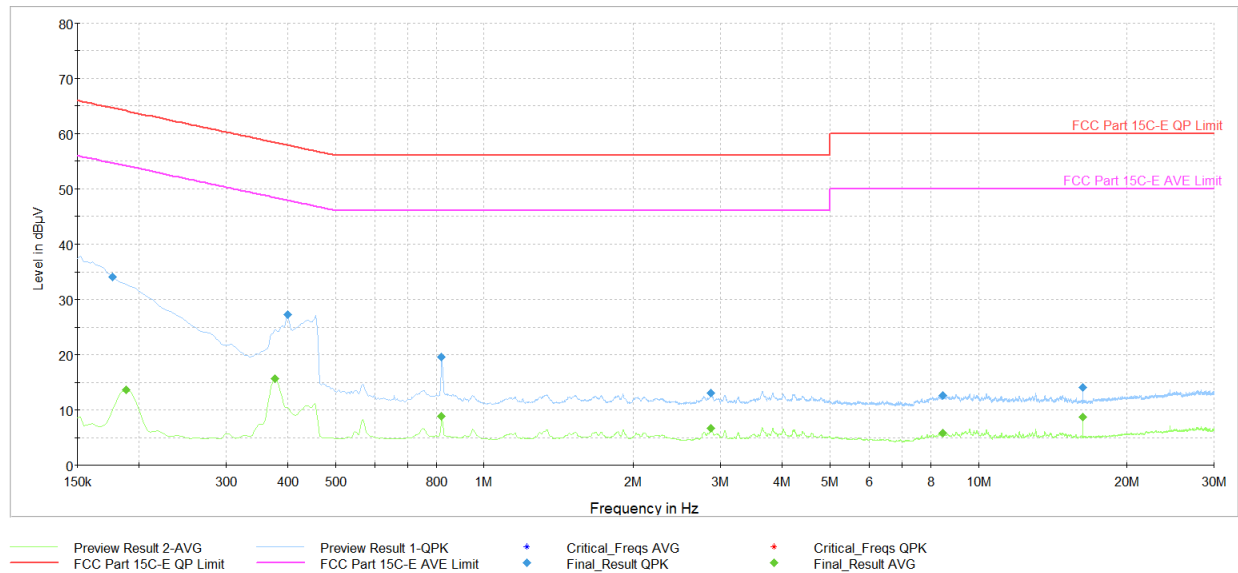
Plot 7-69. AC Line Conducted Plot with Bluetooth HDR (N, HDR4 - Ch.38 with Laptop)
