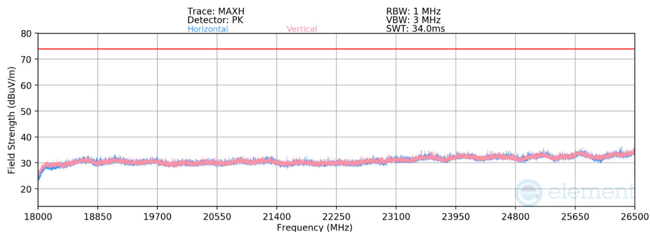
Plot 7-53. Radiated Spurious Emissions Above 18GHz (4Mbps, HDR4 – Ch. 38)
