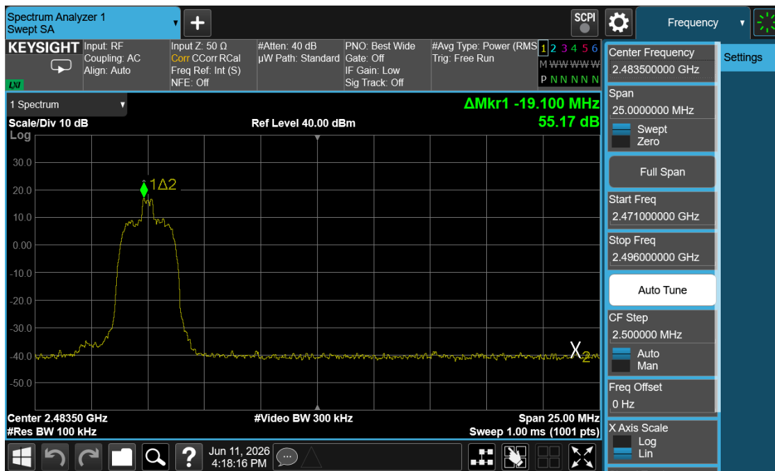
Plot 7-38. Band Edge Plot (Bluetooth (HDR4) – Ch. 73)
