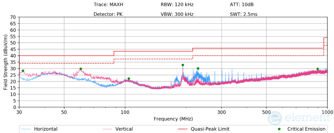
Plot 7-67. Radiated Spurious Emissions Below 1GHz (HDR4 – Ch.38 with AC/DC Adapter)
