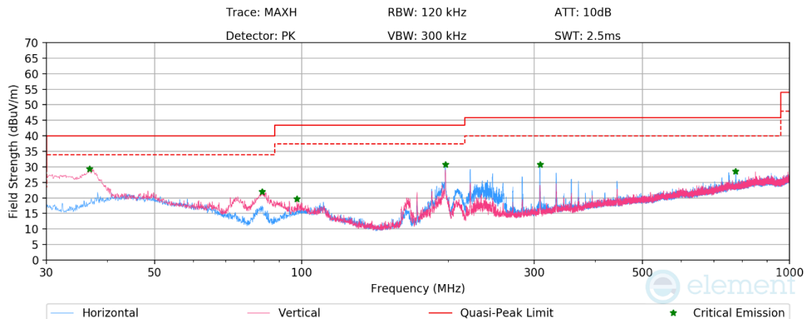
Plot 7-34. Radiated Spurious Emissions Below 1GHz (1Mbps – Ch.37, Pol. H & V, with AC/DC Adapter)
