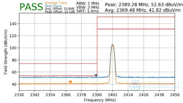
Plot 7-30. Radiated Restricted Lower Band Edge Measurement (Average & Peak)
