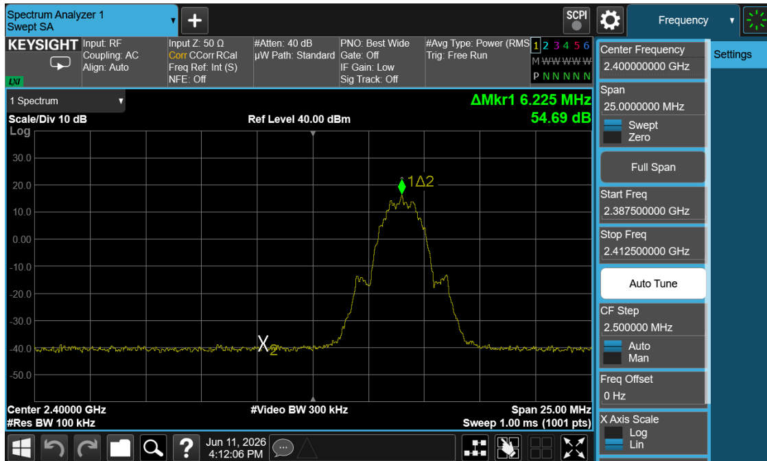
Plot 7-21. Band Edge Plot (Bluetooth (LE), 2Mbps- Ch. 0)
