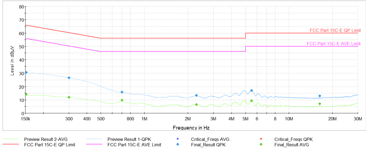
Plot 7-36. AC Line Conducted Plot with Bluetooth LE (N, 1Mbps – Ch.37, with AC/DC Adapter)
