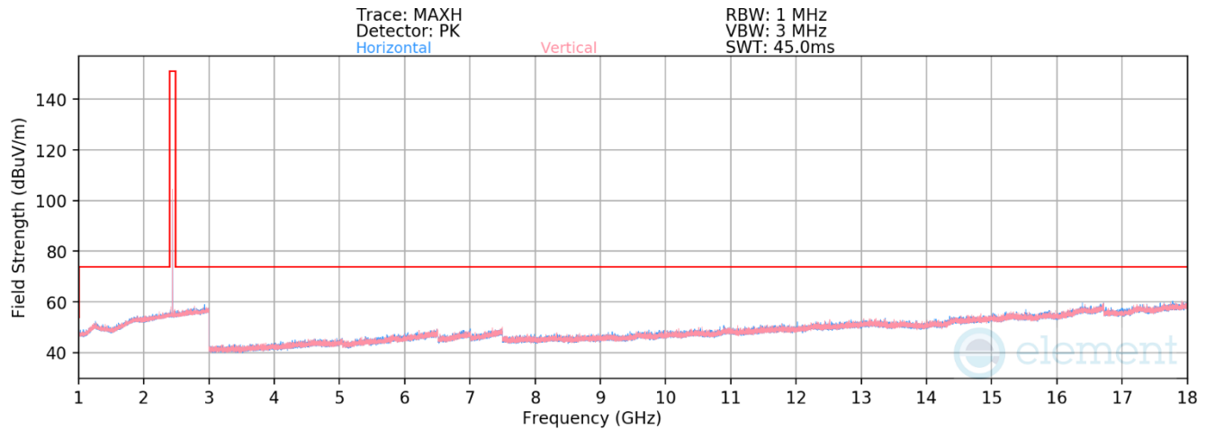
Plot 7-28. Radiated Spurious Emissions 1-18GHz (1Mbps – Ch. 17)
