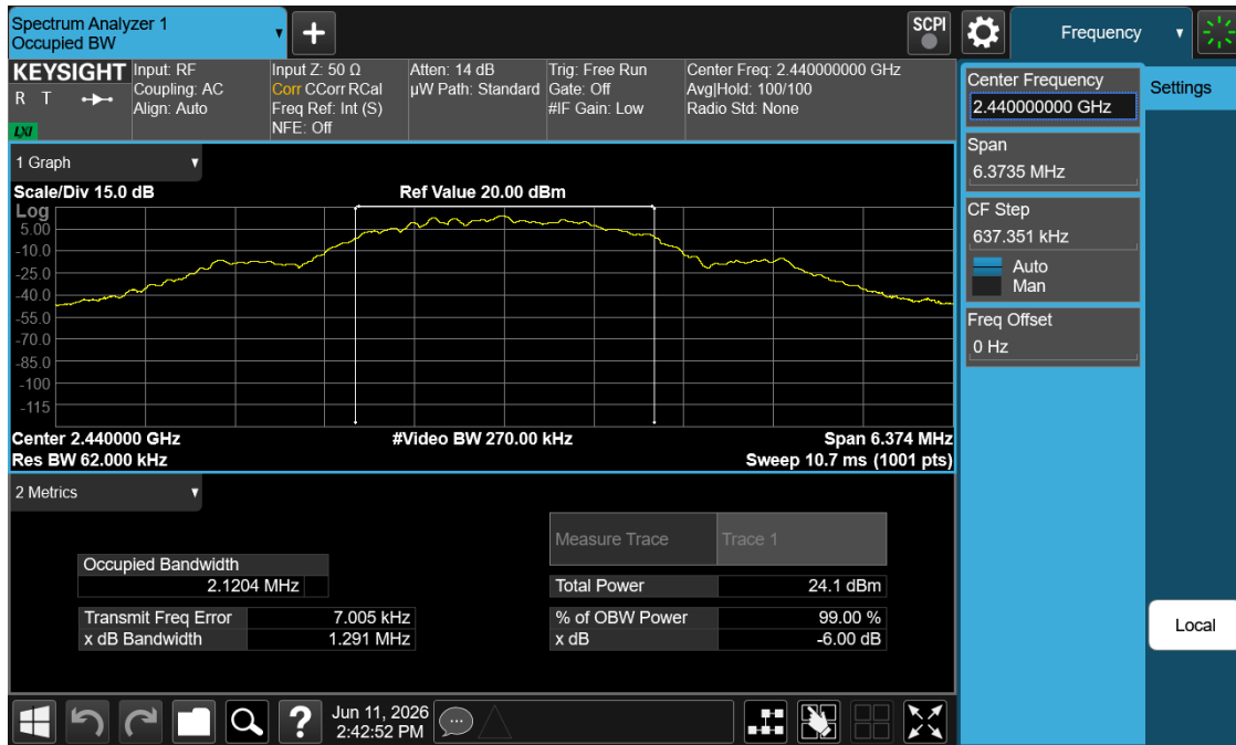
Plot 7-5. 99% OBW Plot (Bluetooth (LE), 2Mbps– Ch. 17)
