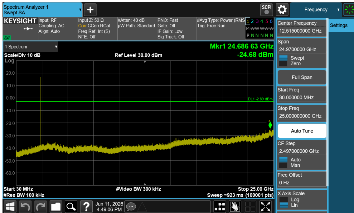
Plot 7-23. Conducted Spurious Plot (Bluetooth (LE), 1Mbps – Ch. 37)
