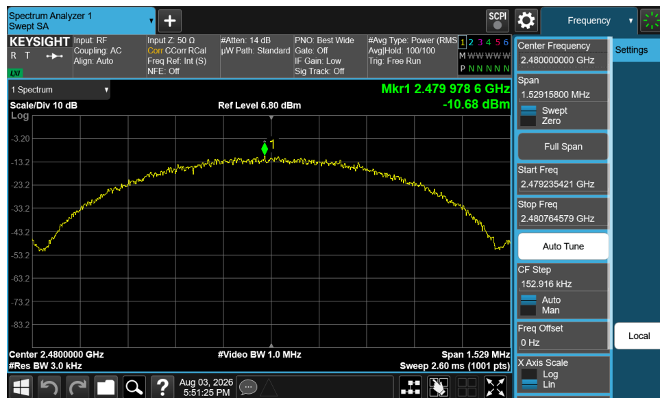
Plot 7-15. Power Spectral Density Plot (Bluetooth (LE), 1Mbps – Ch. 39)
