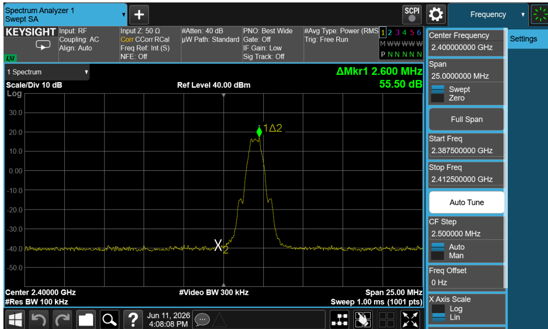
Plot 7-19. Band Edge Plot (Bluetooth (LE), 1Mbps – Ch. 37)
