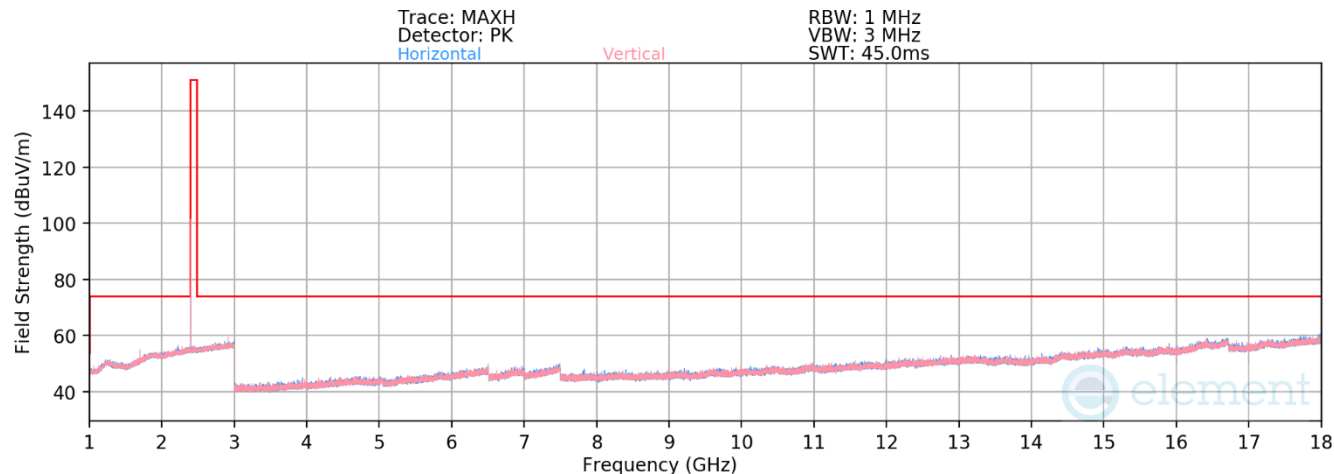
Plot 7-26. Radiated Spurious Emissions 1-18GHz (1Mbps – Ch. 37)
