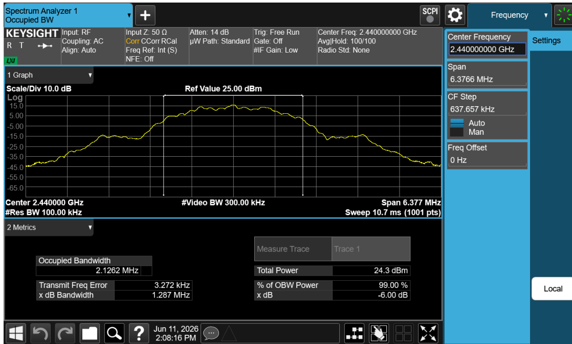
Plot 7-11. 6dB BW Plot (Bluetooth (LE), 2Mbps– Ch. 17)
