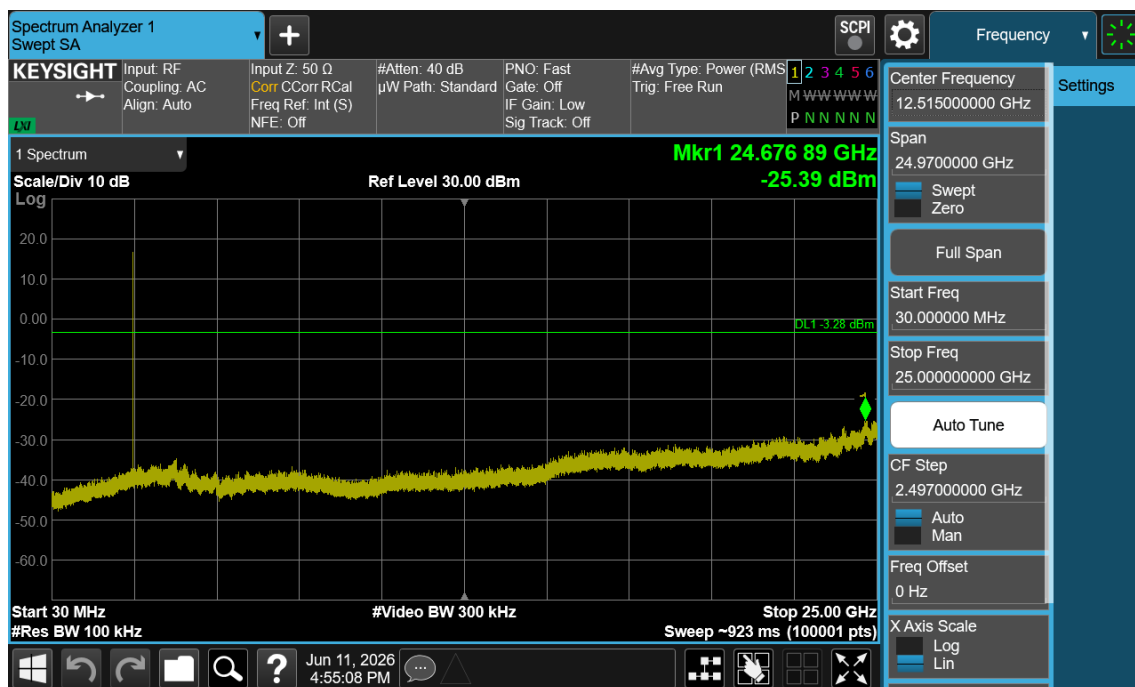
Plot 7-25. Conducted Spurious Plot (Bluetooth (LE), 1Mbps – Ch. 39)
