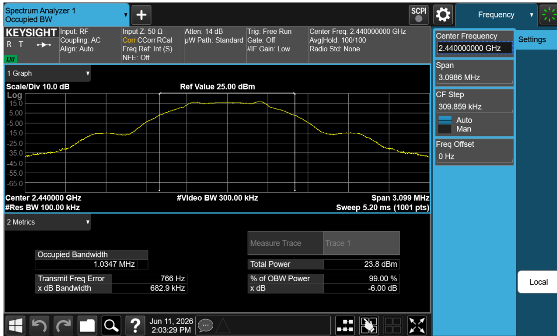
Plot 7-8. 6dB BW Plot (Bluetooth (LE), 1Mbps – Ch. 17)
