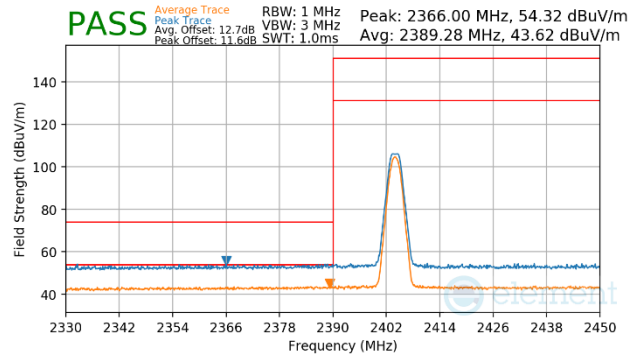
Plot 7-32. Radiated Restricted Lower Band Edge Measurement (Average & Peak)
