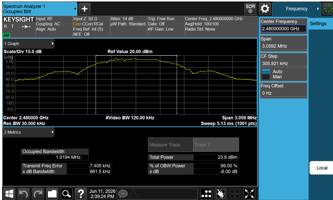
Plot 7-3. 99% OBW Plot (Bluetooth (LE), 1Mbps – Ch. 39)
