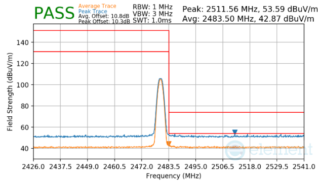
Plot 7-31. Radiated Restricted Upper Band Edge Measurement (Average & Peak)
