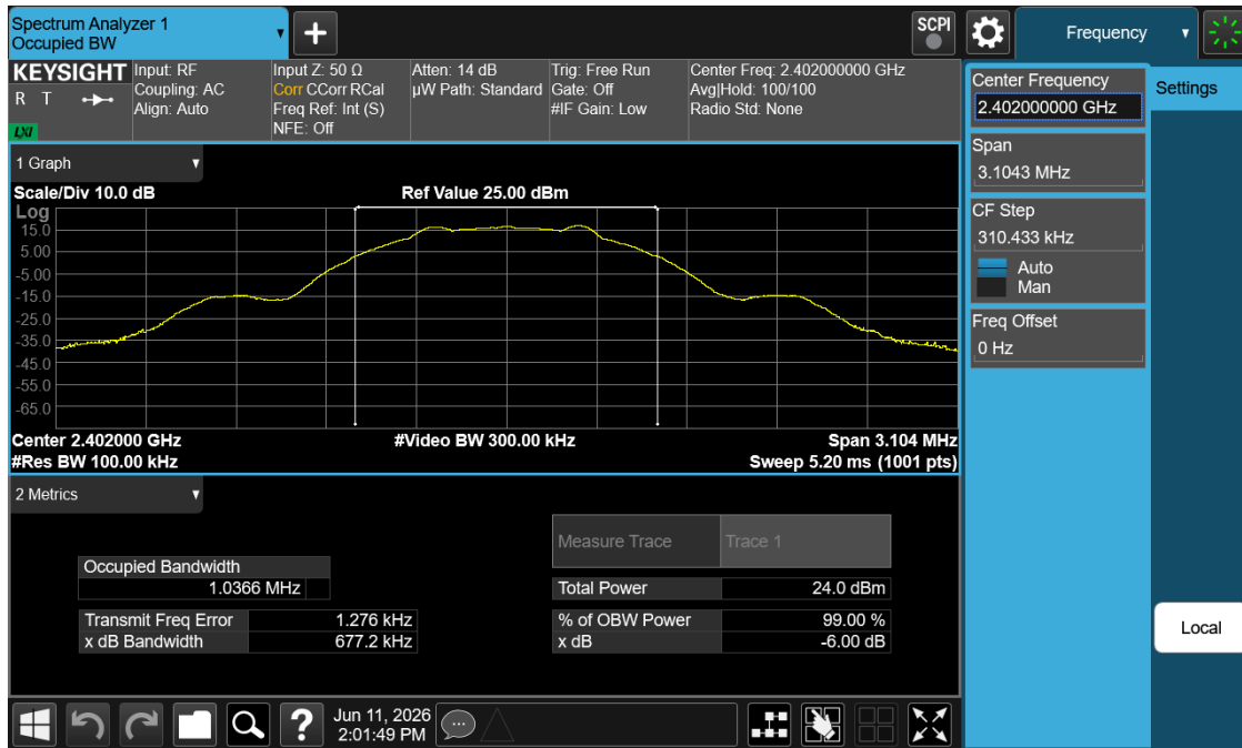
Plot 7-7. 6dB BW Plot (Bluetooth (LE), 1Mbps – Ch. 37)
