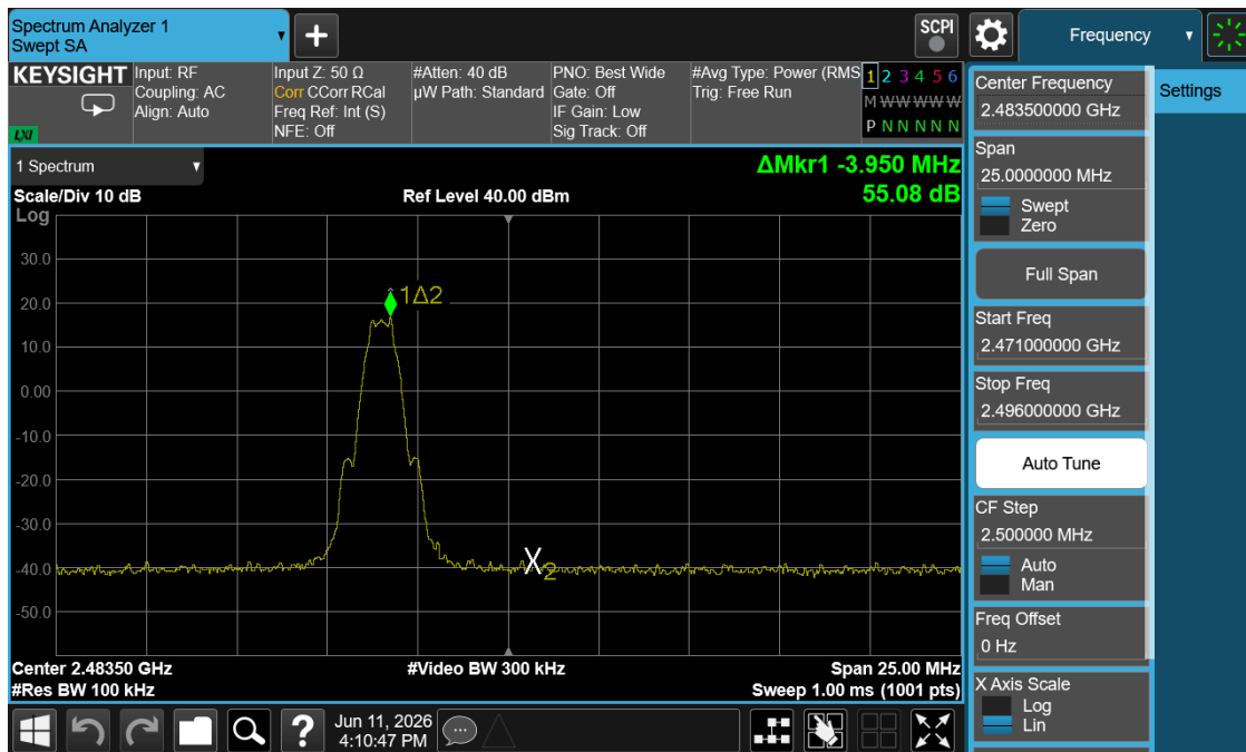
Plot 7-20. Band Edge Plot (Bluetooth (LE), 1Mbps – Ch. 39)
