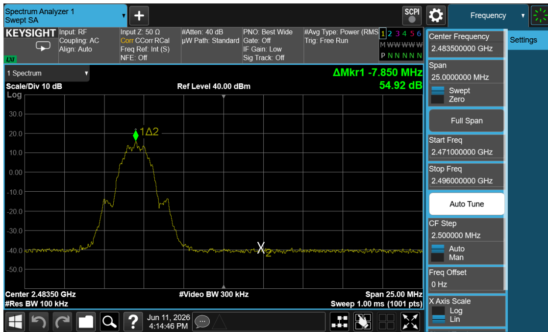
Plot 7-22. Band Edge Plot (Bluetooth (LE), 2Mbps- Ch. 36)
