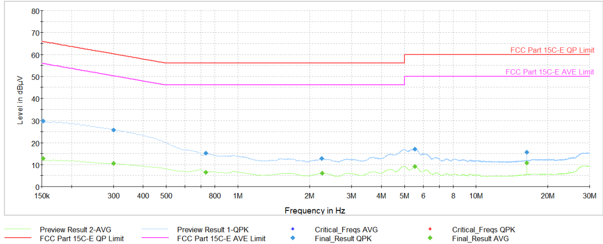
Plot 7-35. AC Line Conducted Plot with Bluetooth LE (L1, 1Mbps – Ch.37 with AC/DC Adapter)
