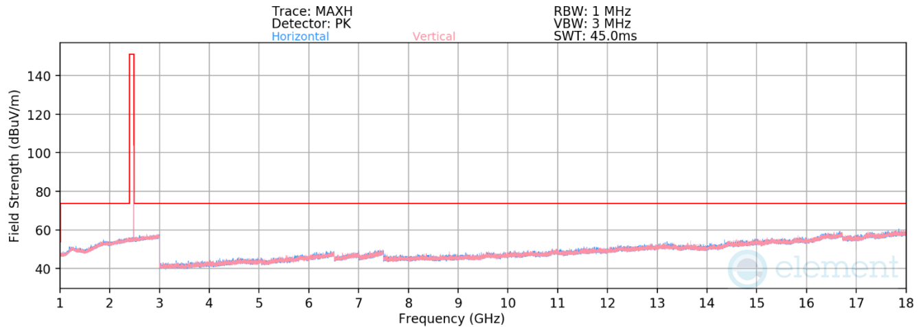
Plot 7-29. Radiated Spurious Emissions 1-18GHz (1Mbps – Ch. 39)
