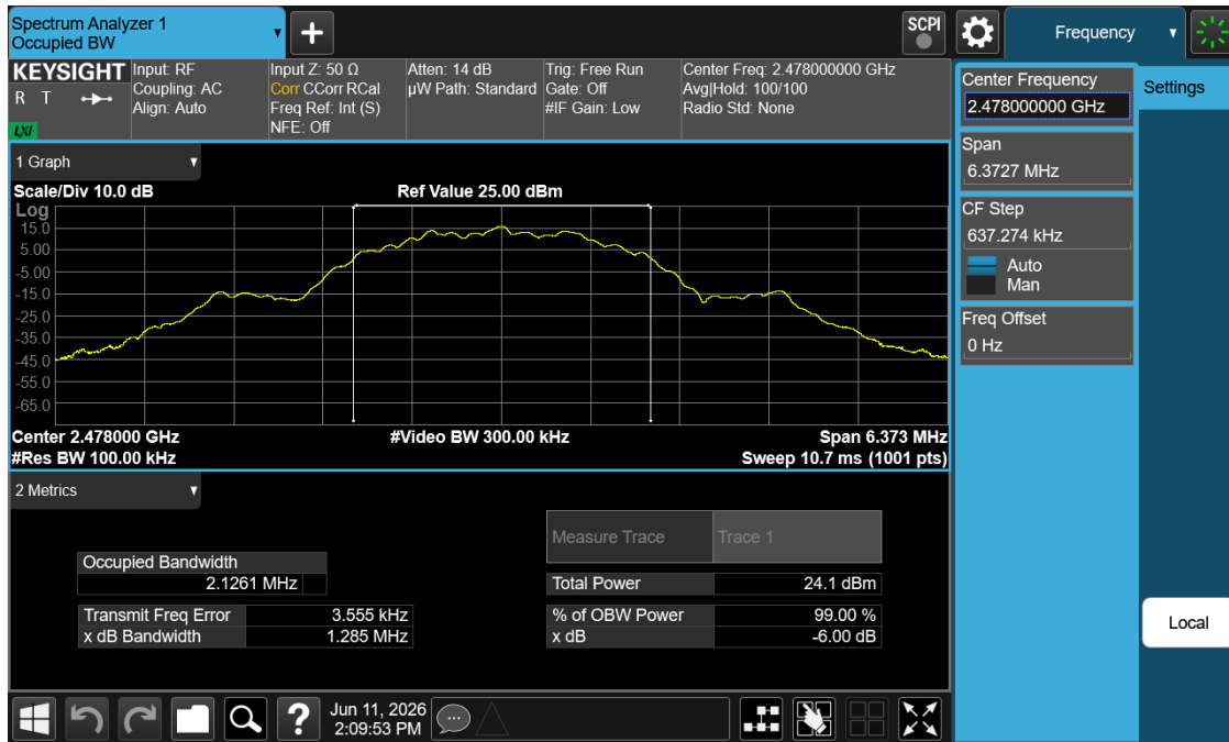
Plot 7-12. 6dB BW Plot (Bluetooth (LE), 2Mbps– Ch. 36)
