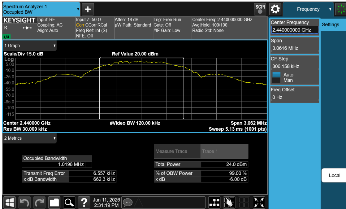
Plot 7-2. 99% OBW Plot (Bluetooth (LE), 1Mbps – Ch. 17)
