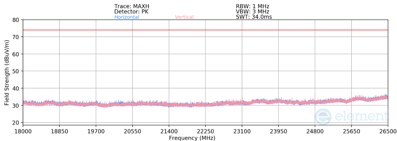
Plot 7-27. Radiated Spurious Emissions Above 18GHz (1Mbps – Ch. 37)
