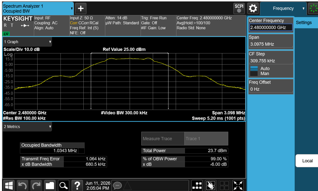
Plot 7-9. 6dB BW Plot (Bluetooth (LE), 1Mbps – Ch. 39)
