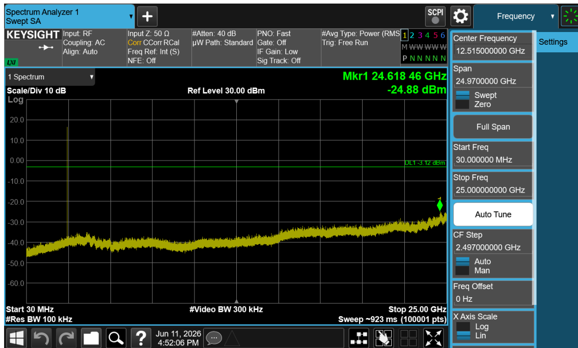
Plot 7-24. Conducted Spurious Plot (Bluetooth (LE), 1Mbps – Ch. 17)
