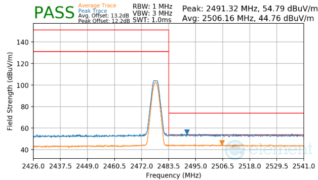
Plot 7-33. Radiated Restricted Upper Band Edge Measurement (Average & Peak)
