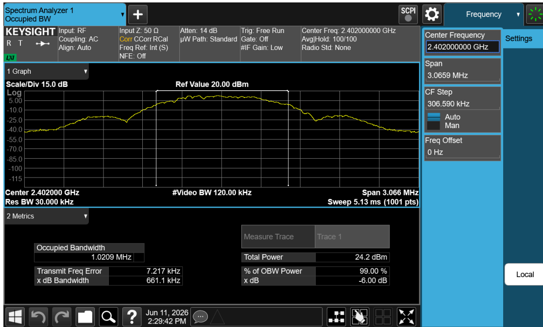
Plot 7-1. 99% OBW Plot (Bluetooth (LE), 1Mbps – Ch. 37)
