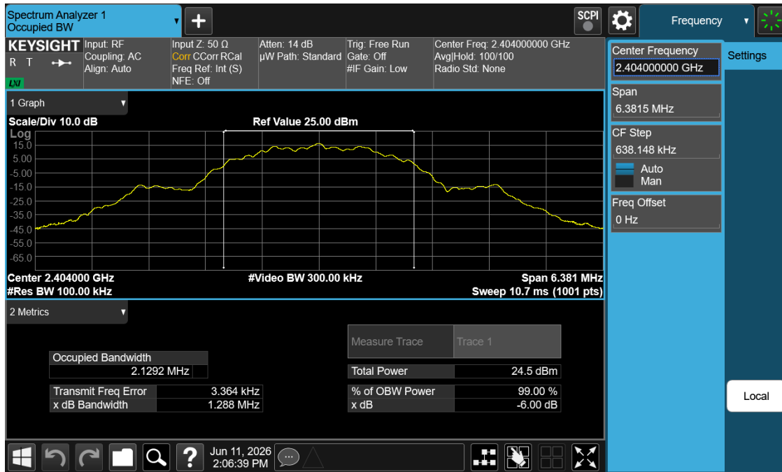
Plot 7-10. 6dB BW Plot (Bluetooth (LE), 2Mbps– Ch. 0)
