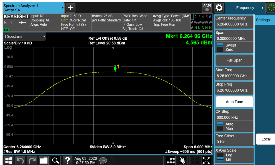
Plot 7-13. PSD (NB UNII HDRp4 – 6264MHz)
