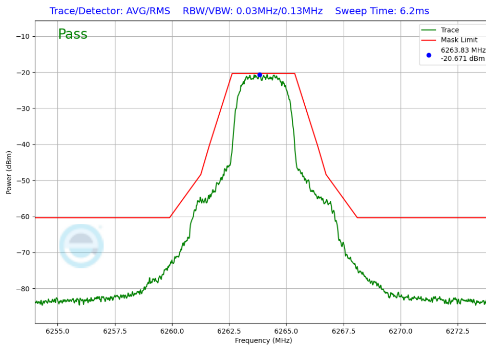
Plot 7-20. In-Band Emission (NB UNII HDRp4 – 6264MHz)
