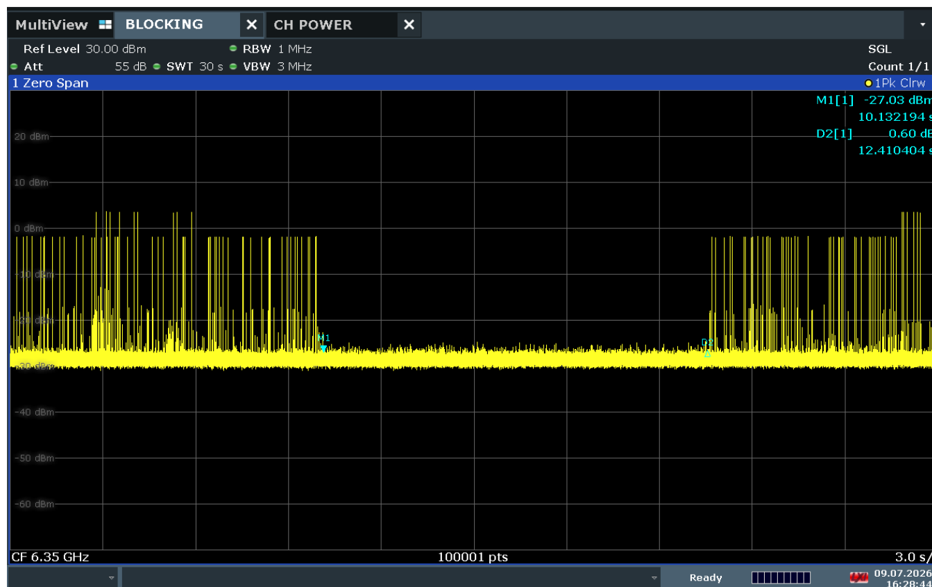
Plot 7-24. Contention Based Protocol Timing Plot
