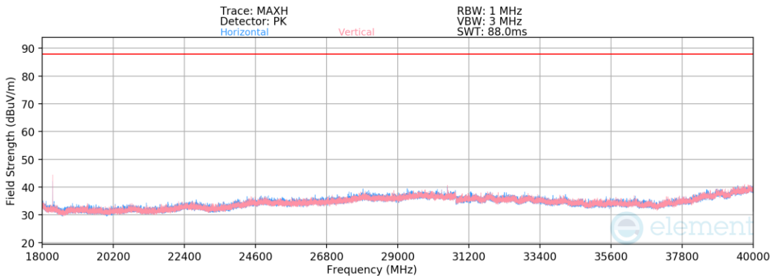
Plot 7-31. Radiated Spurious Emissions Above 18GHz (BDR GFSK – 6108MHz)
