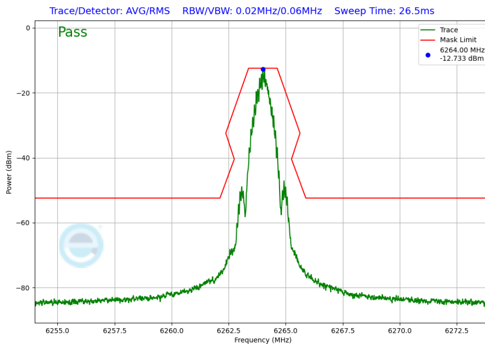
Plot 7-15. In-Band Emission (NB UNII BDR – 6264MHz)
