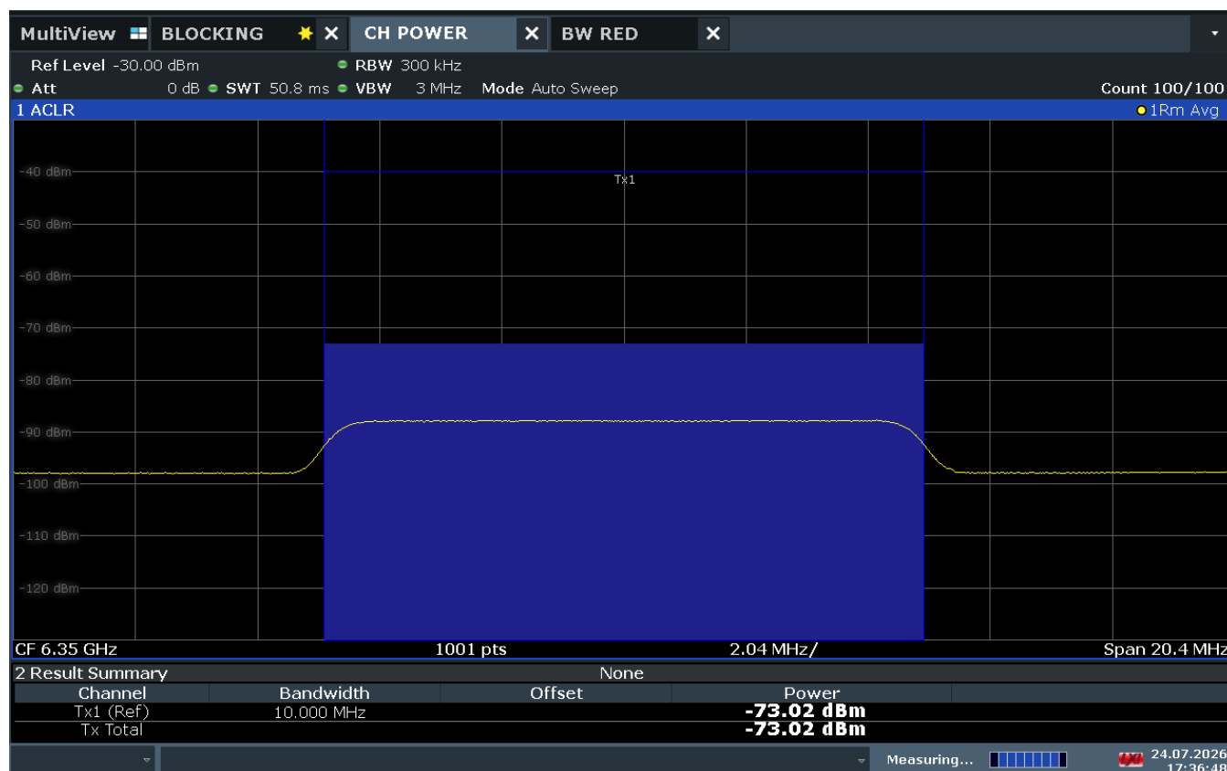
Plot 7-23. Channel Power Signal
