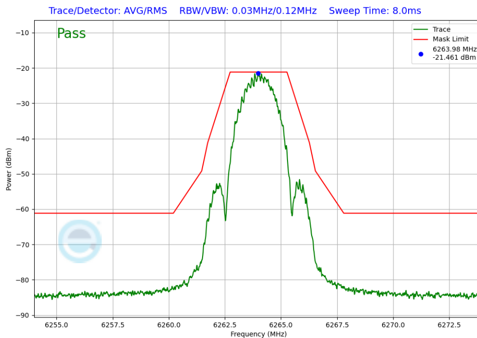
Plot 7-17. In-Band Emission (NB UNII LE2M – 6264MHz)
