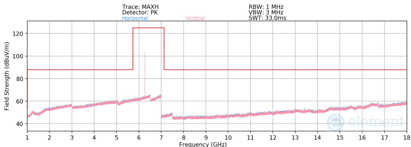
Plot 7-32. Radiated Spurious Emissions 1-18GHz (BDR GFSK – 6264MHz)
