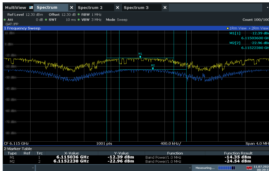
Plot 7-27. Power Density Plot 6115MHz
