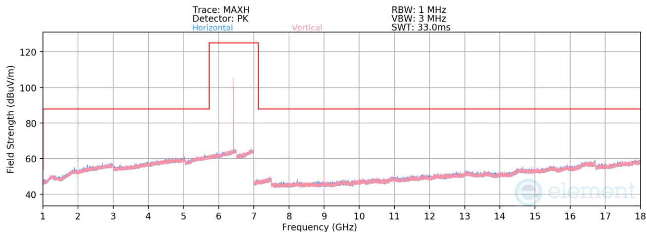
Plot 7-33. Radiated Spurious Emissions 1-18GHz (BDR GFSK – 6420MHz)
