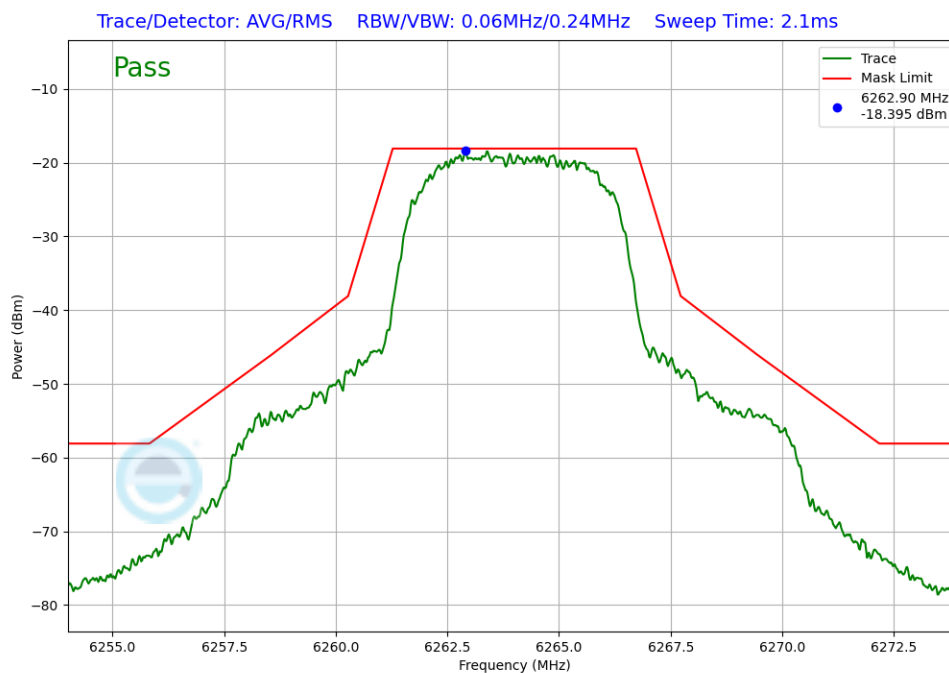
Plot 7-21. In-Band Emission (NB UNII HDRp8 – 6264MHz)
