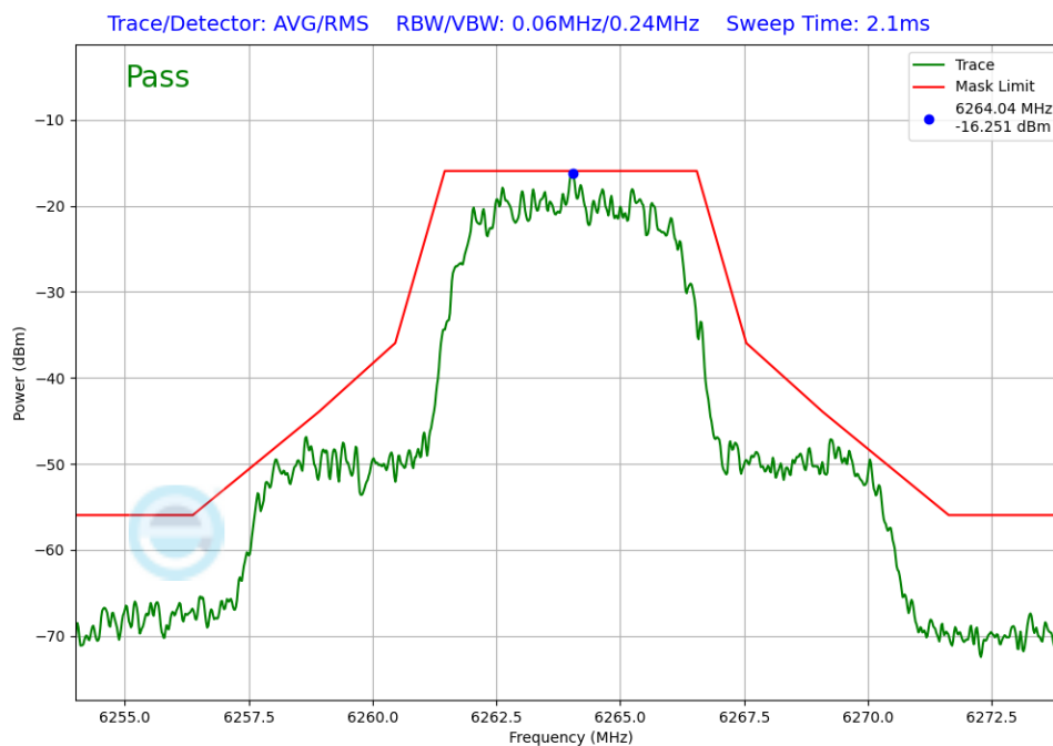
Plot 7-19. In-Band Emission (NB UNII HDR8 – 6264MHz)
