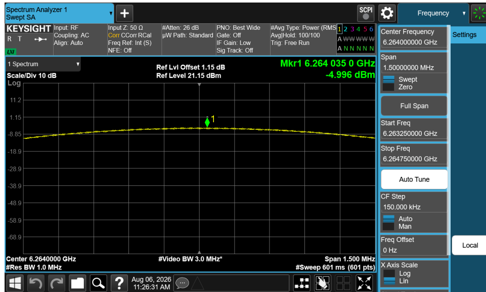
Plot 7-8. PSD (NB UNII BDR – 6264MHz)
