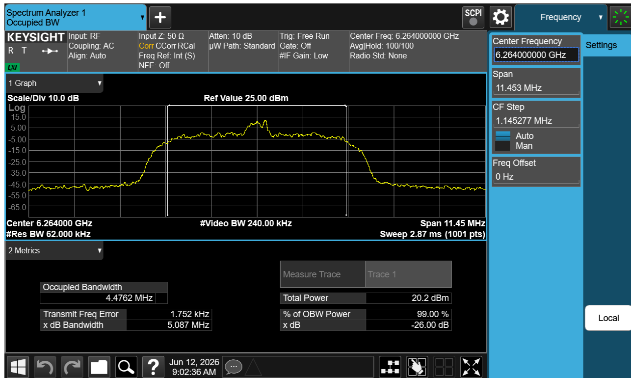
Plot 7-5. 26dB BW & 99% OBW (NB UNII HDR8 – 6264MHz)
