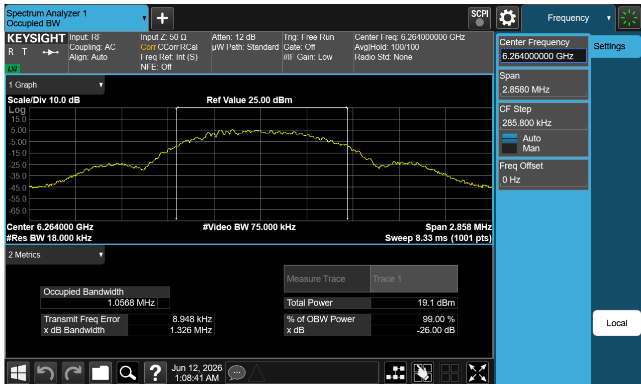
Plot 7-2. 26dB BW & 99% OBW (NB UNII LE1M – 6264MHz)
