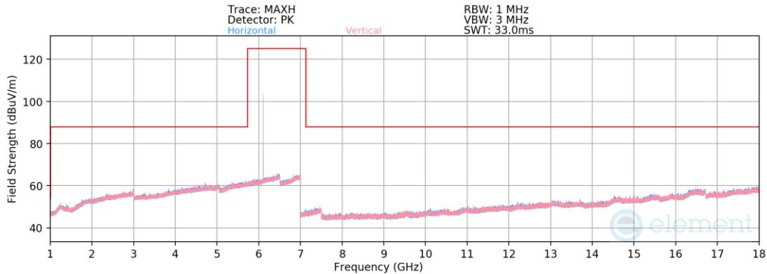
Plot 7-30. Radiated Spurious Emissions 1-18GHz (BDR GFSK – 6108MHz)
