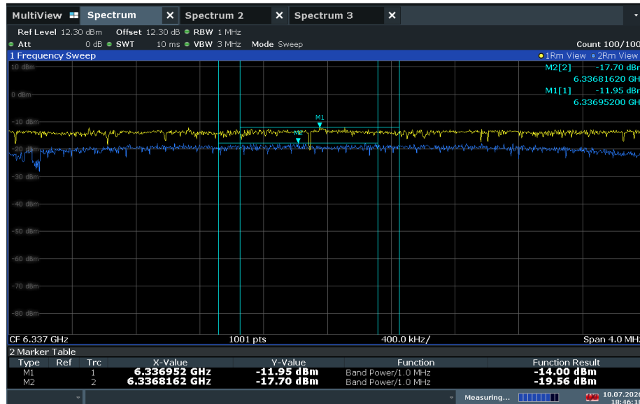
Plot 7-29. Power Density Plot – 6337MHz
