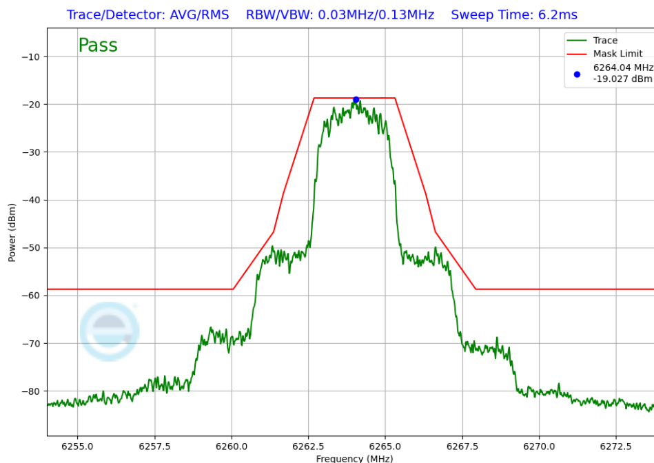
Plot 7-18. In-Band Emission (NB UNII HDR4 – 6264MHz)
