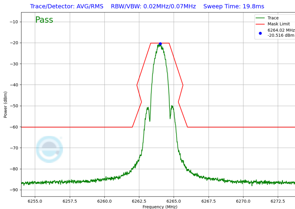
Plot 7-16. In-Band Emission (NB UNII LE1M – 6264MHz)
