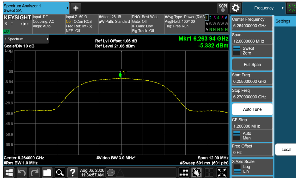
Plot 7-12. PSD (NB UNII HDR8 – 6264MHz)
