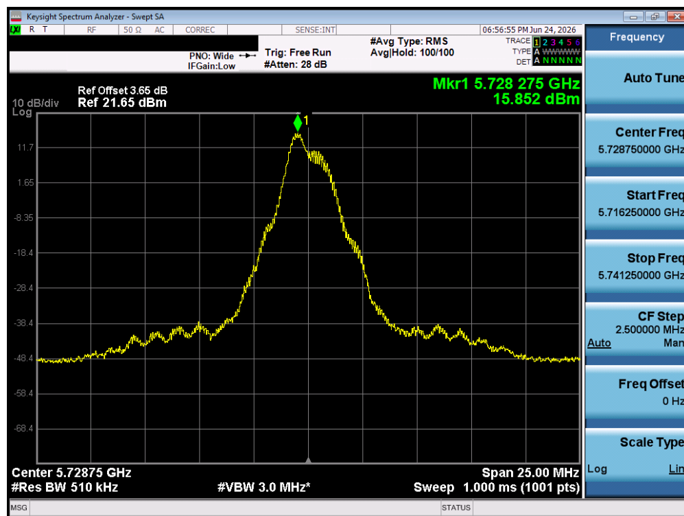
Plot 7-22. PSD (O-QPSK, 5728.75MHz, 500kbps)
