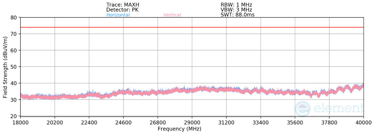
Plot 7-30. Radiated Spurious Emissions Above 18GHz (O-QPSK – 5786.25MHz)
