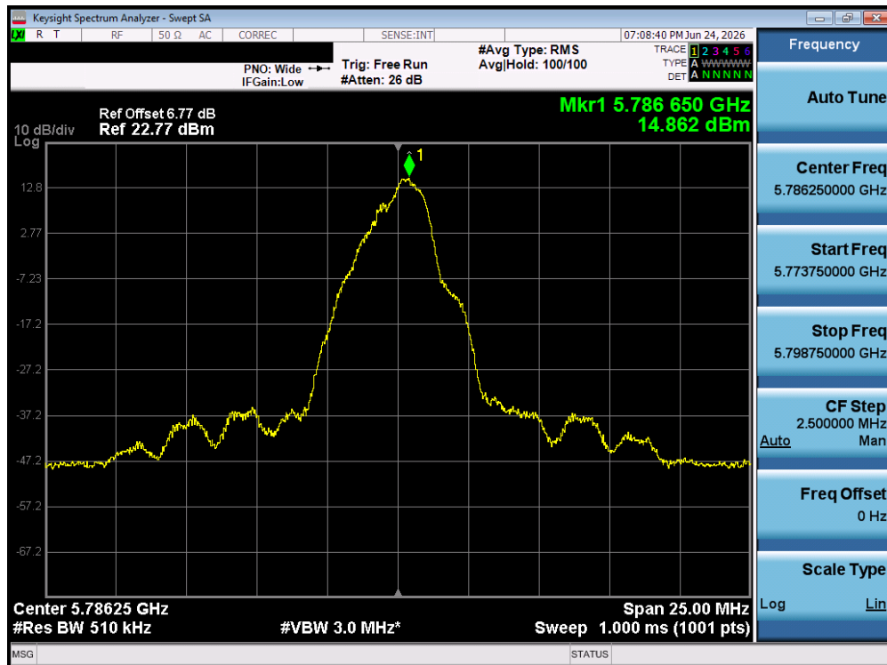
Plot 7-26. PSD (O-QPSK, 5786.25MHz, 1000kbps)
