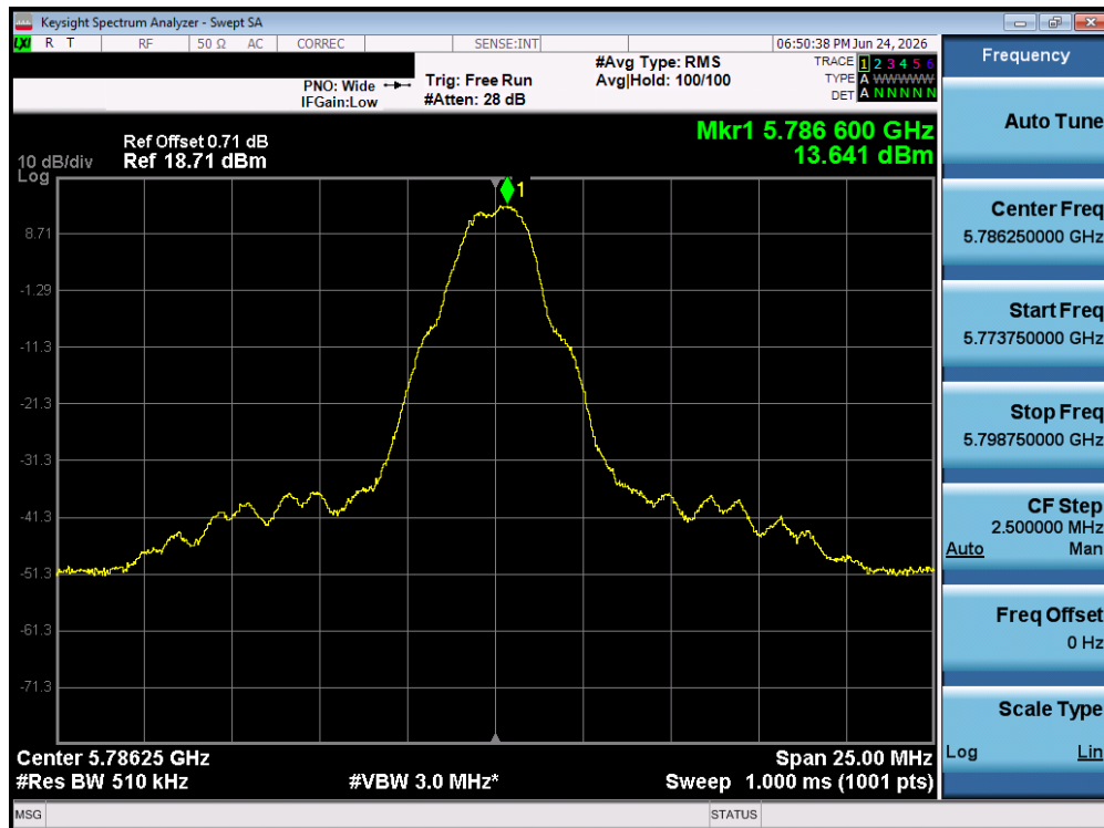
Plot 7-20. PSD (O-QPSK, 5786.25MHz, 250kbps)
