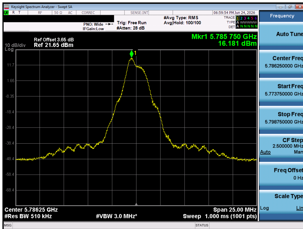
Plot 7-23. PSD (O-QPSK, 5786.25MHz, 500kbps)
