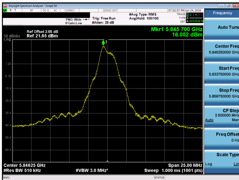
Plot 7-24. PSD (O-QPSK, 5846.25MHz, 500kbps)
