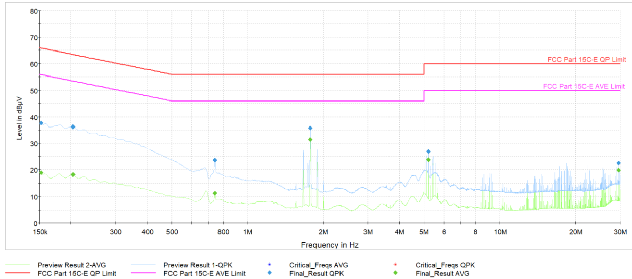
Plot 7-40. AC Line Conducted Plot (O-QPSK, 250Kbps – Ch. 24) (N) with AC/DC Adapter & magnetic charger
