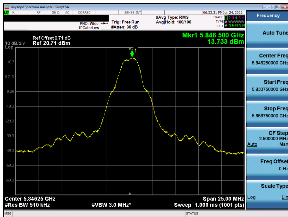
Plot 7-21. PSD (O-QPSK, 5846.25MHz, 250kbps)
