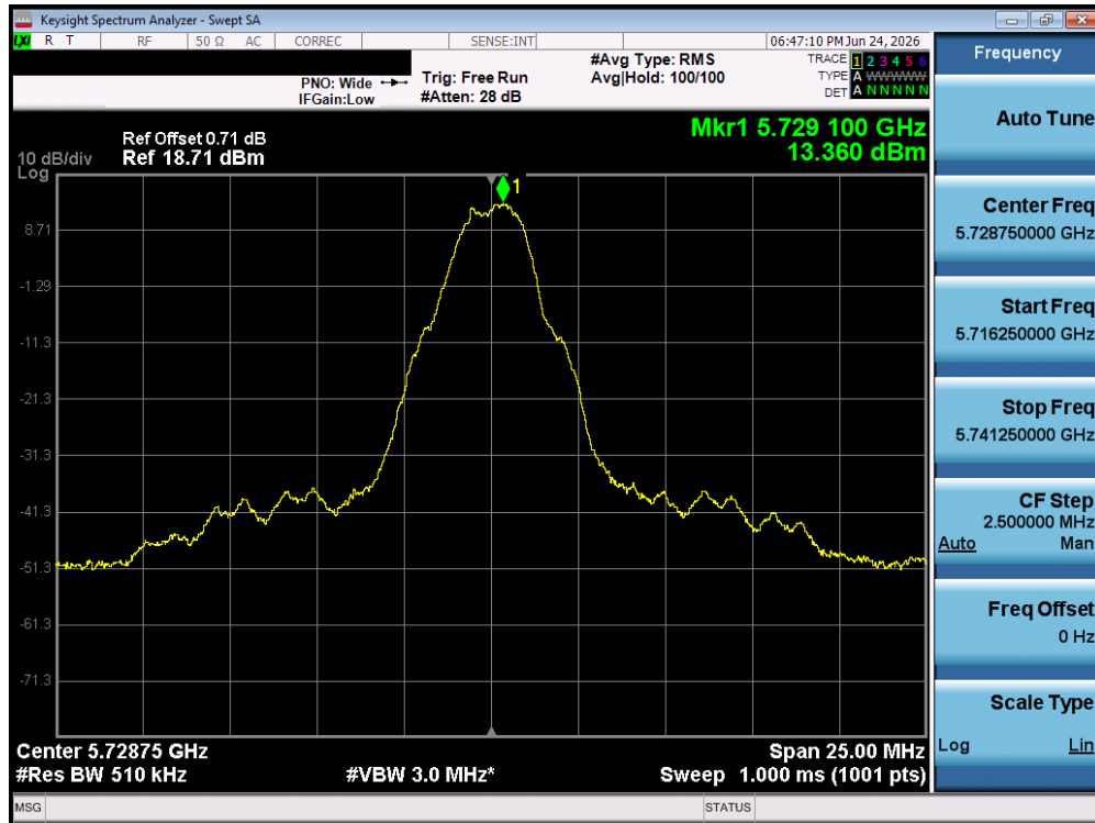
Plot 7-19. PSD (O-QPSK, 5728.75MHz, 250kbps)
