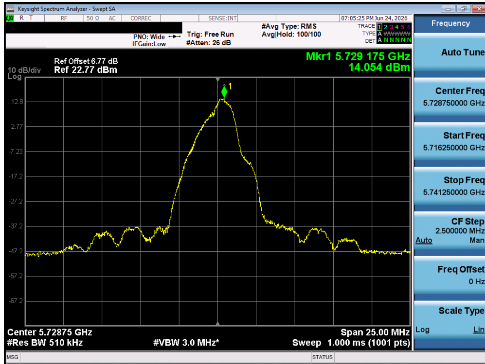
Plot 7-25. PSD (O-QPSK, 5728.75MHz, 1000kbps)
