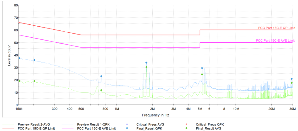
Plot 7-39. AC Line Conducted Plot (O-QPSK, 250Kbps – Ch. 24) (L1) with AC/DC Adapter & magnetic charger
