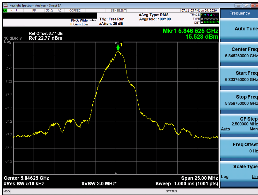
Plot 7-27. PSD (O-QPSK, 5846.25MHz, 1000kbps)
