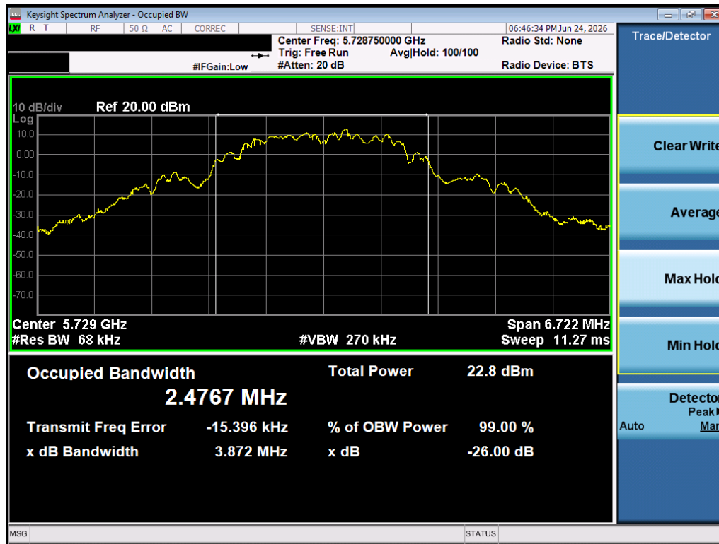
Plot 7-1. 99% OBW (O-QPSK, 5728.75MHz, 250kbps)
