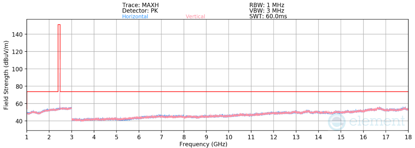
Plot 7-19. Radiated Spurious Emissions 1-18GHz (4Mbps, HDR4, ePA – Ch. 73)
