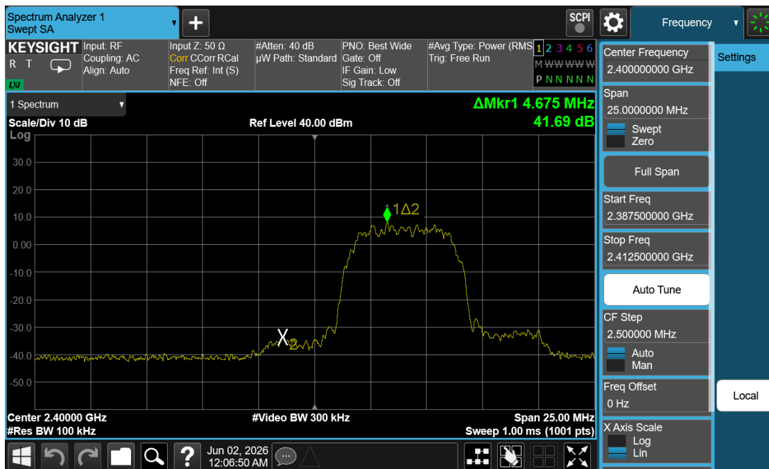
Plot 7-11. Band Edge Plot (Bluetooth (HDR8), ePA – Ch. 1)
