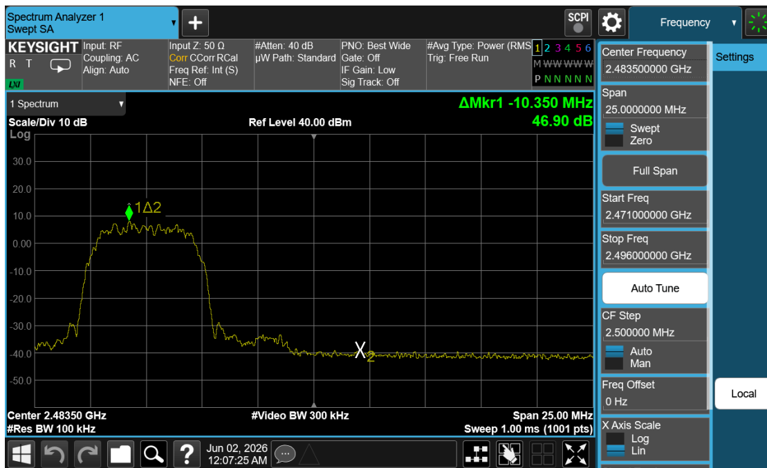
Plot 7-12. Band Edge Plot (Bluetooth (HDR8), ePA – Ch. 73)
