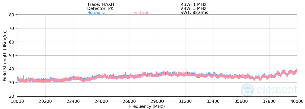
Plot 7-18. Radiated Spurious Emissions above 18GHz (4Mbps, HDR4, ePA – Ch. 38)
