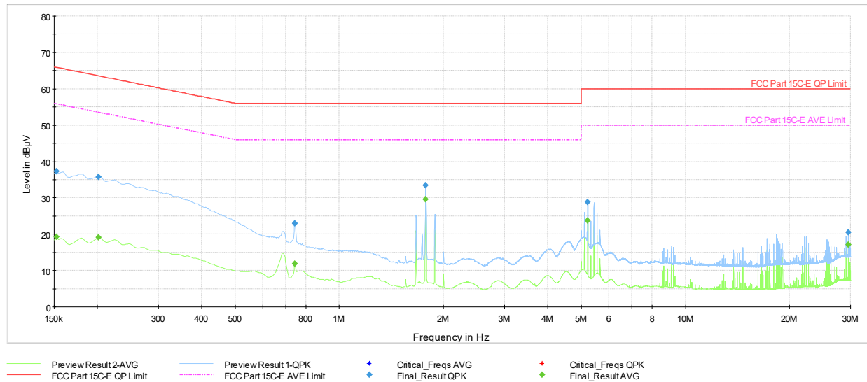
Plot 7-25. AC Line Conducted Plot with Bluetooth HDR (L1, HDR4 ePA - Ch.38 with AC/DC Adapter)
