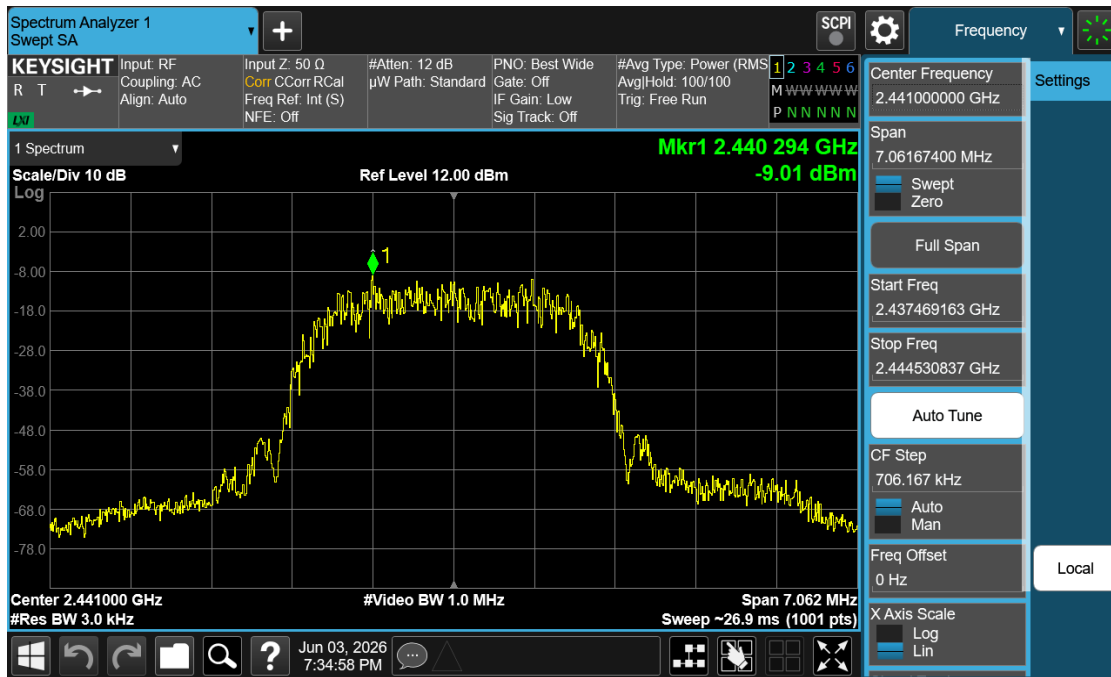
Plot 7-6. Power Spectral Density Plot (Bluetooth (HDR4), 4Mbps, iPA – Ch. 38)
