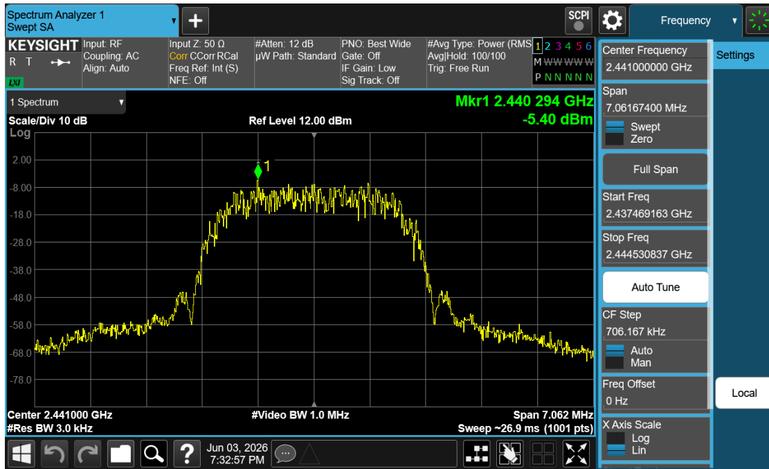
Plot 7-5. Power Spectral Density Plot (Bluetooth (HDR4), 4Mbps, ePA – Ch. 38)
