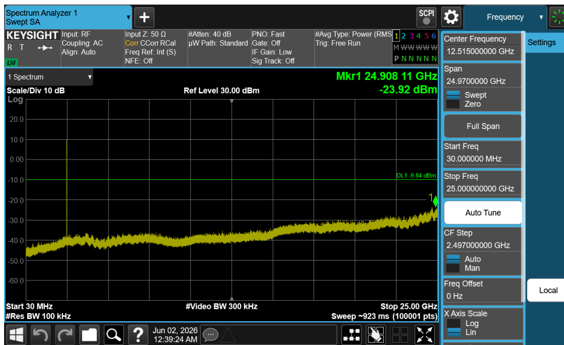
Plot 7-15. Conducted Spurious Plot (Bluetooth (HDR4), 4 Mbps, ePA – Ch. 73)
