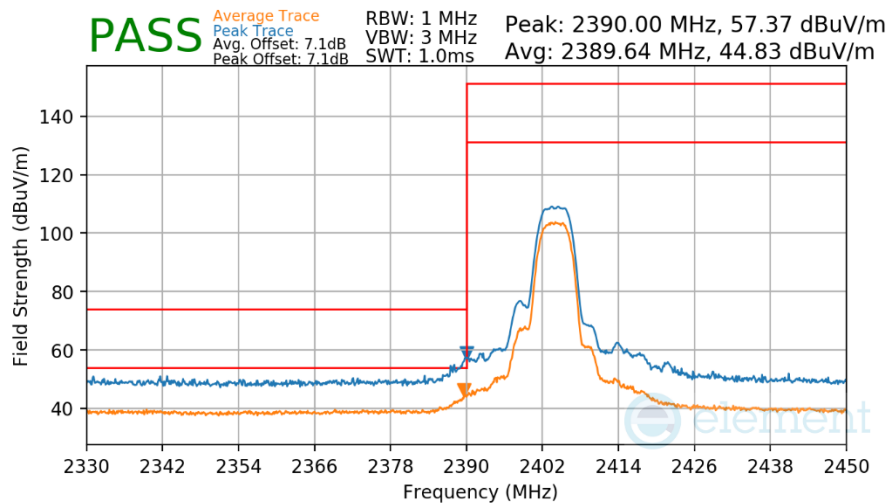
Plot 7-21. Radiated Restricted Lower Band Edge Measurement
