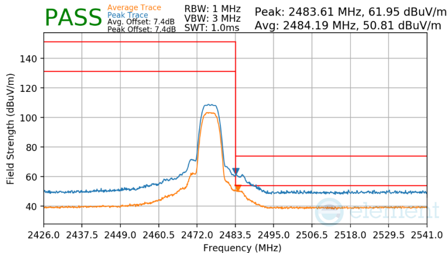
Plot 7-23. Radiated Restricted Upper Band Edge Measurement
