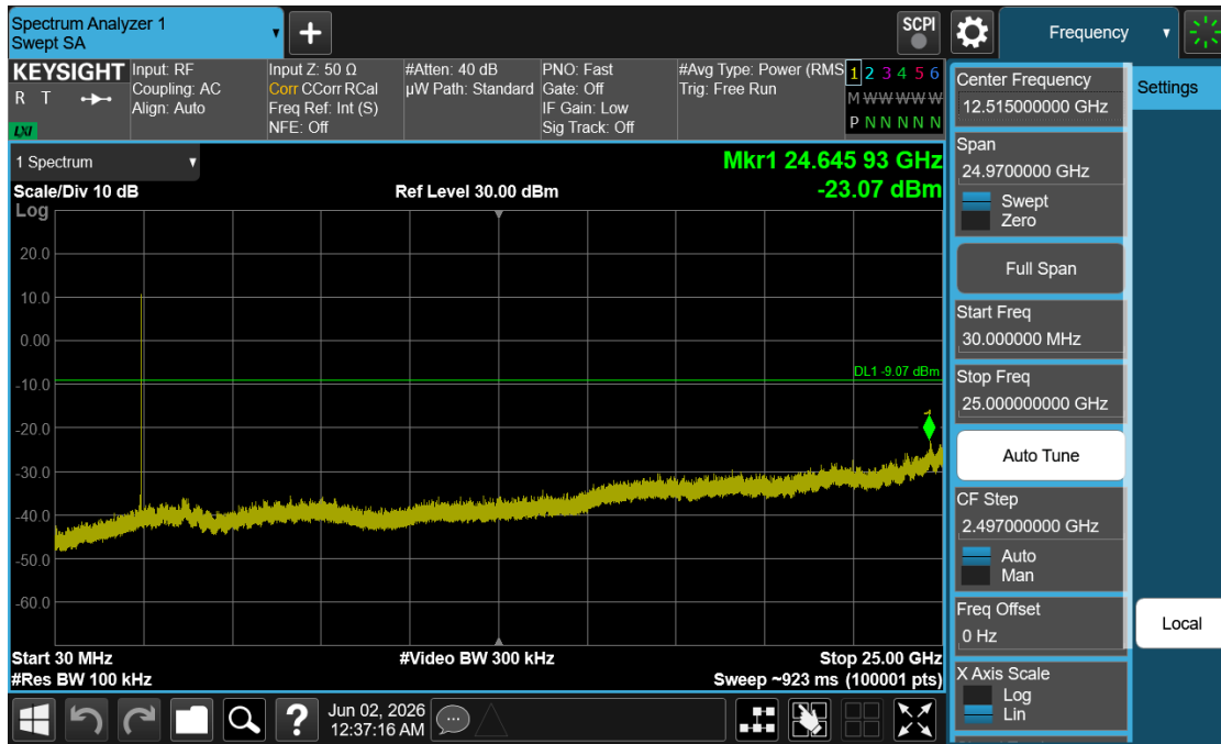
Plot 7-14. Conducted Spurious Plot (Bluetooth (HDR4), 4 Mbps, ePA – Ch. 38)
