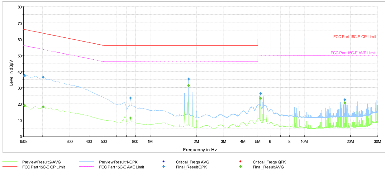
Plot 7-26. AC Line Conducted Plot with Bluetooth HDR (N, HDR4 ePA - Ch.38 with AC/DC Adapter)
