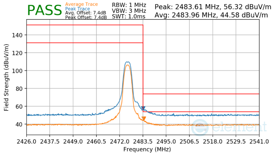
Plot 7-22. Radiated Restricted Upper Band Edge Measurement
