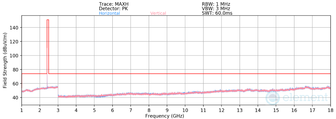
Plot 7-16. Radiated Spurious Emissions 1-18GHz (4Mbps, HDR4, ePA – Ch. 1)
