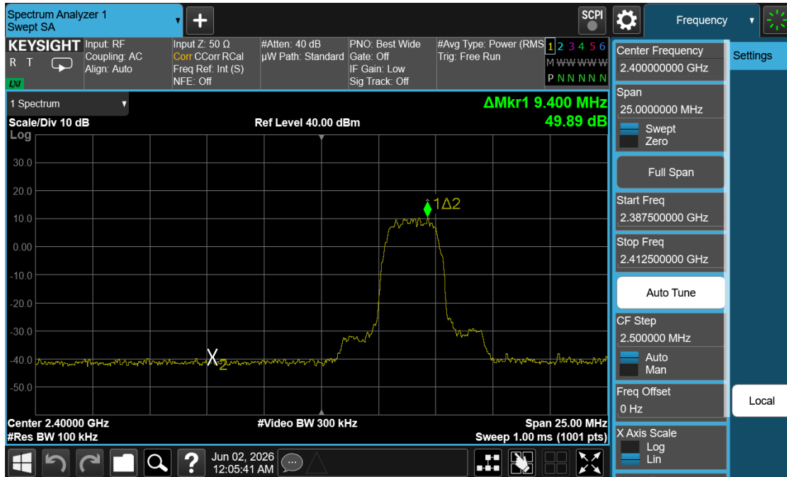
Plot 7-9. Band Edge Plot (Bluetooth (HDR4), ePA – Ch. 1)
