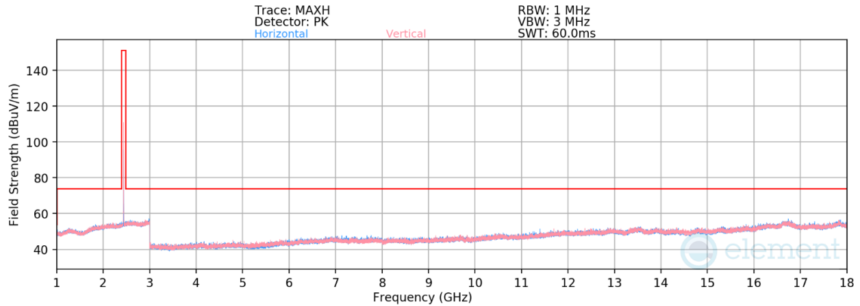
Plot 7-17. Radiated Spurious Emissions 1-18GHz (4Mbps, HDR4, ePA – Ch. 38)
