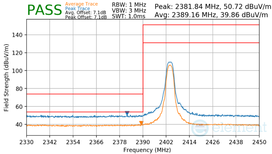
Plot 7-20. Radiated Restricted Lower Band Edge Measurement
