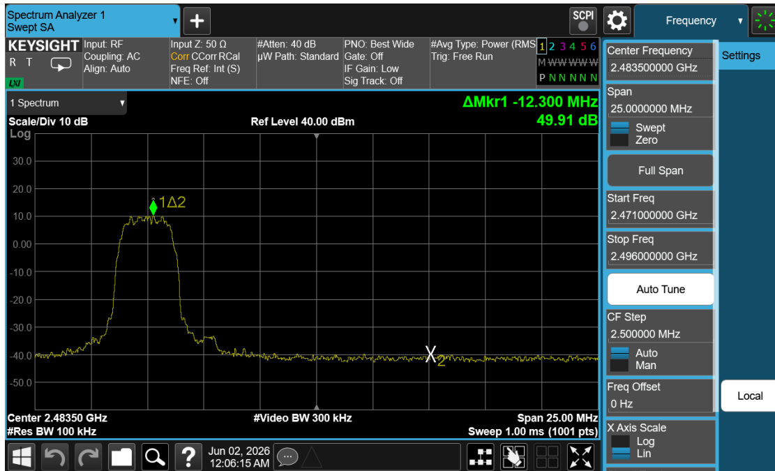
Plot 7-10. Band Edge Plot (Bluetooth (HDR4), ePA – Ch. 73)
