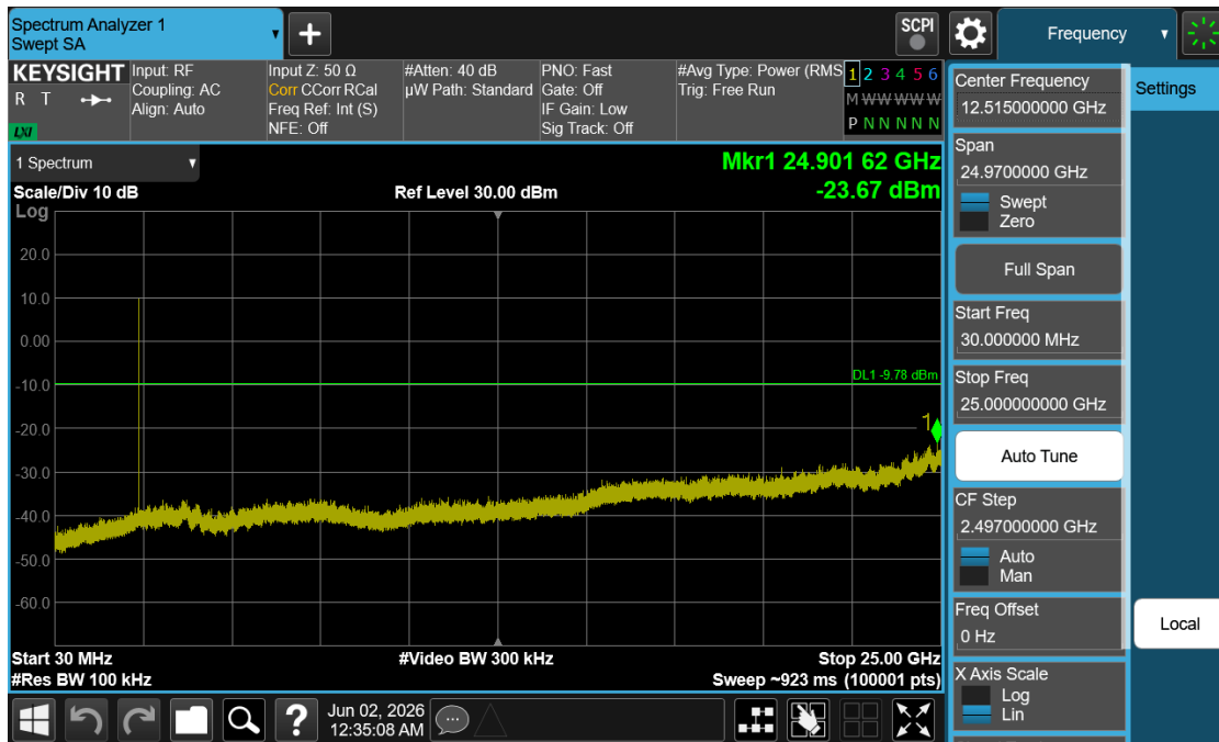
Plot 7-13. Conducted Spurious Plot (Bluetooth (HDR4), 4 Mbps, ePA – Ch. 1)
