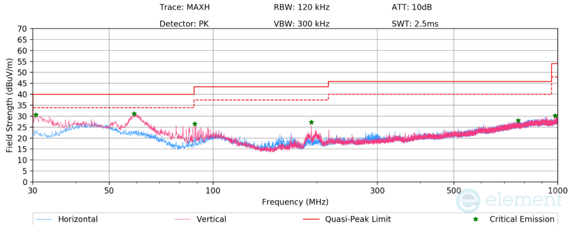
Plot 7-24. Radiated Spurious Emissions Below 1GHz (HDR4, ePA – Ch.38 with AC/DC Adapter)
