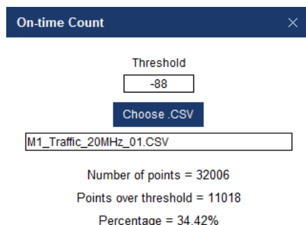
Figure 9-2. 5520MHz - Channel Loading Calculation - (20MHz)
