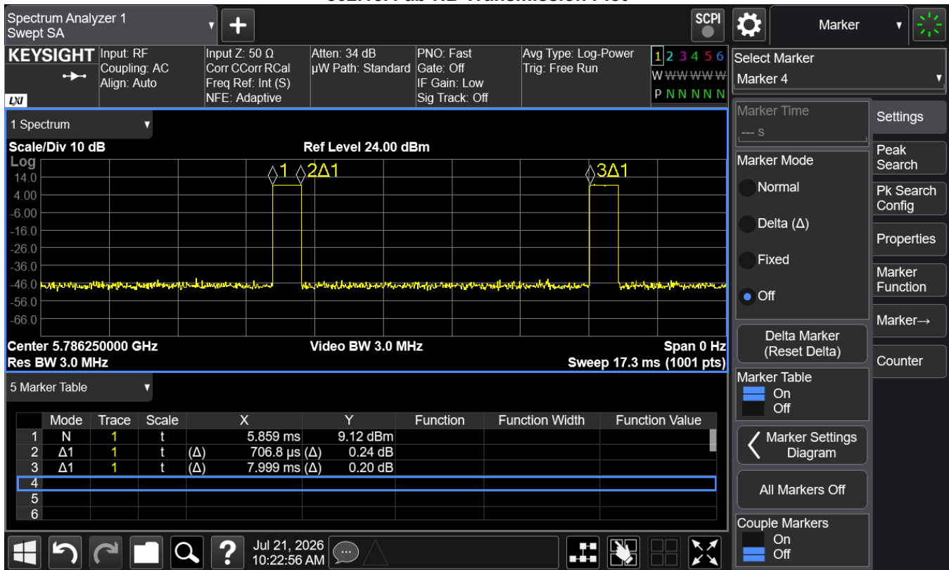
Figure 7-4 802.15.4 ab-NB Transmission Plot
