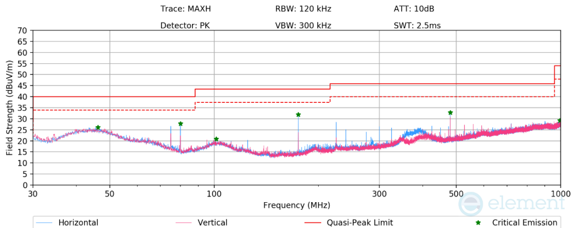
Plot 6-10. Radiated Spurious Emissions 30MHz – 1GHz (Mode 1, with Host Laptop via USB-C Cable)
