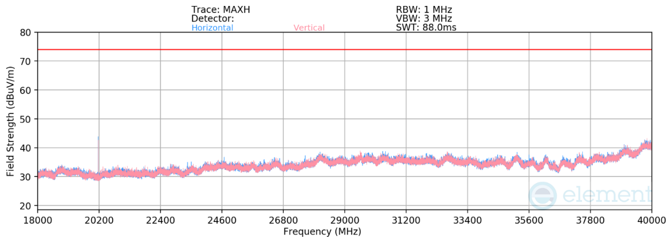
Plot 6-9. Radiated Spurious Emissions 18GHz – 40GHz (Mode 1)
