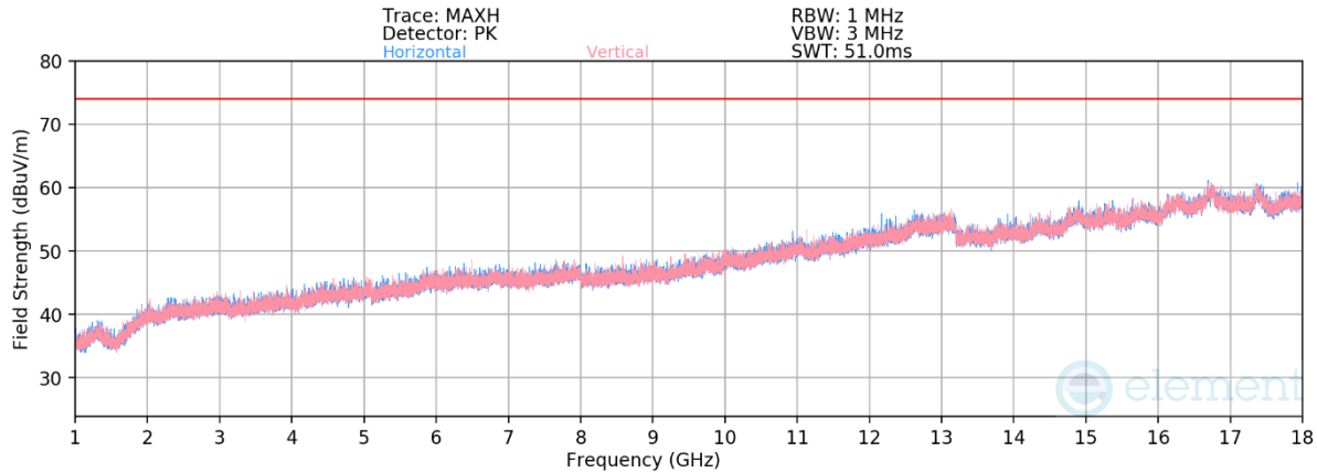
Plot 6-8. Radiated Spurious Emissions 1GHz – 18GHz (Mode 1)
