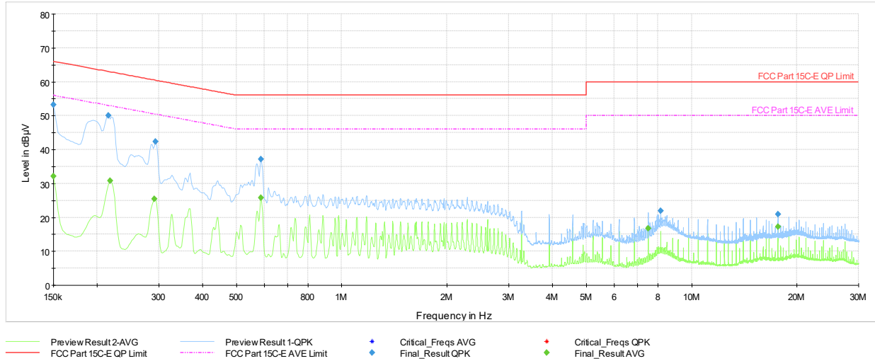
Plot 6-12. AC Line Conducted Plot (N - Mode 1, with Host Laptop via USB-C Cable)
