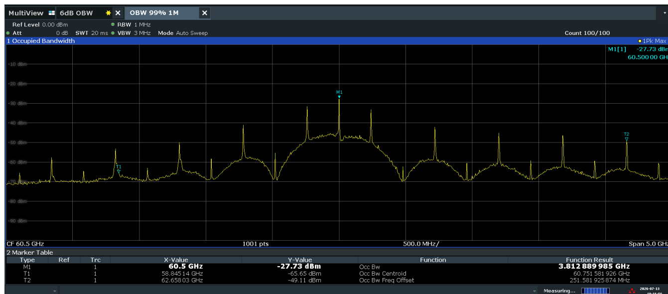
Plot 6-2. 99% Occupied Bandwidth Measurement (Mode 1)
