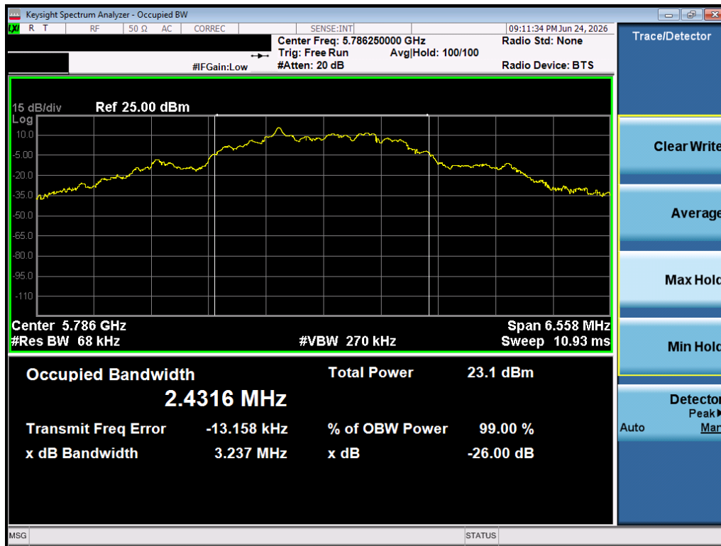
Plot 7-5. 99% OBW (O-QPSK, 5786.25 MHz, 500kbps)
