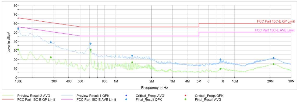
Plot 7-40. AC Line Conducted Plot (O-QPSK, 250Kbps – Ch. 24) (N) with host PC via USB-C cable with magnetic charger
