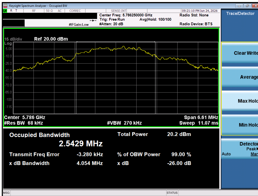
Plot 7-8. 99% OBW (O-QPSK, 5786.25 MHz, 1000kbps)
