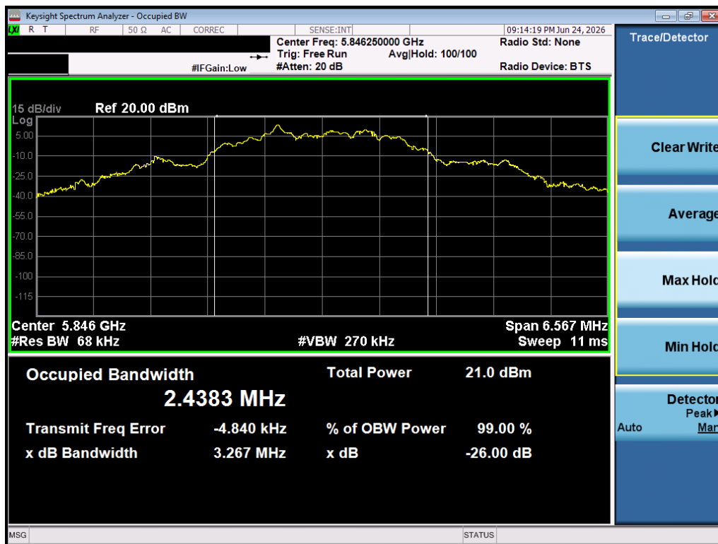
Plot 7-6. 99% OBW (O-QPSK, 5846.25 MHz, 500kbps)
