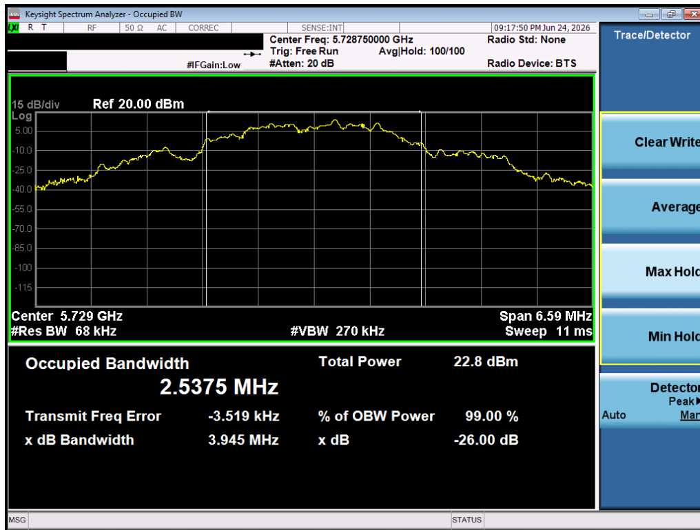
Plot 7-7. 99% OBW (O-QPSK, 5728.75 MHz, 1000kbps)
