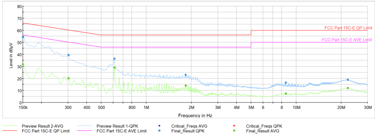
Plot 7-39. AC Line Conducted Plot (O-QPSK, 250Kbps – Ch. 24) (L1) with host PC via USB-C cable with magnetic charger
