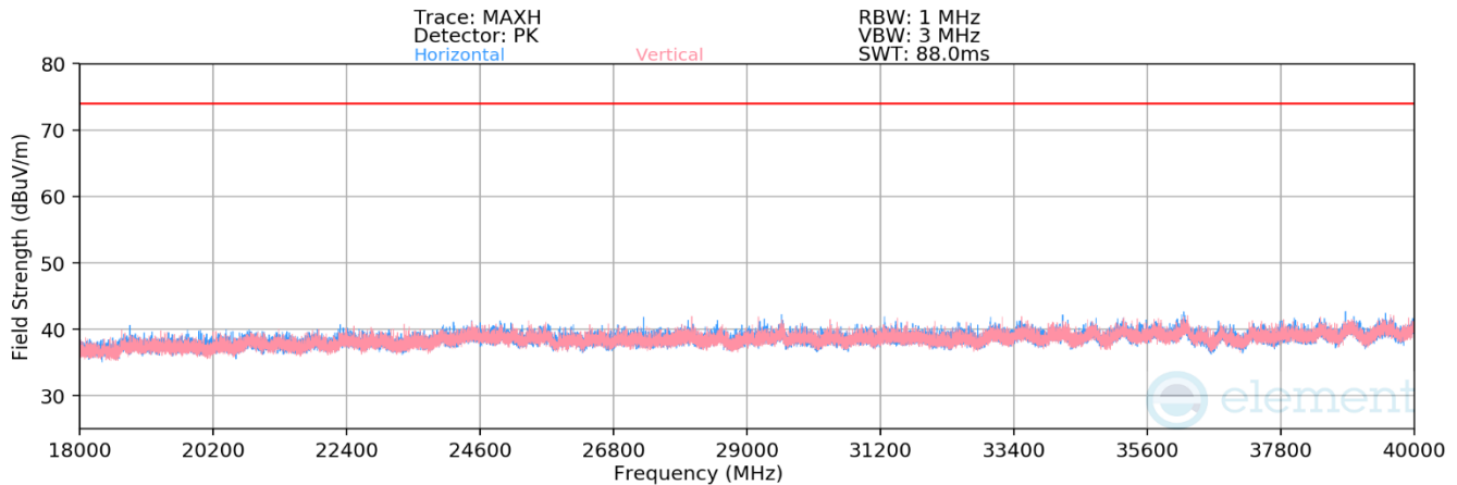
Plot 7-30. Radiated Spurious Emissions Above 18GHz (O-QPSK – 5786.25 MHz)
