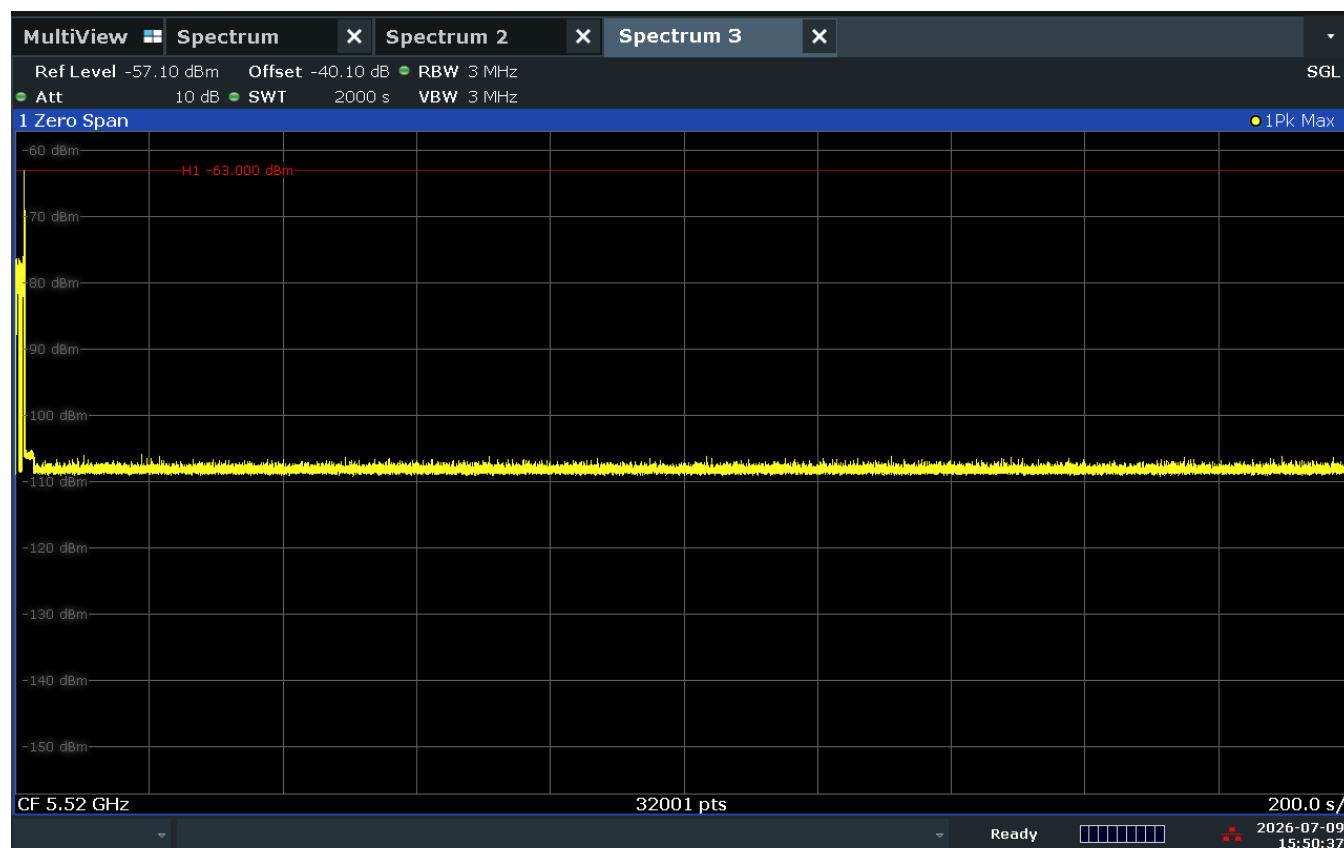
Figure 9-4. 5520MHz - Non-Occupancy Period (30 Minutes) - (20MHz)
