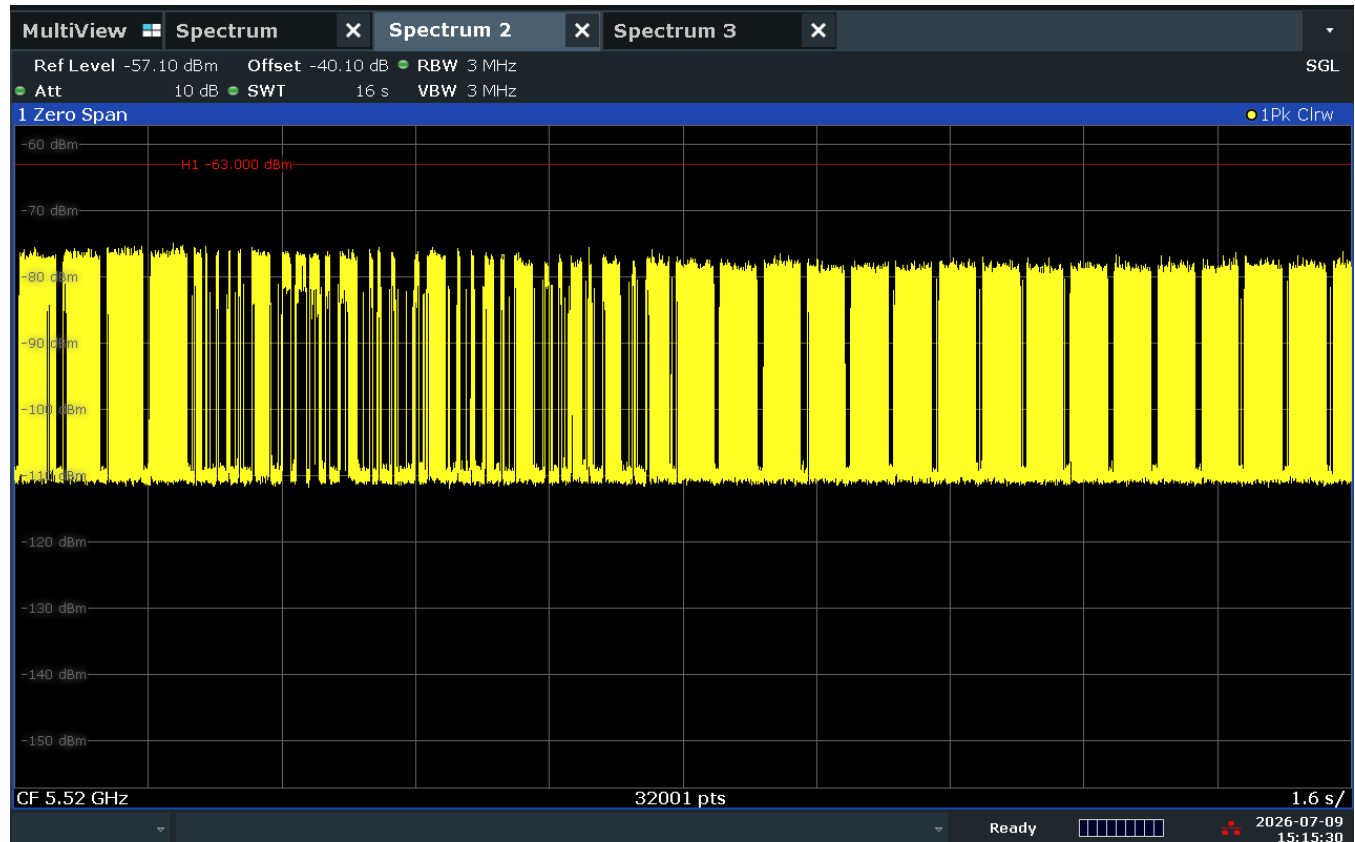
Figure 9-1. 5520MHz - Channel Loading - (20MHz)
