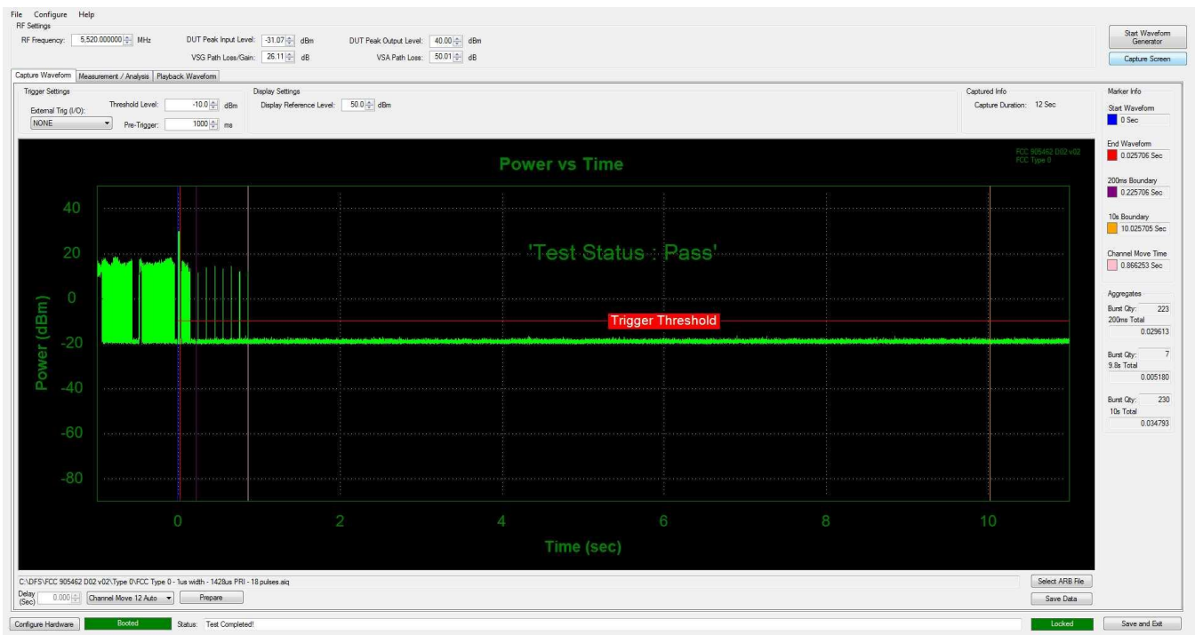
Figure 9-3. 5520MHz - Channel Move/ Closing Transmission Time - (20 MHz)
