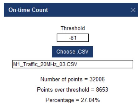
Figure 9-2. 5520MHz - Channel Loading Calculation - (20MHz)
