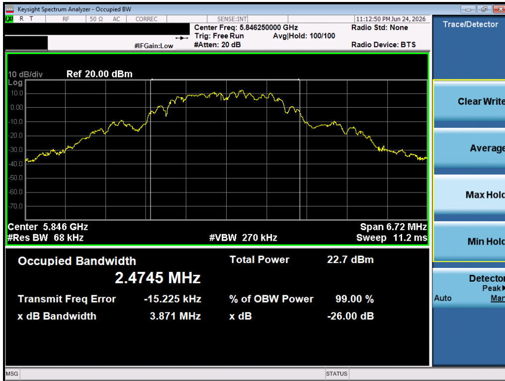
Plot 7-3. 99% OBW (O-QPSK, 5846.25MHz, 250kbps)
