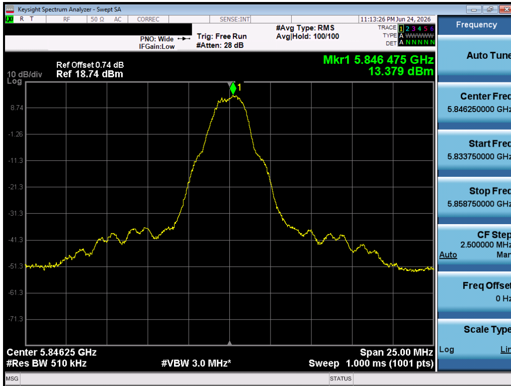
Plot 7-21. PSD (O-QPSK, 5846.25MHz, 250kbps)
