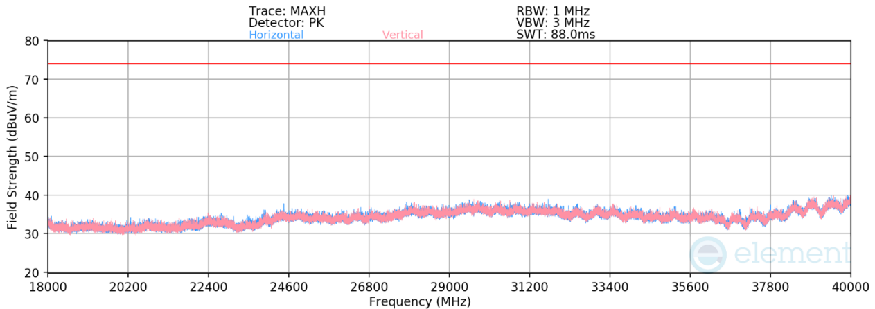
Plot 7-31. Radiated Spurious Emissions Above 18GHz (O-QPSK – 5846.25MHz)
