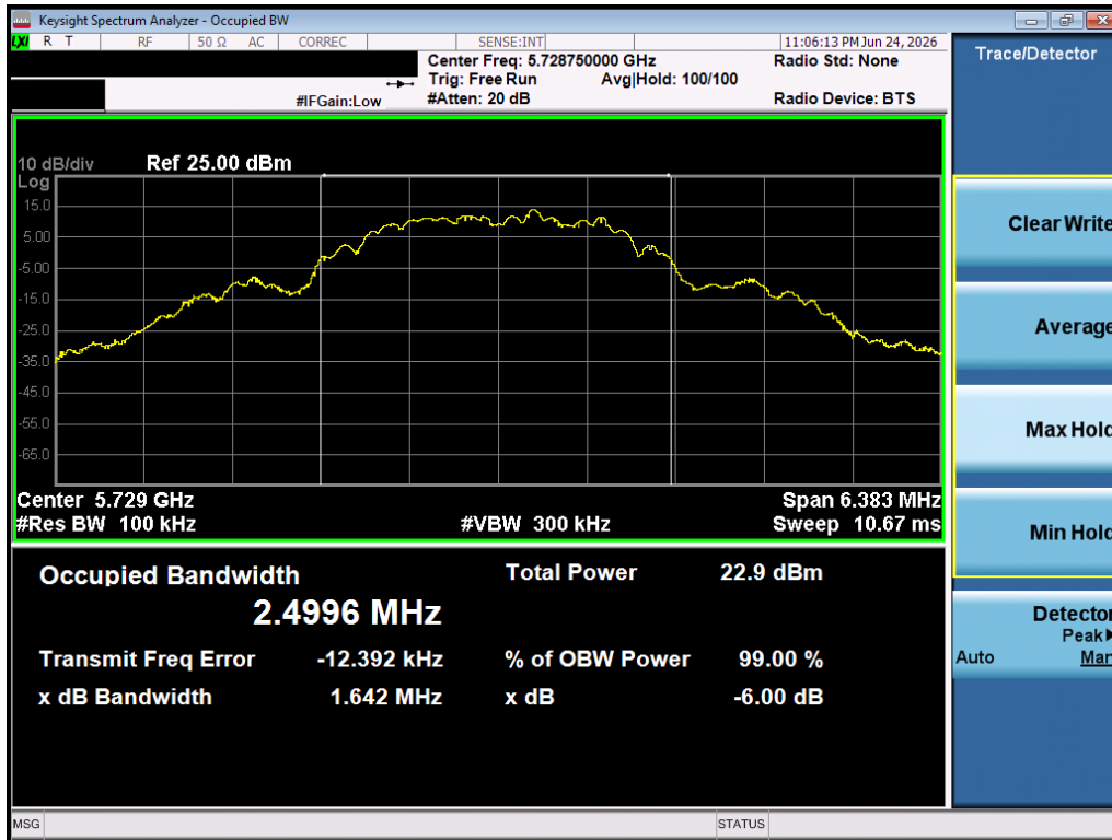
Plot 7-10. 6dB BW (O-QPSK, 5728.75MHz, 250kbps)
