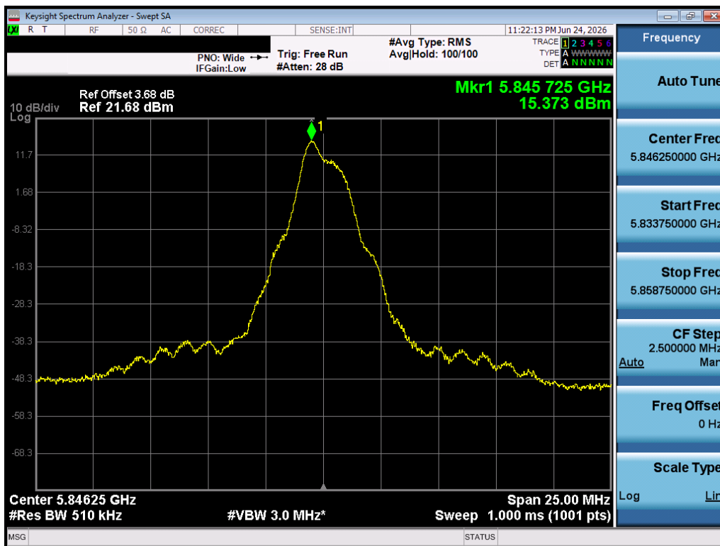
Plot 7-24. PSD (O-QPSK, 5846.25MHz, 500kbps)
