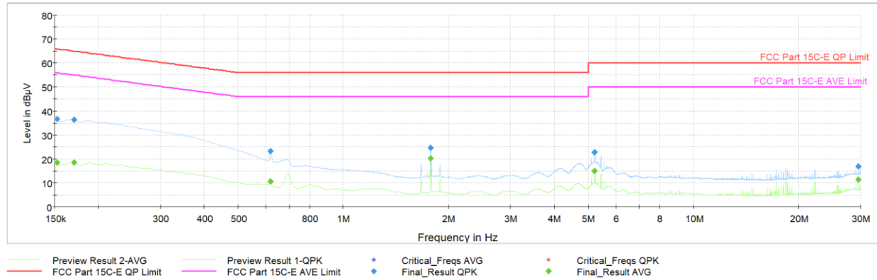
Plot 7-40. AC Line Conducted Plot (O-QPSK, 250Kbps – Ch. 48) (N) with AC/DC Adapter & magnetic charger
