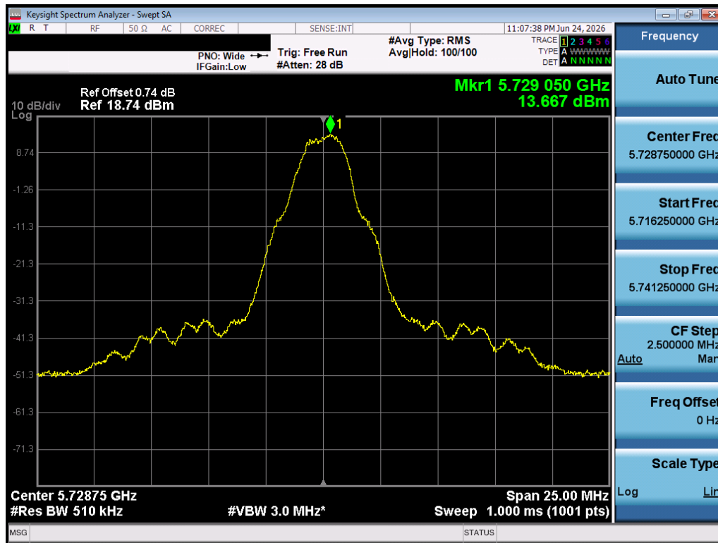
Plot 7-19. PSD (O-QPSK, 5728.75MHz, 250kbps)
