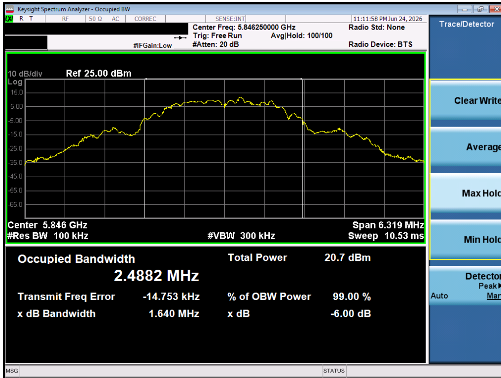
Plot 7-12. 6dB BW (O-QPSK, 5846.25MHz, 250kbps)
