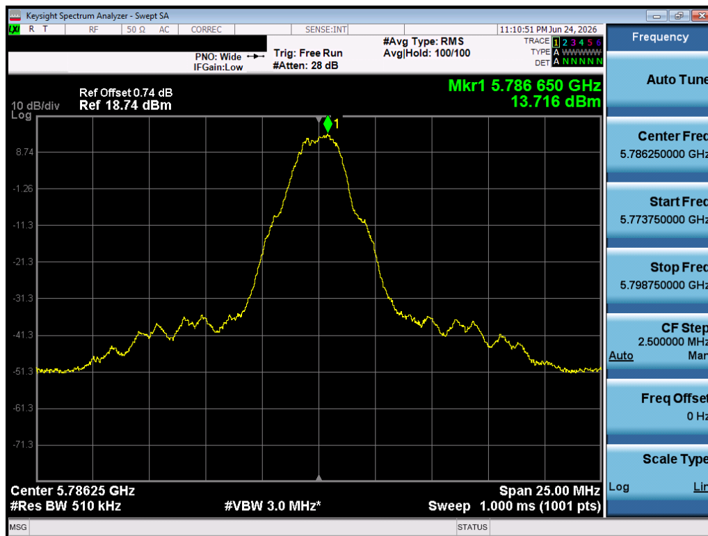
Plot 7-20. PSD (O-QPSK, 5786.25MHz, 250kbps)
