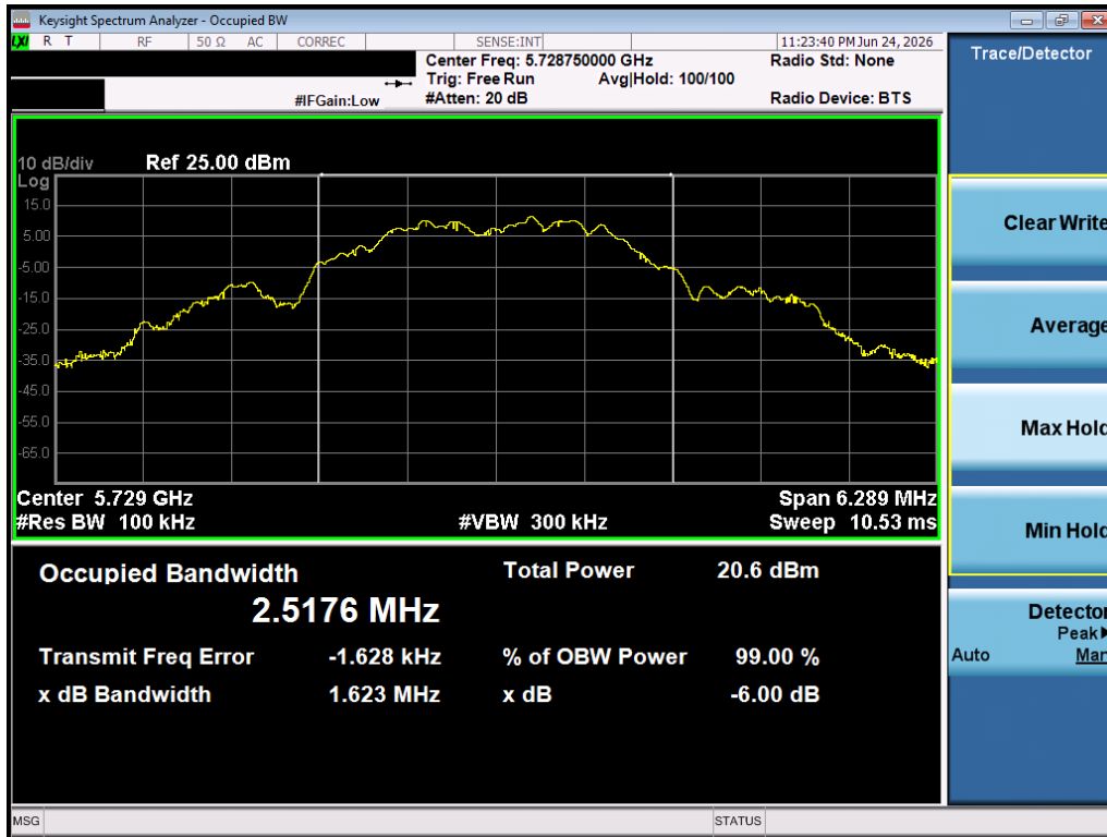
Plot 7-16. 6dB BW (O-QPSK, 5728.75MHz, 1000kbps)
