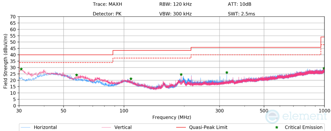
Plot 7-38. RSE 30MHz - 1GHz (O-QPSK, 250Kbps – Ch. 48), with AC/DC Adapter & magnetic charger
