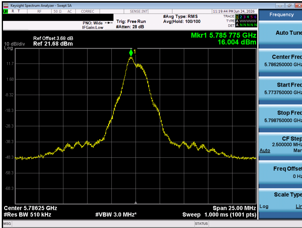
Plot 7-23. PSD (O-QPSK, 5786.25MHz, 500kbps)
