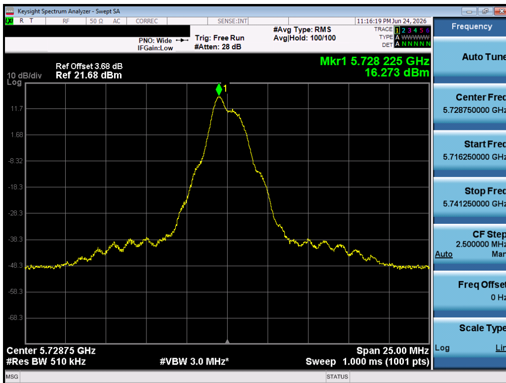
Plot 7-22. PSD (O-QPSK, 5728.75MHz, 500kbps)
