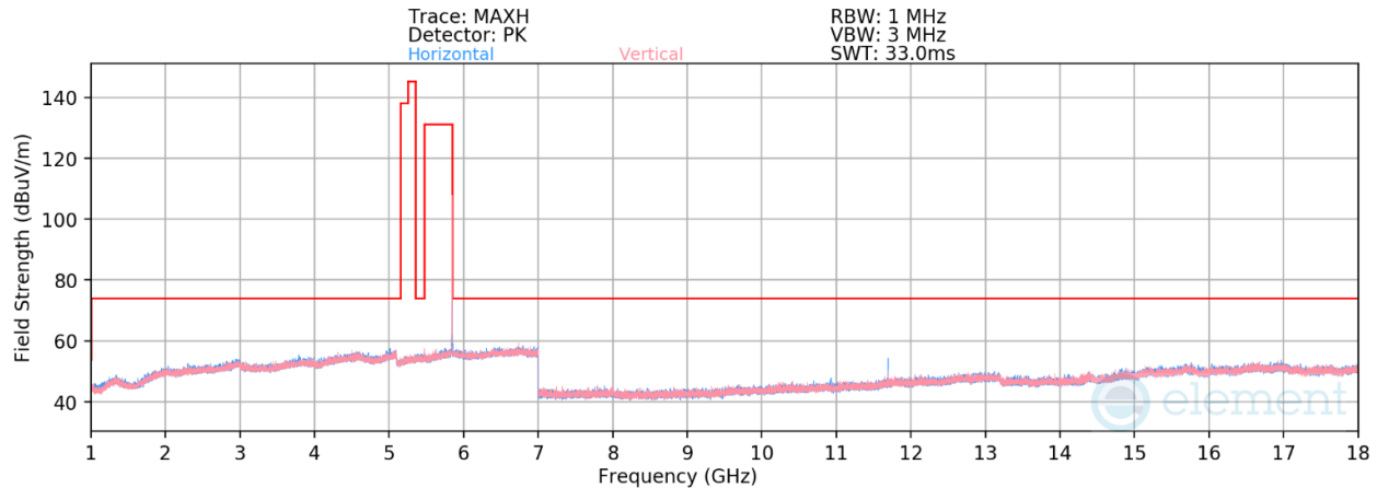
Plot 7-30. Radiated Spurious Emissions 1-18GHz (O-QPSK – 5846.25MHz)
