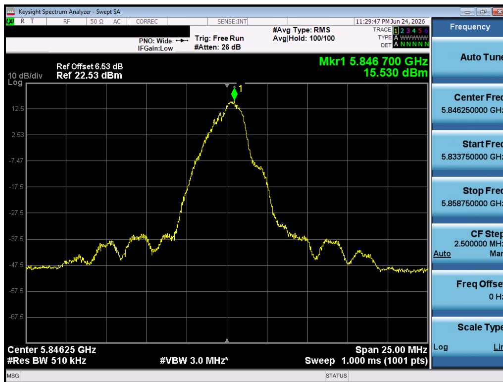
Plot 7-27. PSD (O-QPSK, 5846.25MHz, 1000kbps)
