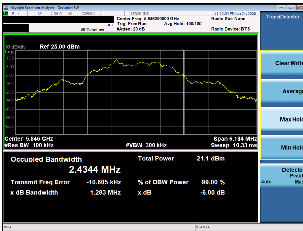
Plot 7-15. 6dB BW (O-QPSK, 5846.25MHz, 500kbps)
