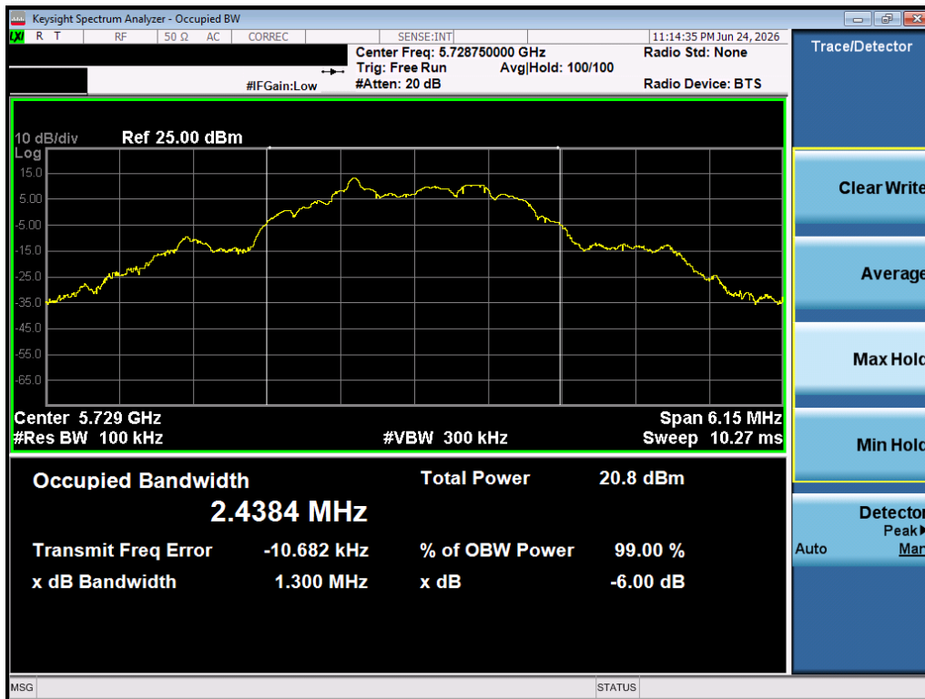
Plot 7-13. 6dB BW (O-QPSK, 5728.75MHz, 500kbps)
