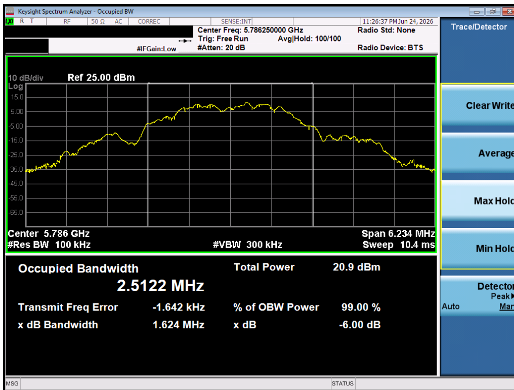
Plot 7-17. 6dB BW (O-QPSK, 5786.25MHz, 1000kbps)
