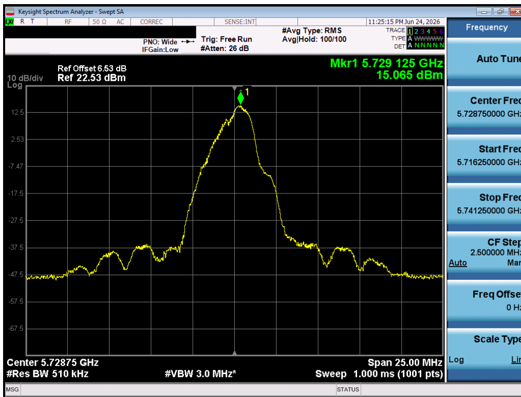
Plot 7-25. PSD (O-QPSK, 5728.75MHz, 1000kbps)
