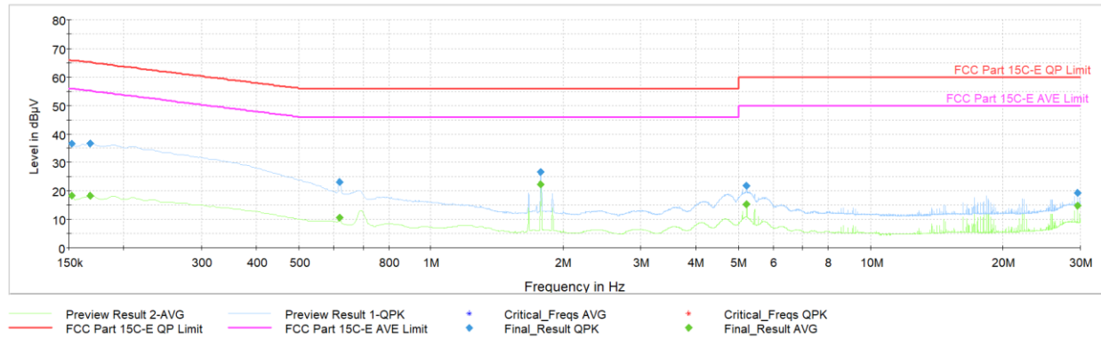
Plot 7-39. AC Line Conducted Plot (O-QPSK, 250Kbps – Ch. 48) (L1) with AC/DC Adapter & magnetic charger
