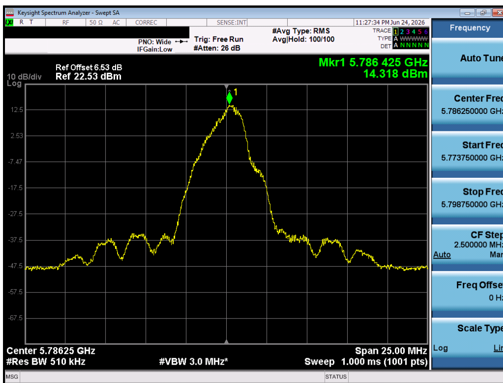
Plot 7-26. PSD (O-QPSK, 5786.25MHz, 1000kbps)
