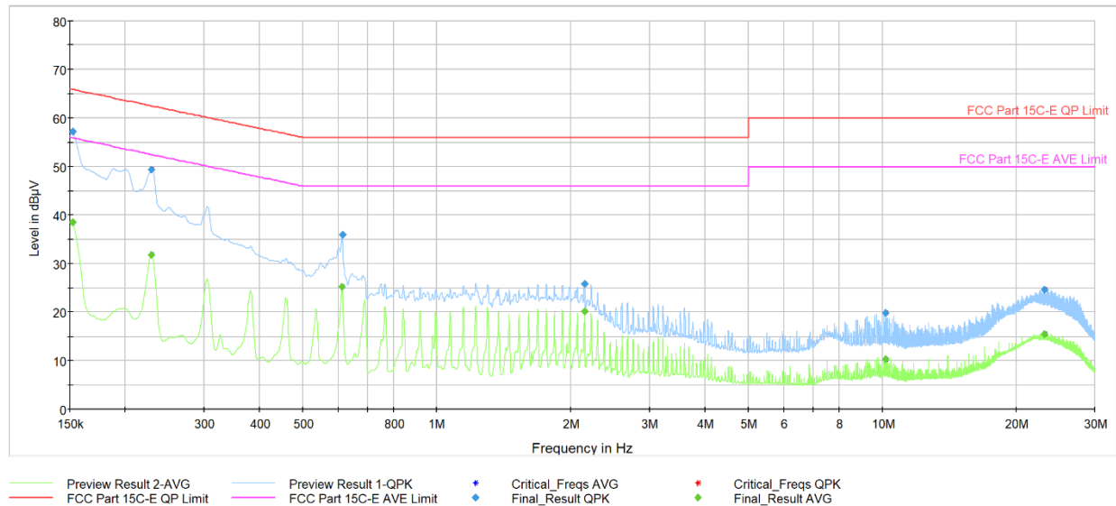
Plot 7-39. AC Line Conducted Plot (O-QPSK, 250Kbps – Ch. 24) (L1) with host PC via USB-C cable with magnetic charger
