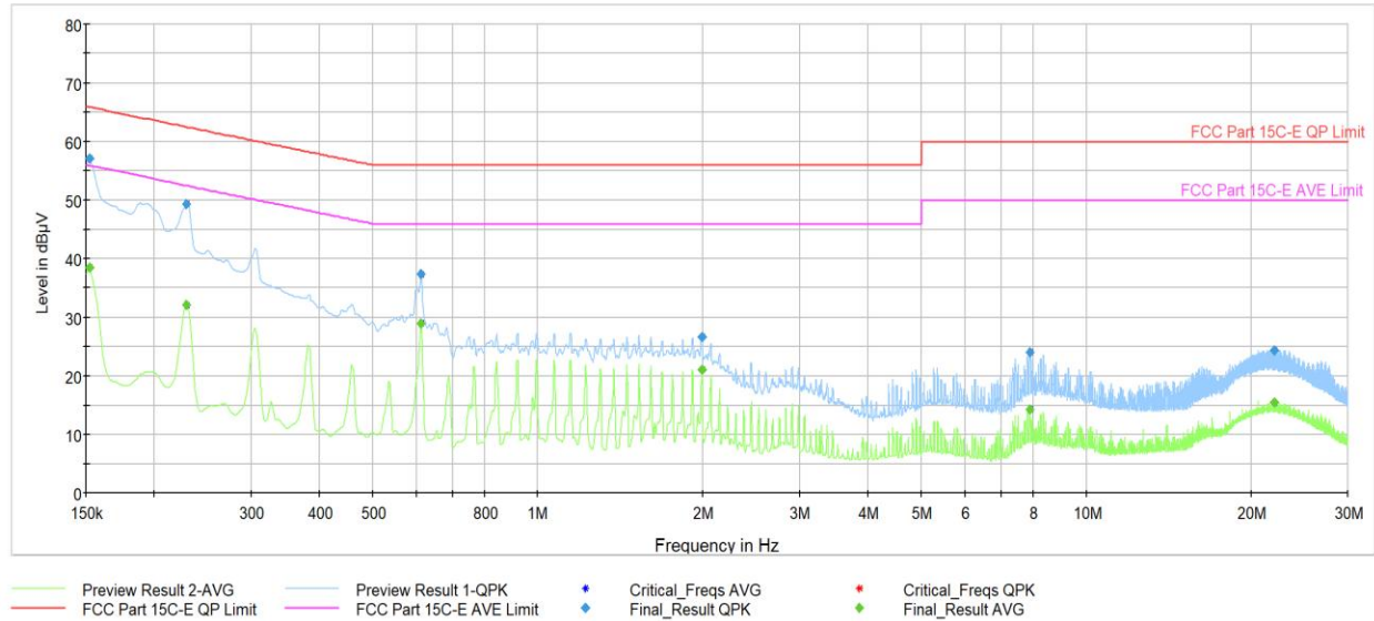
Plot 7-40. AC Line Conducted Plot (O-QPSK, 250Kbps – Ch. 24) (N) with host PC via USB-C cable with magnetic charger
