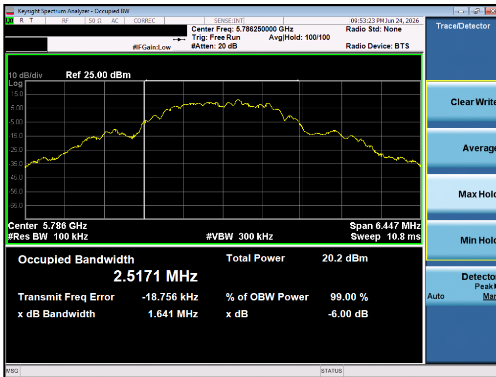
Plot 7-11. 6dB BW (O-QPSK, 5786.25 MHz, 250kbps)
