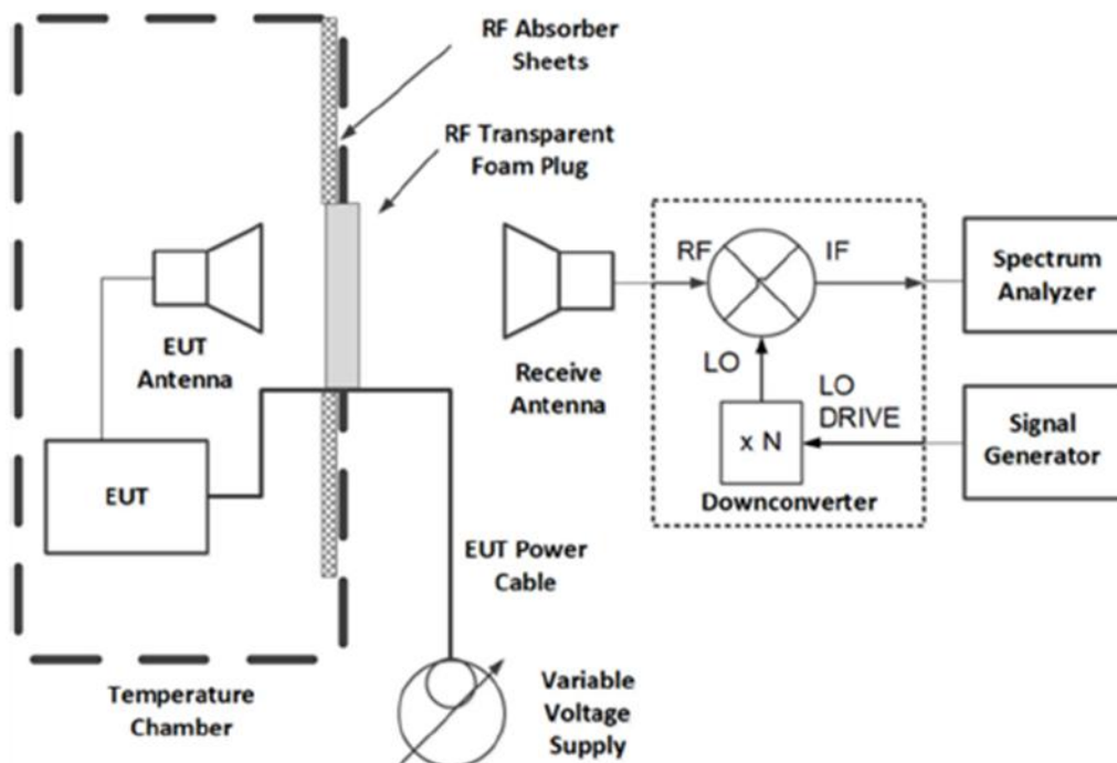
Figure 6-8. Frequency Stability Test Instrument & Measurement Setup
