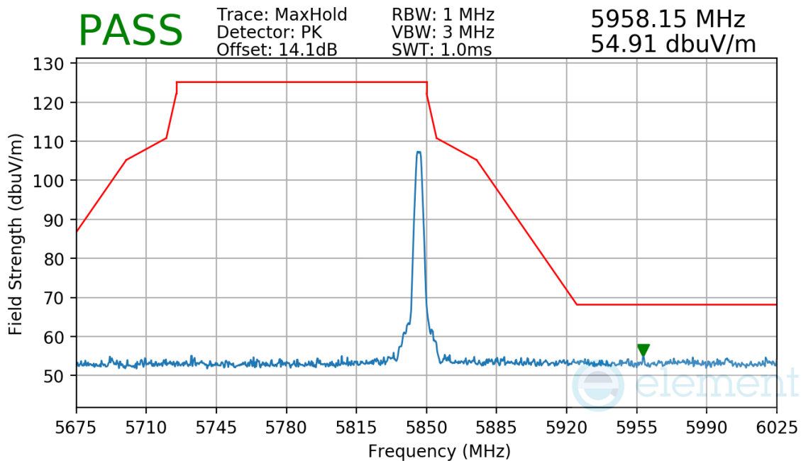
Plot 7-37. Radiated Upper Band Edge Measurement (Pk, Ch. 48, O-QPSK, 1000Kbps)
