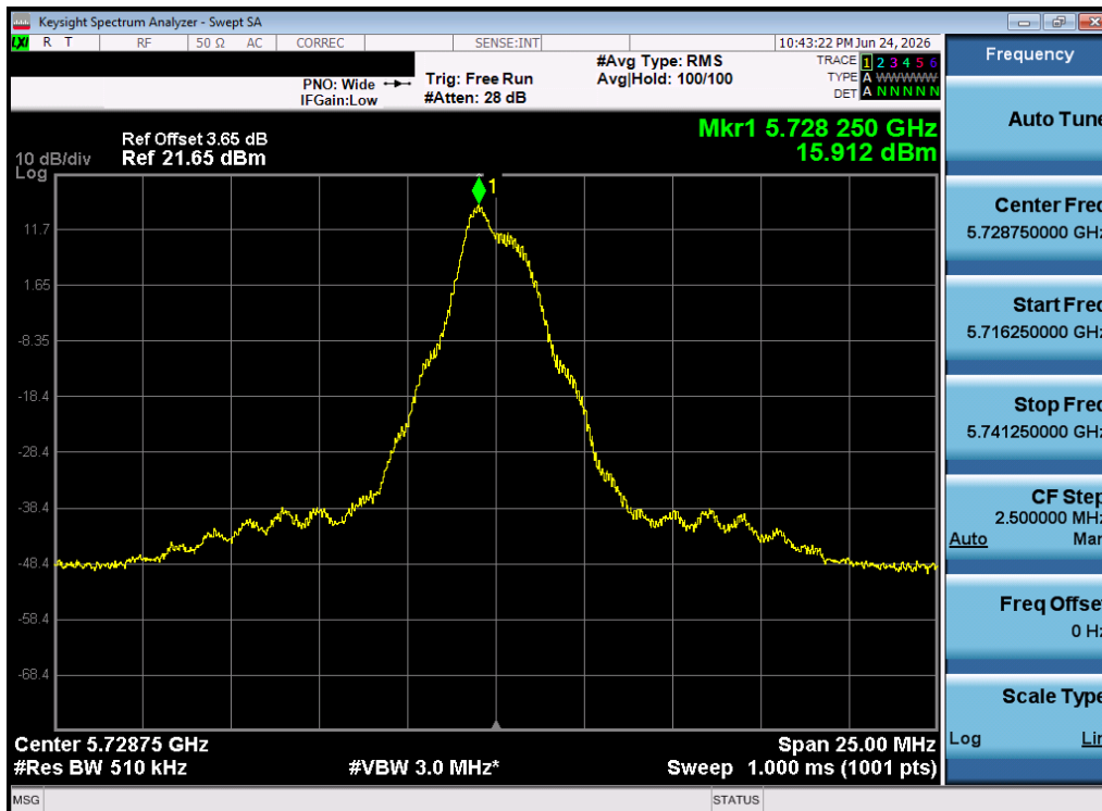
Plot 7-22. PSD (O-QPSK, 5728.75 MHz, 500kbps)
