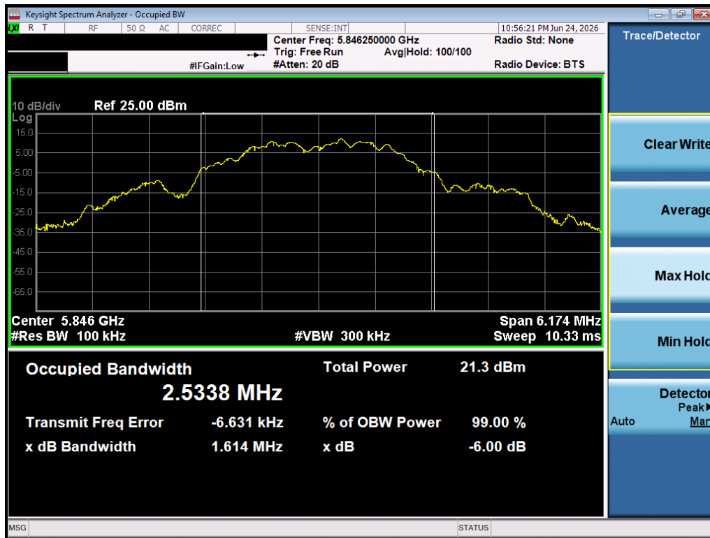
Plot 7-18. 6dB BW (O-QPSK, 5846.25 MHz, 1000kbps)
