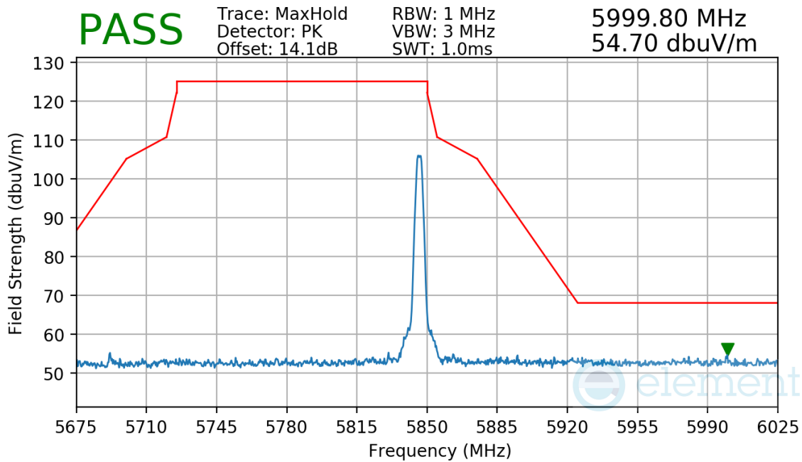
Plot 7-35. Radiated Upper Band Edge Measurement (Pk, Ch. 48, O-QPSK, 500Kbps)
