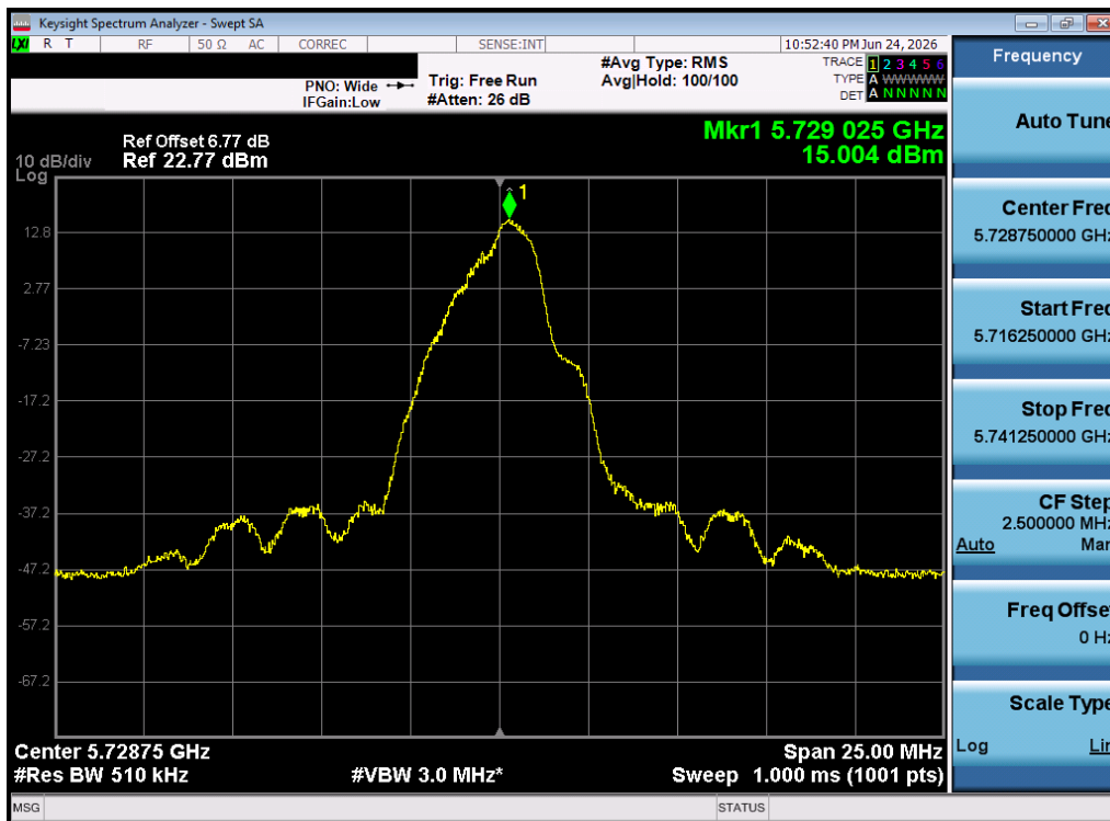
Plot 7-25. PSD (O-QPSK, 5728.75 MHz, 1000kbps)
