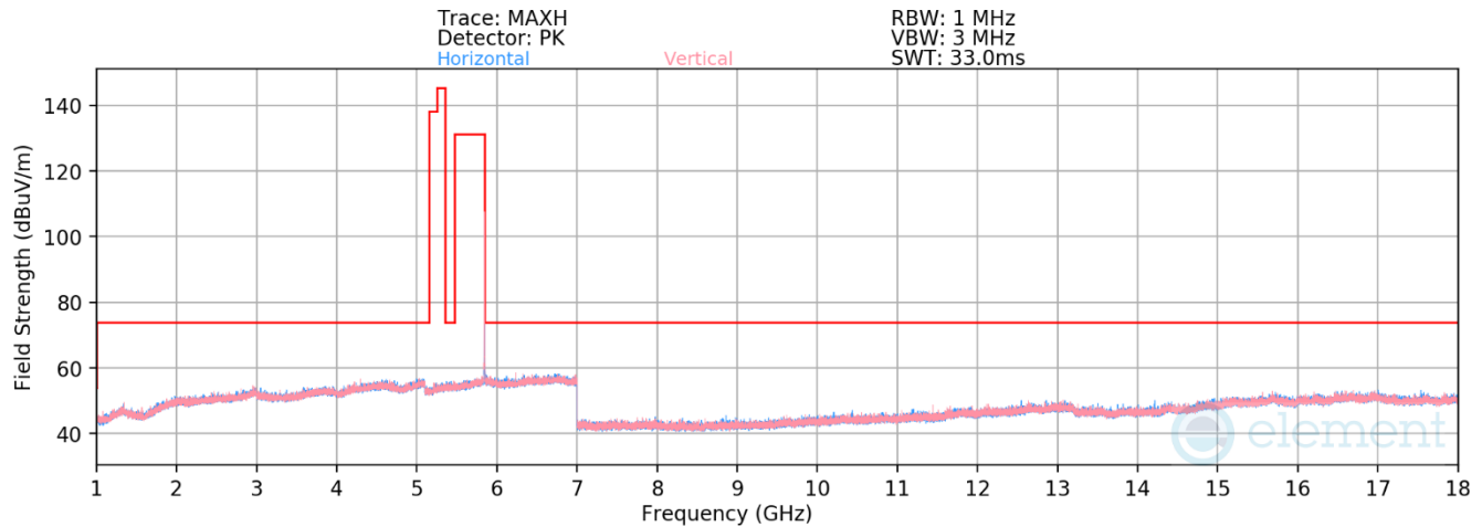
Plot 7-31. Radiated Spurious Emissions 1-18GHz (O-QPSK – 5846.25 MHz)
