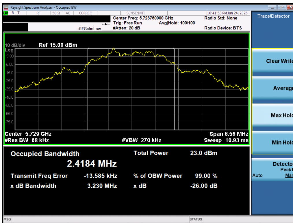
Plot 7-4. 99% OBW (O-QPSK, 5728.75 MHz, 500kbps)
