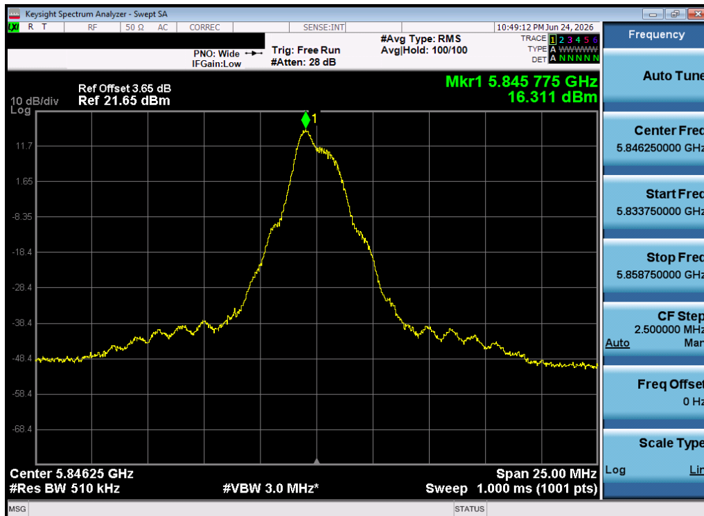
Plot 7-24. PSD (O-QPSK, 5846.25 MHz, 500kbps)
