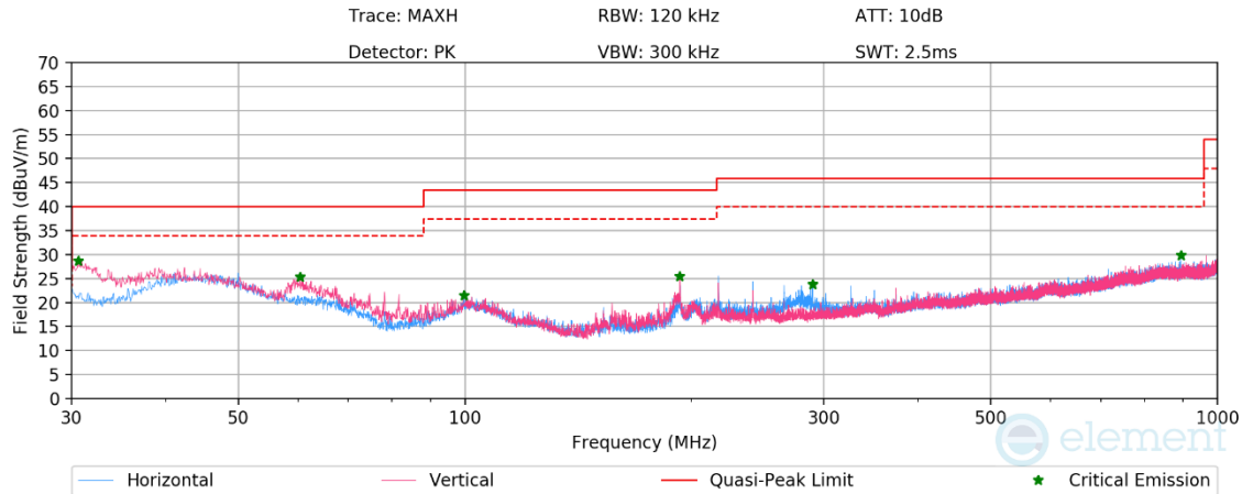
Plot 7-38. RSE 30 MHz – 1 GHz (O-QPSK, 250Kbps – Ch. 24), with AC/DC Adapter & magnetic charger
