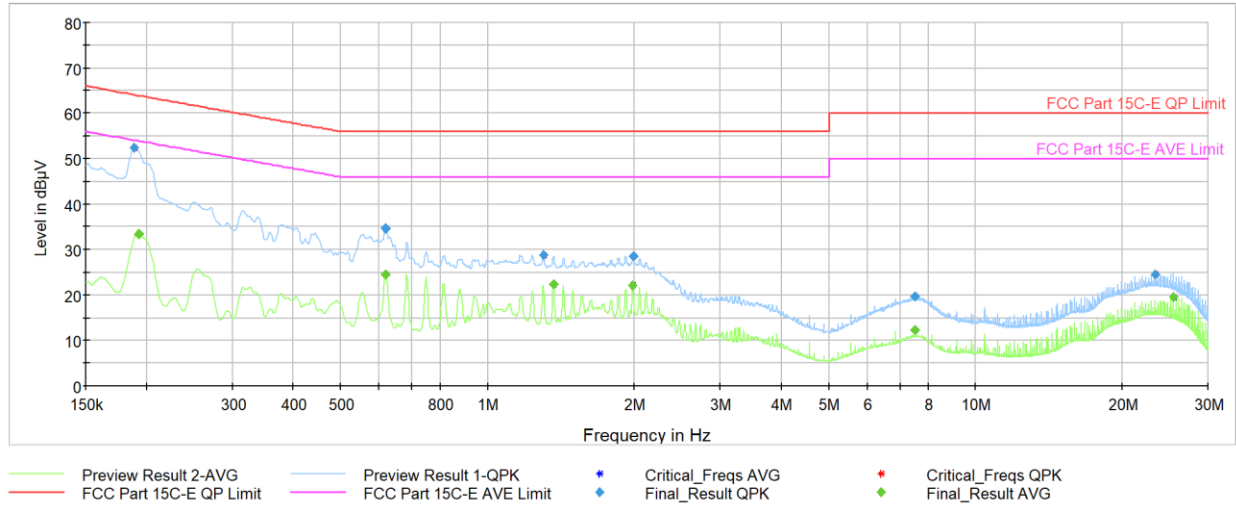
Plot 7-40. AC Line Conducted Plot (O-QPSK, 250Kbps – Ch. 24) (N) with host PC via USB-C cable with magnetic charger
