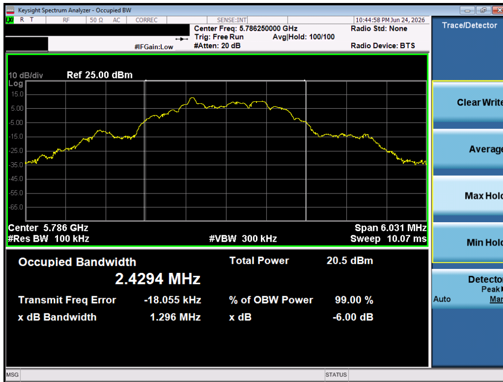
Plot 7-14. 6dB BW (O-QPSK, 5786.25 MHz, 500kbps)
