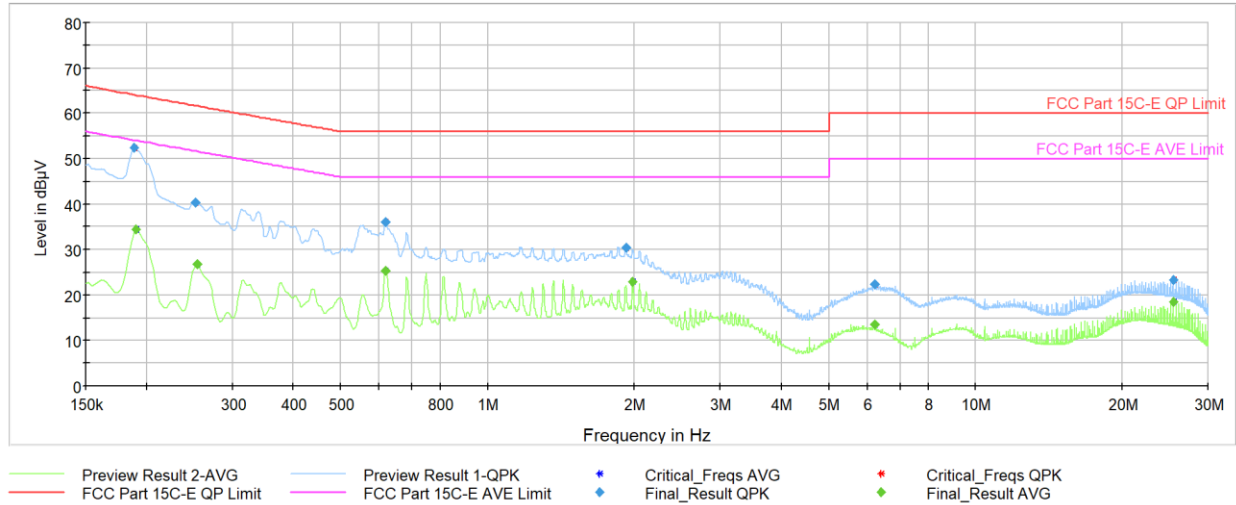
Plot 7-39. AC Line Conducted Plot (O-QPSK, 250Kbps – Ch. 24) (L1) with host PC via USB-C cable with magnetic charger
