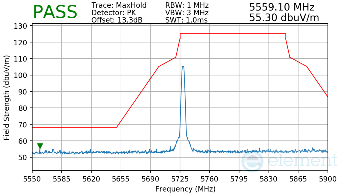
Plot 7-32. Radiated Lower Band Edge Measurement (Pk, Ch. 1, O-QPSK, 250Kbps)
