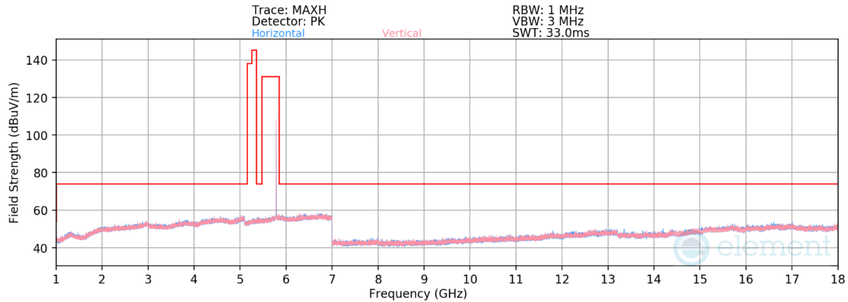
Plot 7-29. Radiated Spurious Emissions 1-18GHz (O-QPSK – 5786.25 MHz)
