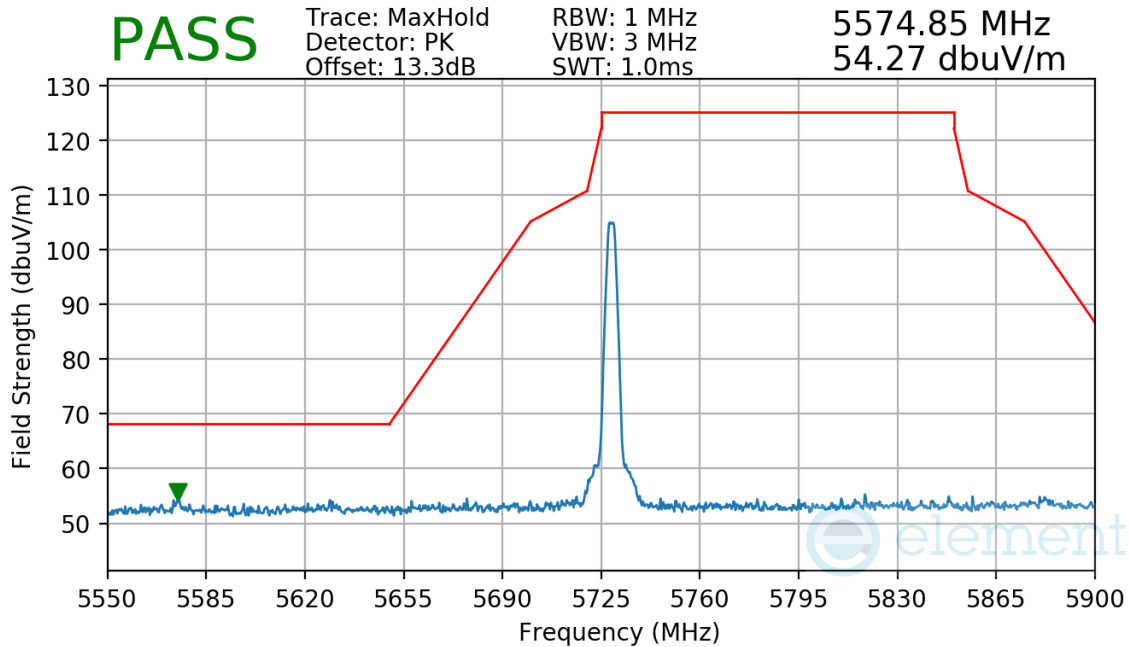
Plot 7-34. Radiated Lower Band Edge Measurement (Pk, Ch. 1, O-QPSK, 500Kbps)
