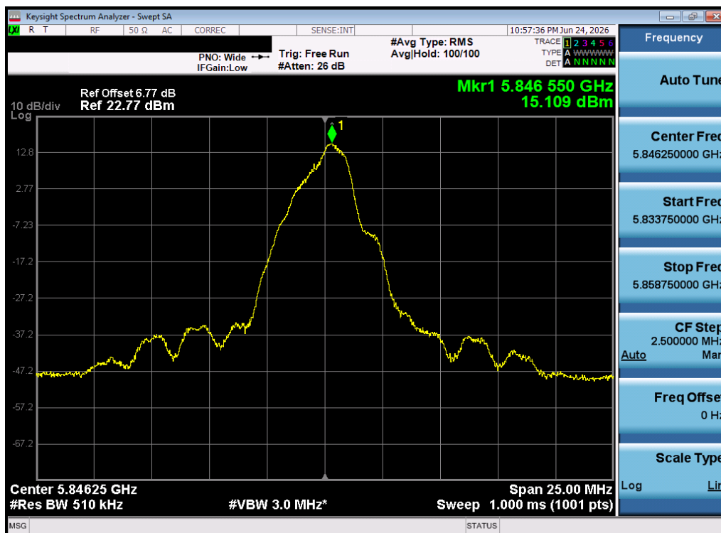
Plot 7-27. PSD (O-QPSK, 5846.25 MHz, 1000kbps)
