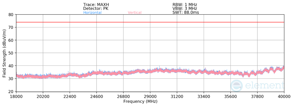
Plot 7-30. Radiated Spurious Emissions Above 18GHz (O-QPSK – 5786.25 MHz)
