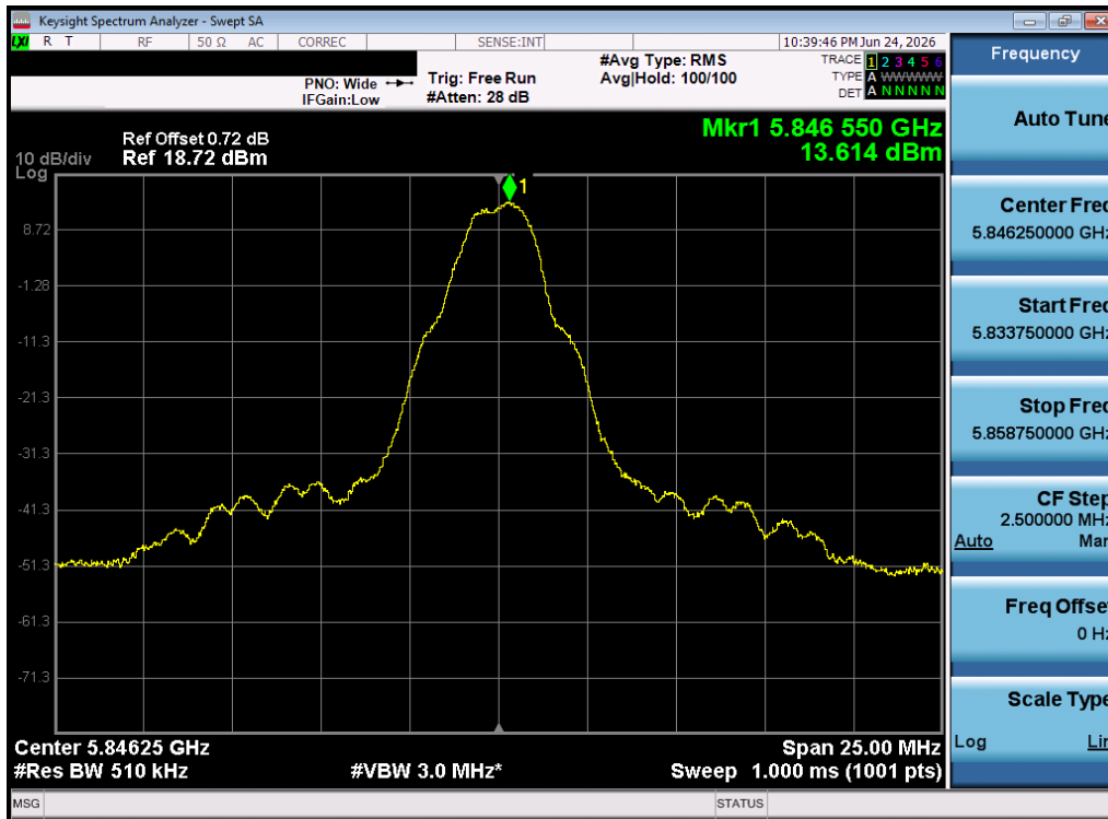
Plot 7-21. PSD (O-QPSK, 5846.25 MHz, 250kbps)
