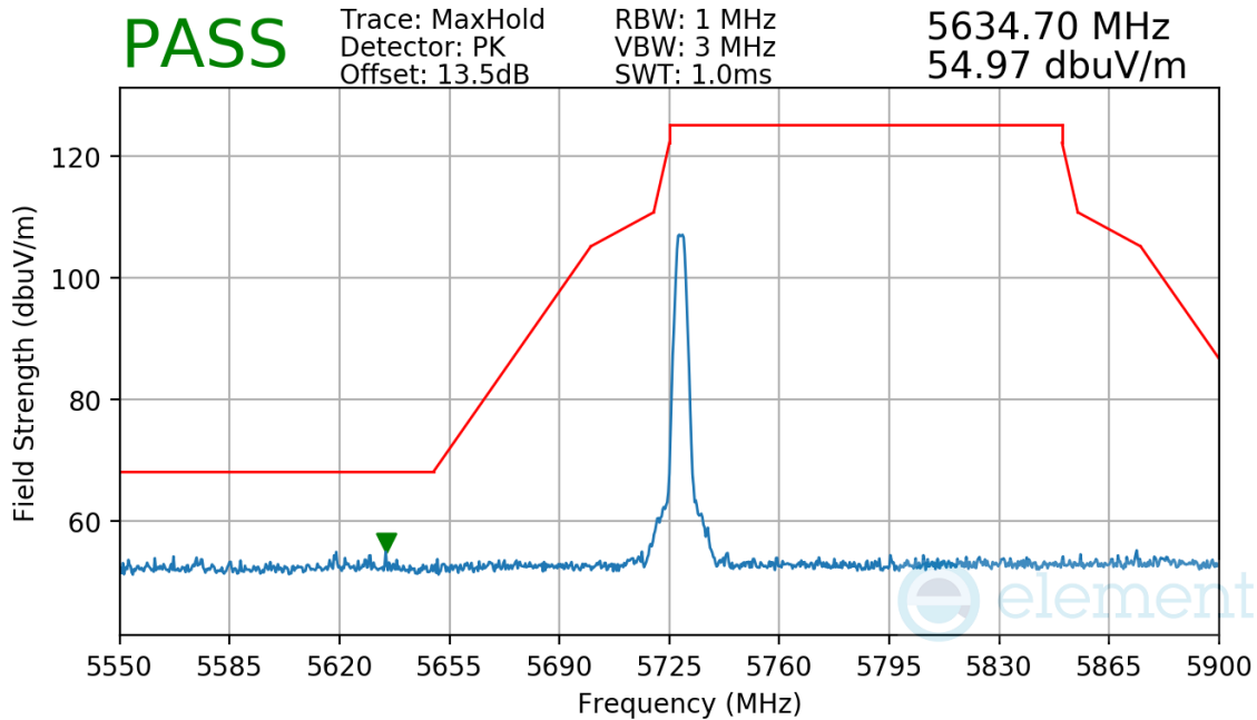
Plot 7-36. Radiated Lower Band Edge Measurement (Pk, Ch. 1, O-QPSK, 1000Kbps)
