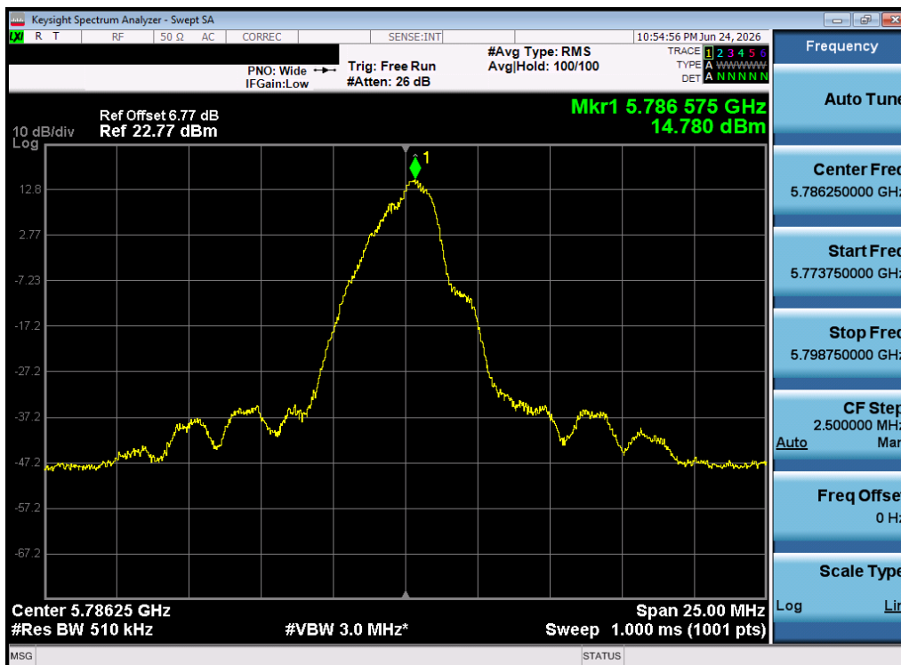
Plot 7-26. PSD (O-QPSK, 5786.25 MHz, 1000kbps)
