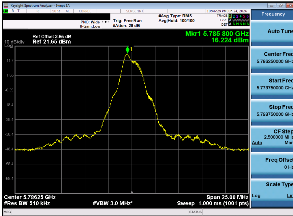
Plot 7-23. PSD (O-QPSK, 5786.25 MHz, 500kbps)
