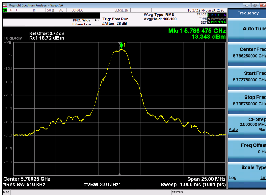
Plot 7-20. PSD (O-QPSK, 5786.25 MHz, 250kbps)
