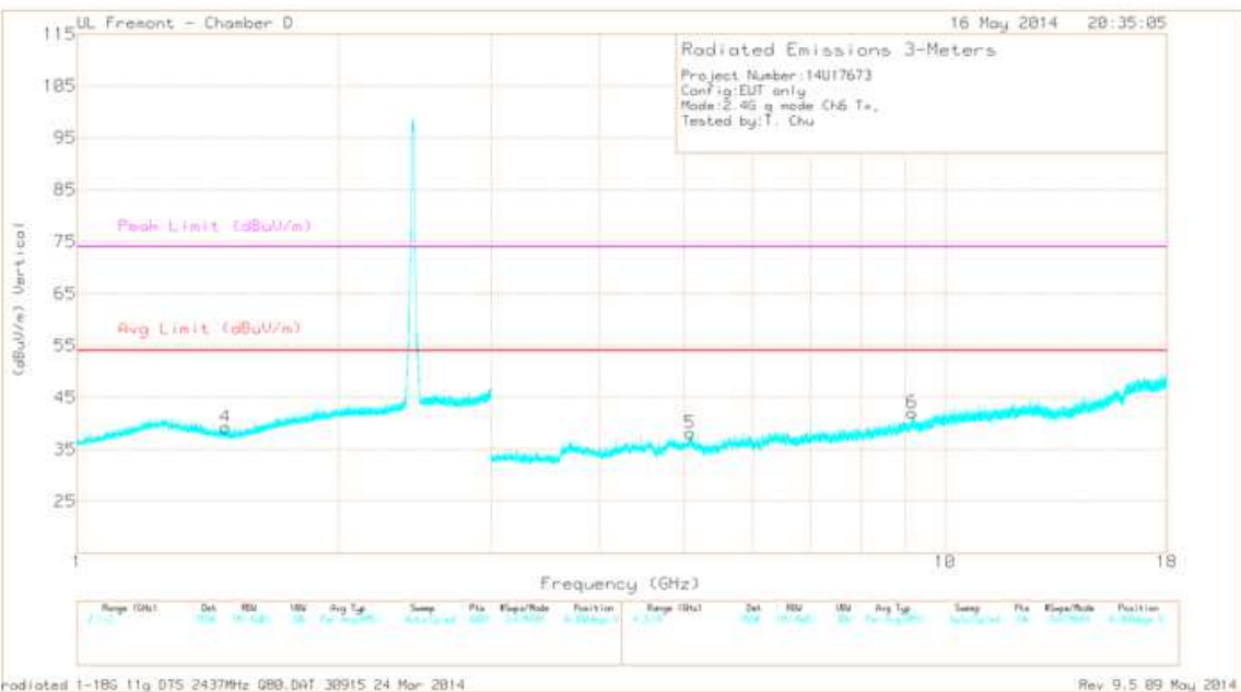
MID CHANNEL VERTICAL PLOT, CH 6
