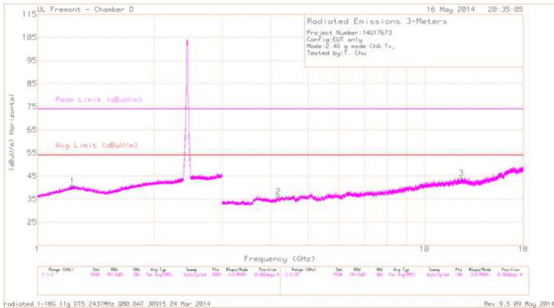
MID CHANNEL HORIZONTAL PLOT, CH 6
