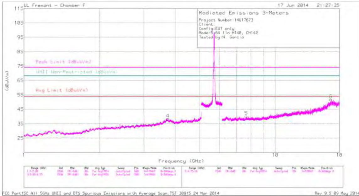
HIGH CHANNEL HORIZONTAL PLOT, CH 142
