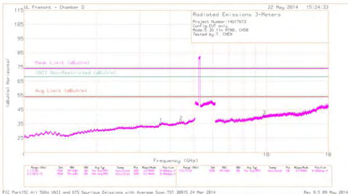
HIGH CHANNEL HORIZONTAL PLOT, CH 58
