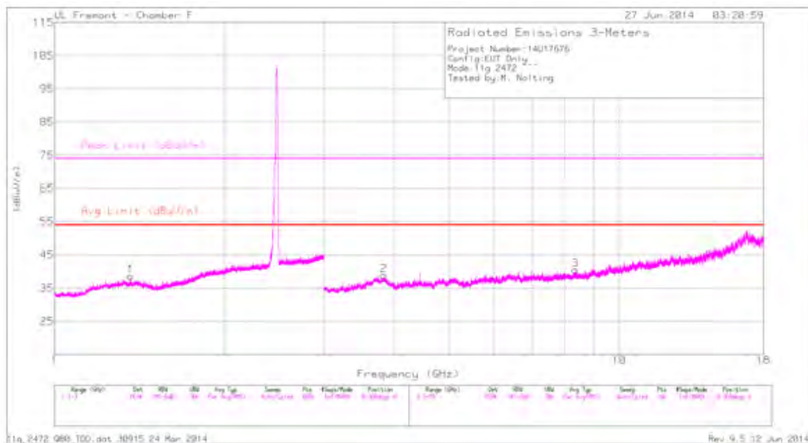
HIGH CHANNEL HORIZONTAL PLOT, CH 13
