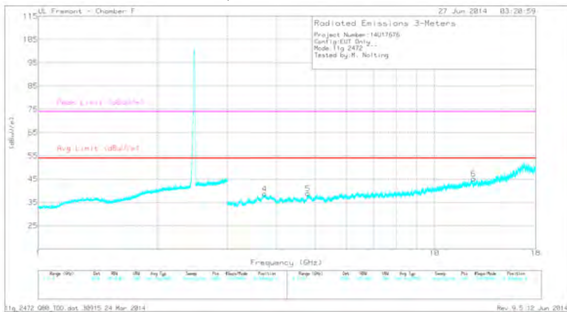
HIGH CHANNEL VERTICAL PLOT, CH 13
