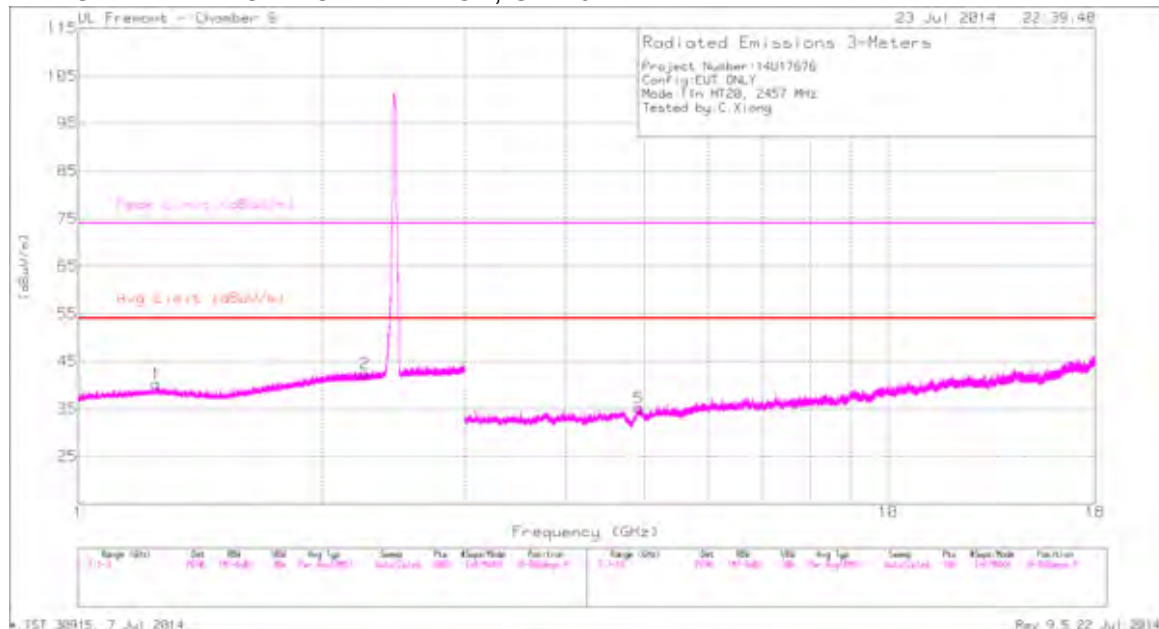
MID CHANNEL HORIZONTAL PLOT, CH 10
