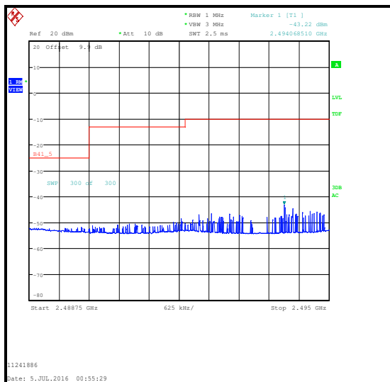
16QAM / 1 RB 24 Offset / 2488.75 to 2495 MHz **See note 8
