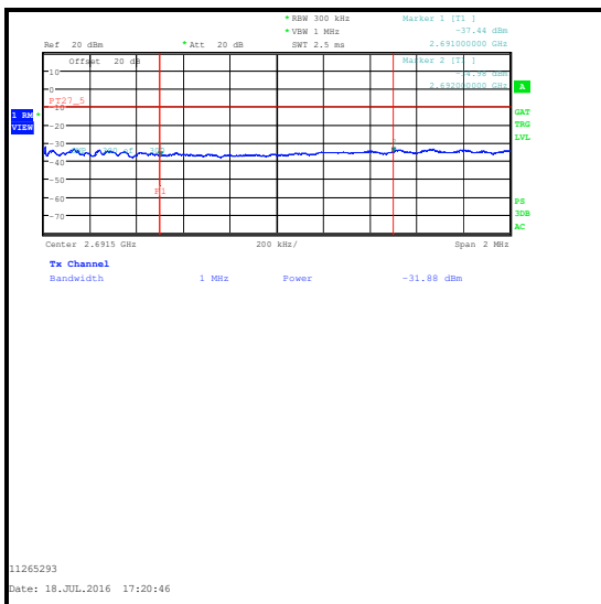
QPSK / 75 RB 0 Offset / 2691 to 2692 MHz / Integrated level
