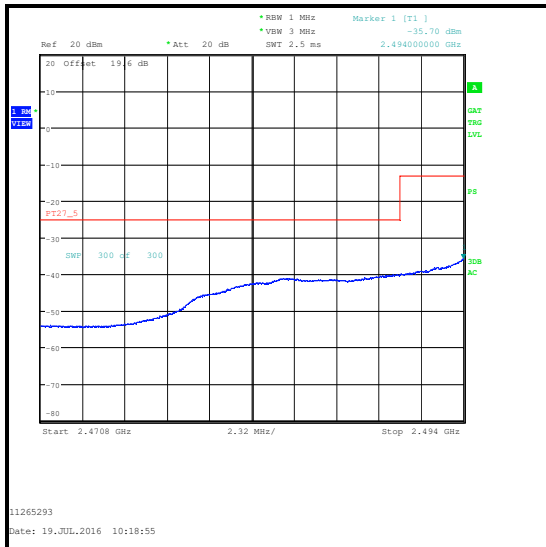
QPSK / 100 RB 0 Offset / 2470.8 to 2494 MHz
