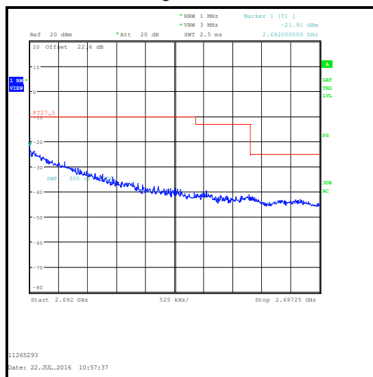
16QAM / 25 RB 0 Offset / 2692 to 2697.25 MHz
