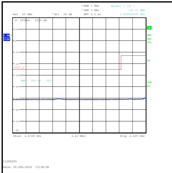
QPSK / 1 RB 99 Offset / 2470.8 to 2495 MHz
