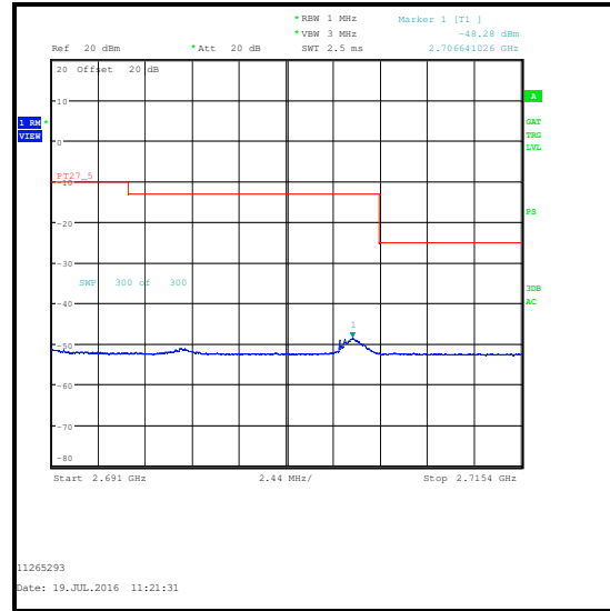
16QAM / 1 RB 0 Offset / 2691 to 2715.4 MHz
