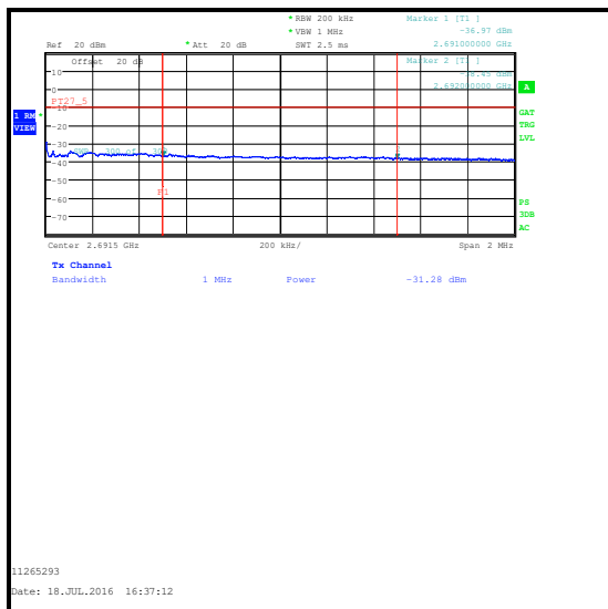
QPSK / 50 RB 0 Offset / 2691 to 2692 MHz / Integrated level
