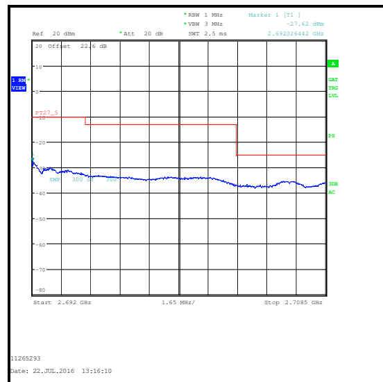
QPSK / 75 RB 0 Offset / 2692 to 2708.5 MHz
