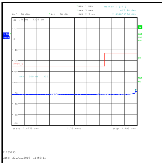
QPSK / 1 RB 74 Offset / 2477.5 to 2495 MHz
