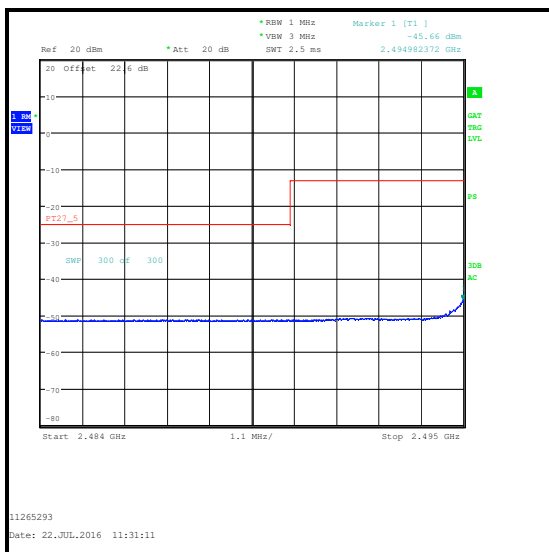
16QAM / 1 RB 49 Offset / 2484 to 2495 MHz
