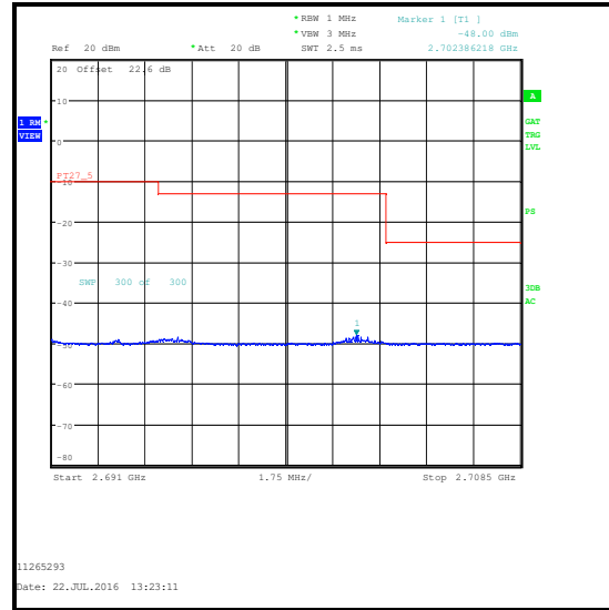
16QAM / 1 RB 0 Offset / 2691 to 2708.5 MHz
