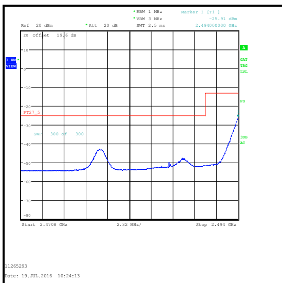
QPSK / 1 RB 0 Offset / 2470.8 to 2494 MHz
