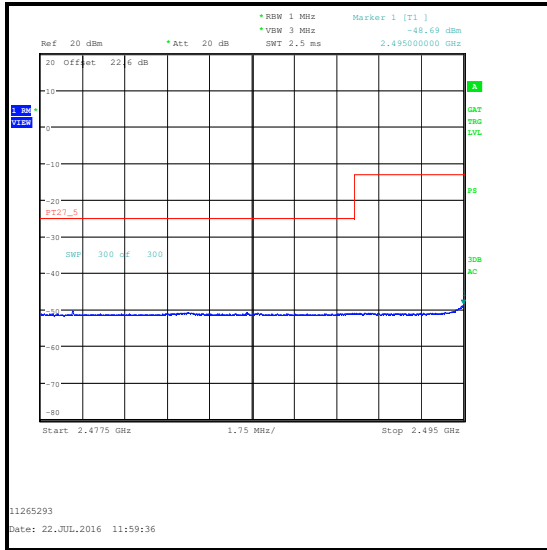
16QAM / 1 RB 24 Offset / 2477.5 to 2495 MHz
