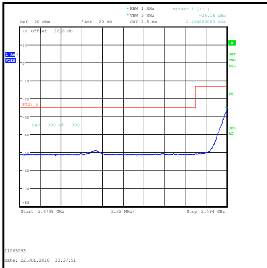
16QAM / 1 RB 0 Offset / 2470.8 to 2494 MHz
