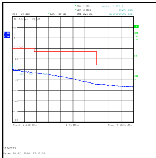
16QAM / 75 RB 0 Offset / 2692 to 2708.5 MHz
