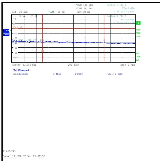
16QAM / 25 RB 0 Offset / 2691 to 2692 MHz / Integrated level
