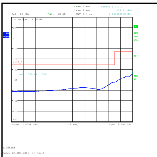
16QAM / 100 RB 0 Offset / 2470.8 to 2494 MHz
