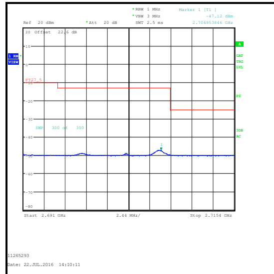
QPSK / 1 RB 0 Offset / 2691 to 2715.4 MHz
