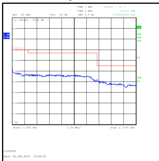
QPSK / 100 RB 0 Offset / 2692 to 2715.4 MHz
