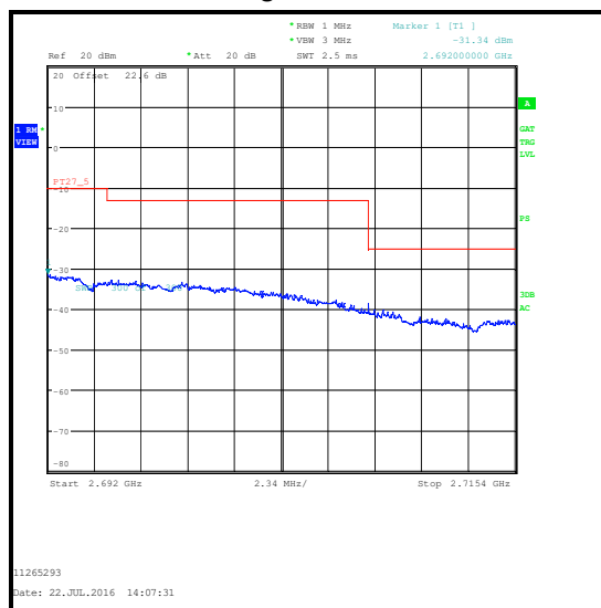
16QAM / 100 RB 0 Offset / 2692 to 2715.4 MHz
