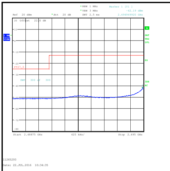
16QAM / 1 RB 24 Offset / 2488.75 to 2495 MHz
