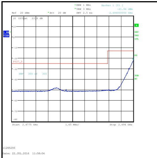
16QAM / 1 RB 0 Offset / 2477.5 to 2494 MHz
