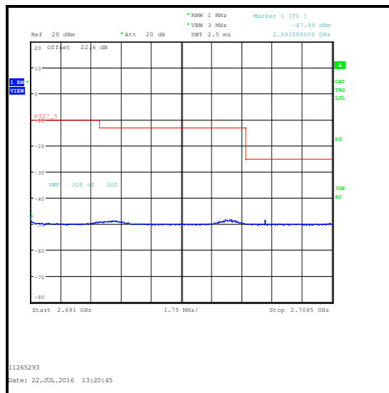
QPSK / 1 RB 0 Offset / 2691 to 2708.5 MHz
