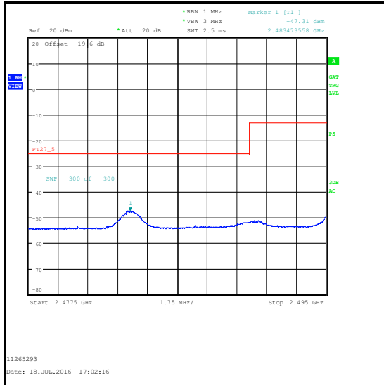
16QAM / 1 RB 74 Offset / 2477.5 to 2495 MHz
