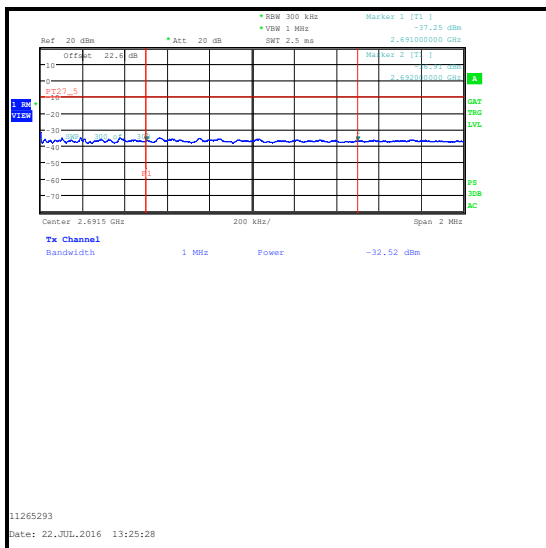
16QAM / 75 RB 0 Offset / 2691 to 2692 MHz / Integrated level
