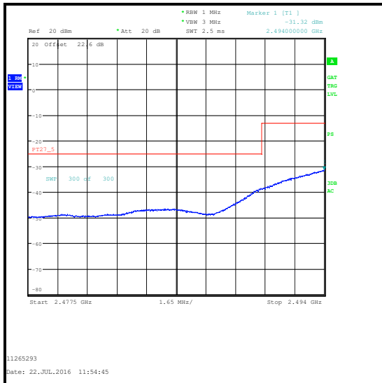
QPSK / 75 RB 0 Offset / 2477.5 to 2494 MHz
