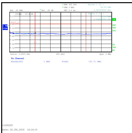
16QAM / 100 RB 0 Offset / 2691 to 2692 MHz / Integrated level
