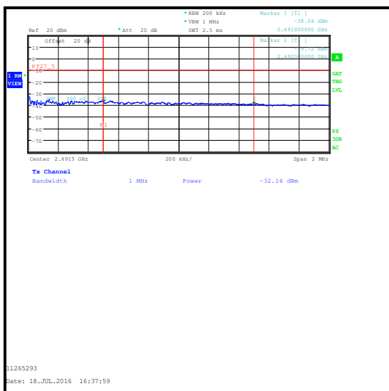
16QAM / 50 RB 0 Offset / 2691 to 2692 MHz / Integrated level
