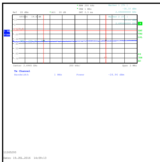
16QAM / 50 RB 0 Offset / 2494 to 2495 MHz / Integrated level
