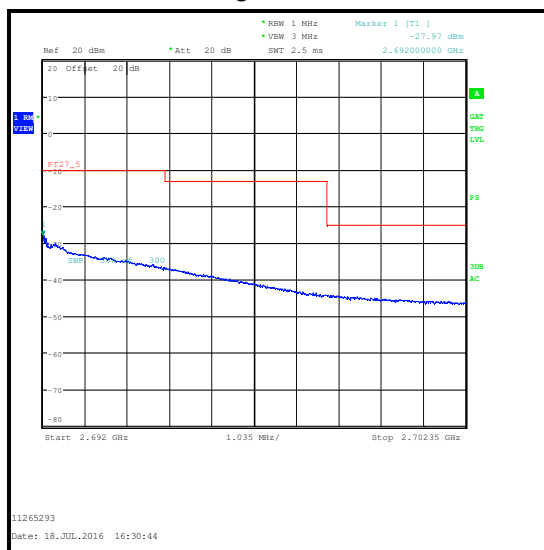
16QAM / 50 RB 0 Offset / 2692 to 2702.35 MHz
