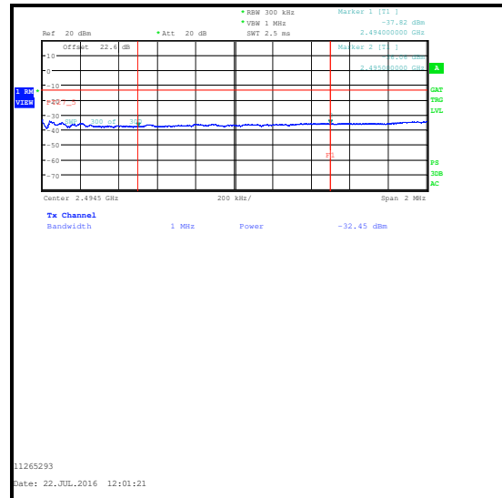
QPSK / 75 RB 0 Offset / 2494 to 2495 MHz / Integrated level
