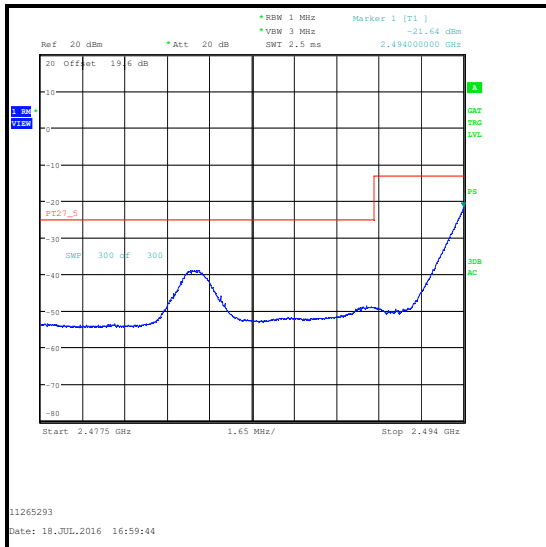
QPSK / 1 RB 0 Offset / 2477.5 to 2494 MHz
