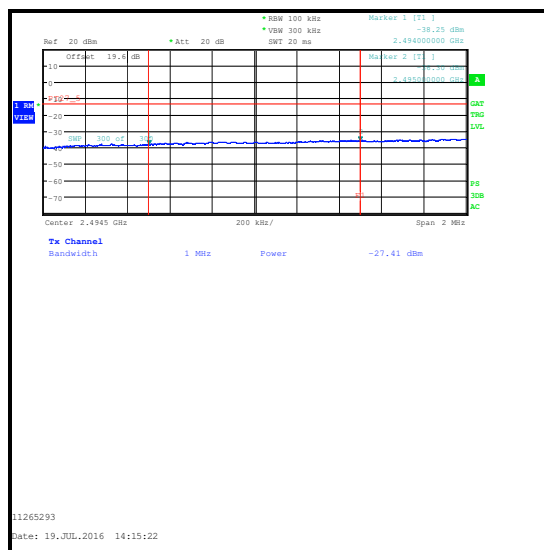
16QAM / 25 RB 0 Offset / 2494 to 2495 MHz / Integrated level
