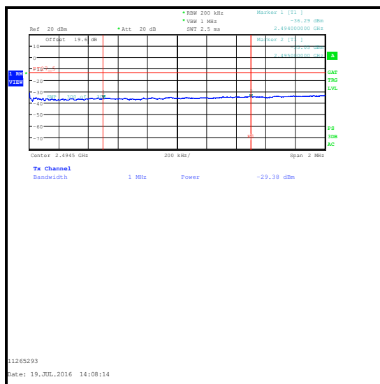
QPSK / 50 RB 0 Offset / 2494 to 2495 MHz / Integrated level
