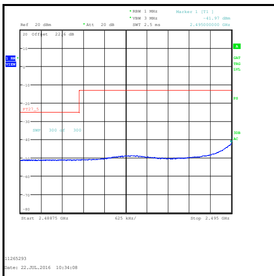
QPSK / 1 RB 24 Offset / 2488.75 to 2495 MHz
