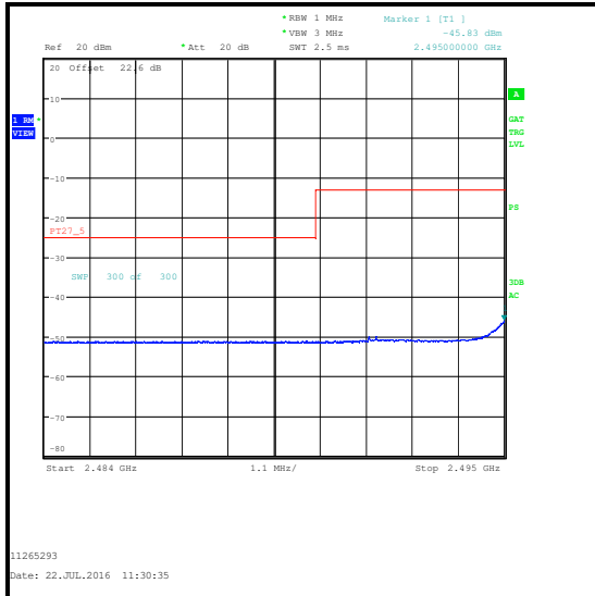
QPSK / 1 RB 49 Offset / 2484 to 2495 MHz
