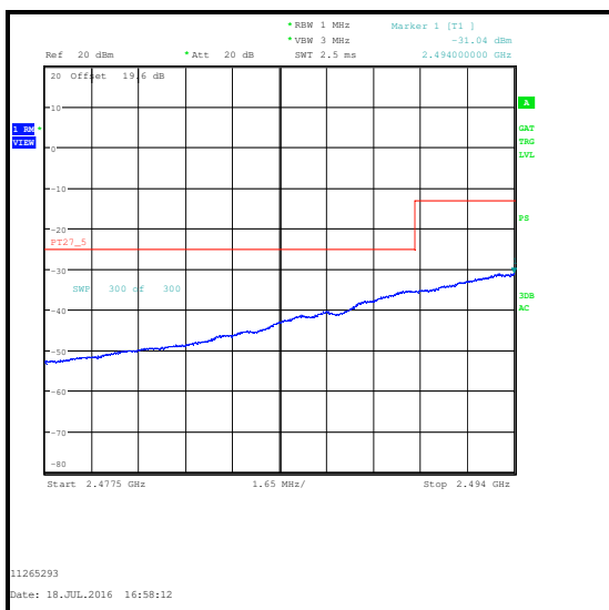
16QAM / 75 RB 0 Offset / 2477.5 to 2494 MHz
