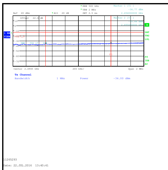
QPSK / 100 RB 0 Offset / 2494 to 2495 MHz / Integrated level
