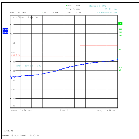
16QAM / 50 RB 0 Offset / 2484 to 2494 MHz
