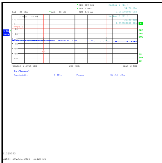
QPSK / 100 RB 0 Offset / 2691 to 2692 MHz / Integrated level
