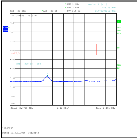
16QAM / 1 RB 24 Offset / 2470.8 to 2495 MHz
