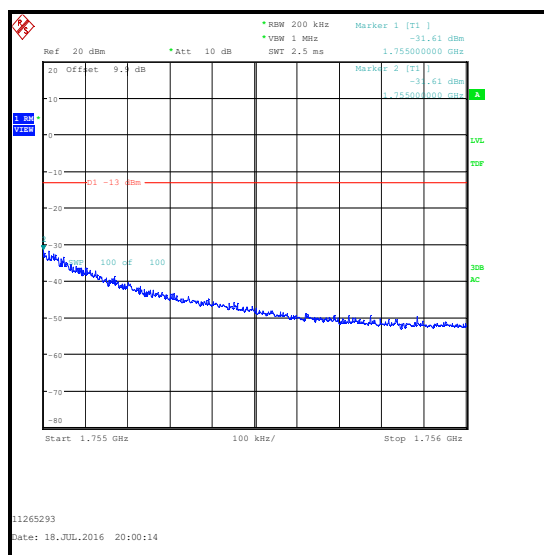
16QAM / 1 RB 74 offset / Upper Band Edge
