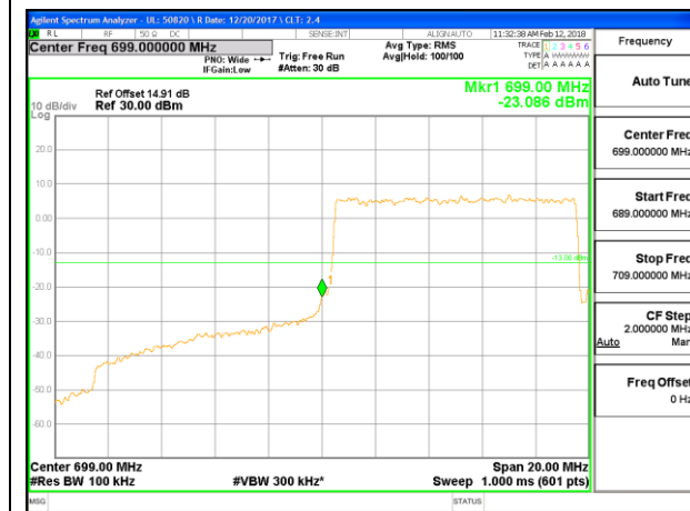
LTE B12 10MHz QPSK Low Channel RB50-0
