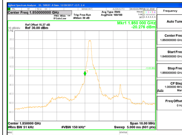
LTE B25 5MHz 16QAM Low Channel RB1-0
