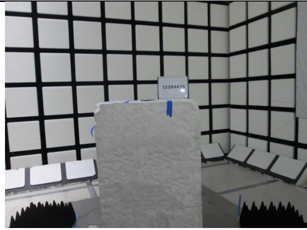
X-Axis (BACK)
